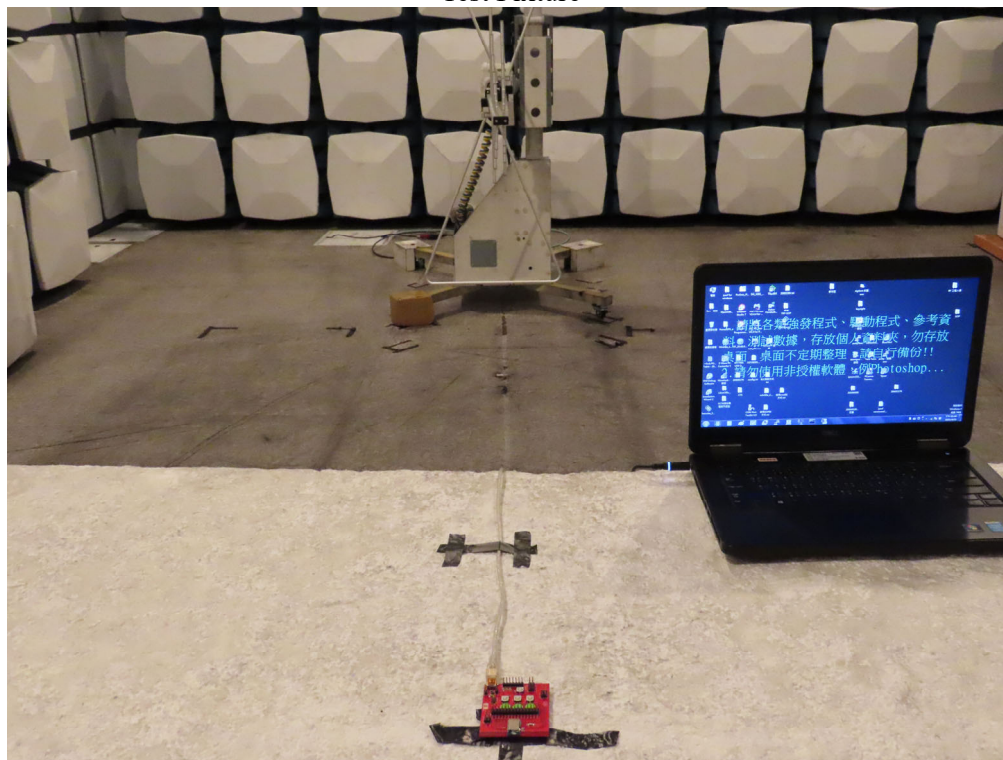
Test Fixture
