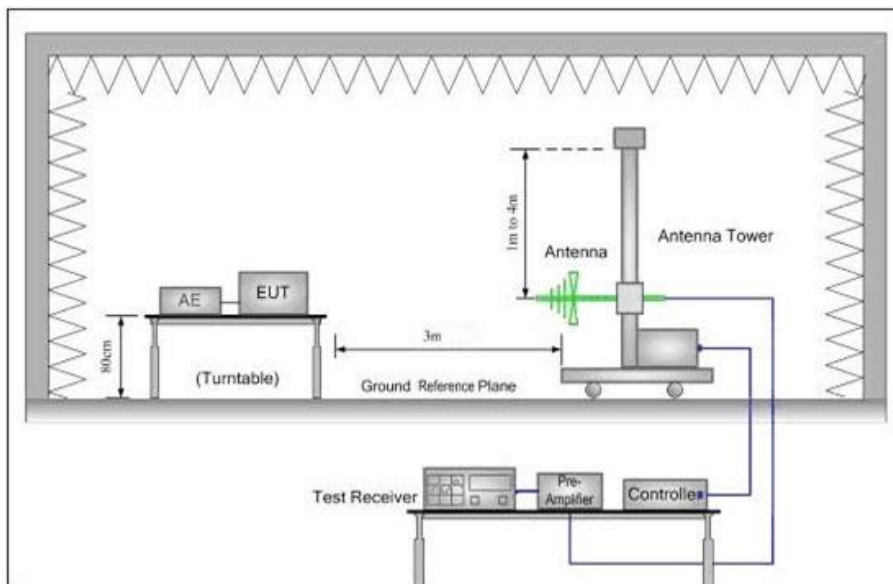
30MHz-1GHz
