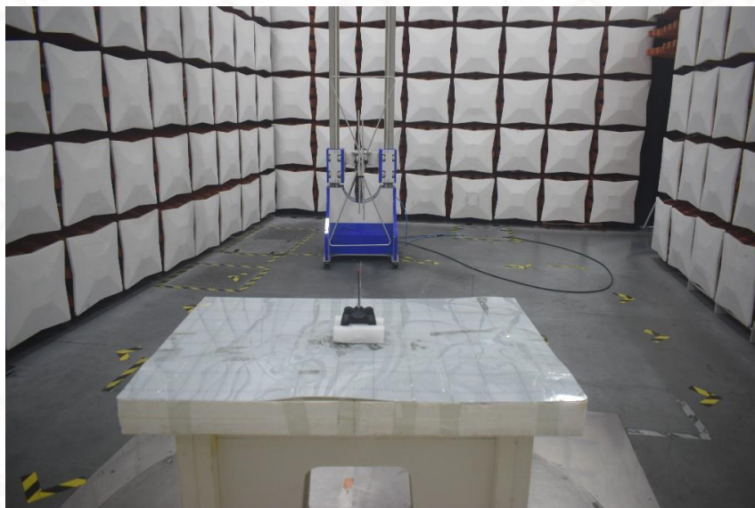
TX 30MHz~1GHz
