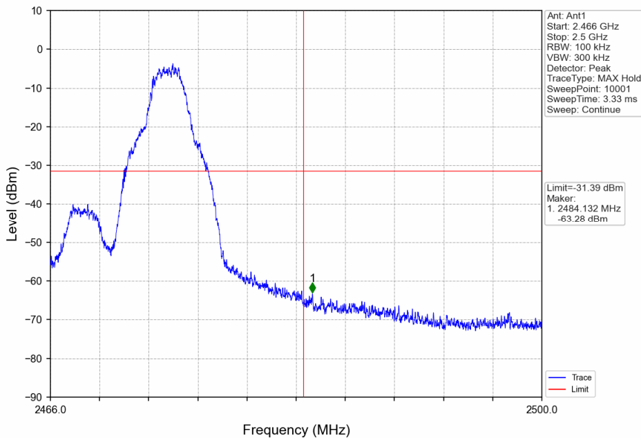
1_HCH_2474MHz_Ant1_NTNV
