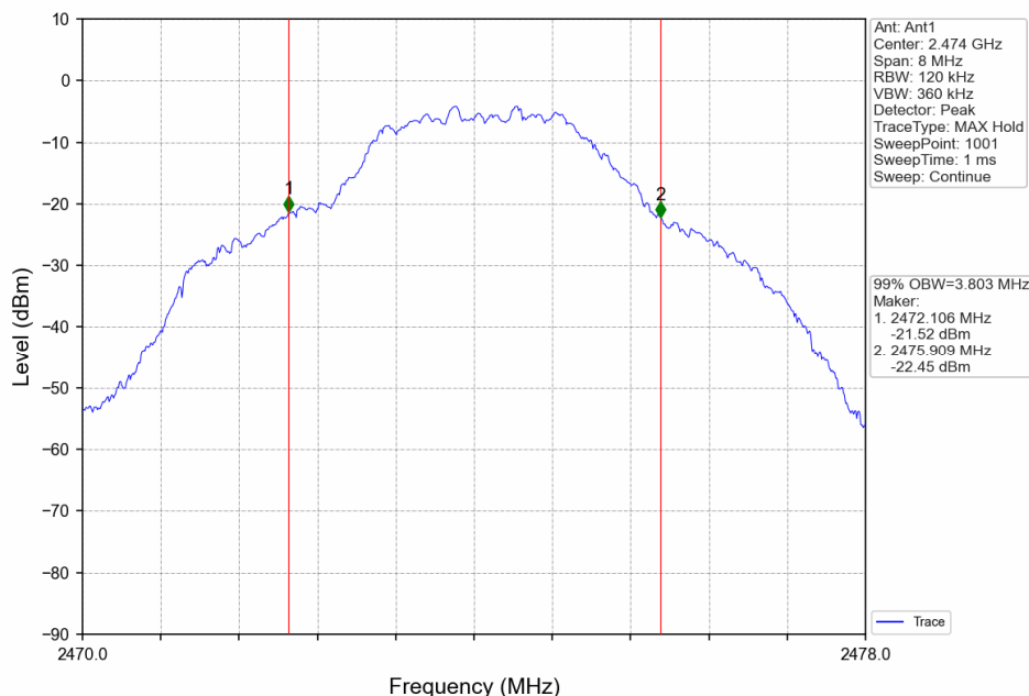
1_HCH_2474MHz_Ant1_NTNV
