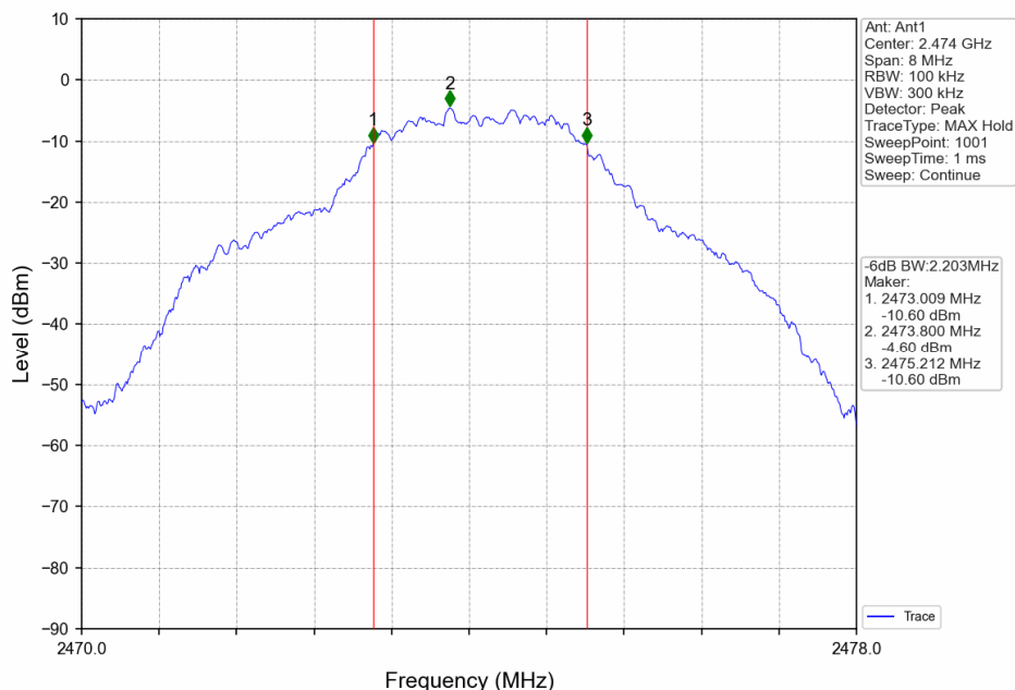
1_HCH_2474MHz_Ant1_NTNV
