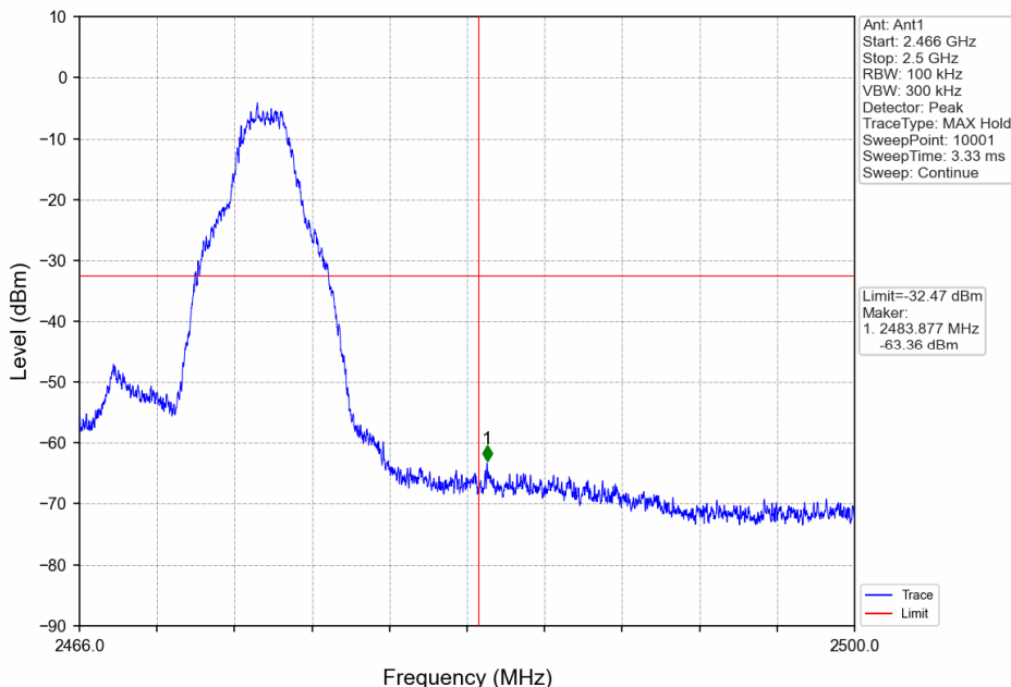
1_HCH_2474MHz_Ant1_NTNV
