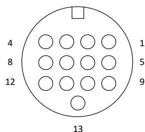
13-pin DIN female connector
