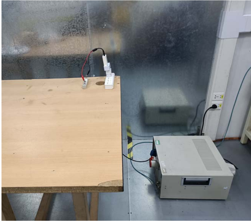
Conducted Emission Test Setup:
