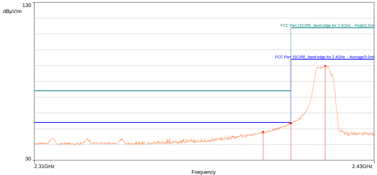
2412MHz Vertical
