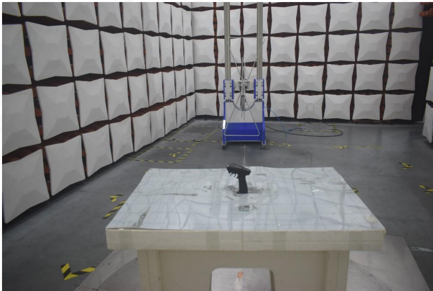
TX 30MHz~1GHz
