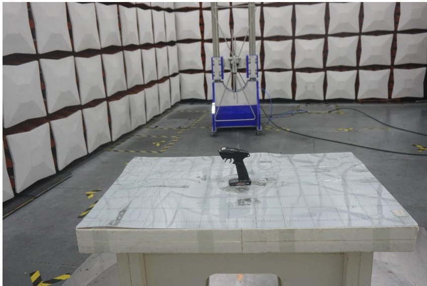
TX 30MHz~1GHz
