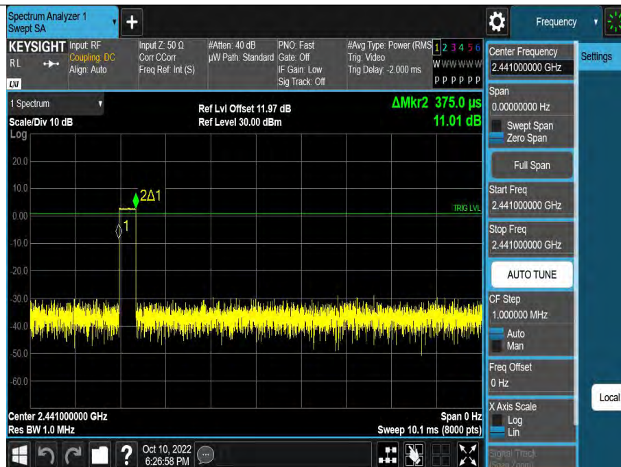
DH1-Ant1-Hop-0.375-320
