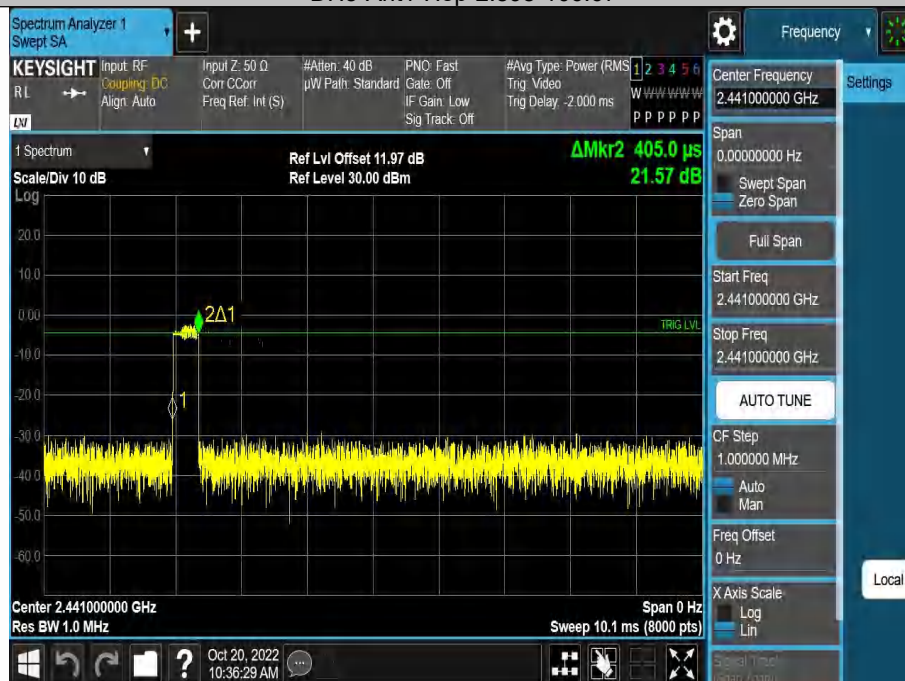
2DH1-Ant1-Hop-0.405-320
