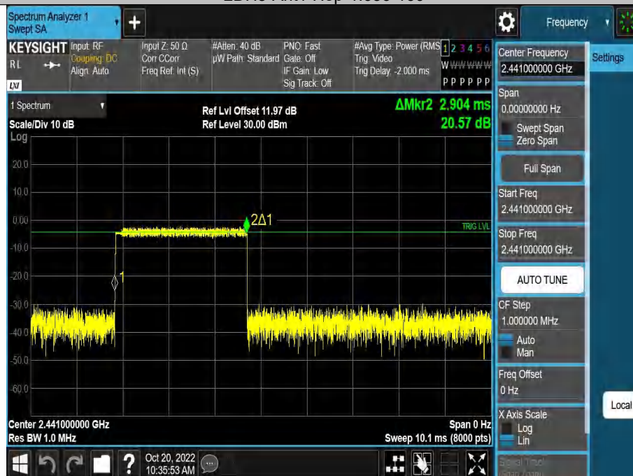
2DH5-Ant1-Hop-2.904-106.67
