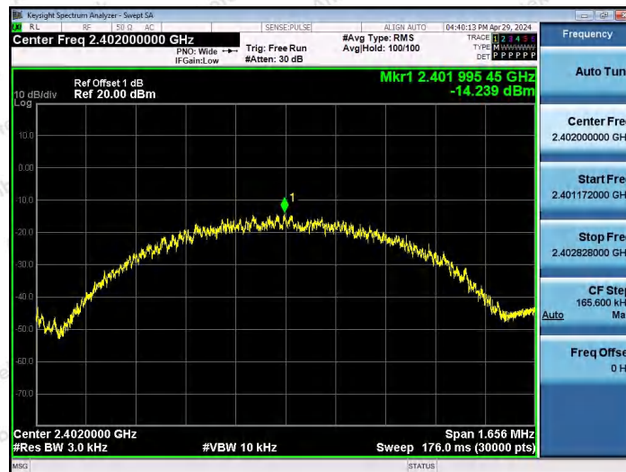
BLE_1M-Ant1-2402-PASS
