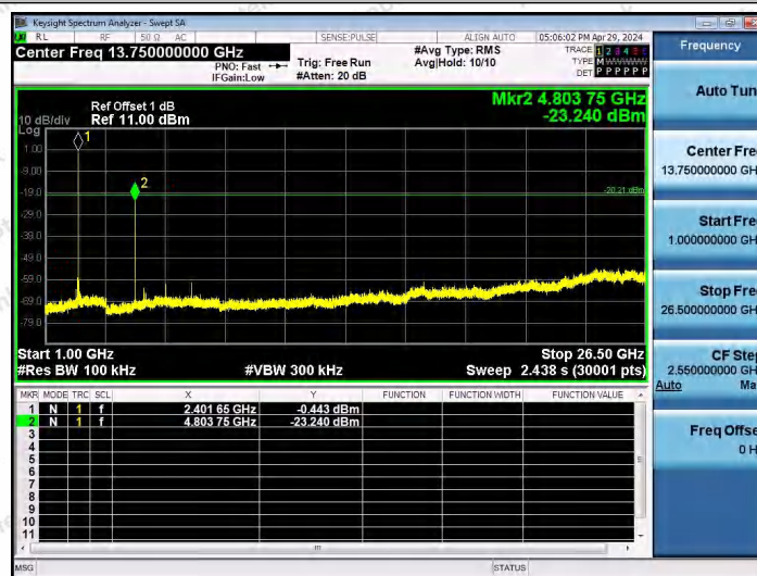
BLE_2M-Ant1-2402-1000~26500-PASS
