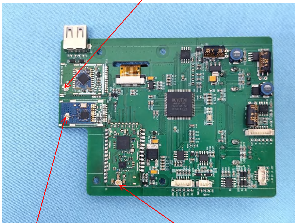
SRD RX Antenna Interface
