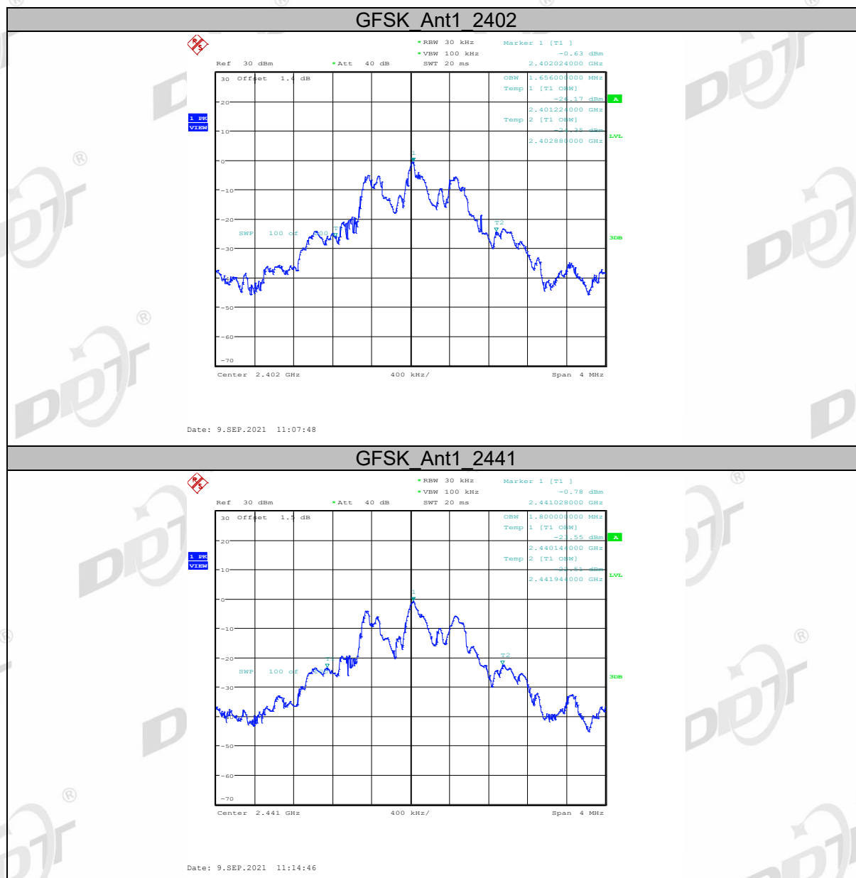
Test Graphs 99% bandwidth
