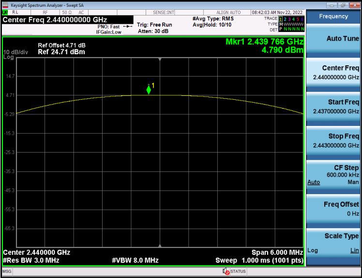
Peak_Output_Power_BLE_1Mbps_2440
