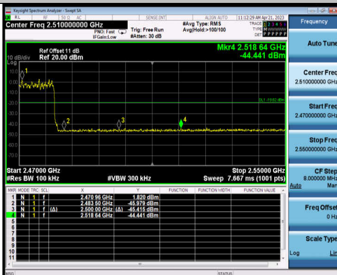
3DH5_Ant1_High_Hop_2480
