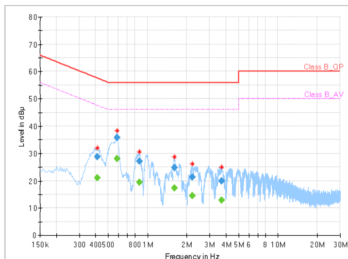
Full Spectrum
