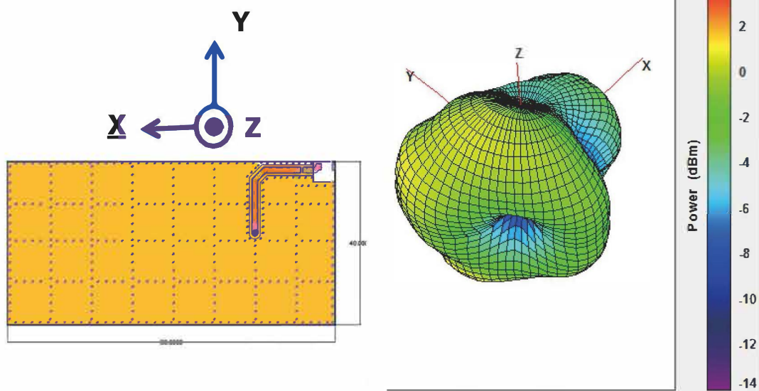
Radiation Pattern
