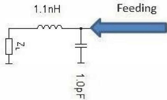
Suggested Matching Circuit
