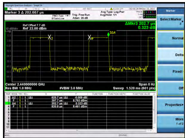
GFSK(BLE 2Mbps)
