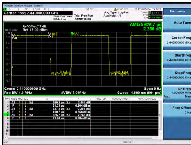
GFSK(BLE 1Mbps)
