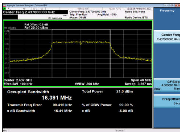
6dB Bandwidth-802.11g,2437MHz,Ant0
