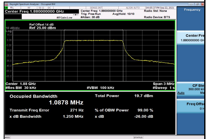
FDD02_MidRange_3_1880_Q16
