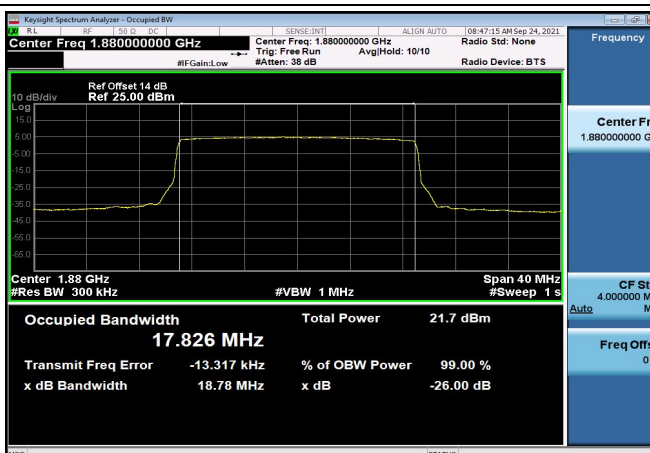
FDD02_MidRange_20_1880_QPSK
