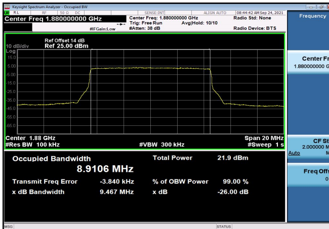
FDD02_MidRange_15_1880_QPSK
