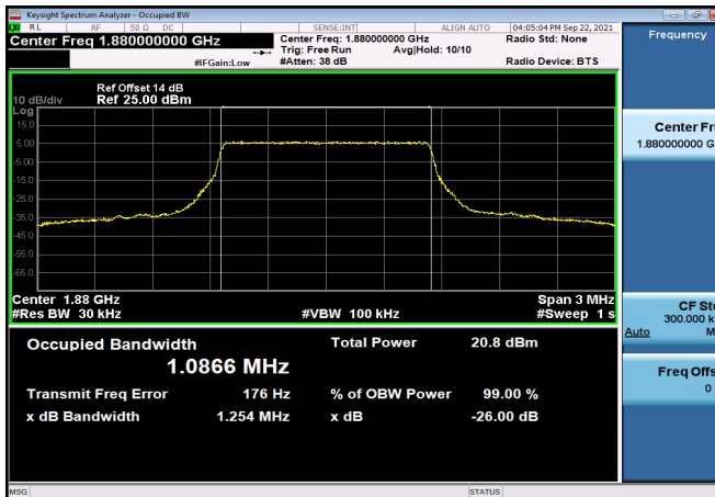
FDD02_MidRange_3_1880_QPSK
