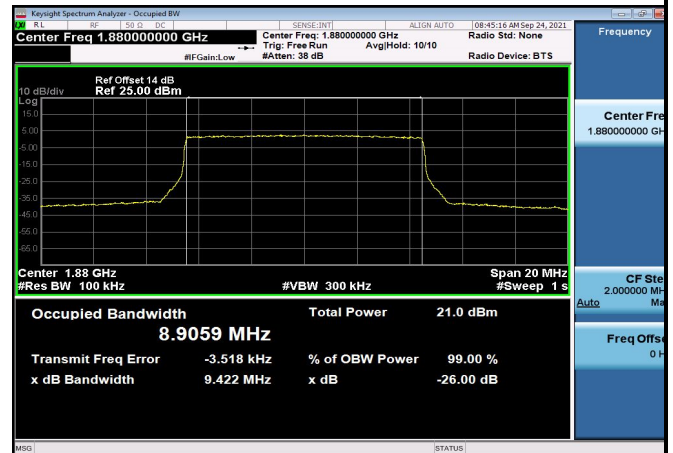
FDD02_MidRange_15_1880_Q16
