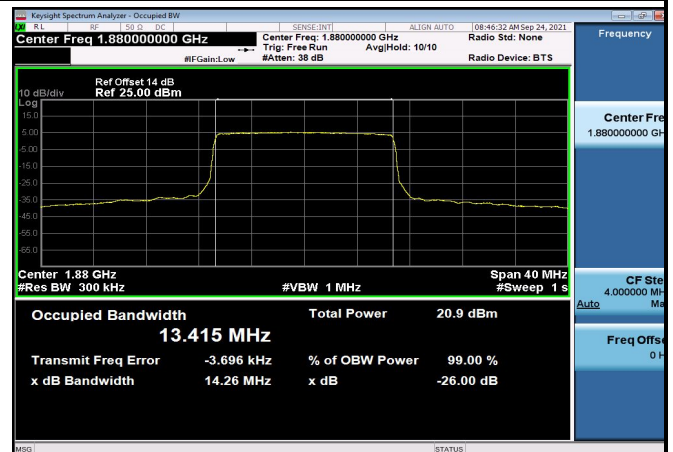
FDD02_MidRange_20_1880_Q16
