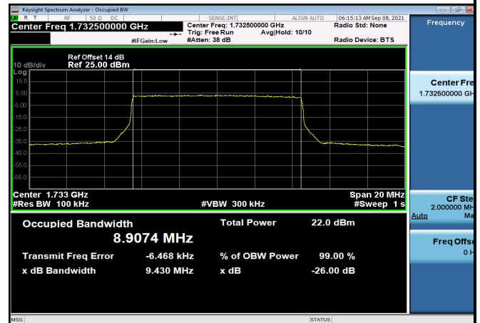
FDD04_MidRange_15_1732.5_Q16
