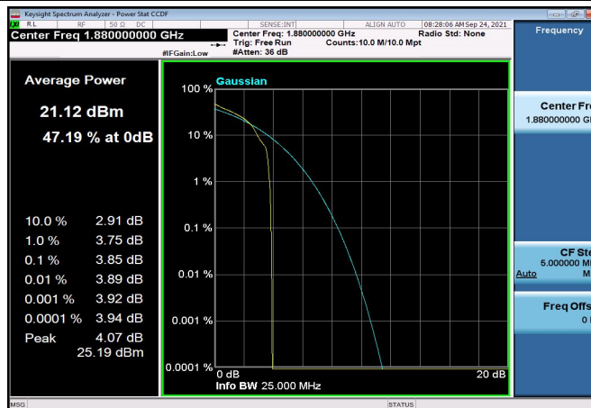
FDD02_HighRange_20MHz_1900_OneRB _high_Q16
