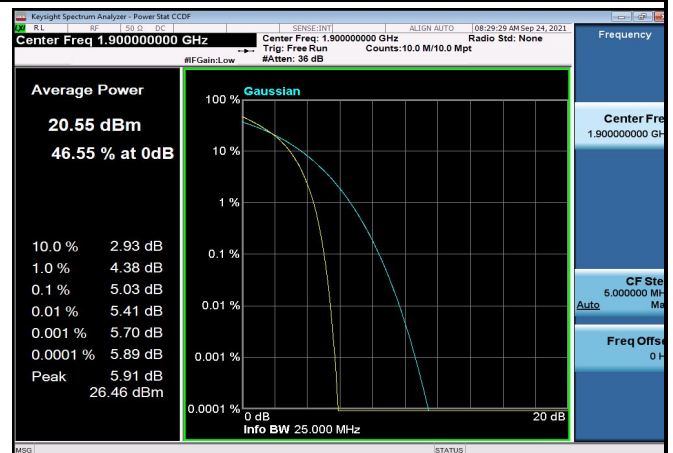
FDD02_HighRange_20MHz_1900_fullRB _Q16
