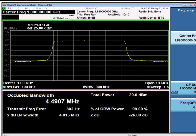
FDD02_MidRange_5_1880_QPSK
