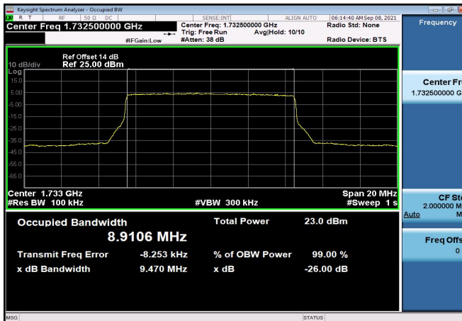
FDD04_MidRange_15_1732.5_QPSK
