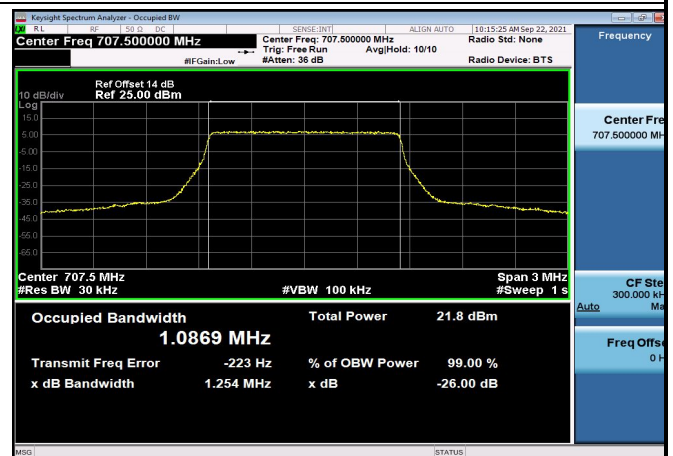
FDD12_MidRange_1.4MHz_707.5MHz_Q16
