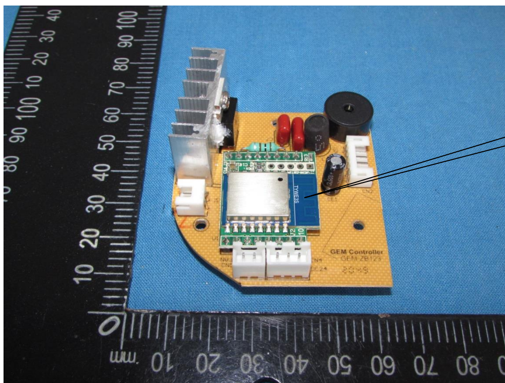
WIFI Antenna
