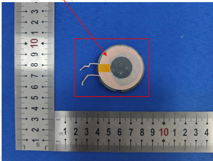
Coil Antenna
