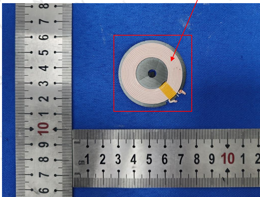
Coil Antenna-Earphone
