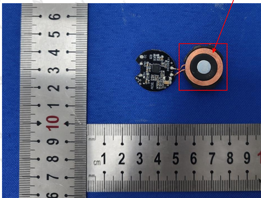
Coil Antenna-Watch
