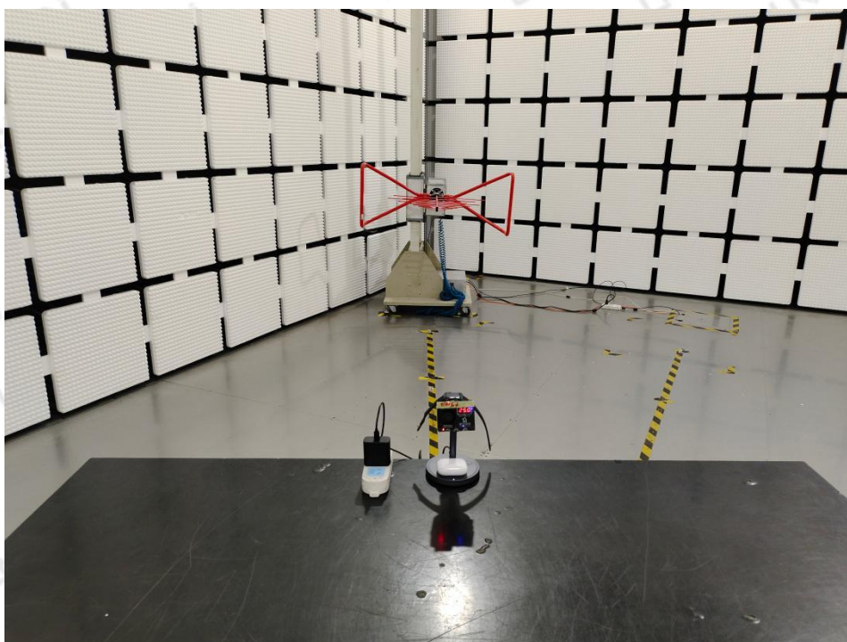
30M-1G
