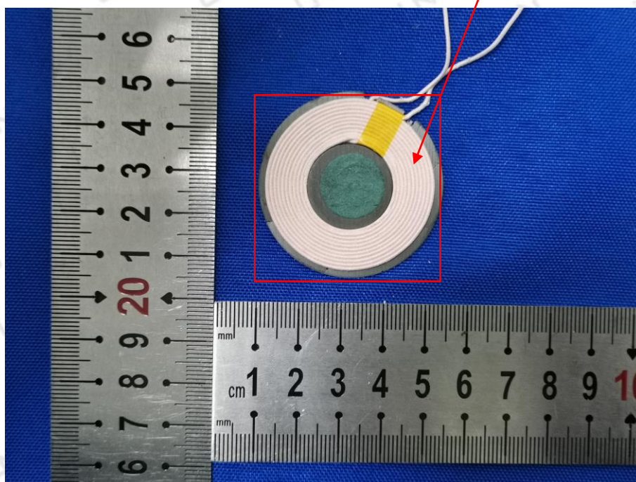
Coil Antenna-Phone
