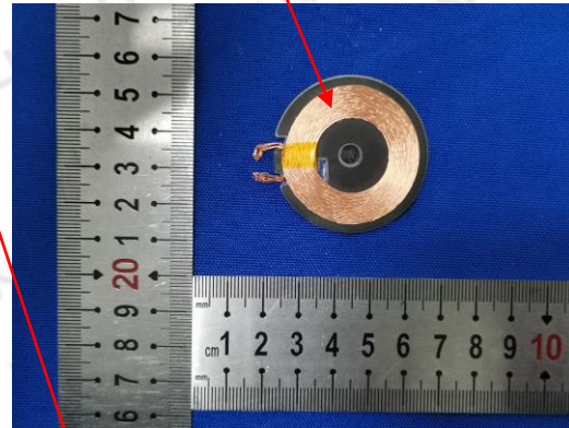
ANTENNA 2:
