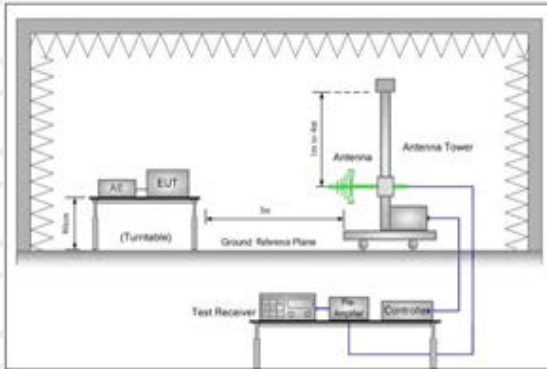
Figure 1. Below 30MHz
