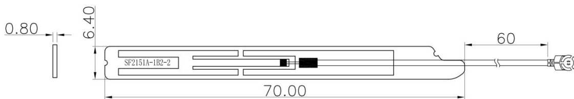
Antenna Top View [With Ruler]
