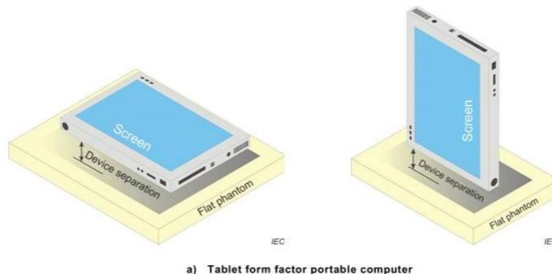
a) Tablet form factor portable computer
