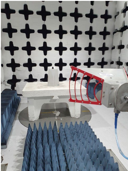
1GHz-15GHz test setup.
