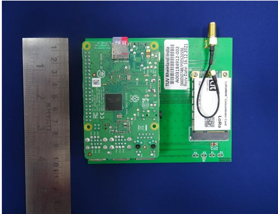
Test Supporting board and EUT Front view
