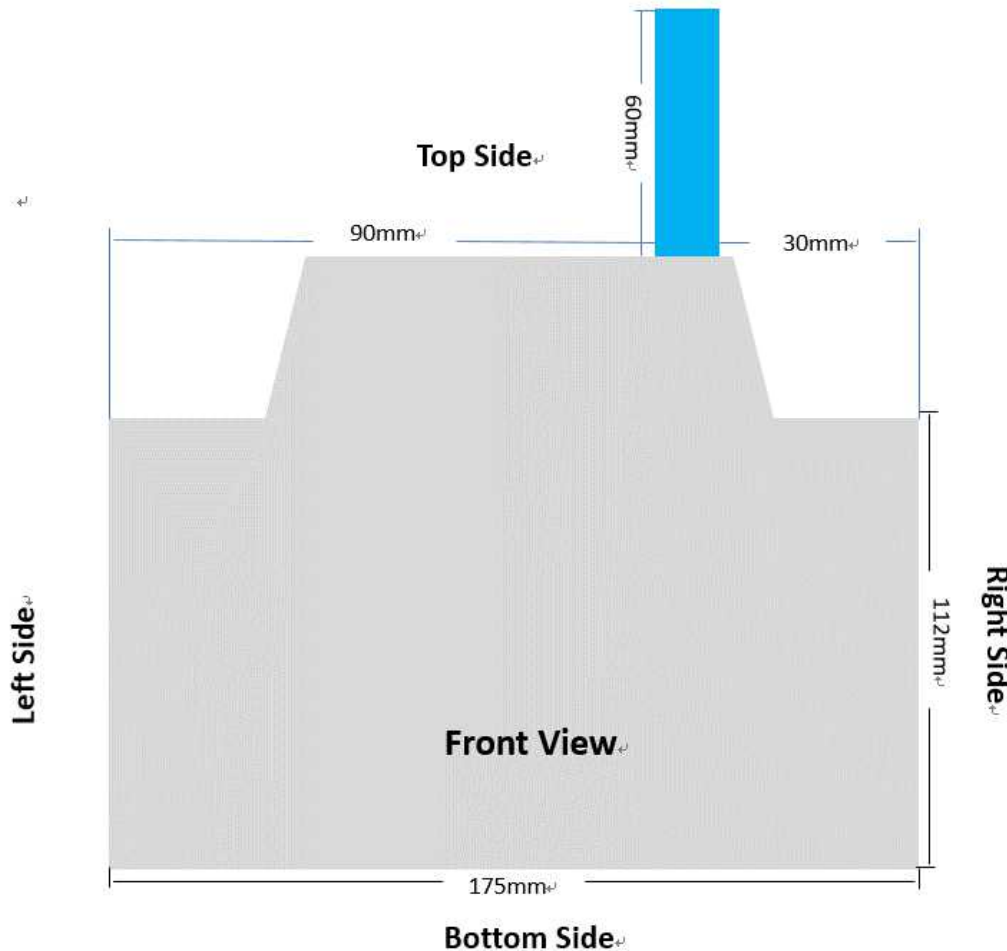
EUT FRONT VIEW
