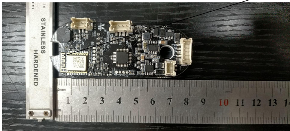
INTERNAL PHOTO OF SAMPLE PCB
