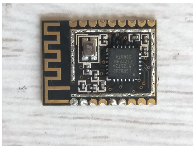
INTERNAL PHOTO OF SAMPLE PCB
