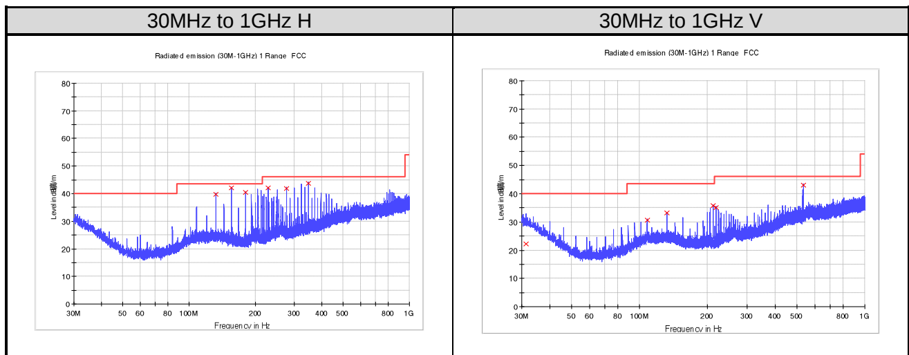
Figure 12: Radiated Spurious Emission, TM1, 30MHz to 1GHz
