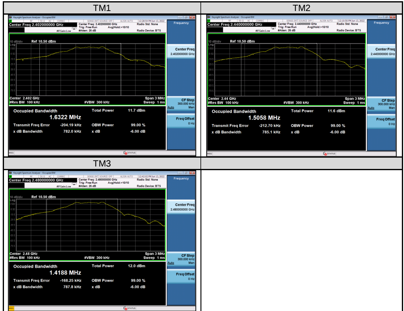
Figure 1: 6dB Bandwidth
