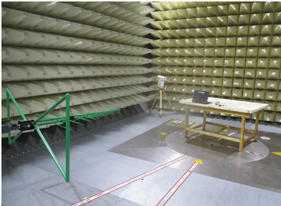
30MHz to 1GHz
