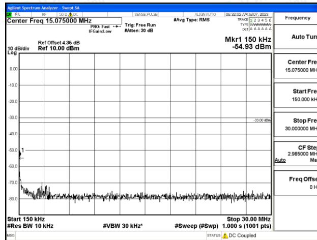
Band4_10MHz_16QAM_20350_1RB#0_0.15~30_0.15~30
