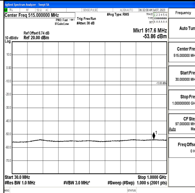
Band4_10MHz_16QAM_20350_1RB#0_30~1000_30~1000
