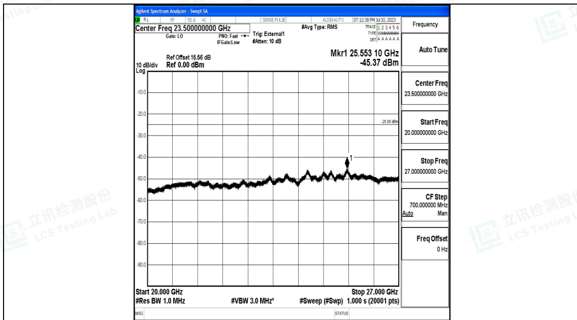
Band41_15MHz_16QAM_39725_1RB#0_20000~27000_20000~27000
