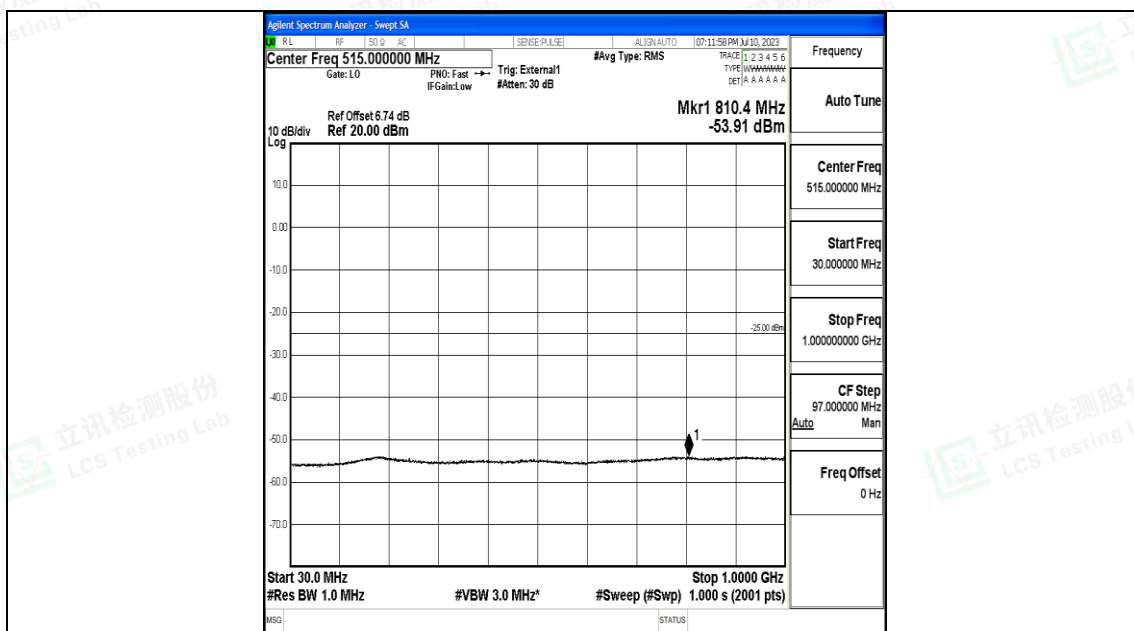
Band41_15MHz_16QAM_39725_1RB#0_30~1000_30~1000
