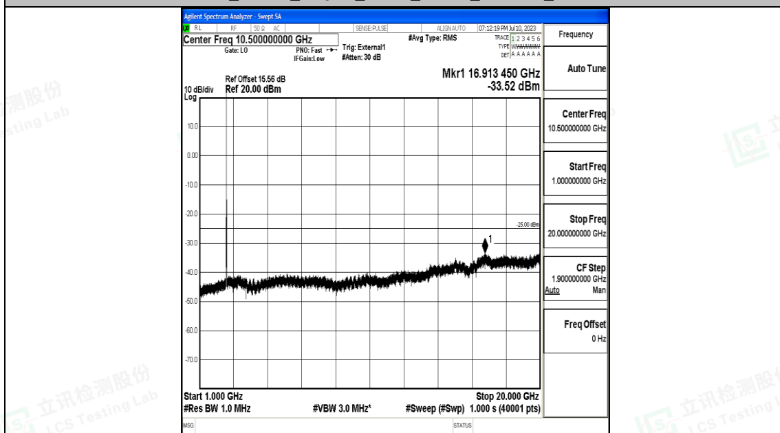
Band41_15MHz_16QAM_39725_1RB#0_1000~20000_1000~20000
