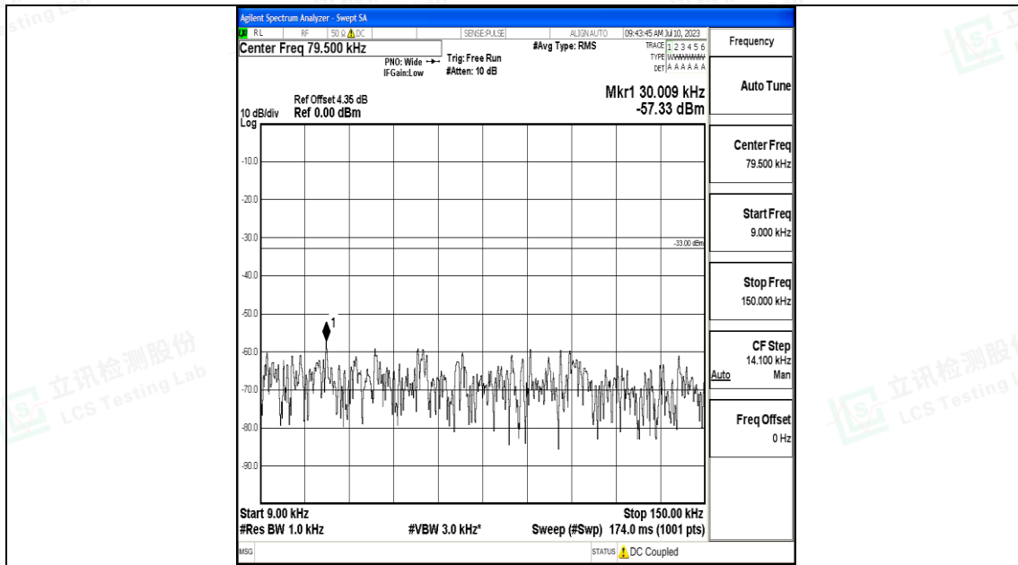
Band71_20MHz_16QAM_133222_1RB#0_0.009~0.15_0.009~0.15
