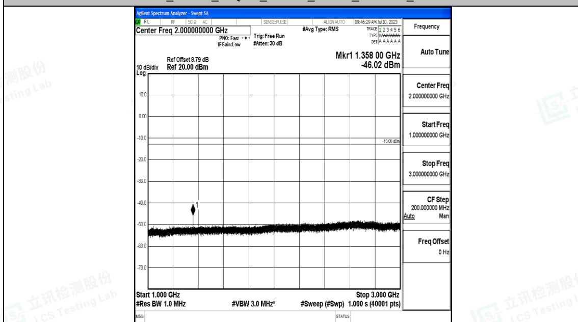
Band71_20MHz_16QAM_133372_1RB#0_1000~3000_1000~3000
