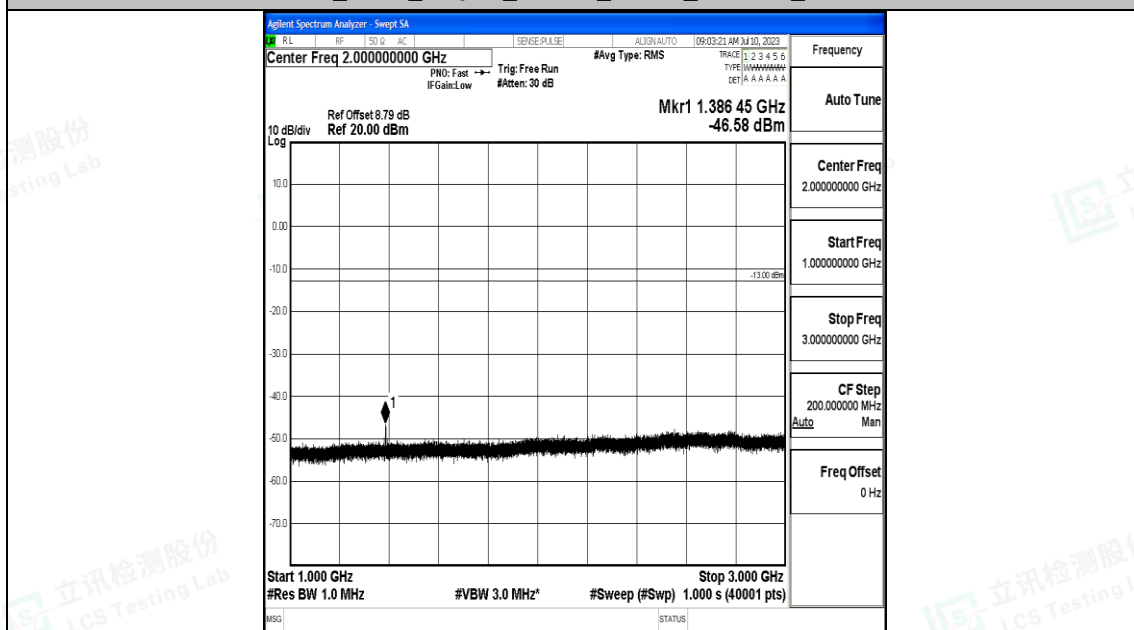
Band71_5MHz_16QAM_133447_1RB#0_1000~3000_1000~3000
