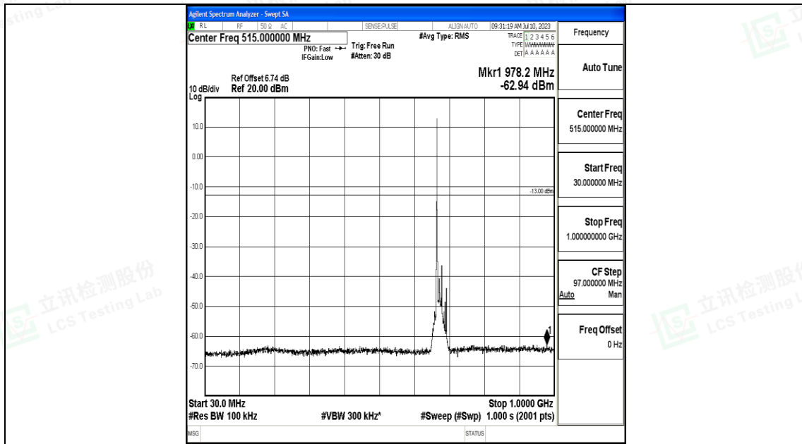
Band71_15MHz_16QAM_133297_1RB#0_30~1000_30~1000
