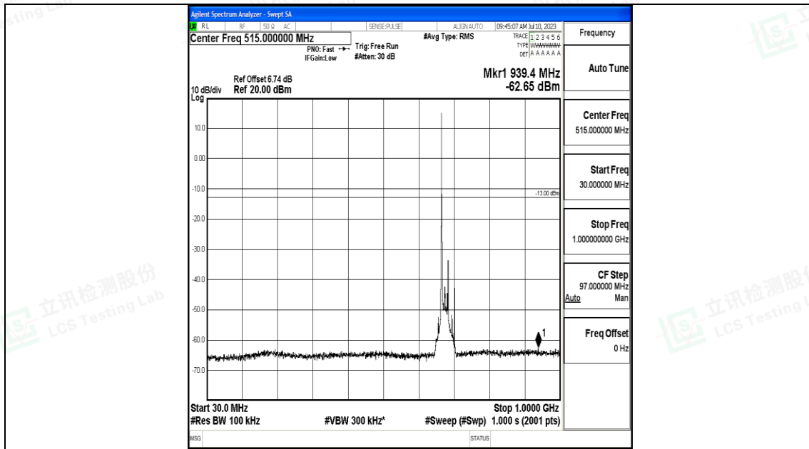
Band71_20MHz_16QAM_133322_1RB#0_30~1000_30~1000
