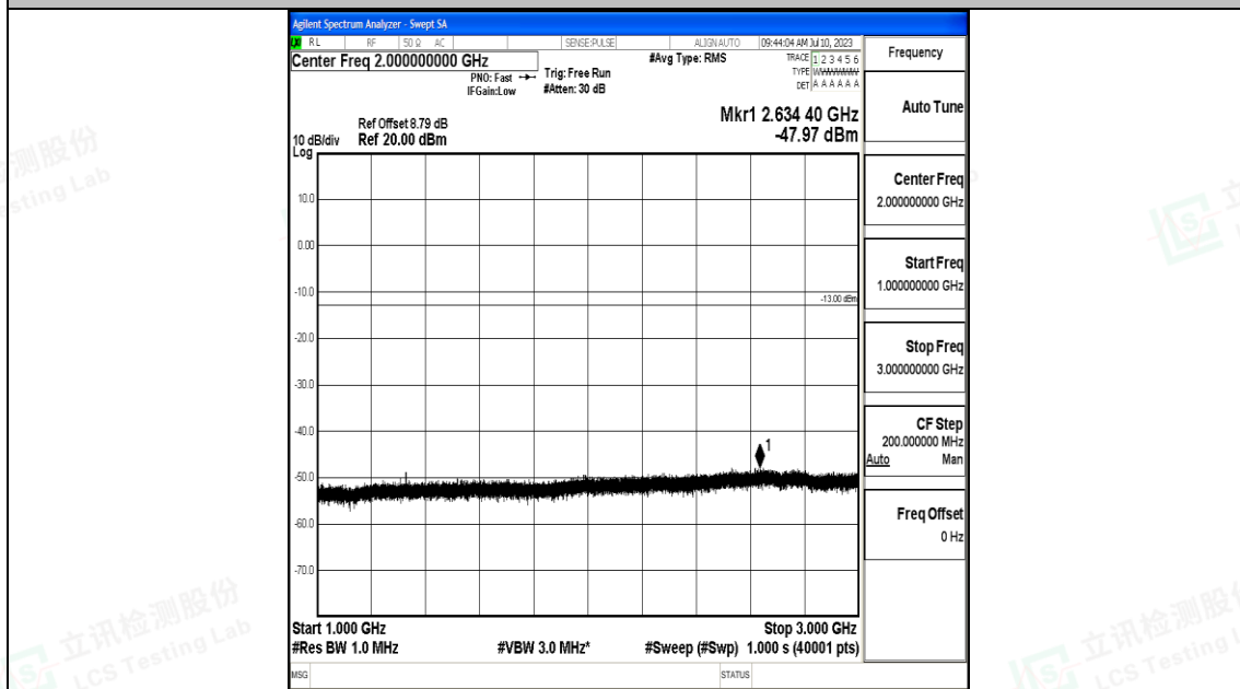
Band71_20MHz_16QAM_133222_1RB#0_1000~3000_1000~3000
