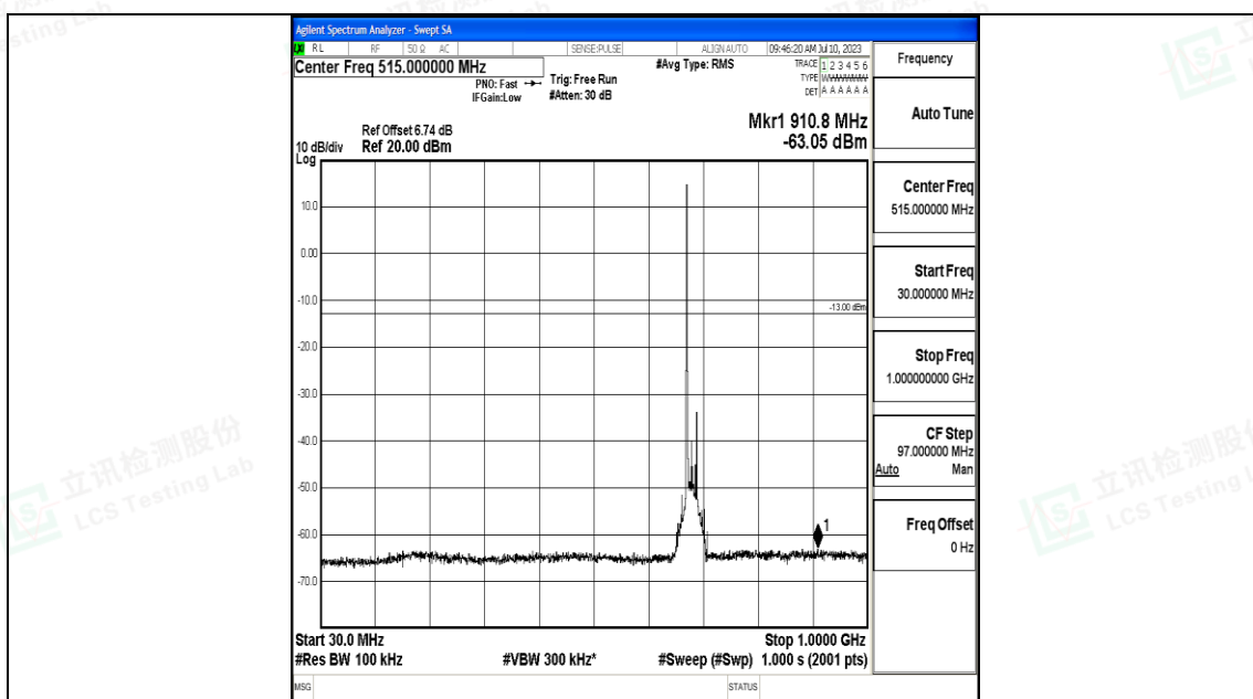
Band71_20MHz_16QAM_133372_1RB#0_30~1000_30~1000
