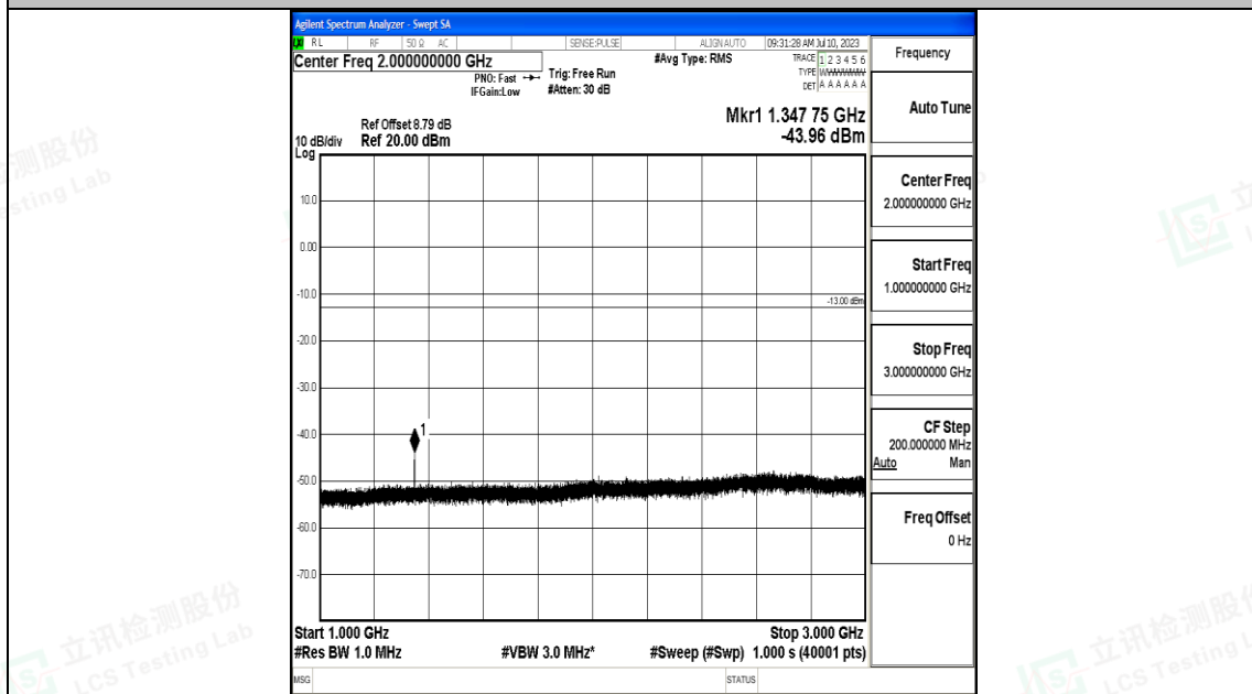
Band71_15MHz_16QAM_133297_1RB#0_1000~3000_1000~3000
