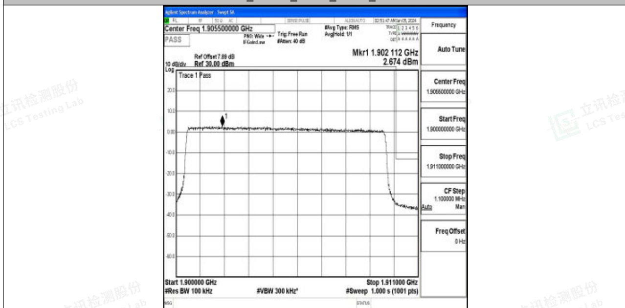
Band2_10MHz_16QAM_19150_50RB#0
