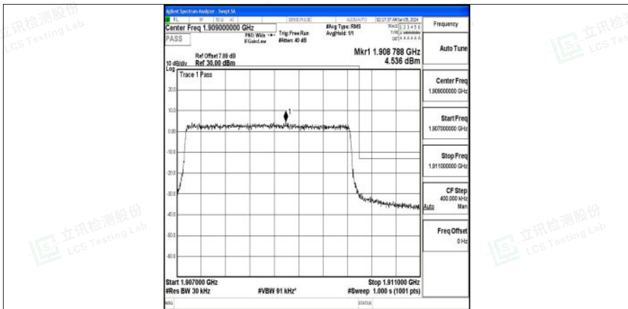
Band2_3MHz_QPSK_19185_15RB#0
