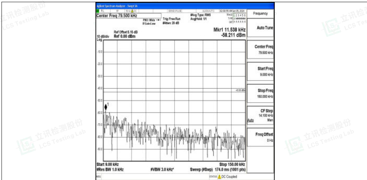
Band2_1.4MHz_16QAM_19193_1RB#0_0.009~0.15_0.009~0.15
