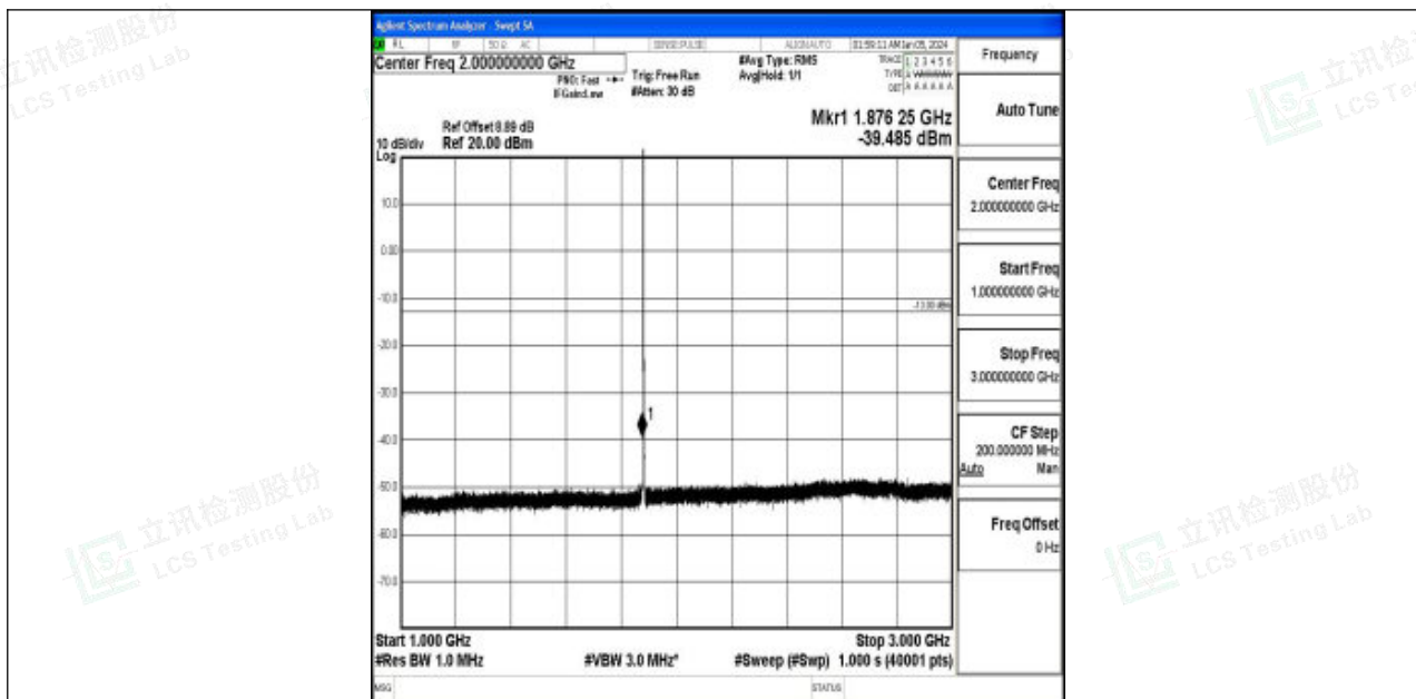
Band2_1.4MHz_QPSK_18900_1RB#0_1000~3000_1000~3000
