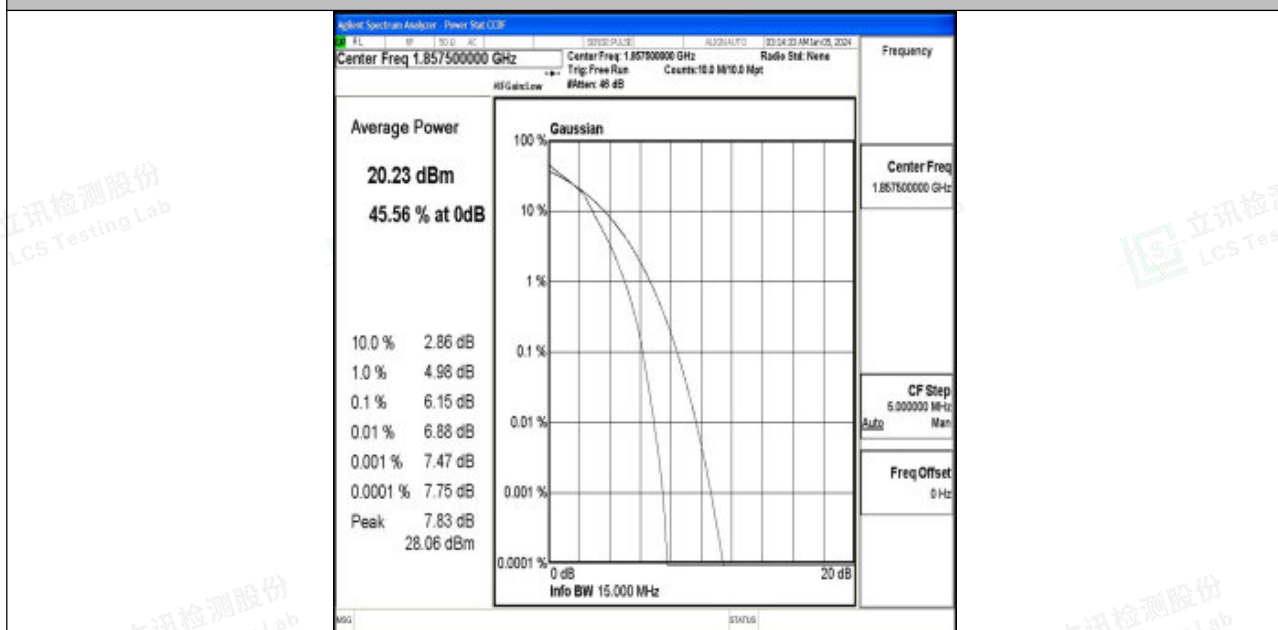
Band2-15MHz-16QAM-18675-75RB#0-PASS
