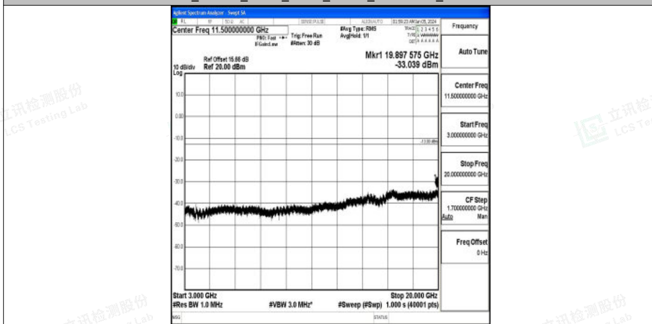
Band2_1.4MHz_QPSK_18900_1RB#0_3000~20000_3000~20000
