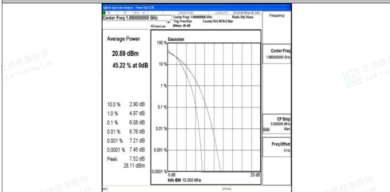
Band2-15MHz-16QAM-18900-75RB#0-PASS
