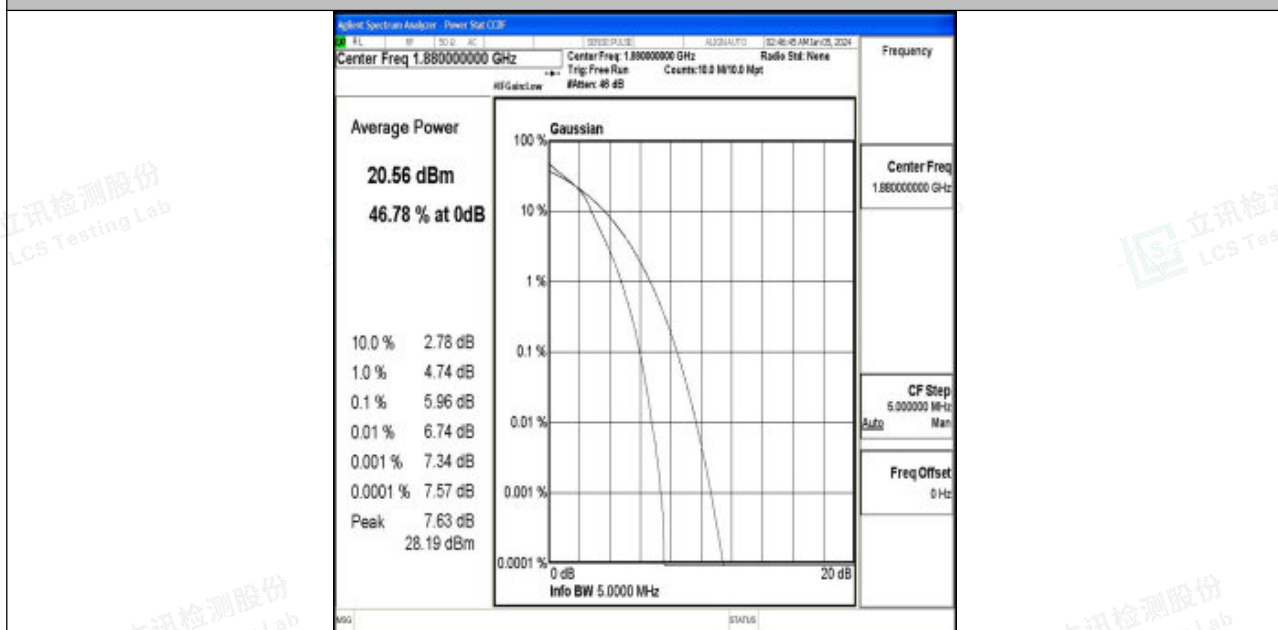
Band2-5MHz-16QAM-18900-25RB#0-PASS
