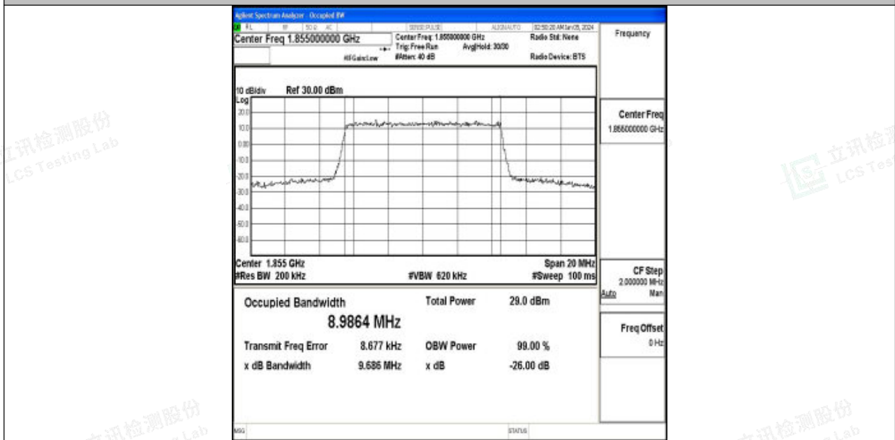
Band2-10MHz-16QAM-18650-50RB#0-PASS
