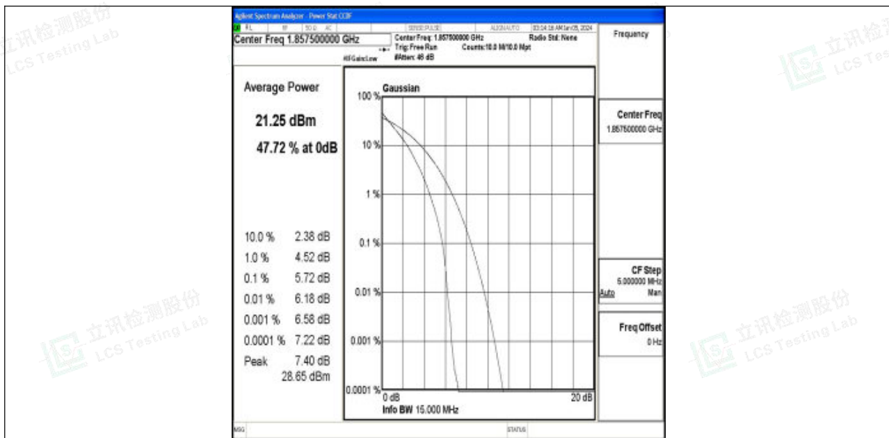
Band2-15MHz-QPSK-18675-75RB#0-PASS
