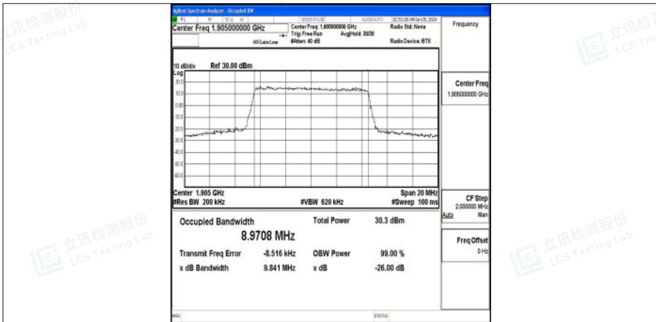
Band2-10MHz-QPSK-19150-50RB#0-PASS
