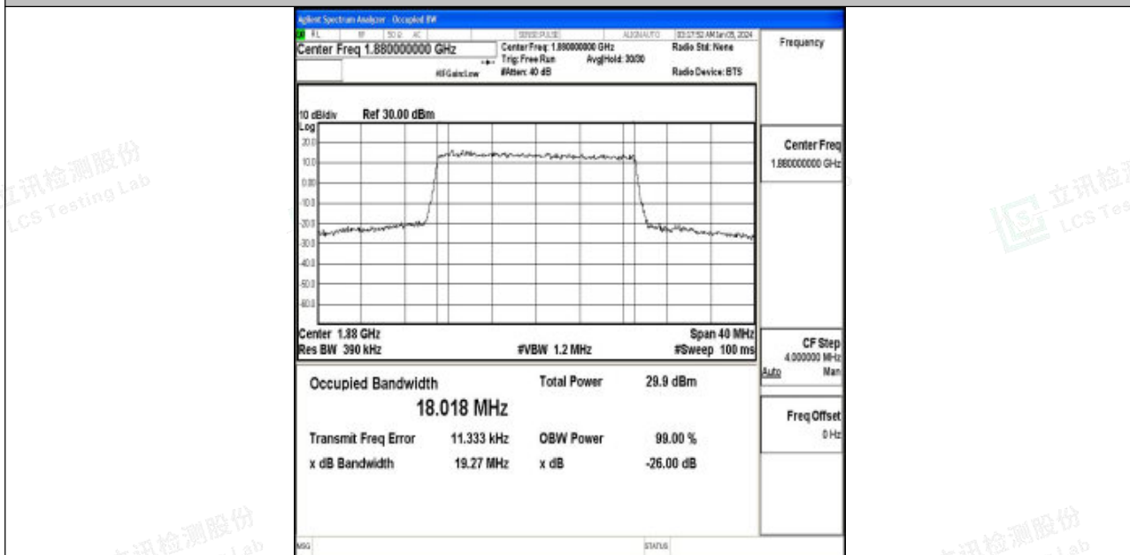
Band2-20MHz-16QAM-18900-100RB#0-PASS
