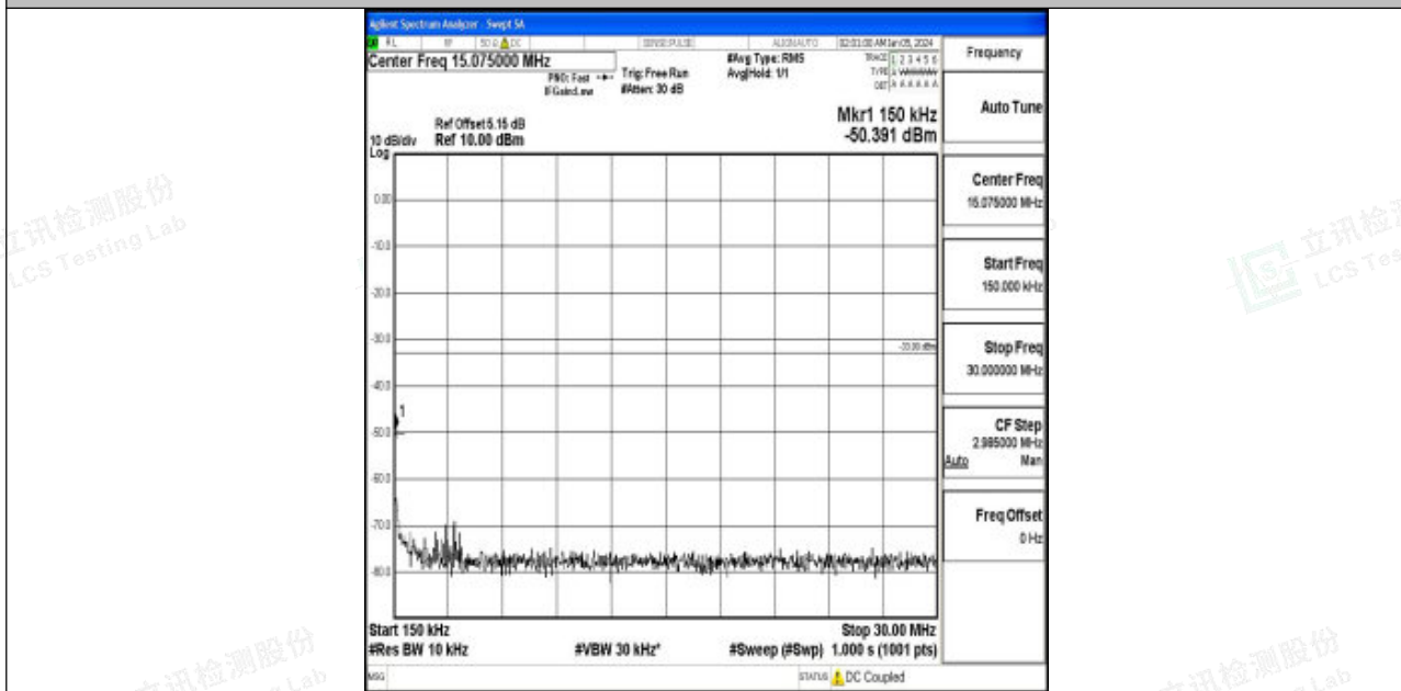
Band2_1.4MHz_16QAM_19193_1RB#0_0.15~30_0.15~30
