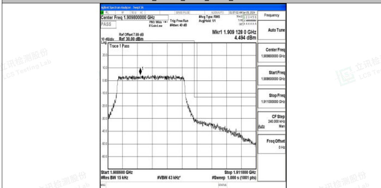
Band2_1.4MHz_16QAM_19193_6RB#0
