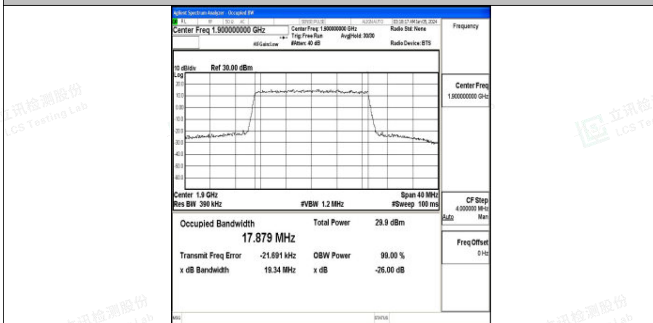
Band2-20MHz-16QAM-19100-100RB#0-PASS
