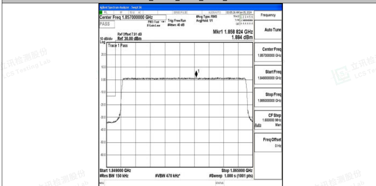
Band2_15MHz_16QAM_18675_75RB#0
