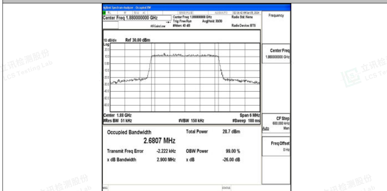
Band2-3MHz-16QAM-18900-15RB#0-PASS
