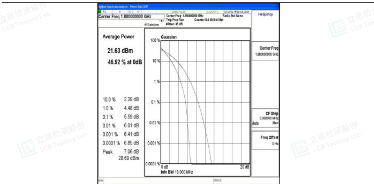
Band2-15MHz-QPSK-18900-75RB#0-PASS
