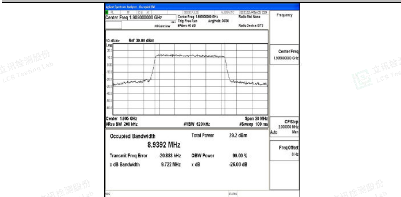
Band2-10MHz-16QAM-19150-50RB#0-PASS
