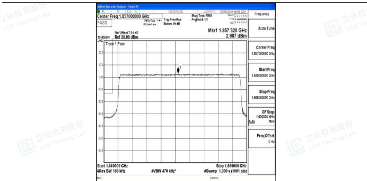
Band2_15MHz_QPSK_18675_75RB#0
