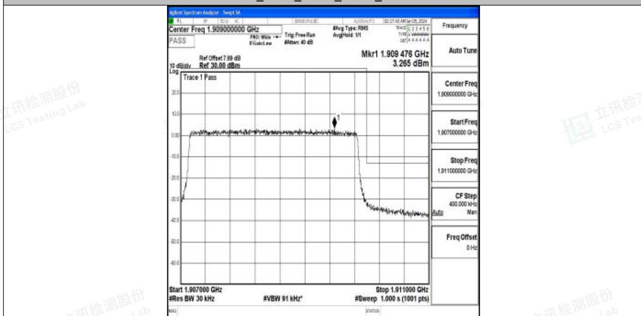
Band2_3MHz_16QAM_19185_15RB#0
