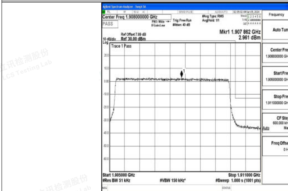
Band2_5MHz_16QAM_19175_25RB#0
