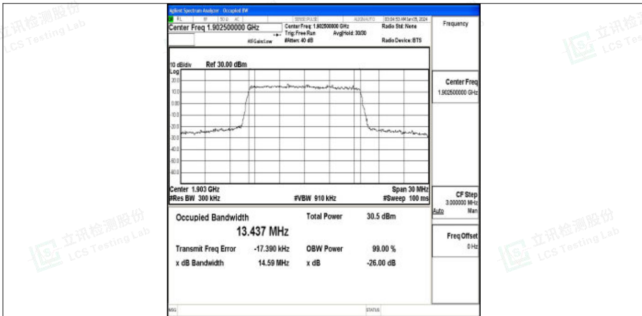
Band2-15MHz-QPSK-19125-75RB#0-PASS
