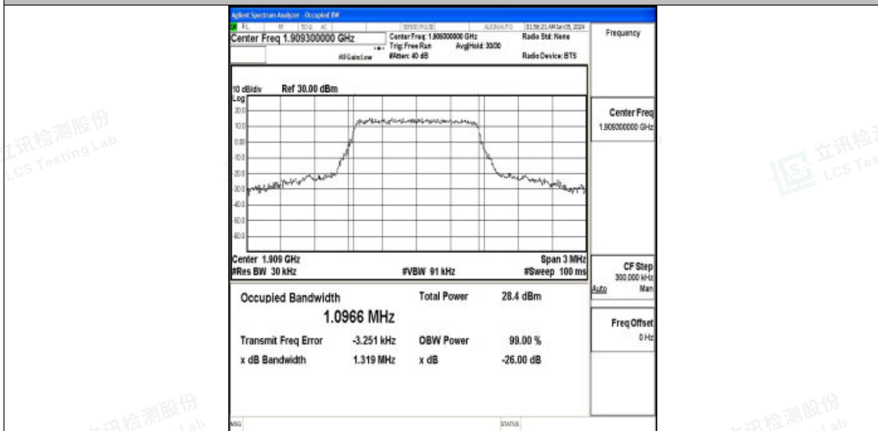
Band2-1.4MHz-16QAM-19193-6RB#0-PASS
