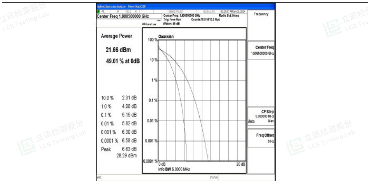
Band2-3MHz-QPSK-19185-15RB#0-PASS
