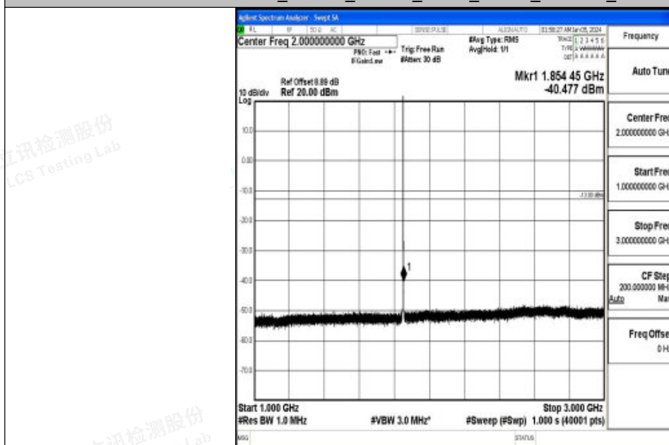
Band2_1.4MHz_16QAM_18607_1RB#0_1000~3000_1000~3000
