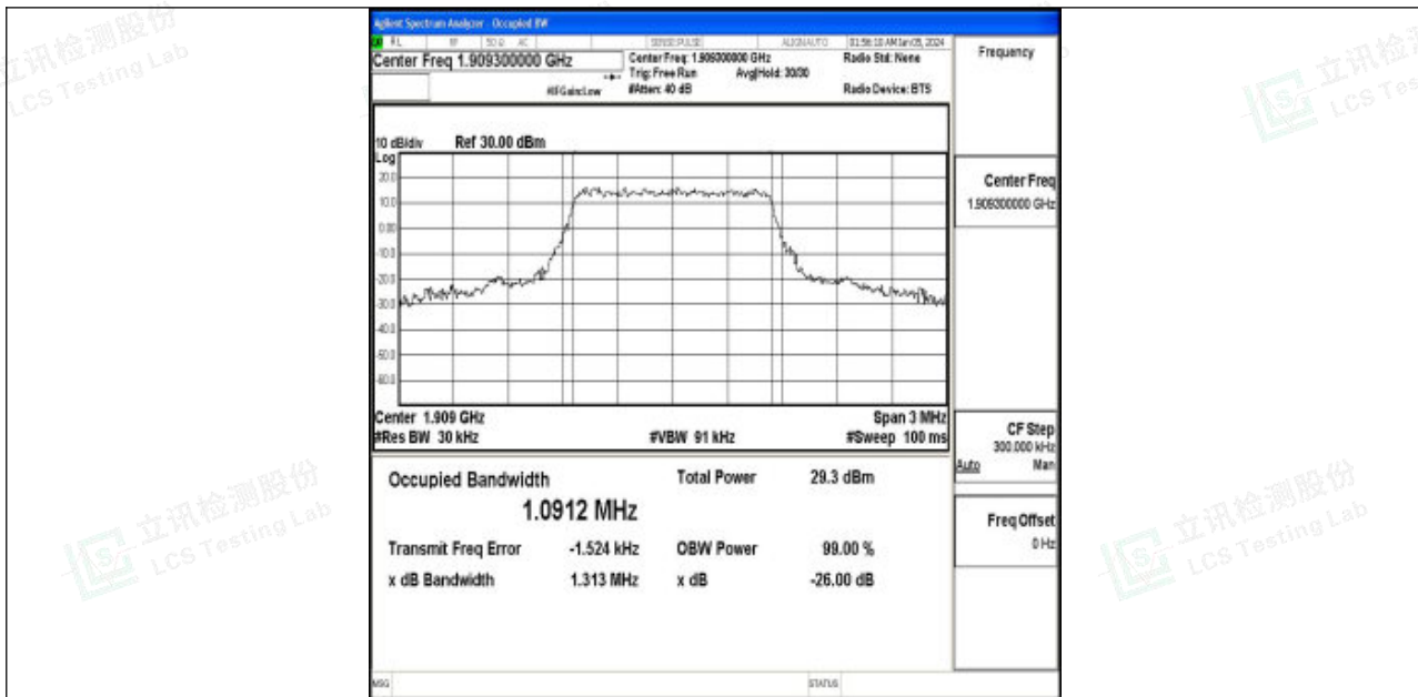
Band2-1.4MHz-QPSK-19193-6RB#0-PASS
