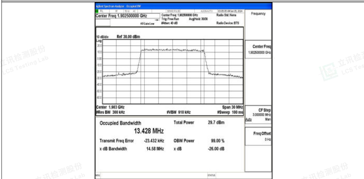
Band2-15MHz-16QAM-19125-75RB#0-PASS
