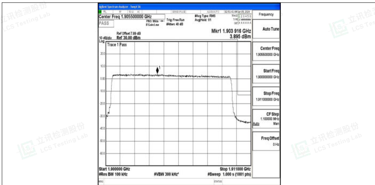
Band2_10MHz_QPSK_19150_50RB#0
