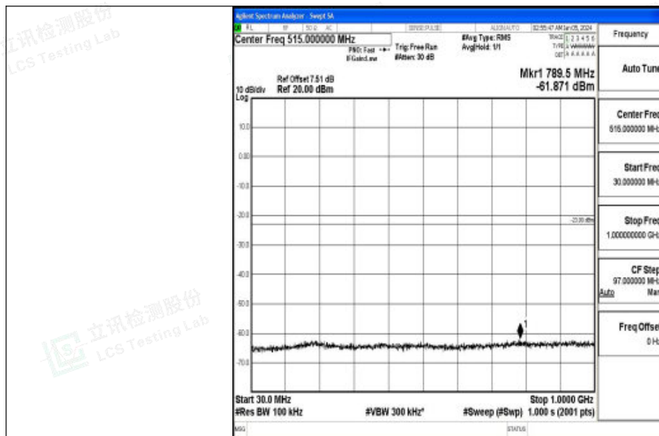
Band2_10MHz_16QAM_19150_1RB#0_30~1000_30~1000
