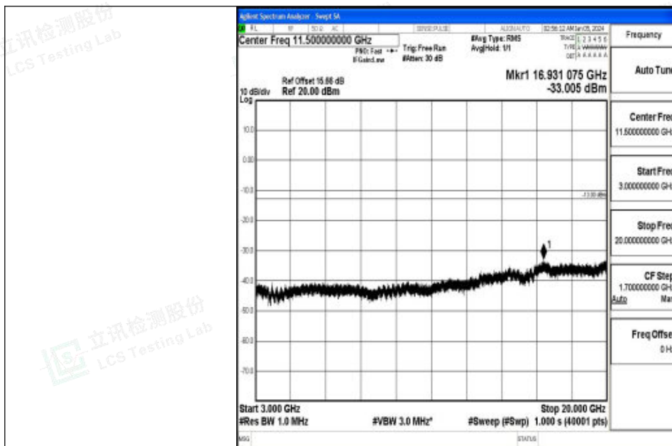
Band2_10MHz_16QAM_19150_1RB#0_3000~20000_3000~20000
