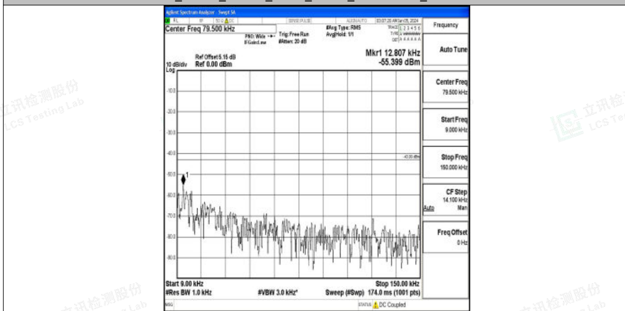
Band2_15MHz_QPSK_18900_1RB#0_0.009~0.15_0.009~0.15
