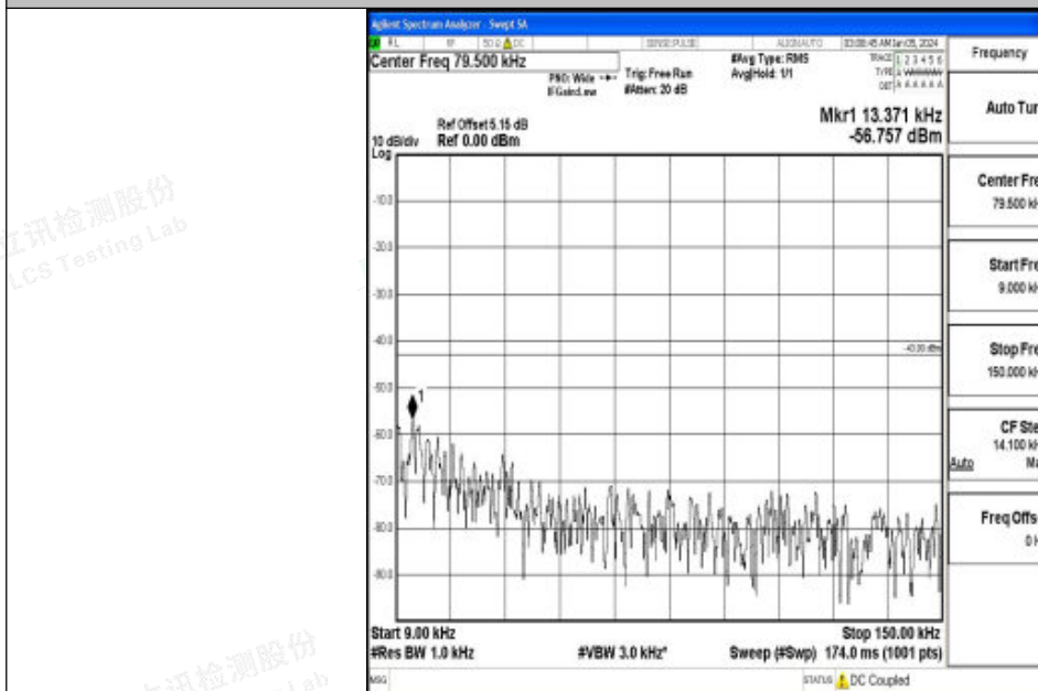
Band2_15MHz_QPSK_19125_1RB#0_0.009~0.15_0.009~0.15
