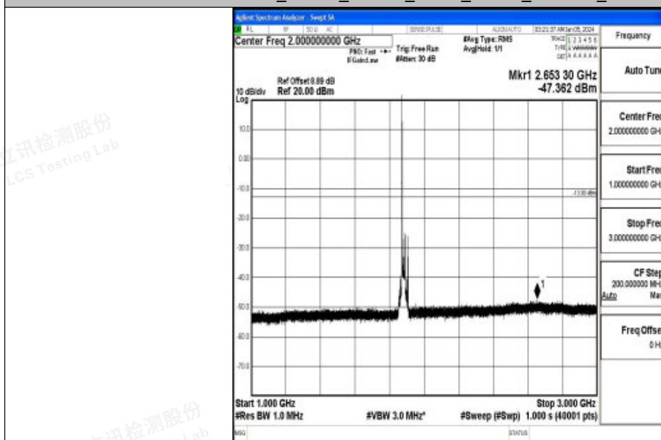
Band2_20MHz_16QAM_18900_1RB#0_1000~3000_1000~3000
