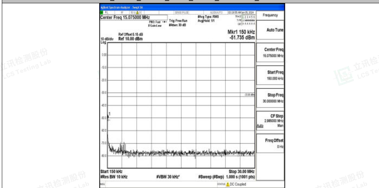
Band2_20MHz_16QAM_18700_1RB#0_0.15~30_0.15~30
