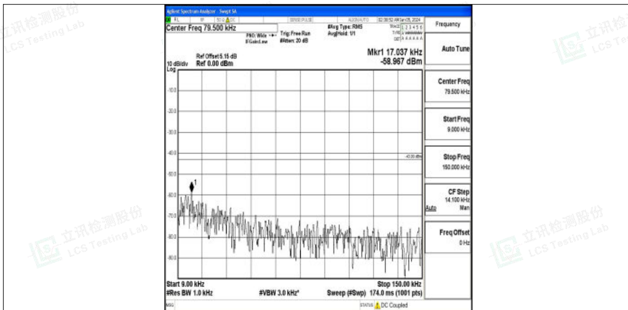
Band2_5MHz_16QAM_19175_1RB#0_0.009~0.15_0.009~0.15
