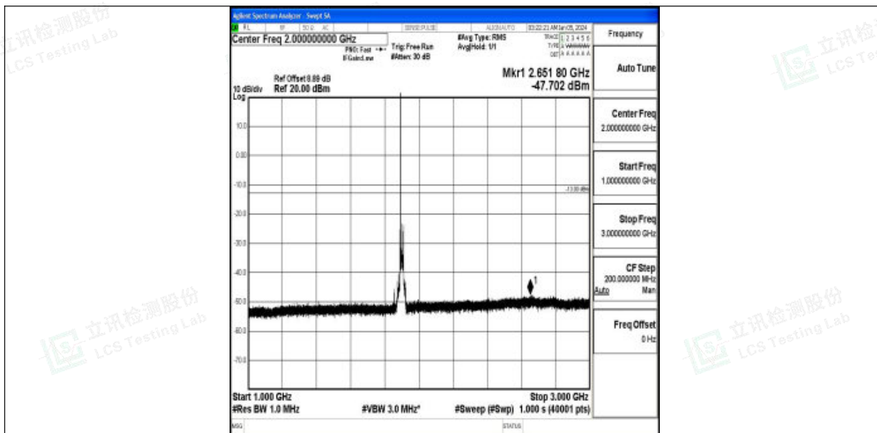
Band2_20MHz_QPSK_19100_1RB#0_1000~3000_1000~3000
