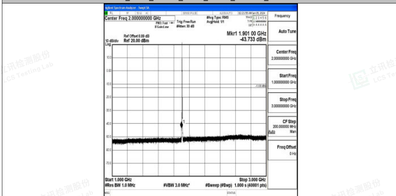
Band2_3MHz_16QAM_19185_1RB#0_1000~3000_1000~3000
