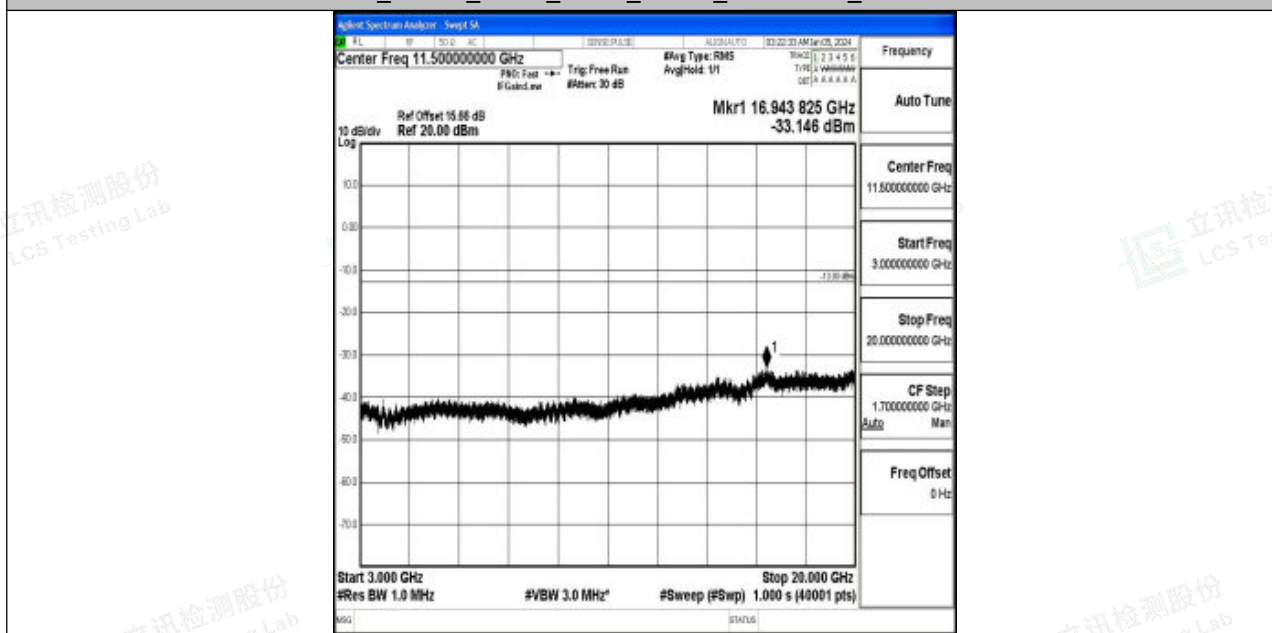
Band2_20MHz_QPSK_19100_1RB#0_3000~20000_3000~20000
