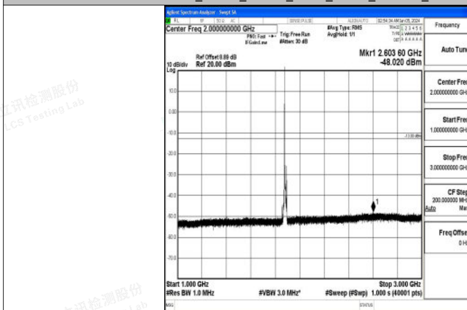
Band2_10MHz_16QAM_18900_1RB#0_1000~3000_1000~3000
