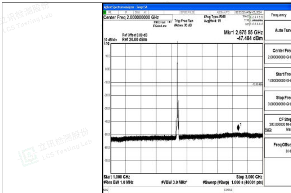
Band2_10MHz_QPSK_18900_1RB#0_1000~3000_1000~3000
