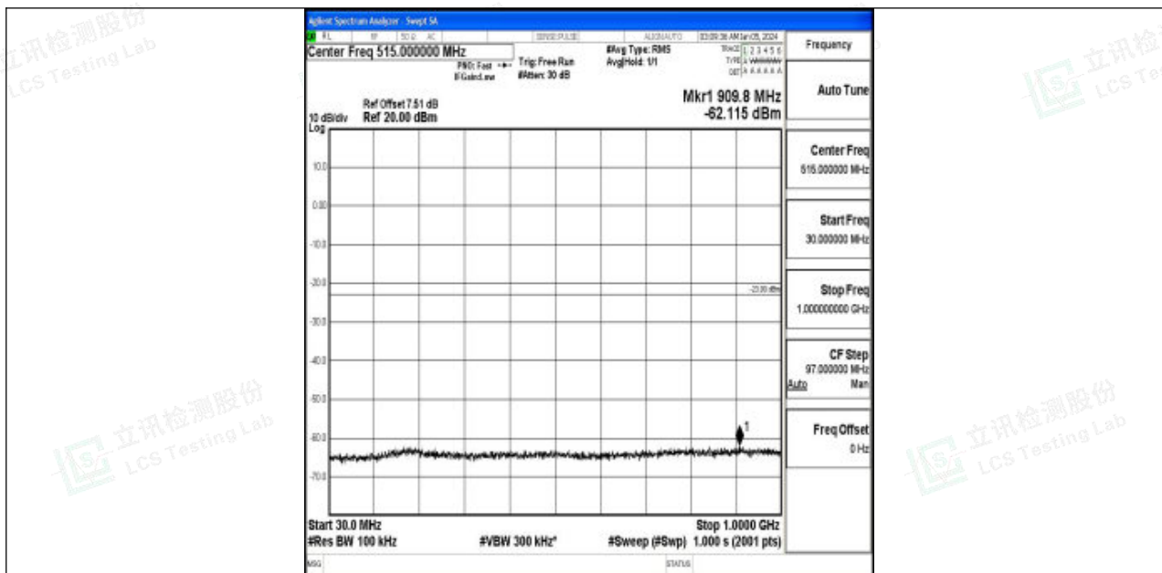
Band2_15MHz_16QAM_19125_1RB#0_30~1000_30~1000
