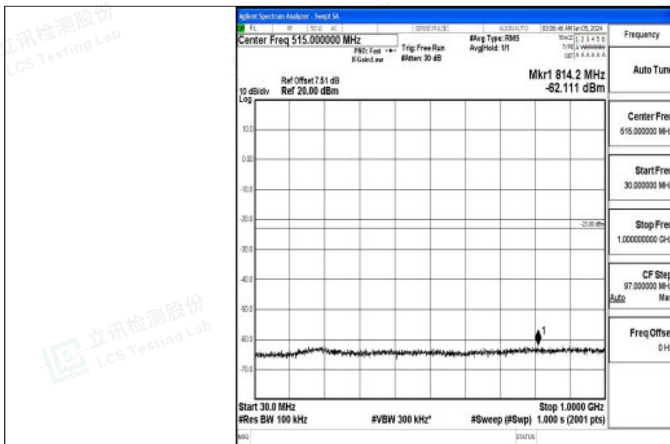
Band2_15MHz_16QAM_18675_1RB#0_30~1000_30~1000
