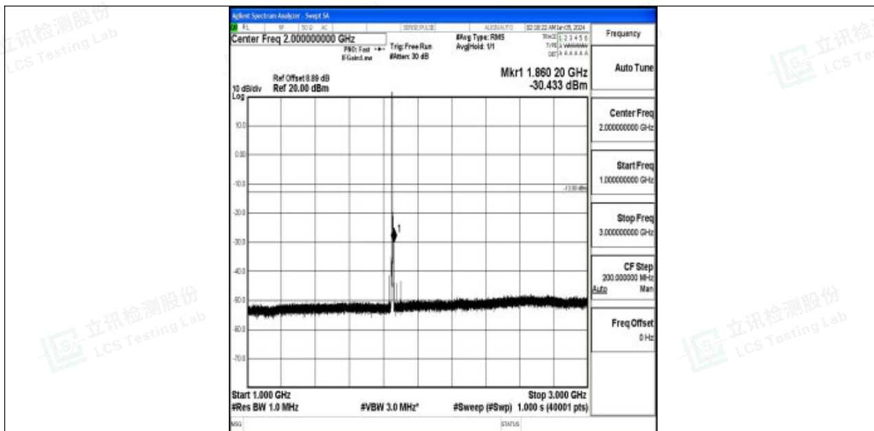
Band2_3MHz_QPSK_18615_1RB#0_1000~3000_1000~3000
