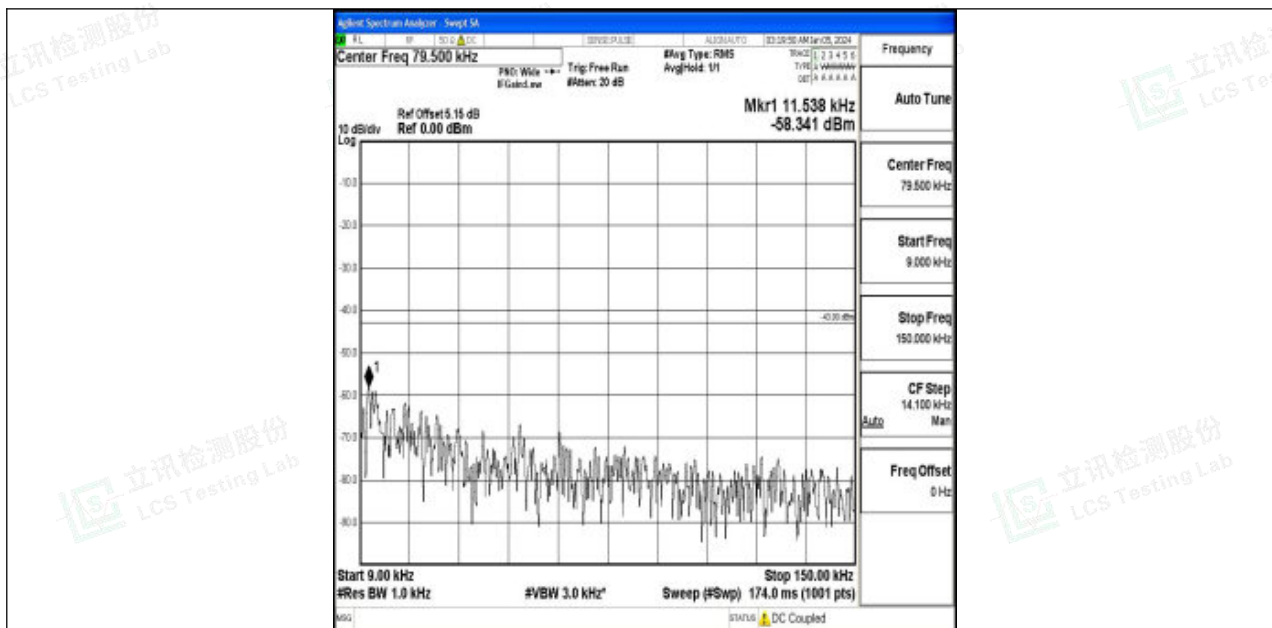
Band2_20MHz_16QAM_18700_1RB#0_0.009~0.15_0.009~0.15
