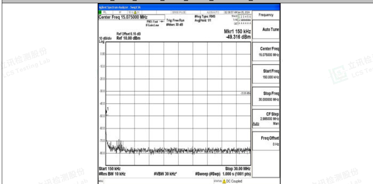
Band2_5MHz_16QAM_19175_1RB#0_0.15~30_0.15~30
