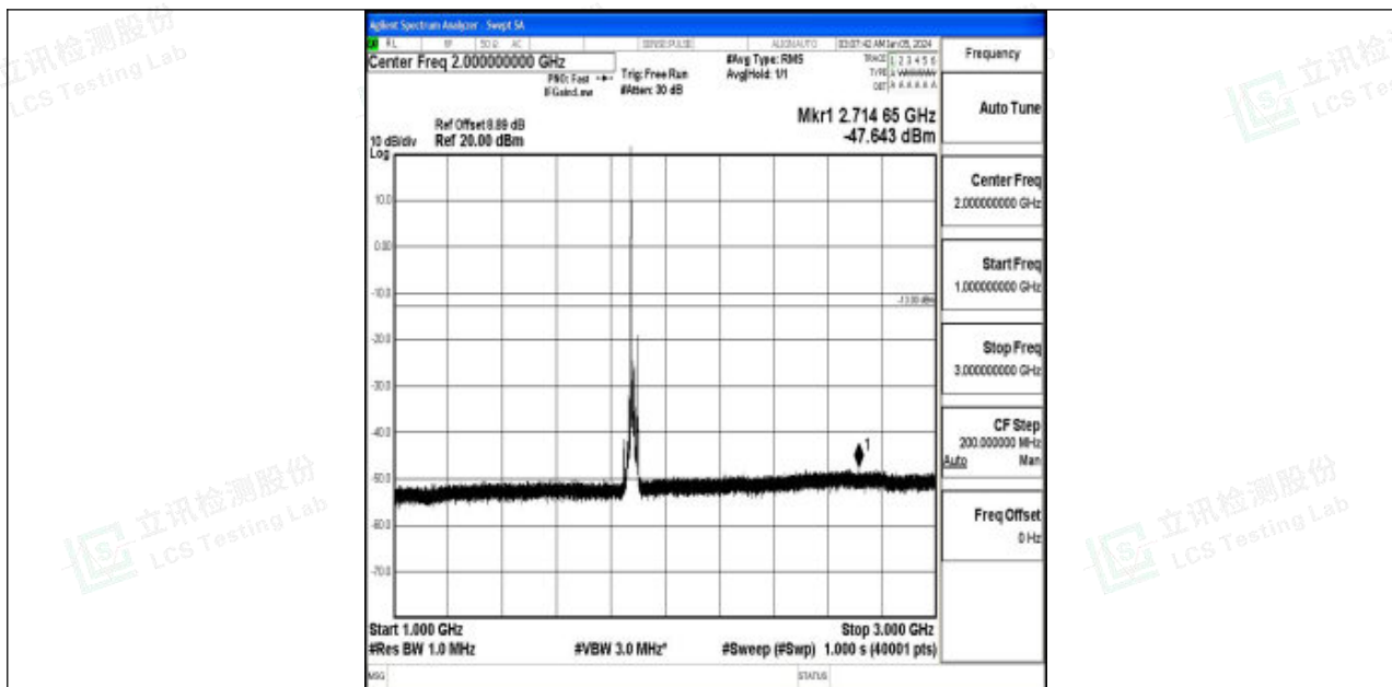
Band2_15MHz_QPSK_18900_1RB#0_1000~3000_1000~3000
