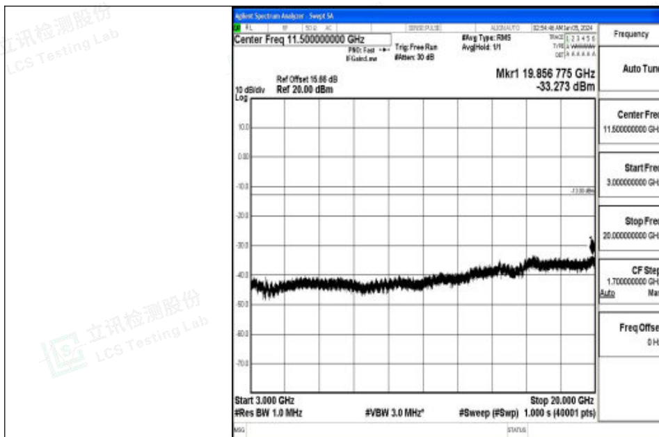
Band2_10MHz_16QAM_18900_1RB#0_3000~20000_3000~20000
