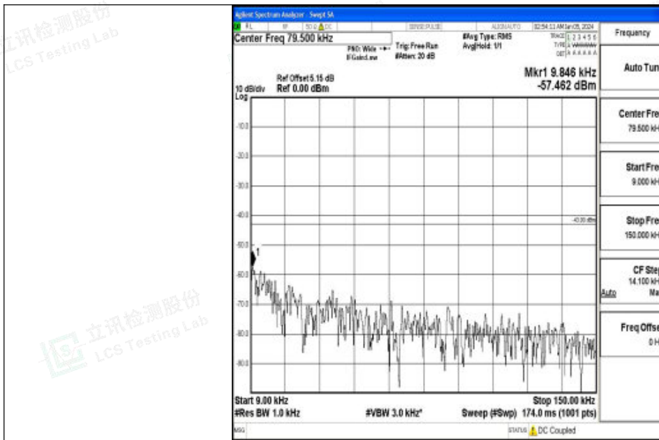
Band2_10MHz_16QAM_18900_1RB#0_0.009~0.15_0.009~0.15
