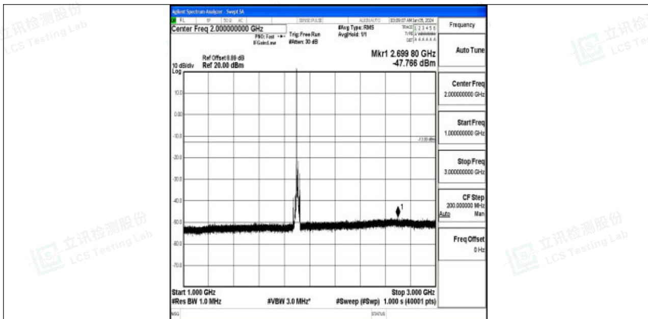
Band2_15MHz_QPSK_19125_1RB#0_1000~3000_1000~3000
