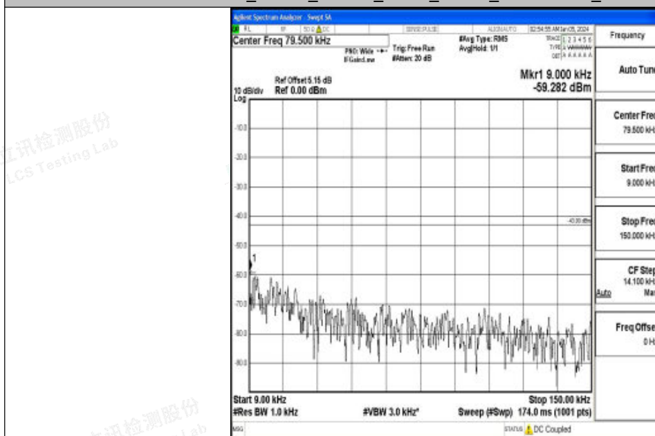
Band2_10MHz_QPSK_19150_1RB#0_0.009~0.15_0.009~0.15
