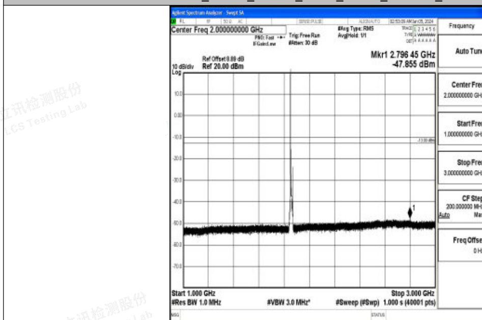
Band2_10MHz_16QAM_18650_1RB#0_1000~3000_1000~3000
