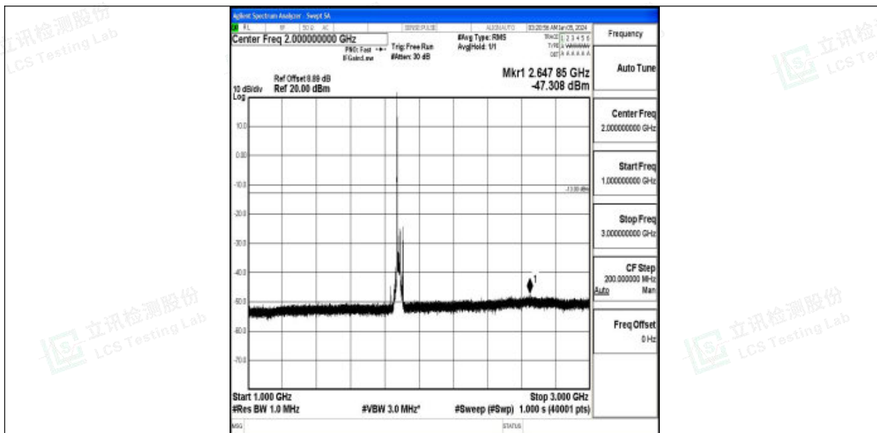
Band2_20MHz_QPSK_18900_1RB#0_1000~3000_1000~3000
