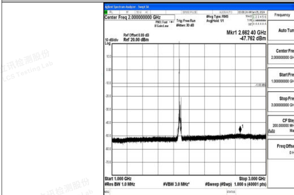
Band2_15MHz_16QAM_18900_1RB#0_1000~3000_1000~3000
