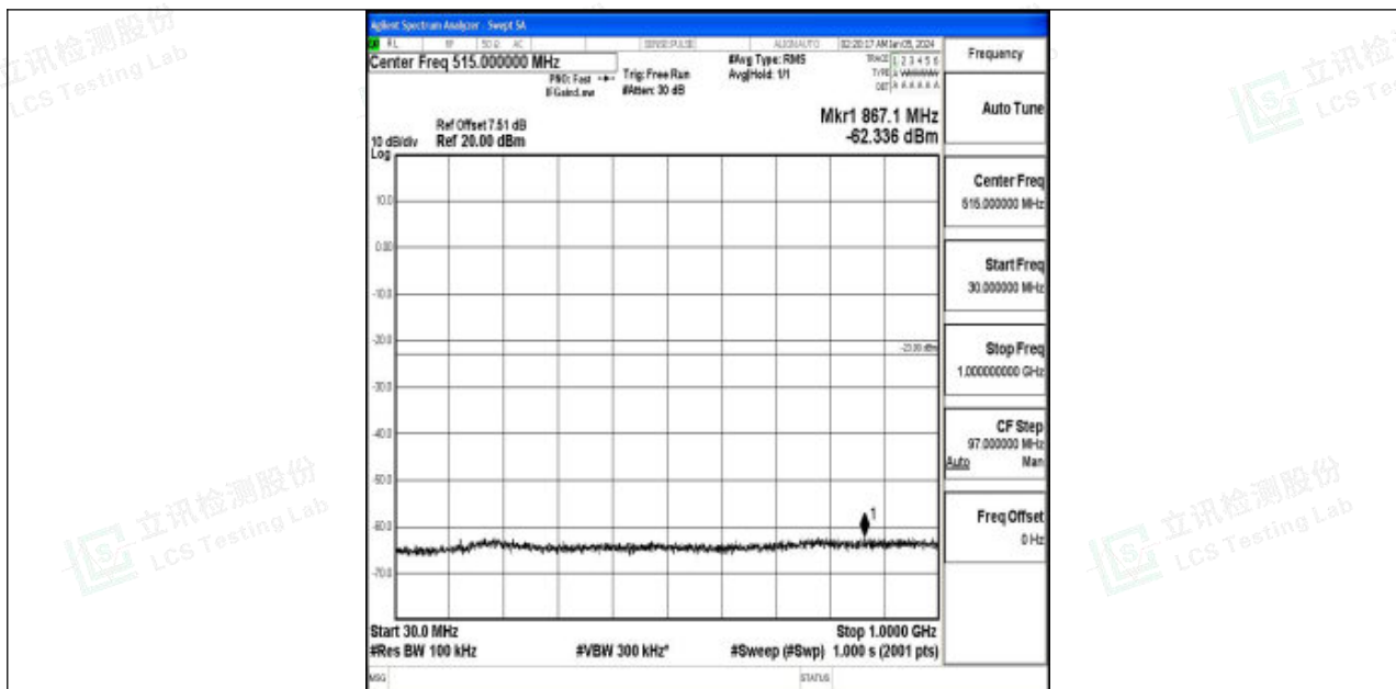
Band2_3MHz_16QAM_18900_1RB#0_30~1000_30~1000
