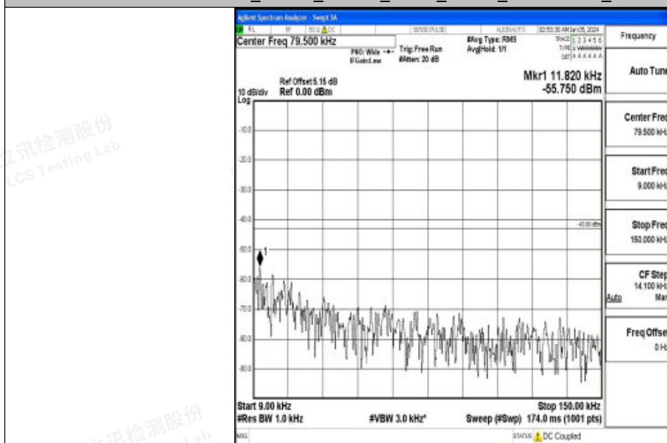
Band2_10MHz_QPSK_18900_1RB#0_0.009~0.15_0.009~0.15
