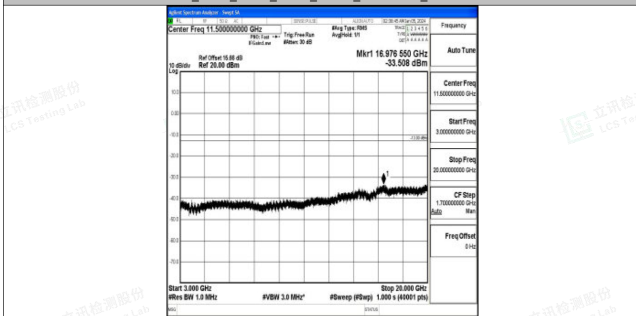
Band2_5MHz_QPSK_19175_1RB#0_3000~20000_3000~20000
