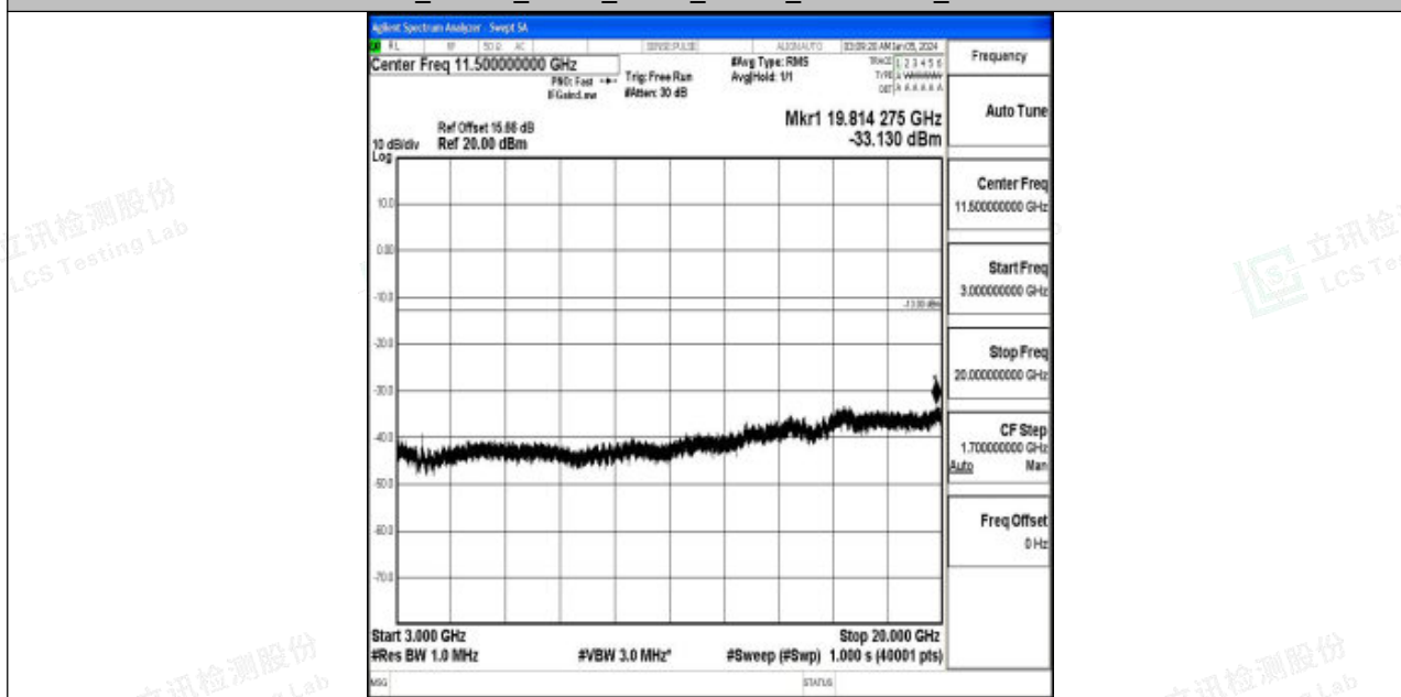
Band2_15MHz_QPSK_19125_1RB#0_3000~20000_3000~20000
