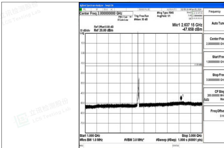
Band2_10MHz_QPSK_19150_1RB#0_1000~3000_1000~3000
