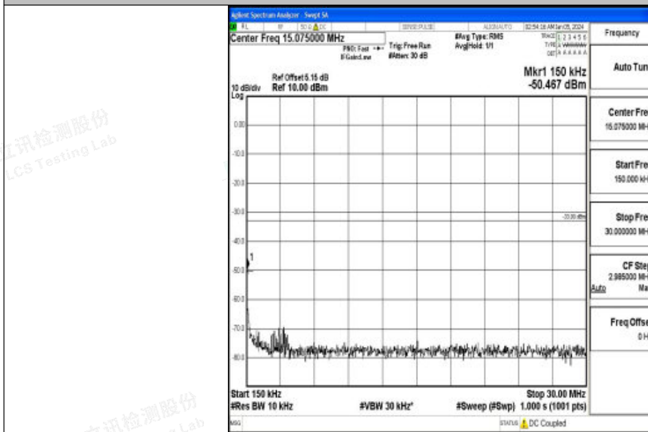
Band2_10MHz_16QAM_18900_1RB#0_0.15~30_0.15~30
