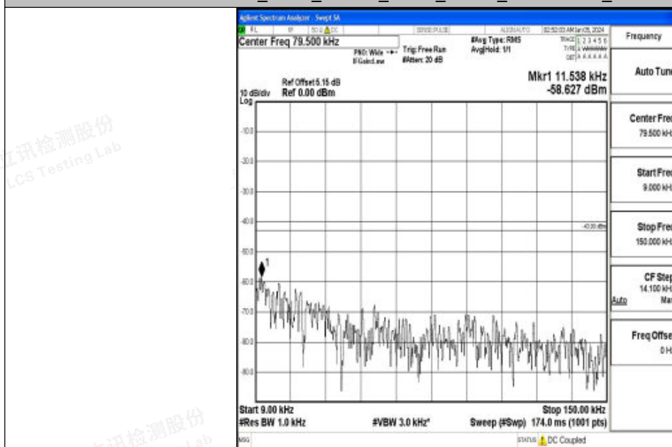
Band2_10MHz_QPSK_18650_1RB#0_0.009~0.15_0.009~0.15
