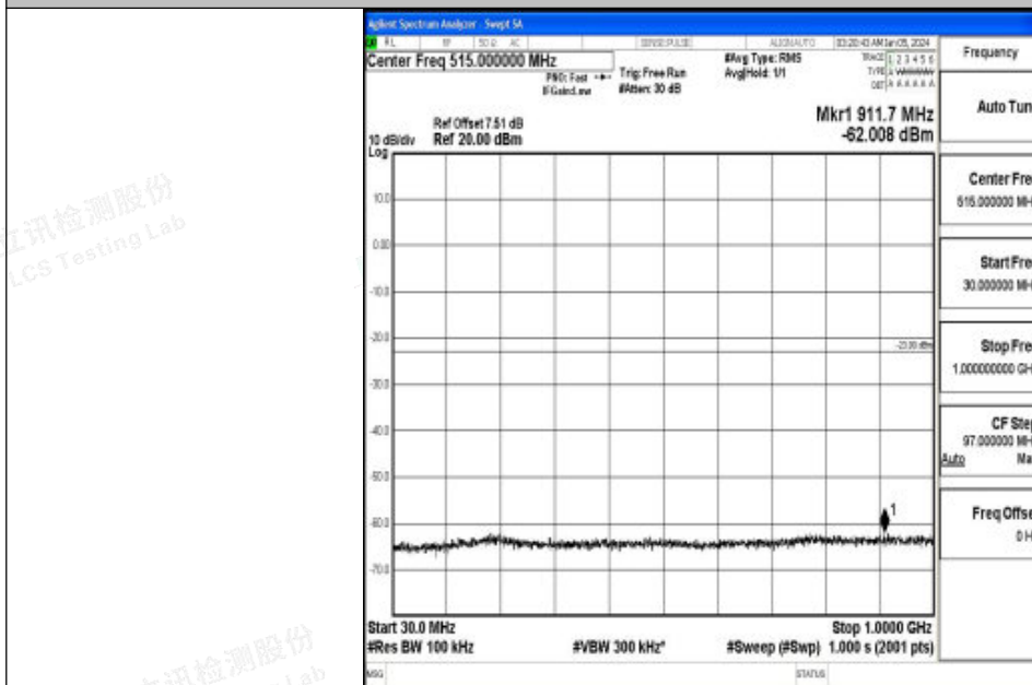
Band2_20MHz_QPSK_18900_1RB#0_30~1000_30~1000
