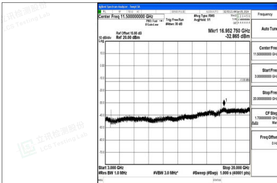
Band2_10MHz_16QAM_18650_1RB#0_3000~20000_3000~20000
