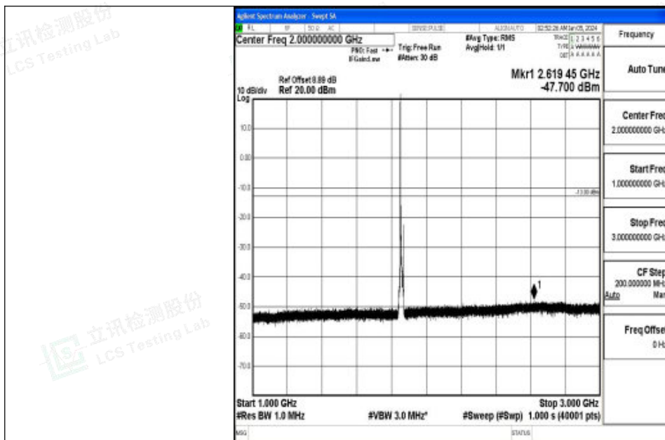
Band2_10MHz_QPSK_18650_1RB#0_1000~3000_1000~3000
