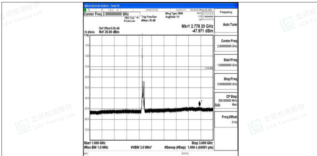
Band2_20MHz_QPSK_18700_1RB#0_1000~3000_1000~3000
