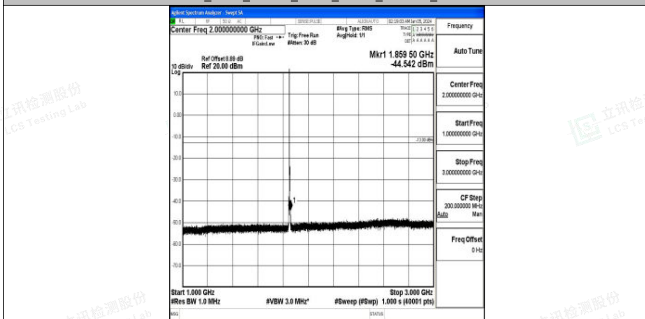
Band2_3MHz_16QAM_18615_1RB#0_1000~3000_1000~3000
