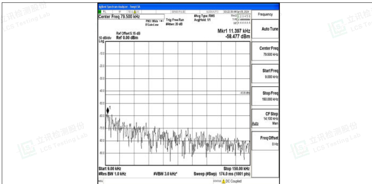
Band2_20MHz_16QAM_19100_1RB#0_0.009~0.15_0.009~0.15
