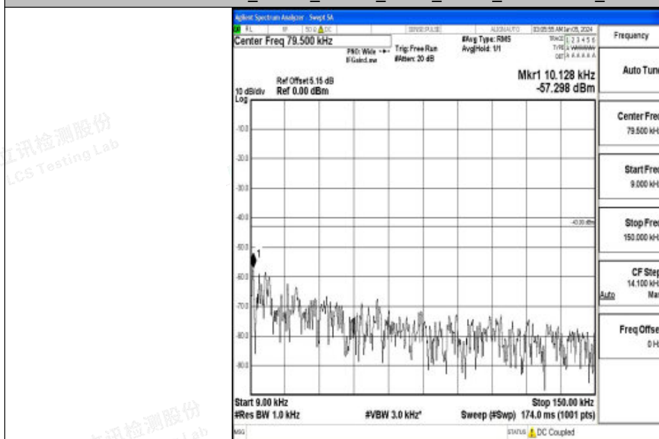
Band2_15MHz_QPSK_18675_1RB#0_0.009~0.15_0.009~0.15
