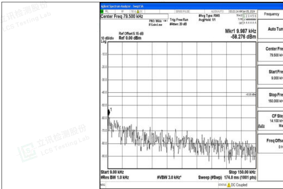
Band2_20MHz_16QAM_18900_1RB#0_0.009~0.15_0.009~0.15
