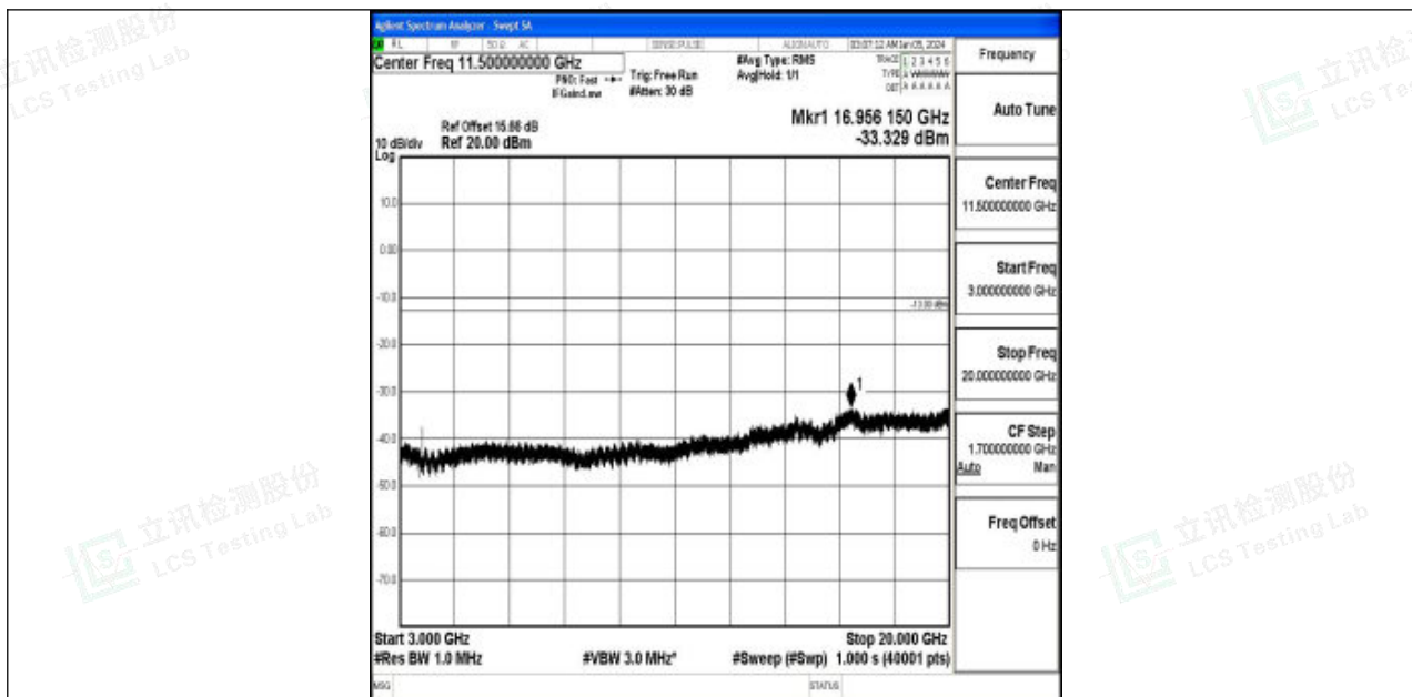
Band2_15MHz_16QAM_18675_1RB#0_3000~20000_3000~20000
