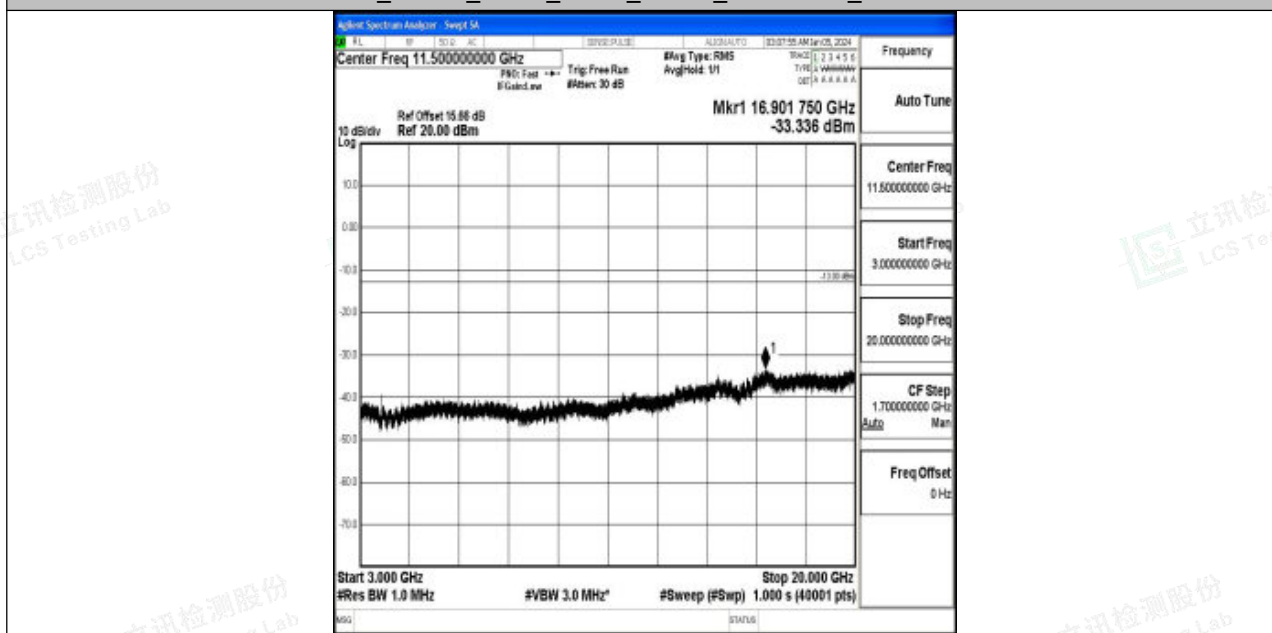
Band2_15MHz_QPSK_18900_1RB#0_3000~20000_3000~20000
