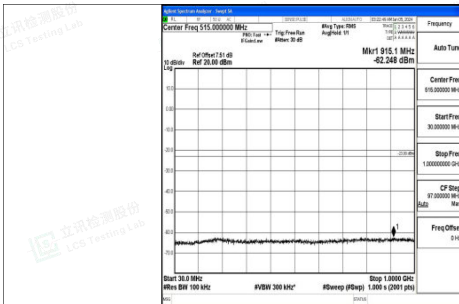
Band2_20MHz_16QAM_19100_1RB#0_30~1000_30~1000
