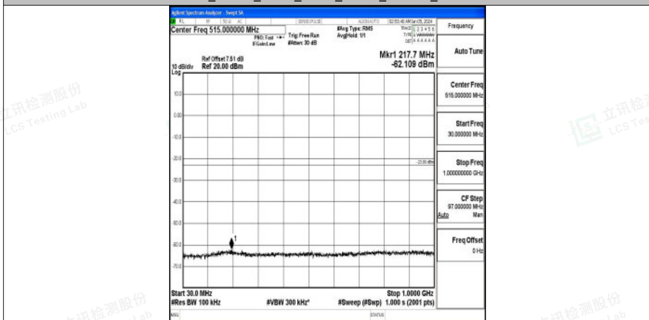
Band2_10MHz_QPSK_18900_1RB#0_30~1000_30~1000
