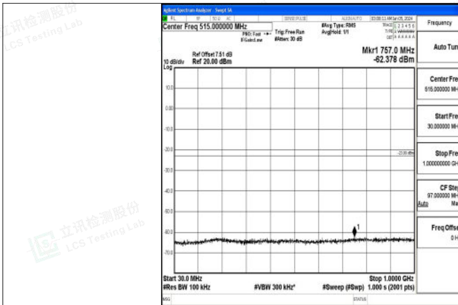
Band2_15MHz_16QAM_18900_1RB#0_30~1000_30~1000
