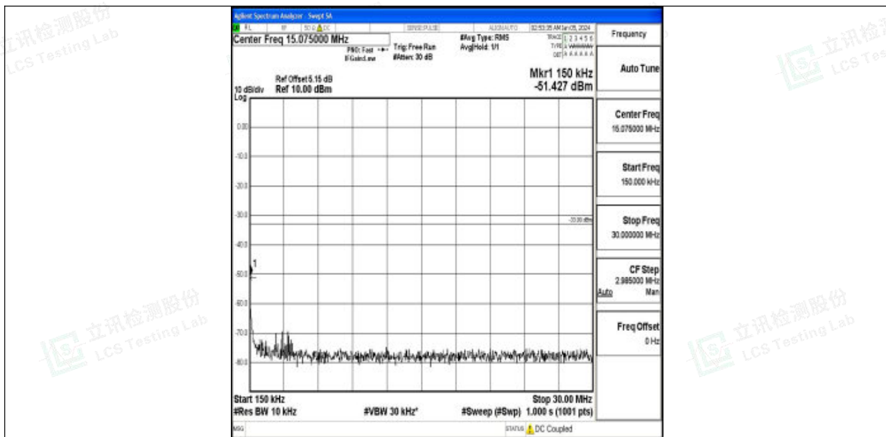
Band2_10MHz_QPSK_18900_1RB#0_0.15~30_0.15~30
