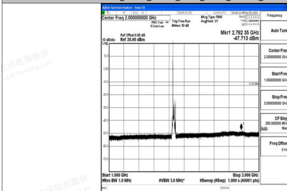
Band2_20MHz_16QAM_18700_1RB#0_1000~3000_1000~3000
