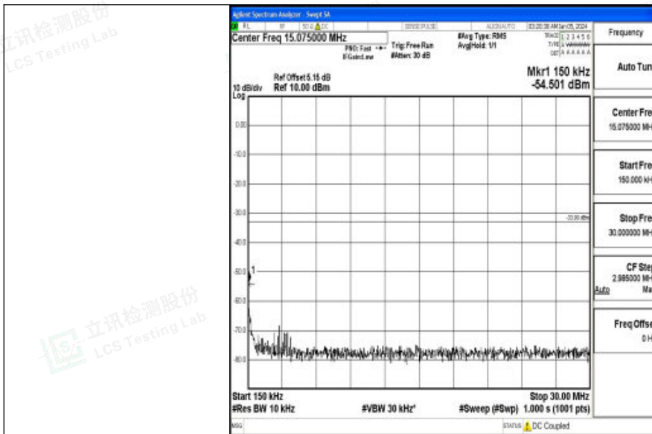
Band2_20MHz_QPSK_18900_1RB#0_0.15~30_0.15~30
