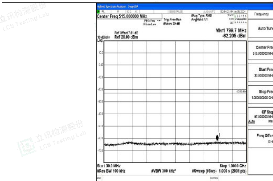
Band2_10MHz_16QAM_18900_1RB#0_30~1000_30~1000
