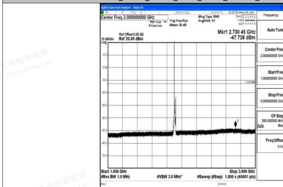
Band2_10MHz_16QAM_19150_1RB#0_1000~3000_1000~3000
