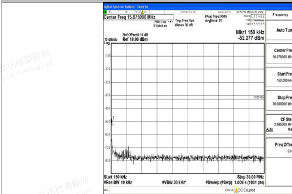
Band2_10MHz_16QAM_18650_1RB#0_0.15~30_0.15~30
