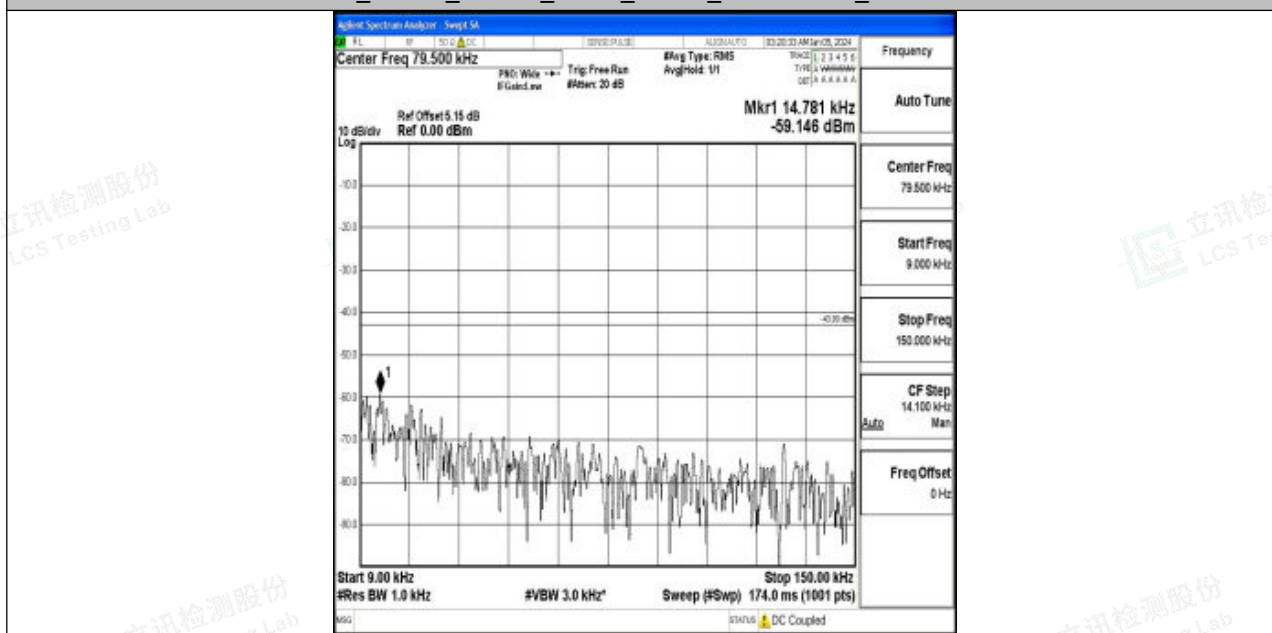
Band2_20MHz_QPSK_18900_1RB#0_0.009~0.15_0.009~0.15
