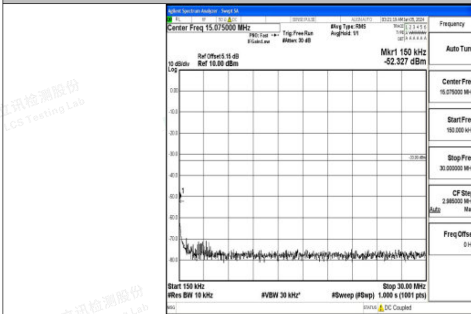
Band2_20MHz_16QAM_18900_1RB#0_0.15~30_0.15~30
