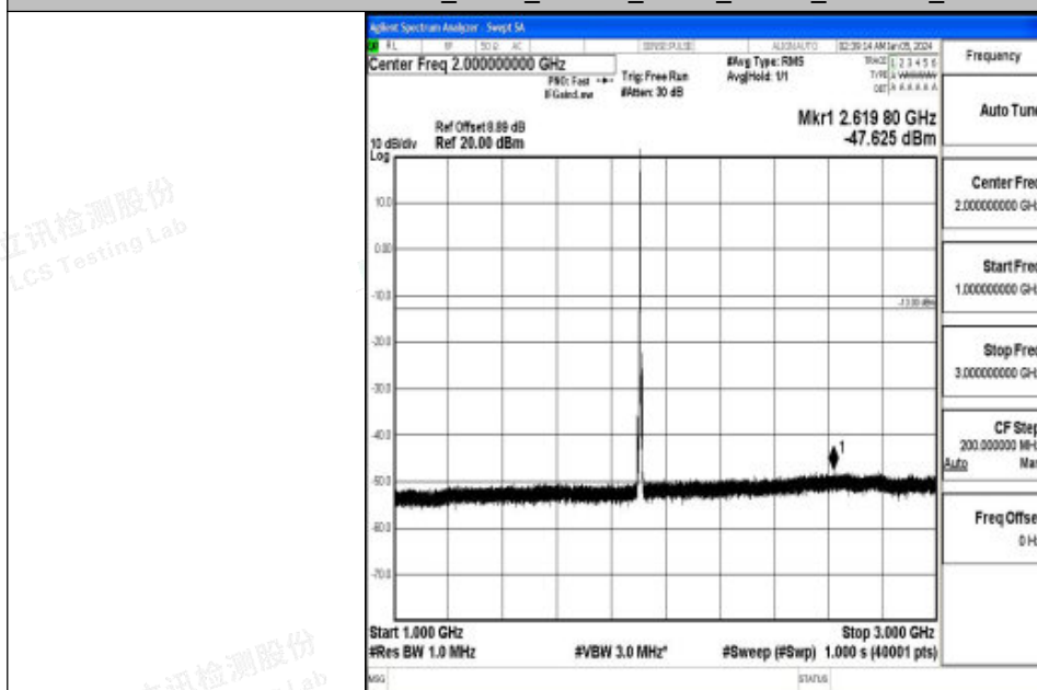
Band2_5MHz_16QAM_19175_1RB#0_1000~3000_1000~3000
