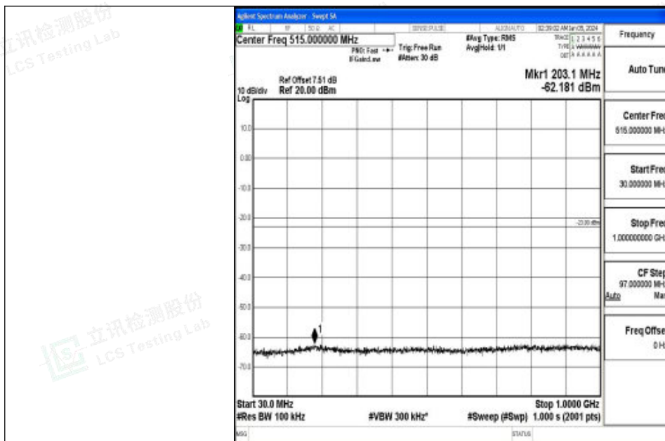
Band2_5MHz_16QAM_19175_1RB#0_30~1000_30~1000
