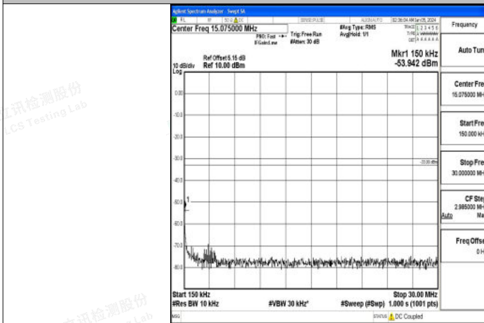
Band2_5MHz_16QAM_18625_1RB#0_0.15~30_0.15~30
