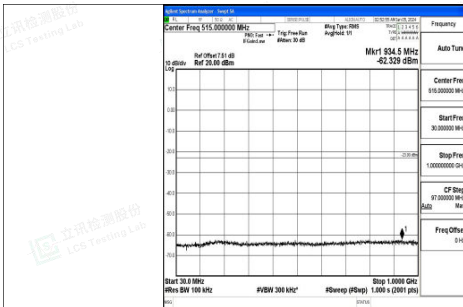
Band2_10MHz_16QAM_18650_1RB#0_30~1000_30~1000
