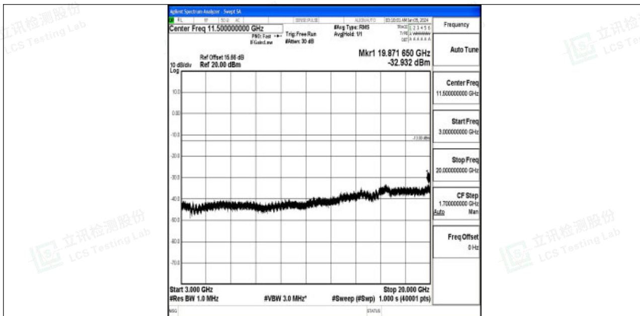
Band2_15MHz_16QAM_19125_1RB#0_3000~20000_3000~20000
