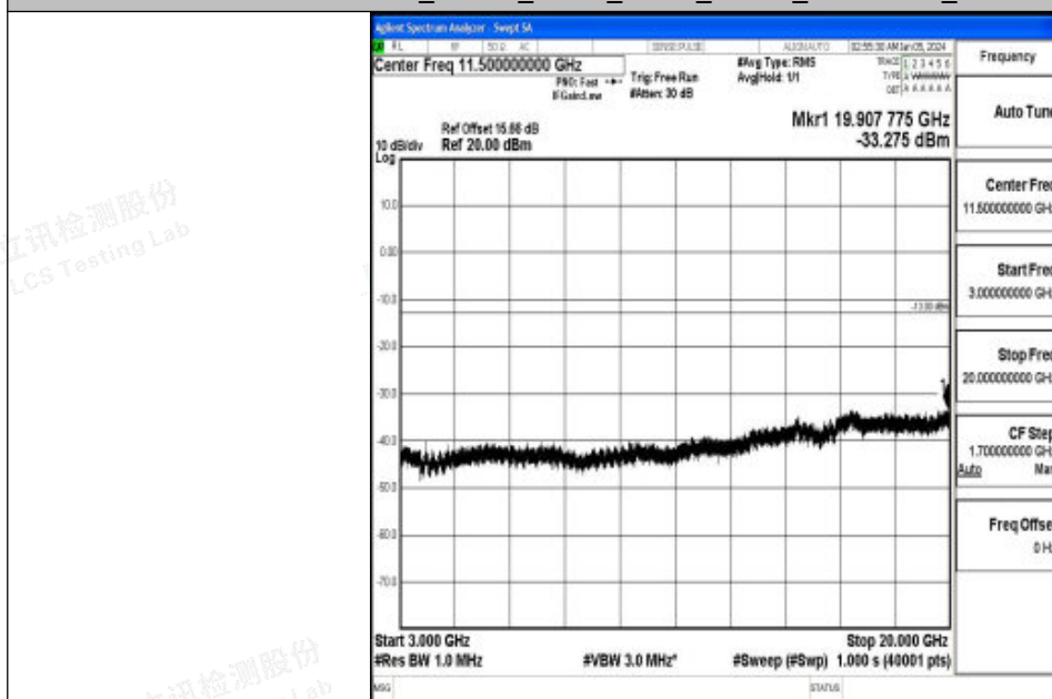
Band2_10MHz_QPSK_19150_1RB#0_3000~20000_3000~20000
