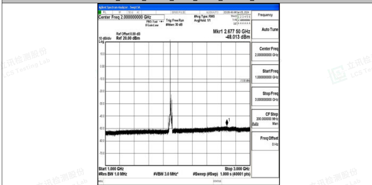
Band2_15MHz_16QAM_19125_1RB#0_1000~3000_1000~3000
