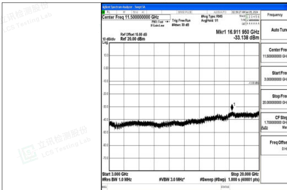
Band2_5MHz_16QAM_19175_1RB#0_3000~20000_3000~20000
