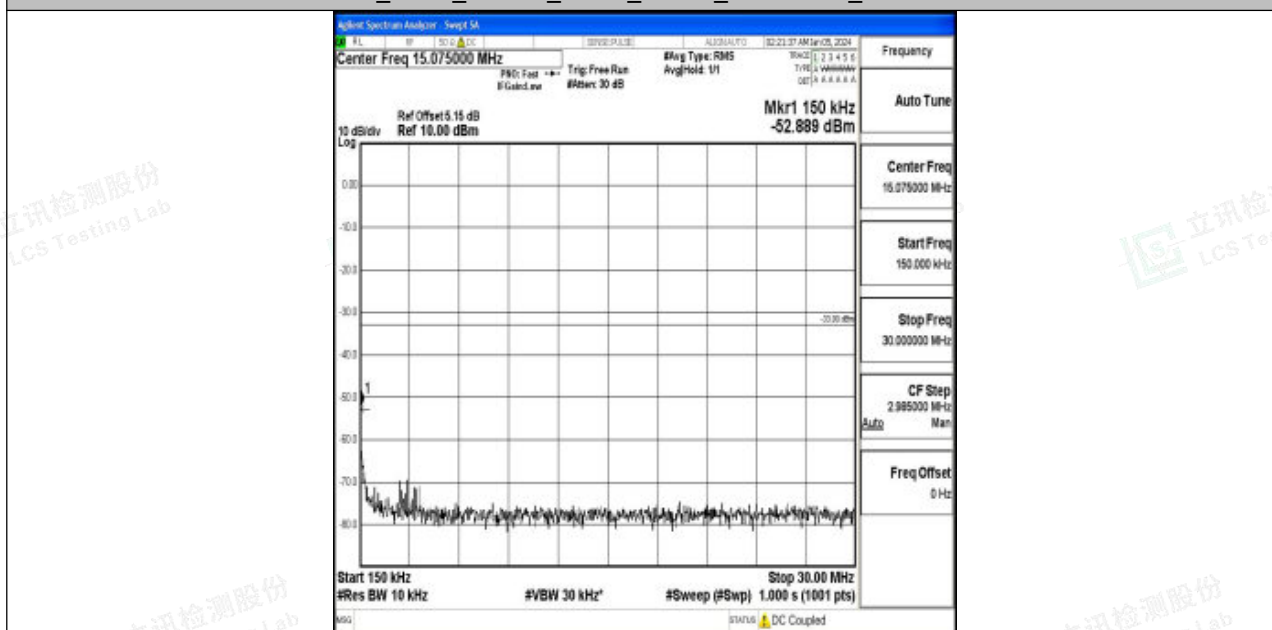
Band2_3MHz_16QAM_19185_1RB#0_0.15~30_0.15~30
