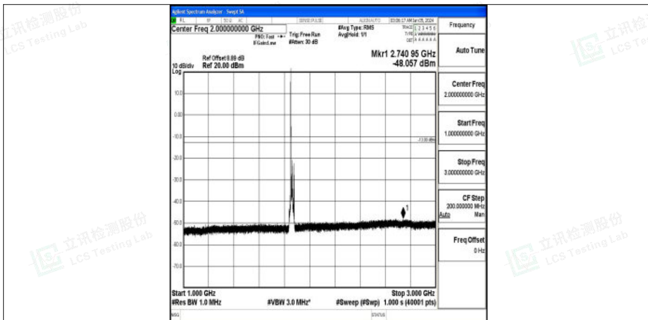
Band2_15MHz_QPSK_18675_1RB#0_1000~3000_1000~3000
