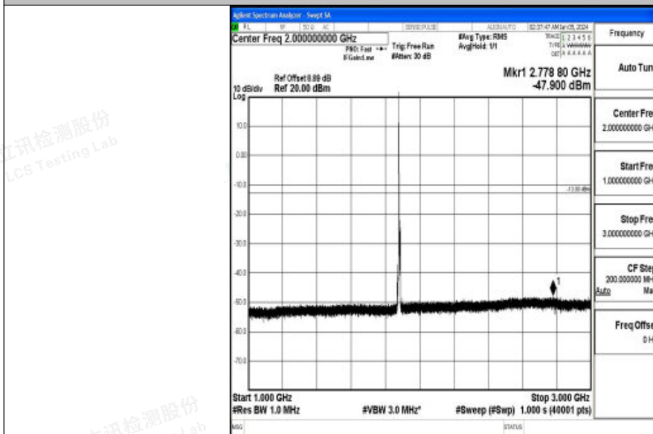
Band2_5MHz_16QAM_18900_1RB#0_1000~3000_1000~3000
