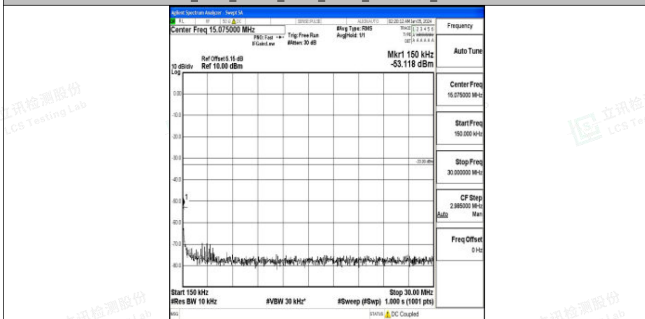
Band2_3MHz_16QAM_18900_1RB#0_0.15~30_0.15~30
