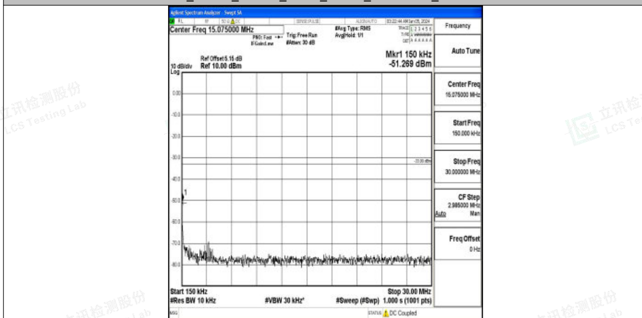
Band2_20MHz_16QAM_19100_1RB#0_0.15~30_0.15~30
