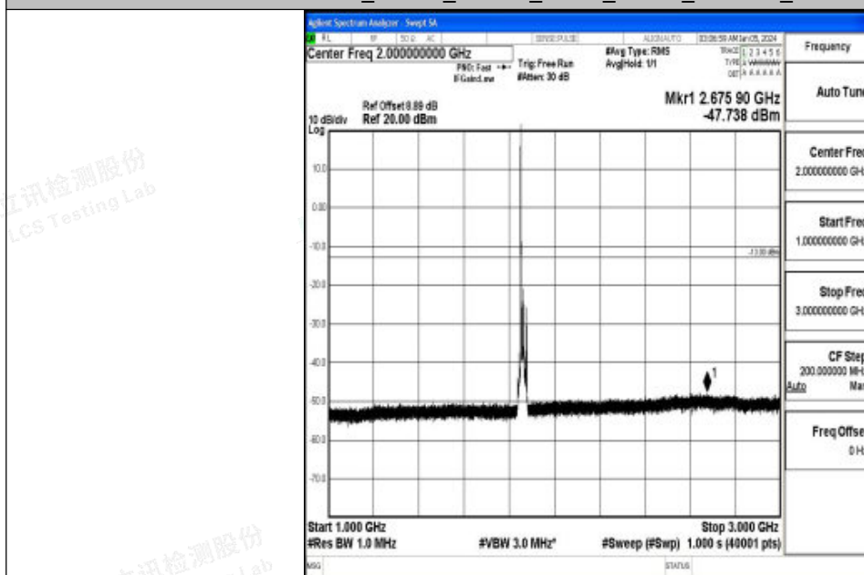
Band2_15MHz_16QAM_18675_1RB#0_1000~3000_1000~3000
