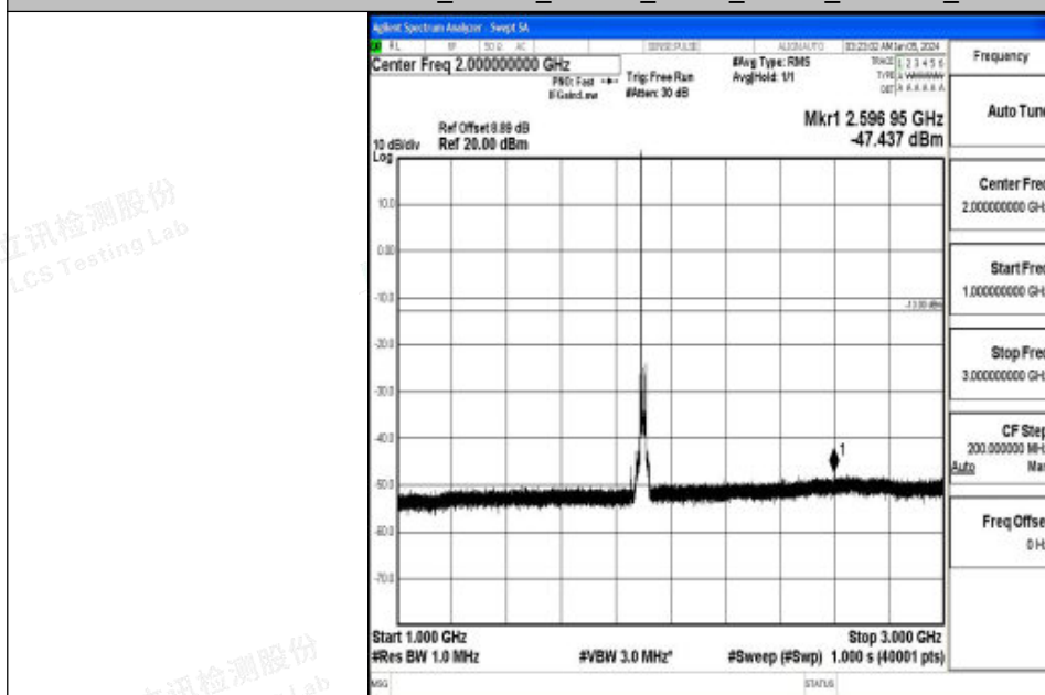
Band2_20MHz_16QAM_19100_1RB#0_1000~3000_1000~3000
