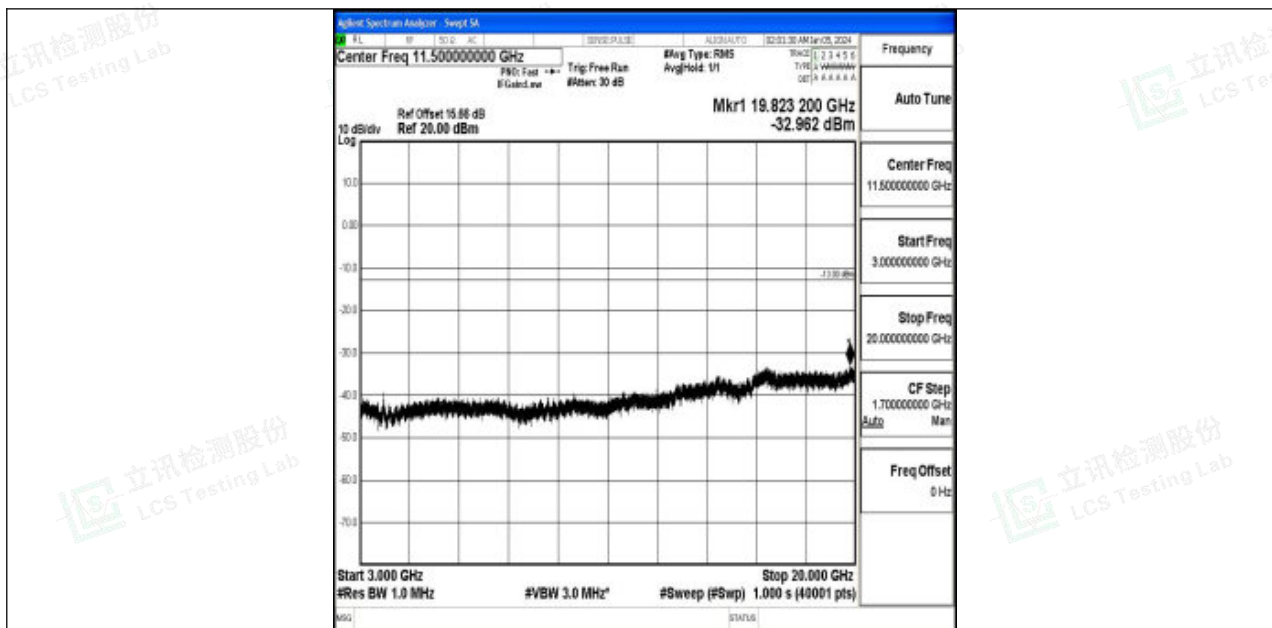
Band2_1.4MHz_16QAM_19193_1RB#0_3000~20000_3000~20000
