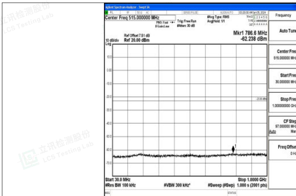
Band2_20MHz_16QAM_18700_1RB#0_30~1000_30~1000
