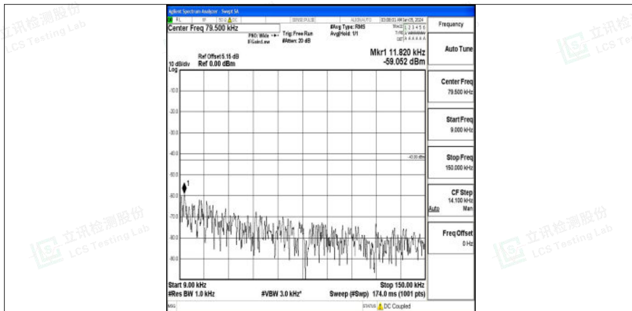
Band2_15MHz_16QAM_18900_1RB#0_0.009~0.15_0.009~0.15
