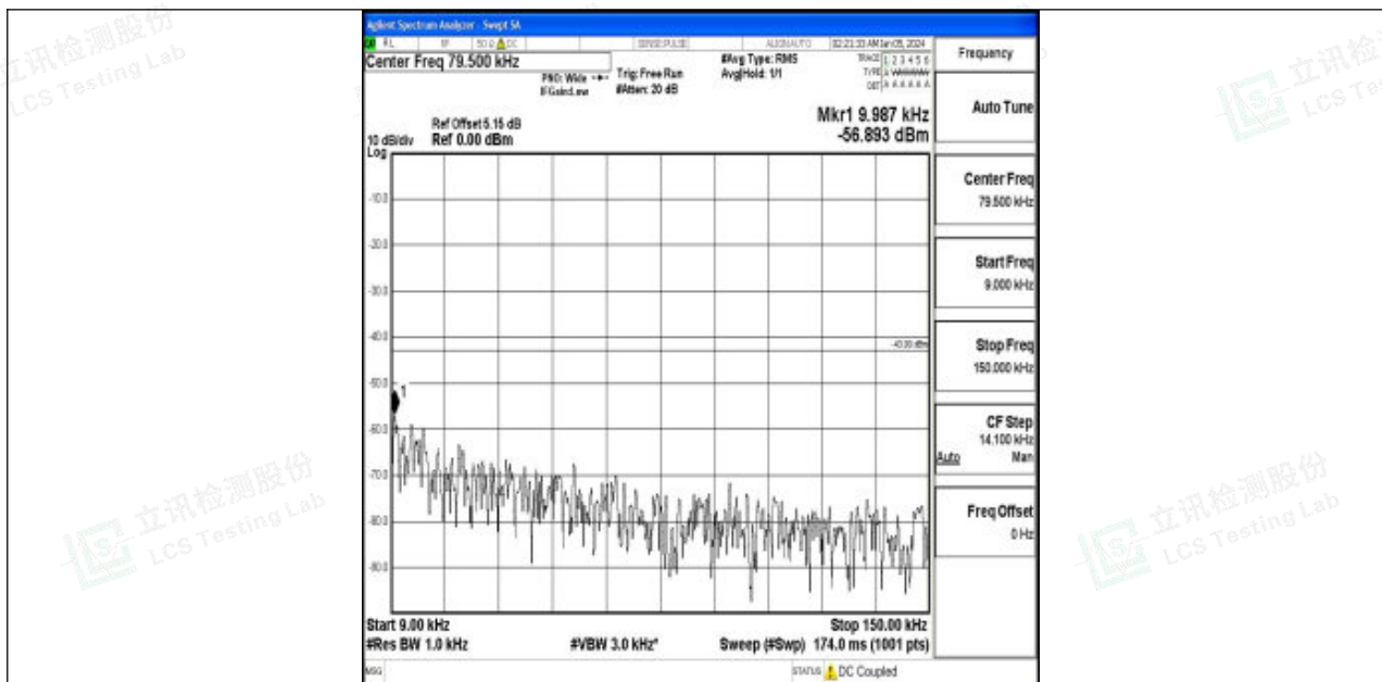
Band2_3MHz_16QAM_19185_1RB#0_0.009~0.15_0.009~0.15
