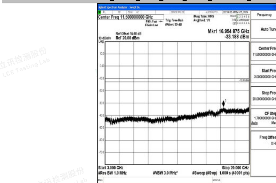
Band2_10MHz_QPSK_18900_1RB#0_3000~20000_3000~20000
