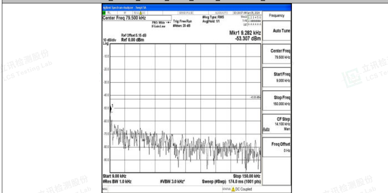
Band2_20MHz_QPSK_18700_1RB#0_0.009~0.15_0.009~0.15
