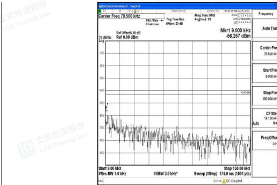
Band2_10MHz_16QAM_18650_1RB#0_0.009~0.15_0.009~0.15
