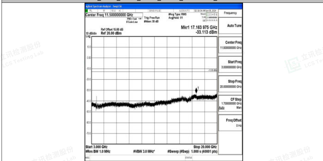
Band2_3MHz_QPSK_18615_1RB#0_3000~20000_3000~20000
