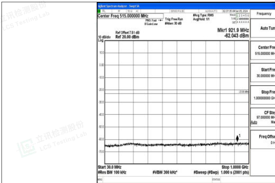
Band2_5MHz_16QAM_18900_1RB#0_30~1000_30~1000
