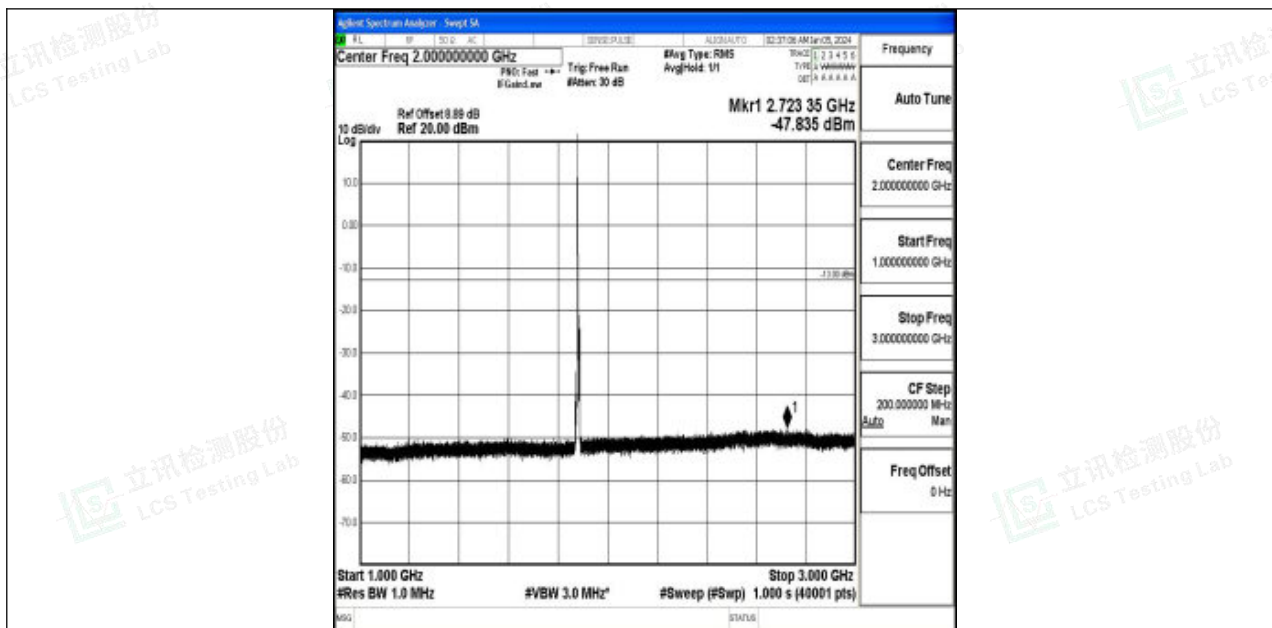
Band2_5MHz_QPSK_18900_1RB#0_1000~3000_1000~3000
