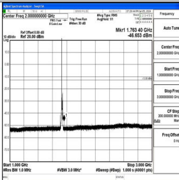
Band4_10MHz_16QAM_20175_1RB#0_1000~3000_1000~3000
