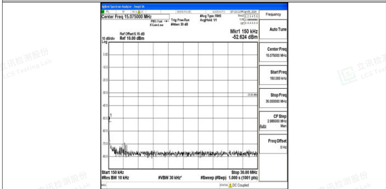
Band4_5MHz_16QAM_20375_1RB#0_0.15~30_0.15~30
