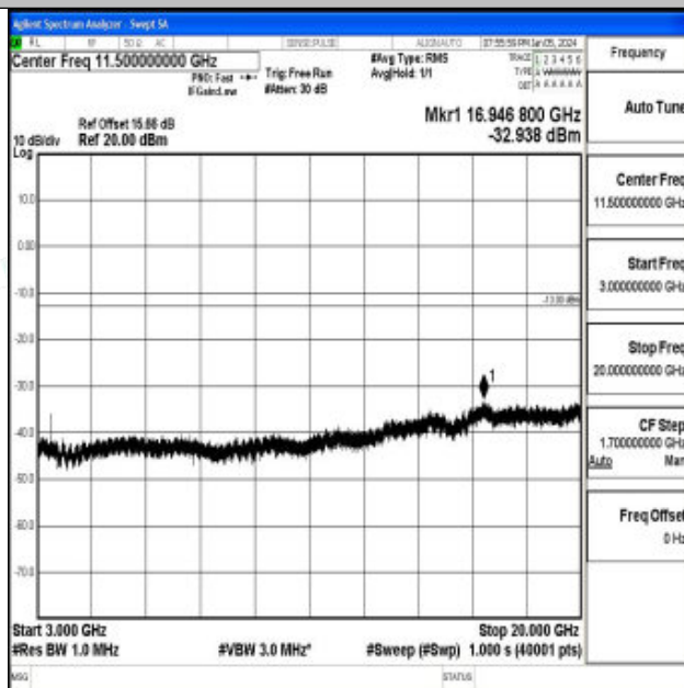
Band4_20MHz_QPSK_20050_1RB#0_3000~20000_3000~20000
