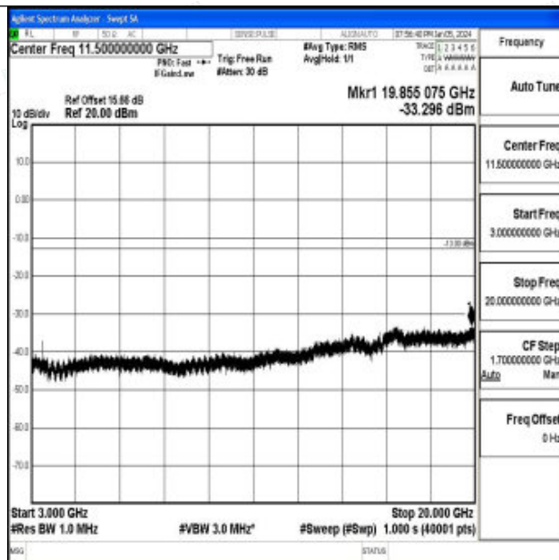
Band4_20MHz_16QAM_20050_1RB#0_3000~20000_3000~20000
