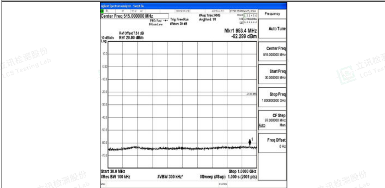
Band4_20MHz_QPSK_20300_1RB#0_30~1000_30~1000
