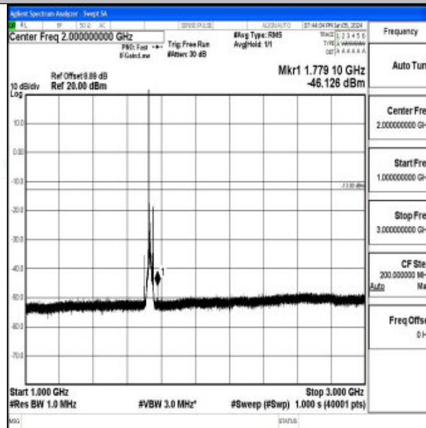
Band4_15MHz_16QAM_20175_1RB#0_1000~3000_1000~3000
