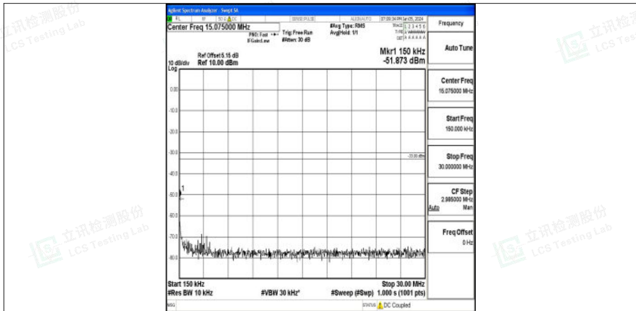
Band4_5MHz_QPSK_19975_1RB#0_0.15~30_0.15~30
