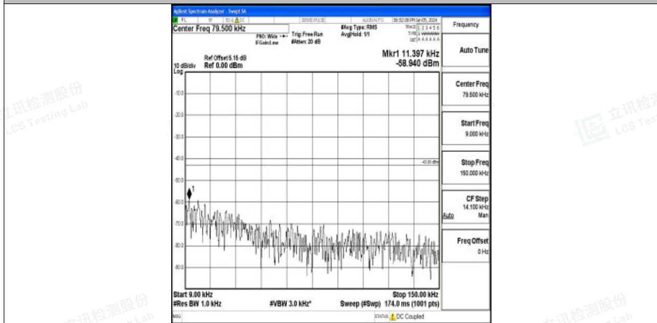
Band4_3MHz_QPSK_20175_1RB#0_0.009~0.15_0.009~0.15
