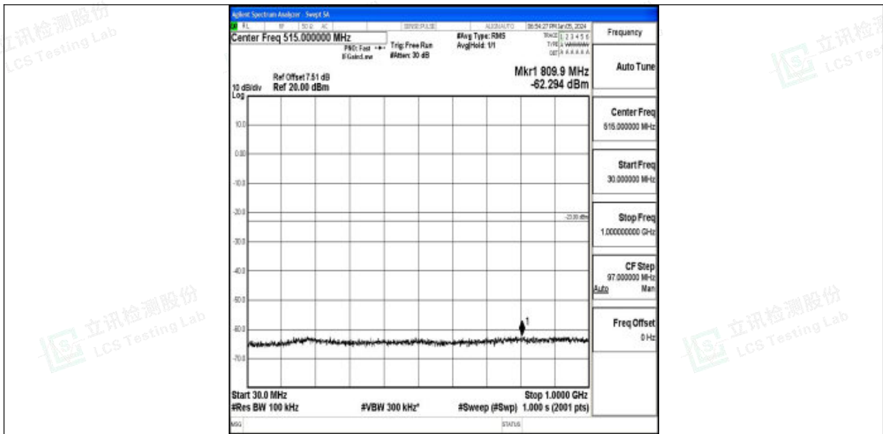
Band4_3MHz_16QAM_20385_1RB#0_30~1000_30~1000
