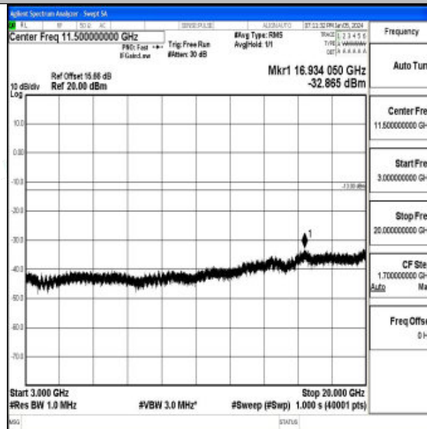
Band4_5MHz_QPSK_20175_1RB#0_3000~20000_3000~20000
