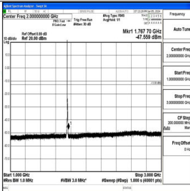
Band4_5MHz_16QAM_20375_1RB#0_1000~3000_1000~3000
