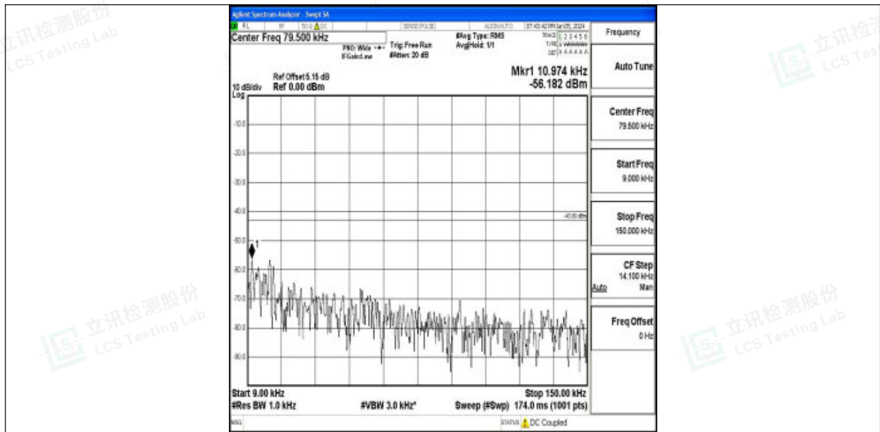
Band4_15MHz_16QAM_20175_1RB#0_0.009~0.15_0.009~0.15
