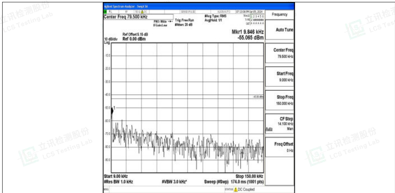
Band4_5MHz_16QAM_20375_1RB#0_0.009~0.15_0.009~0.15
