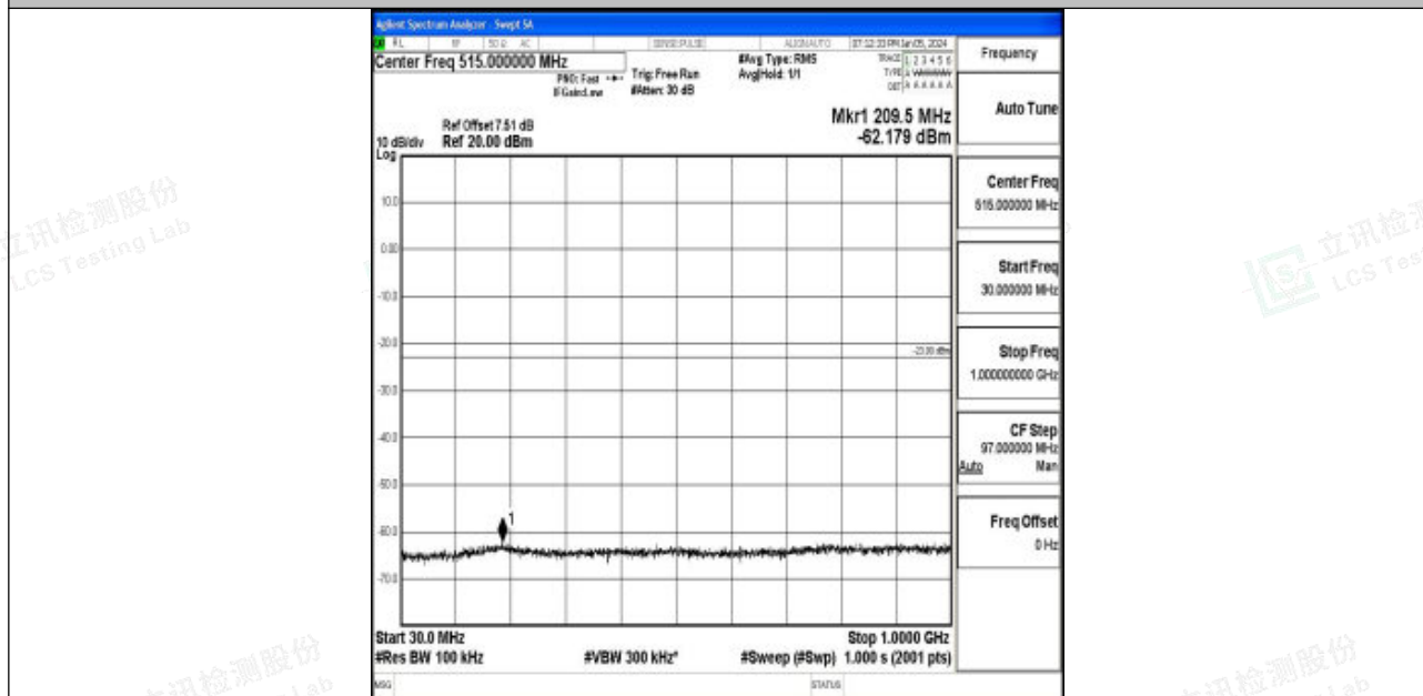
Band4_5MHz_QPSK_20375_1RB#0_30~1000_30~1000
