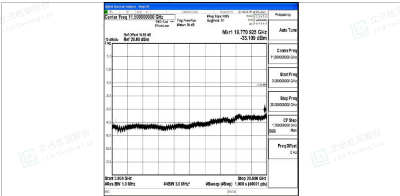
Band4_10MHz_16QAM_20000_1RB#0_3000~20000_3000~20000
