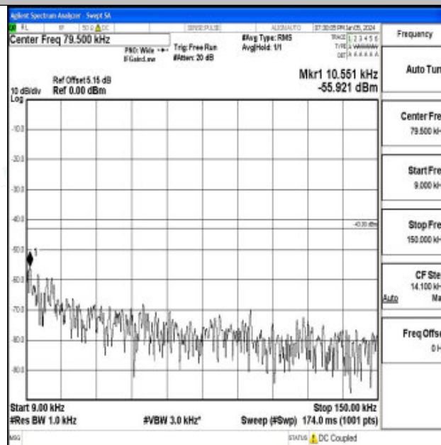
Band4_10MHz_QPSK_20350_1RB#0_0.009~0.15_0.009~0.15
