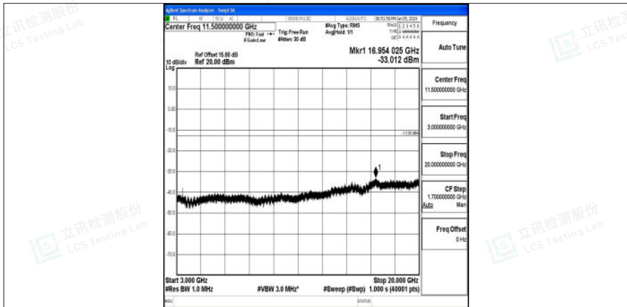
Band4_3MHz_16QAM_19965_1RB#0_3000~20000_3000~20000
