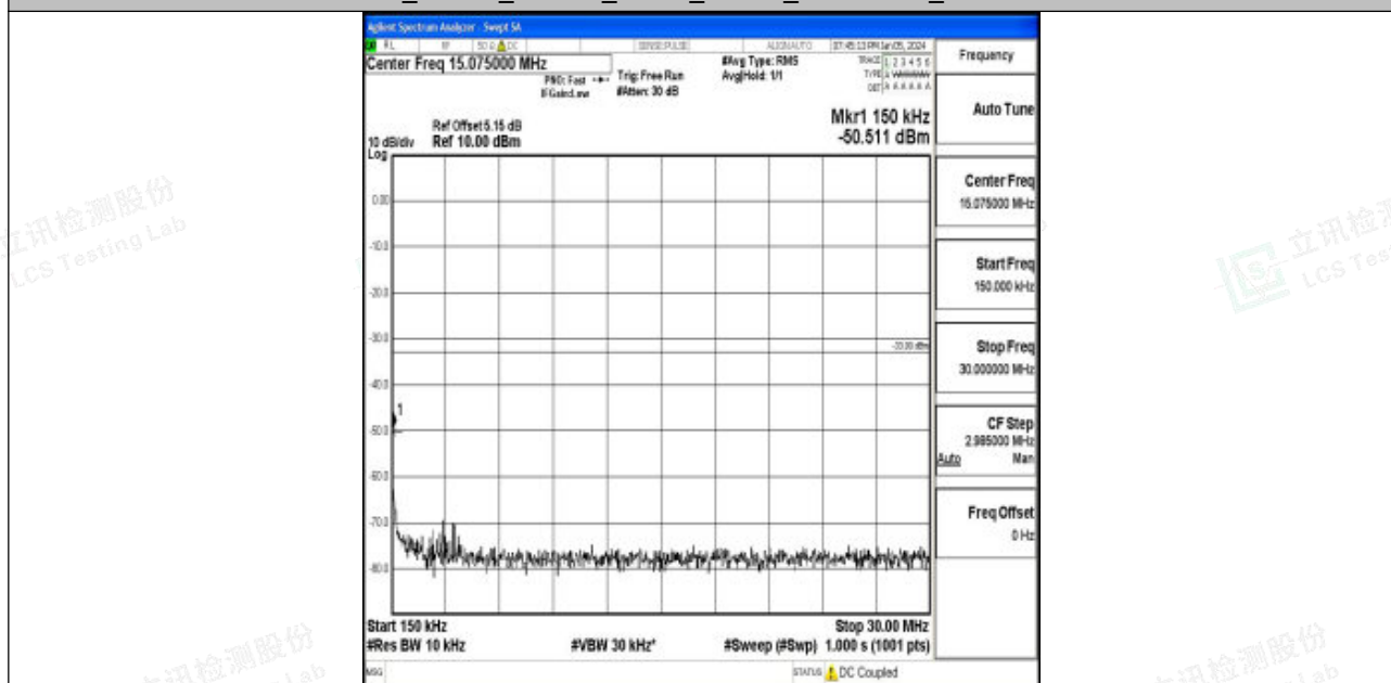
Band4_15MHz_16QAM_20325_1RB#0_0.15~30_0.15~30
