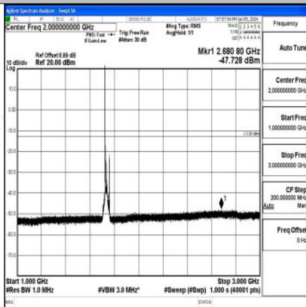
Band4_20MHz_16QAM_20175_1RB#0_1000~3000_1000~3000
