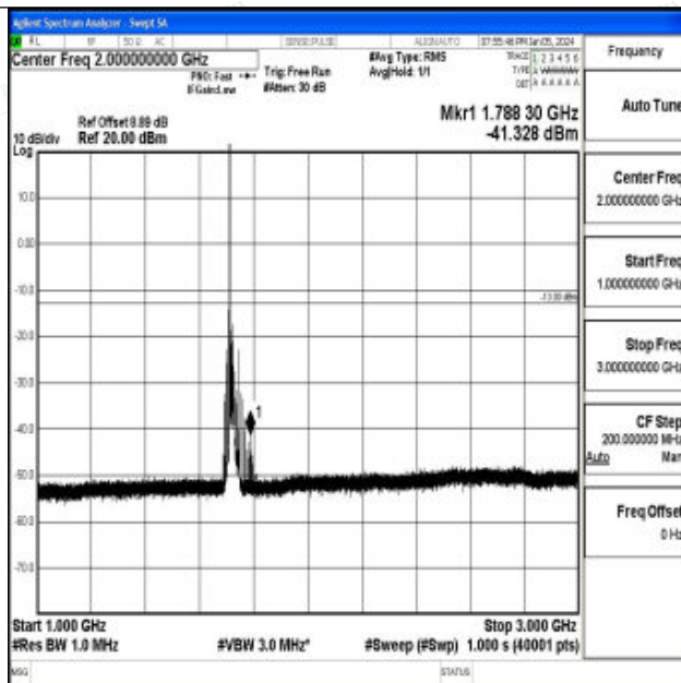
Band4_20MHz_QPSK_20050_1RB#0_1000~3000_1000~3000
