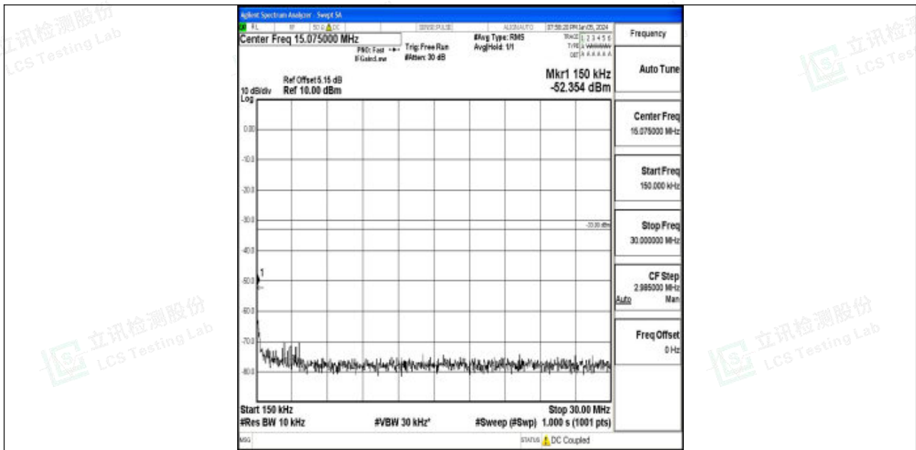
Band4_20MHz_QPSK_20300_1RB#0_0.15~30_0.15~30
