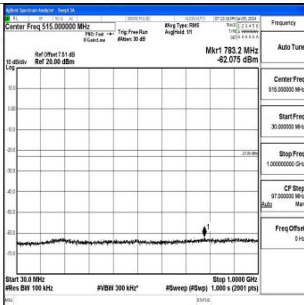
Band4_5MHz_16QAM_20375_1RB#0_30~1000_30~1000
