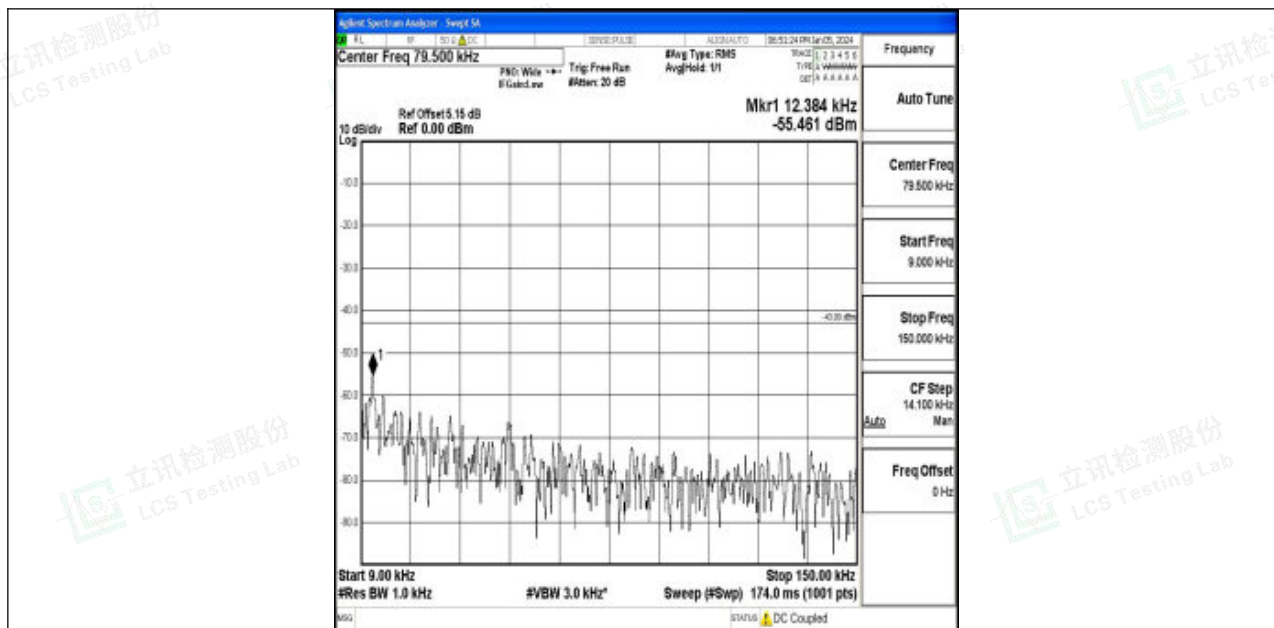
Band4_3MHz_16QAM_19965_1RB#0_0.009~0.15_0.009~0.15
