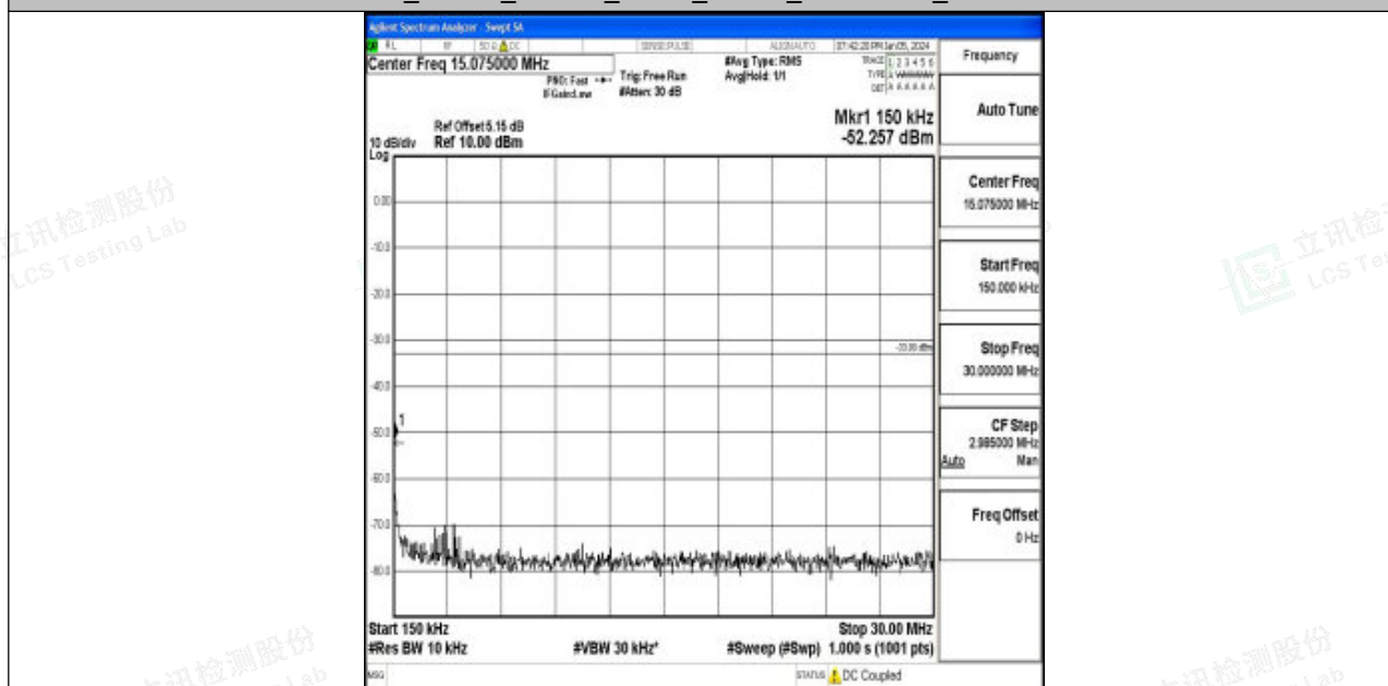
Band4_15MHz_16QAM_20025_1RB#0_0.15~30_0.15~30
