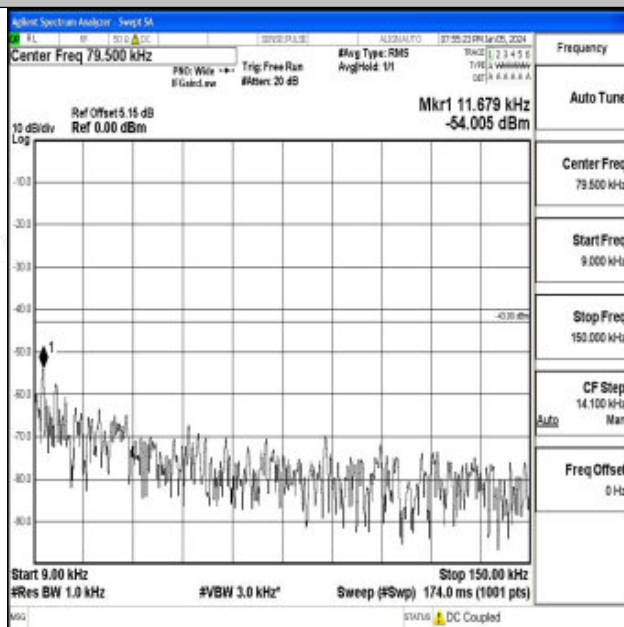
Band4_20MHz_QPSK_20050_1RB#0_0.009~0.15_0.009~0.15
