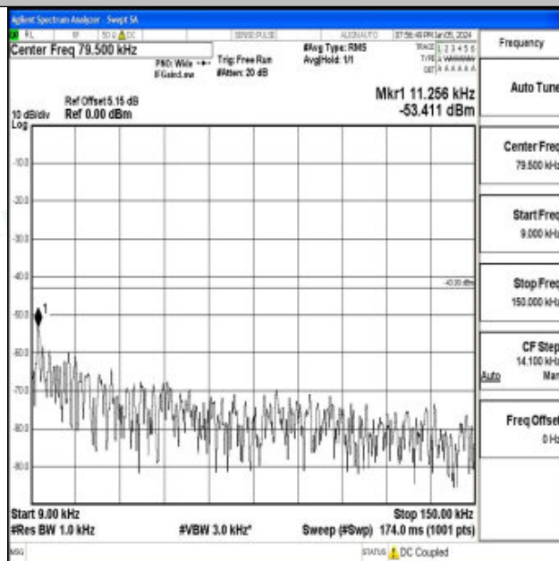
Band4_20MHz_QPSK_20175_1RB#0_0.009~0.15_0.009~0.15
