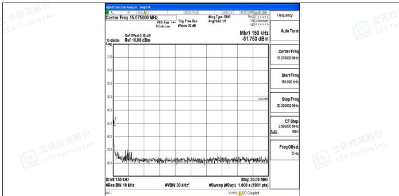
Band4_10MHz_QPSK_20000_1RB#0_0.15~30_0.15~30
