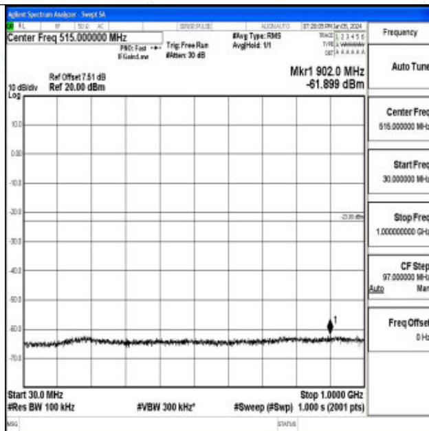
Band4_10MHz_16QAM_20000_1RB#0_30~1000_30~1000
