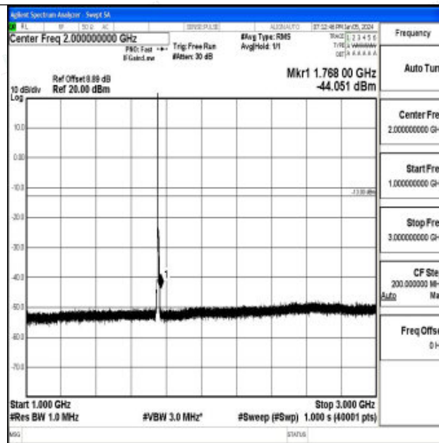
Band4_5MHz_QPSK_20375_1RB#0_1000~3000_1000~3000
