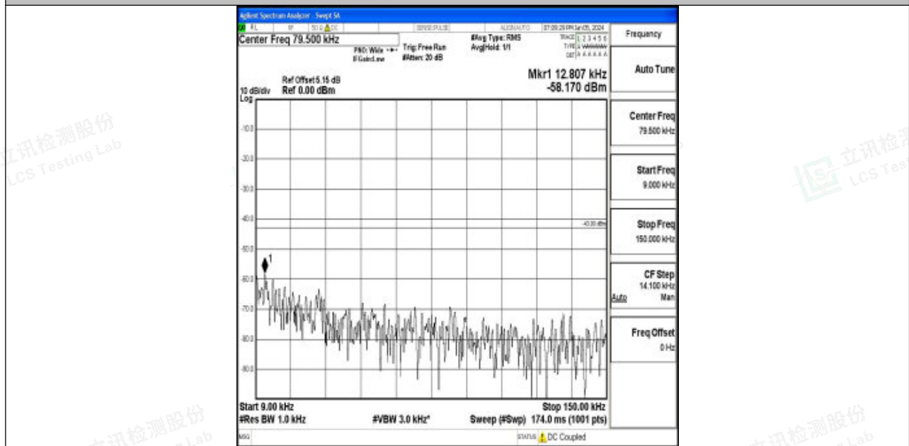
Band4_5MHz_QPSK_19975_1RB#0_0.009~0.15_0.009~0.15
