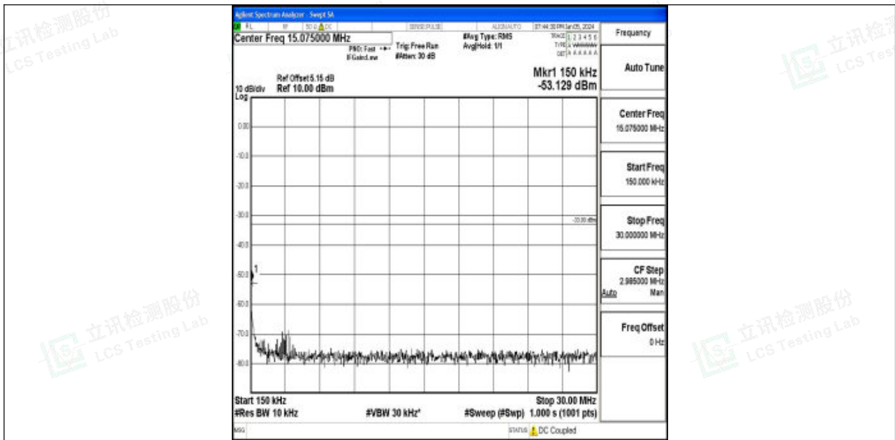
Band4_15MHz_QPSK_20325_1RB#0_0.15~30_0.15~30
