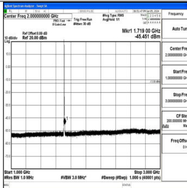
Band4_3MHz_16QAM_19965_1RB#0_1000~3000_1000~3000
