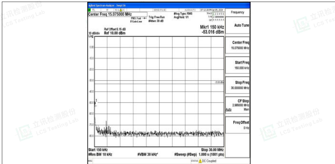
Band4_5MHz_QPSK_20375_1RB#0_0.15~30_0.15~30
