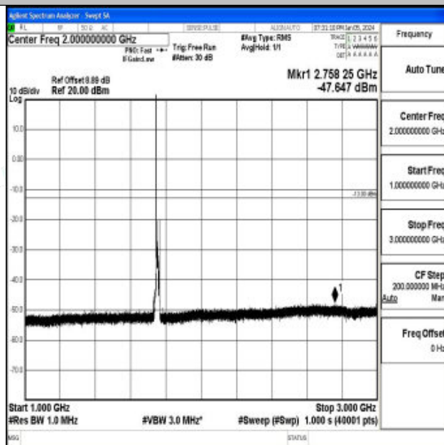
Band4_10MHz_16QAM_20350_1RB#0_1000~3000_1000~3000
