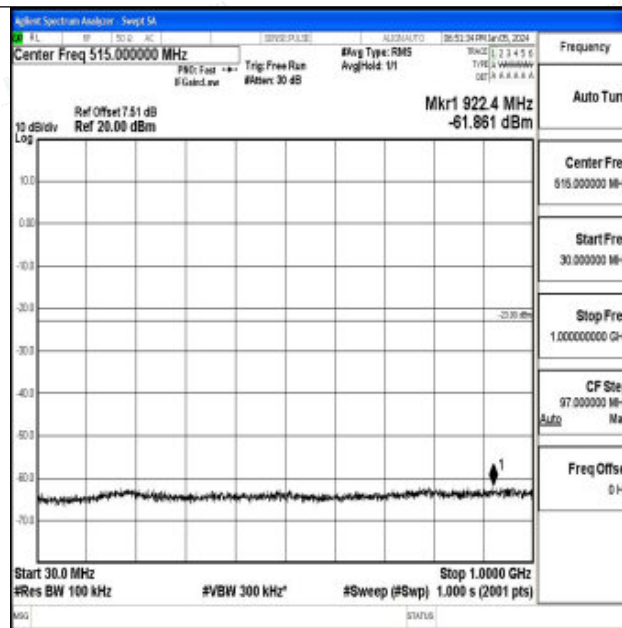
Band4_3MHz_16QAM_19965_1RB#0_30~1000_30~1000
