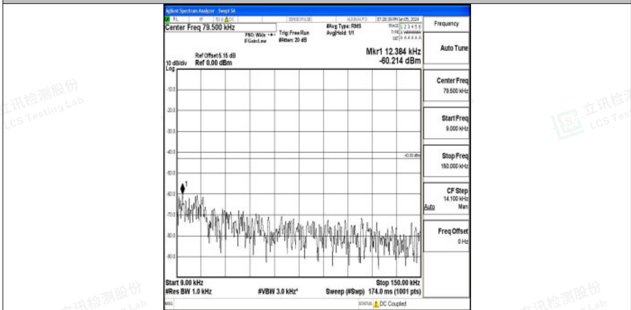
Band4_10MHz_QPSK_20175_1RB#0_0.009~0.15_0.009~0.15
