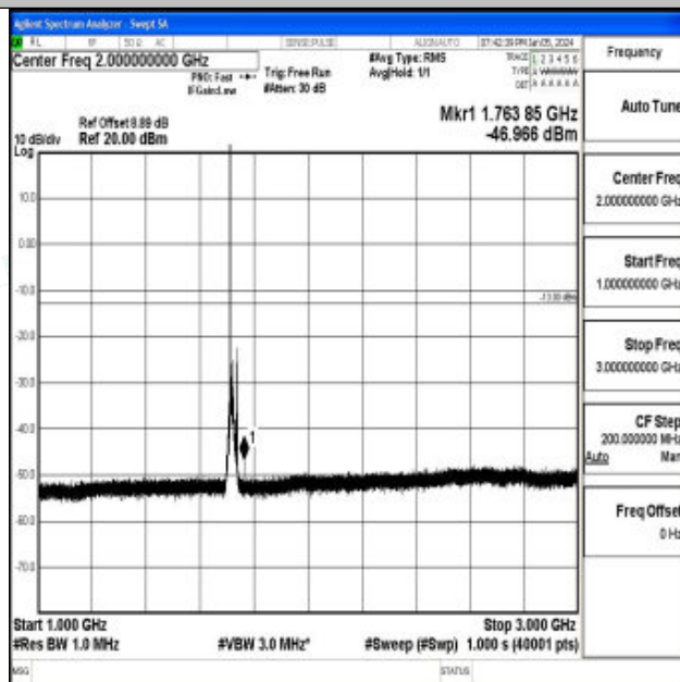
Band4_15MHz_16QAM_20025_1RB#0_1000~3000_1000~3000
