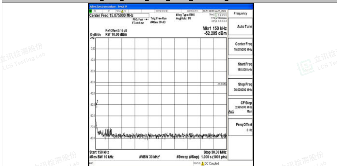
Band4_3MHz_16QAM_19965_1RB#0_0.15~30_0.15~30
