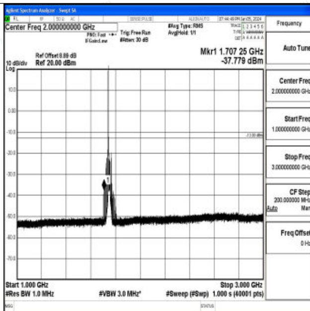
Band4_15MHz_QPSK_20325_1RB#0_1000~3000_1000~3000
