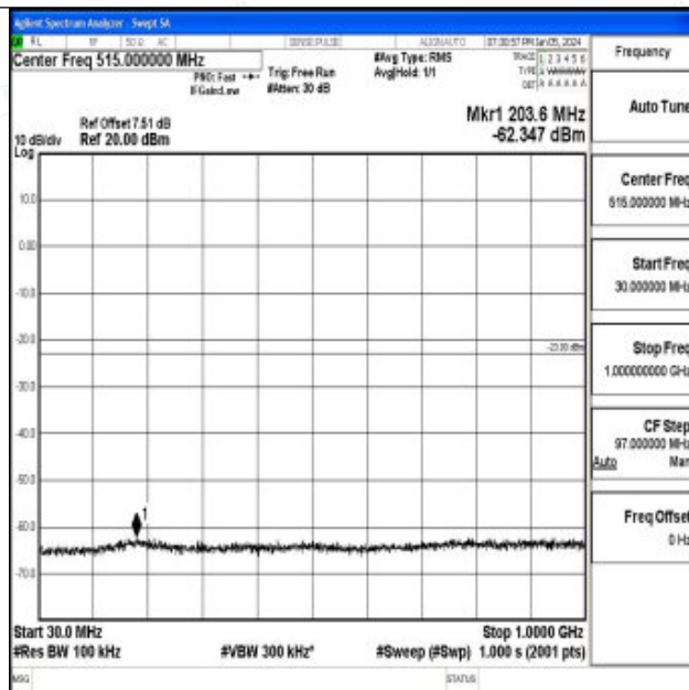
Band4_10MHz_16QAM_20350_1RB#0_30~1000_30~1000
