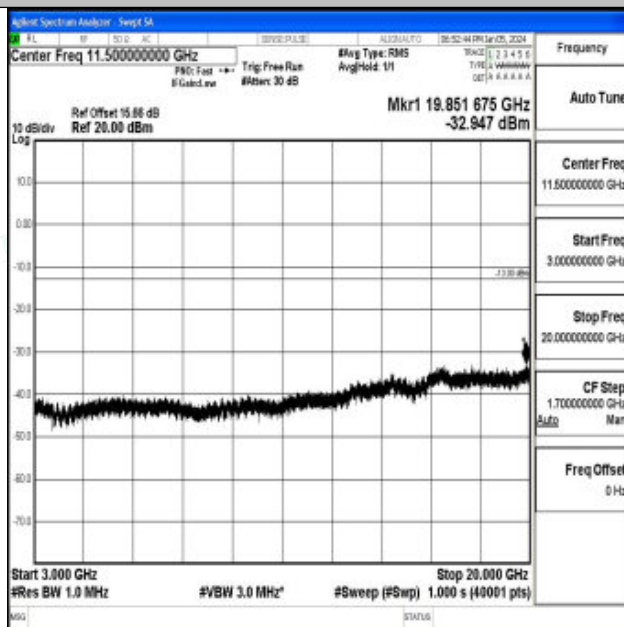
Band4_3MHz_QPSK_20175_1RB#0_3000~20000_3000~20000
