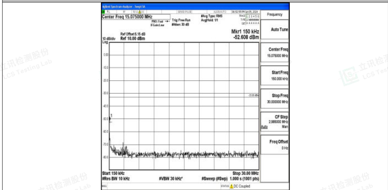
Band4_3MHz_16QAM_20175_1RB#0_0.15~30_0.15~30
