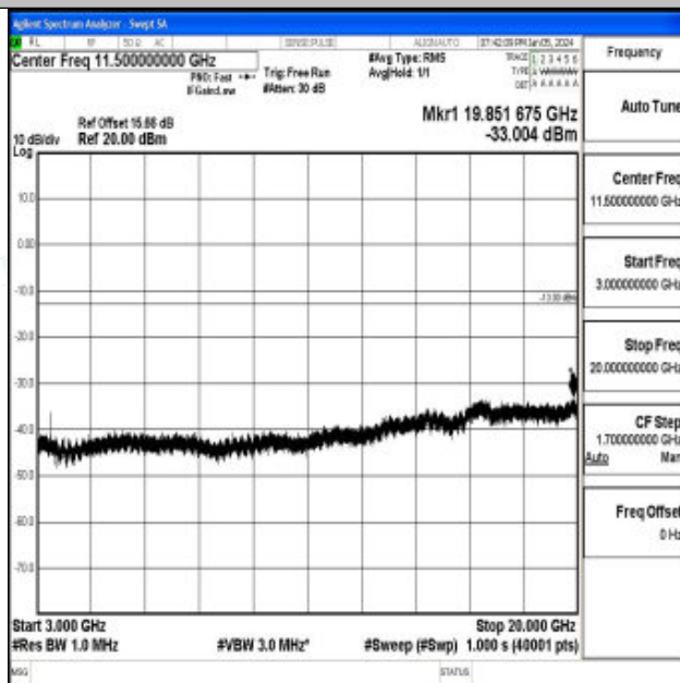
Band4_15MHz_QPSK_20025_1RB#0_3000~20000_3000~20000
