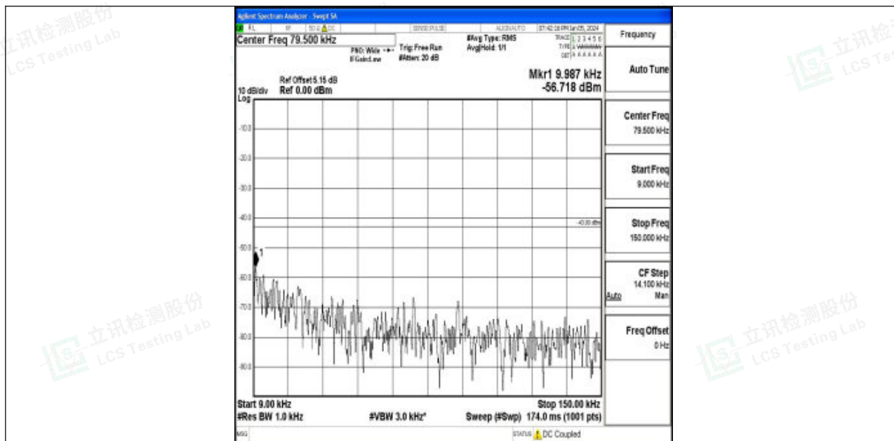
Band4_15MHz_16QAM_20025_1RB#0_0.009~0.15_0.009~0.15
