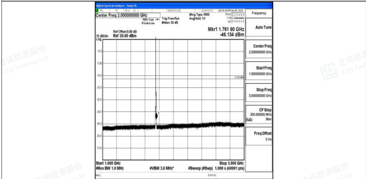
Band4_3MHz_16QAM_20385_1RB#0_1000~3000_1000~3000
