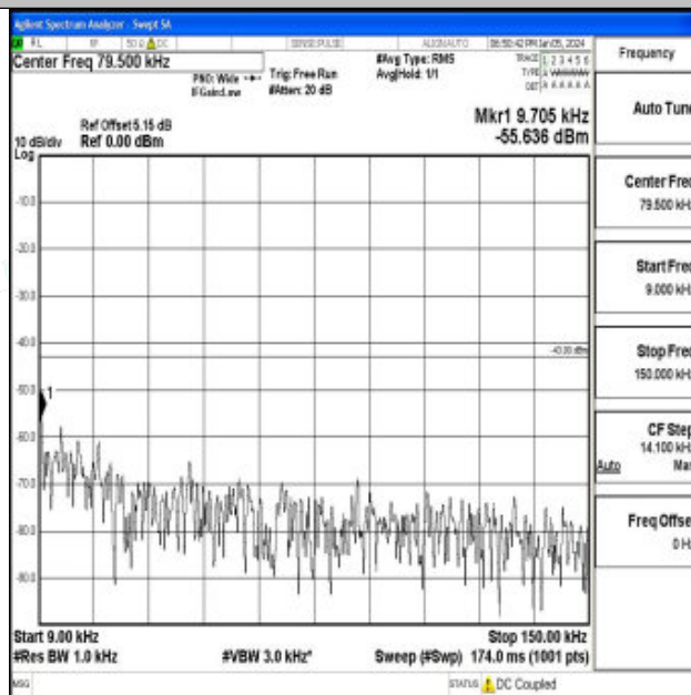
Band4_3MHz_QPSK_19965_1RB#0_0.009~0.15_0.009~0.15
