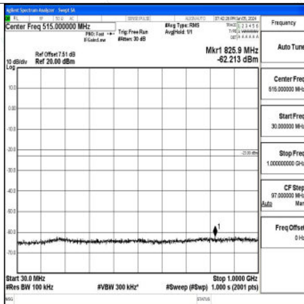
Band4_15MHz_16QAM_20025_1RB#0_30~1000_30~1000
