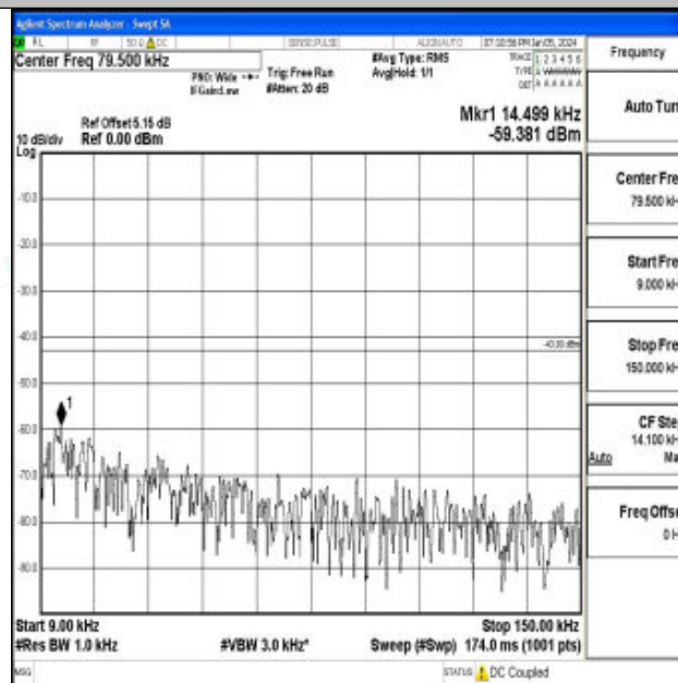
Band4_5MHz_QPSK_20175_1RB#0_0.009~0.15_0.009~0.15
