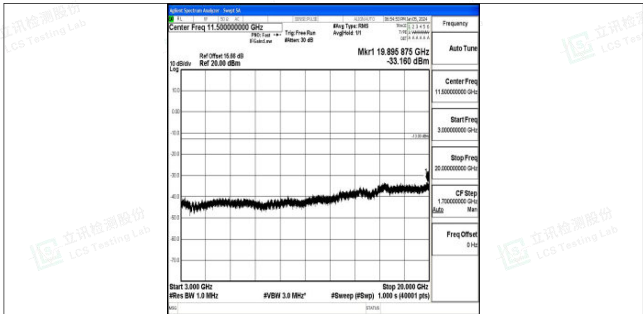
Band4_3MHz_16QAM_20385_1RB#0_3000~20000_3000~20000
