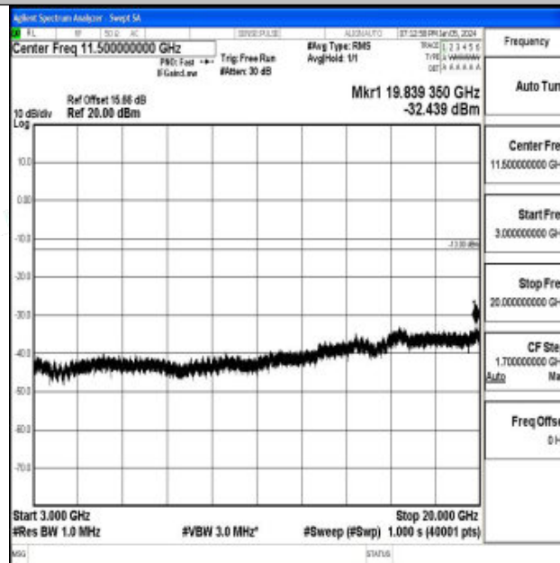
Band4_5MHz_QPSK_20375_1RB#0_3000~20000_3000~20000
