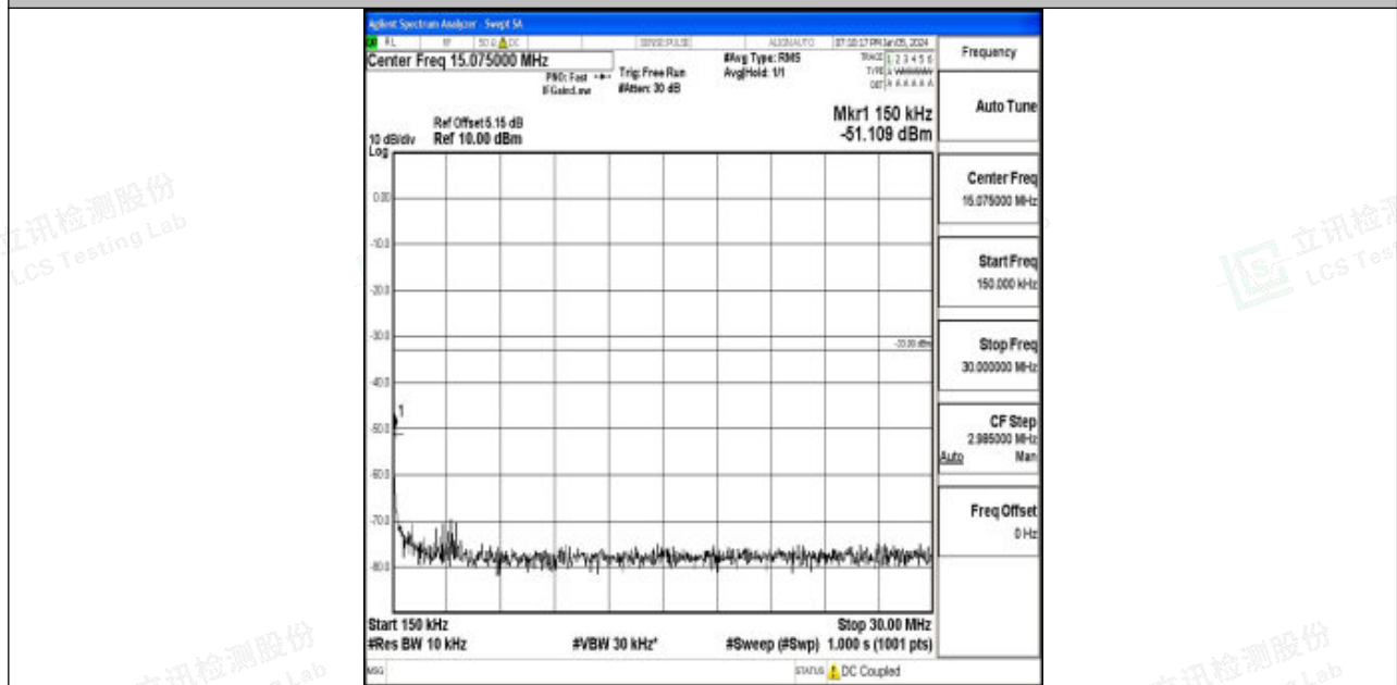
Band4_5MHz_16QAM_19975_1RB#0_0.15~30_0.15~30
