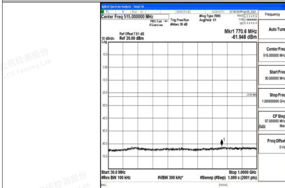
Band4_20MHz_QPSK_20175_1RB#0_30~1000_30~1000
