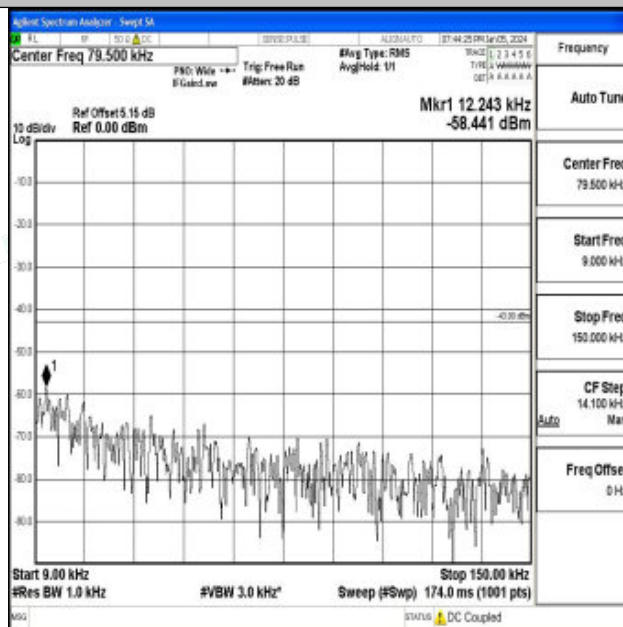
Band4_15MHz_QPSK_20325_1RB#0_0.009~0.15_0.009~0.15
