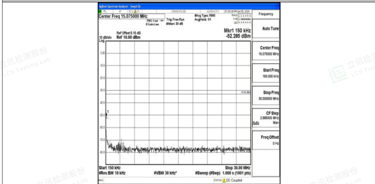
Band4_10MHz_16QAM_20175_1RB#0_0.15~30_0.15~30
