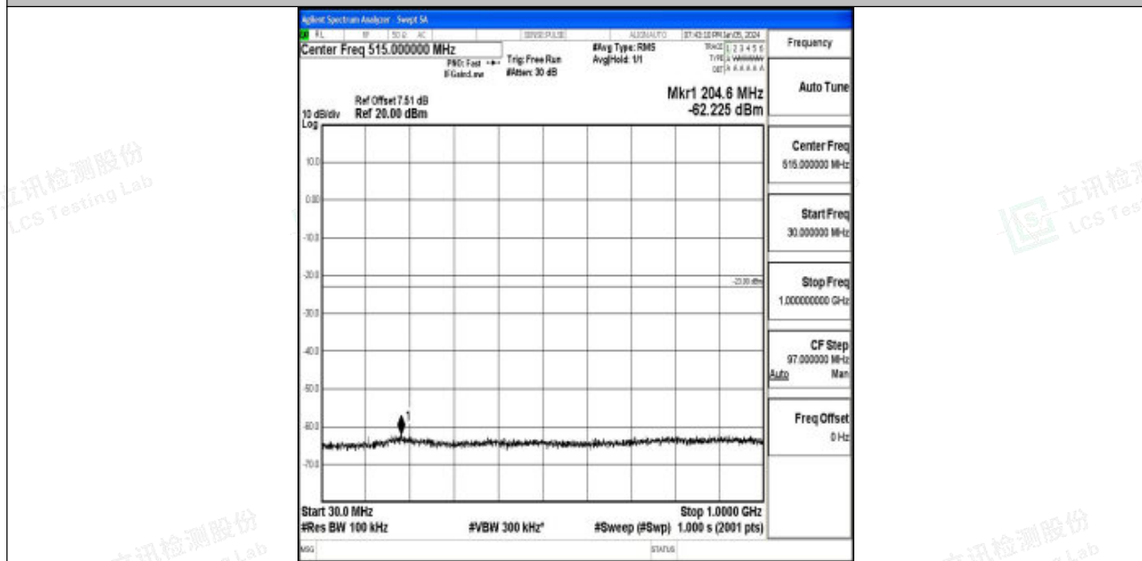
Band4_15MHz_QPSK_20175_1RB#0_30~1000_30~1000
