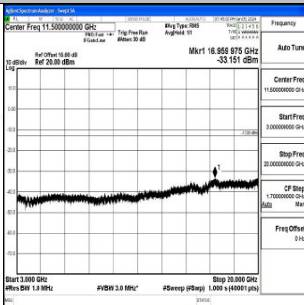
Band4_15MHz_QPSK_20325_1RB#0_3000~20000_3000~20000
