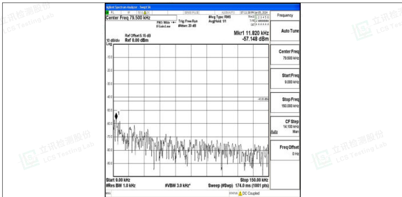
Band4_5MHz_16QAM_20175_1RB#0_0.009~0.15_0.009~0.15
