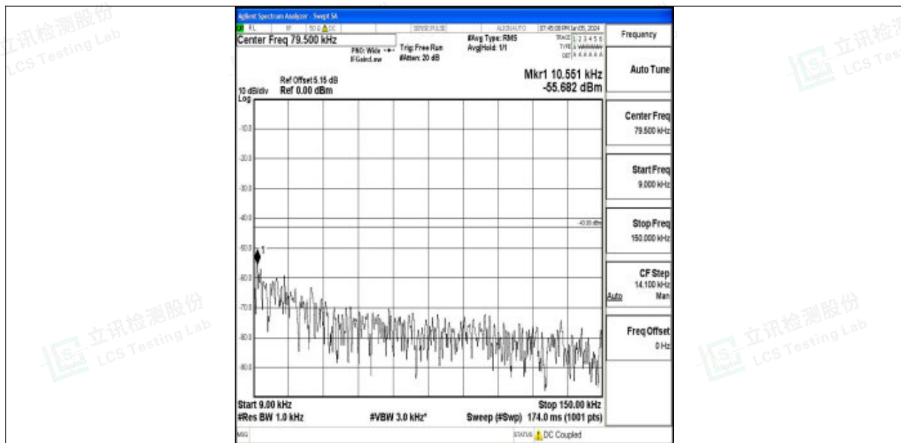
Band4_15MHz_16QAM_20325_1RB#0_0.009~0.15_0.009~0.15
