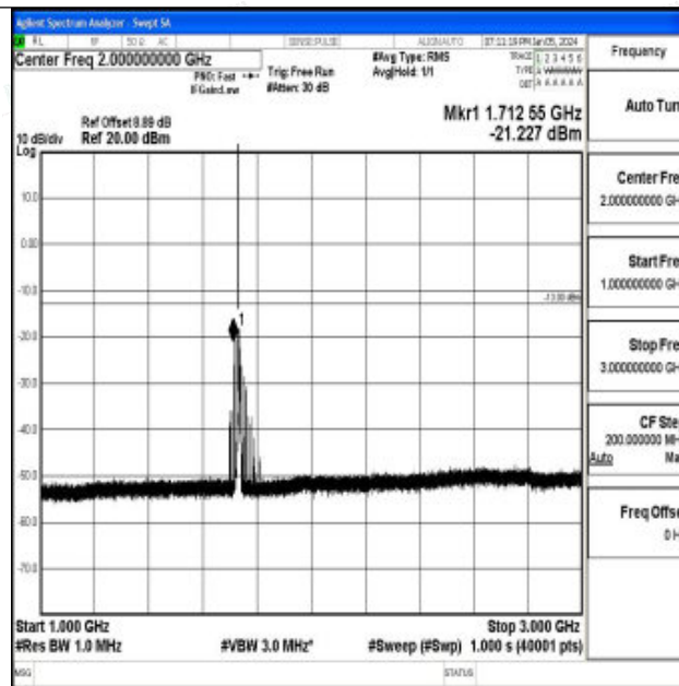
Band4_5MHz_QPSK_20175_1RB#0_1000~3000_1000~3000
