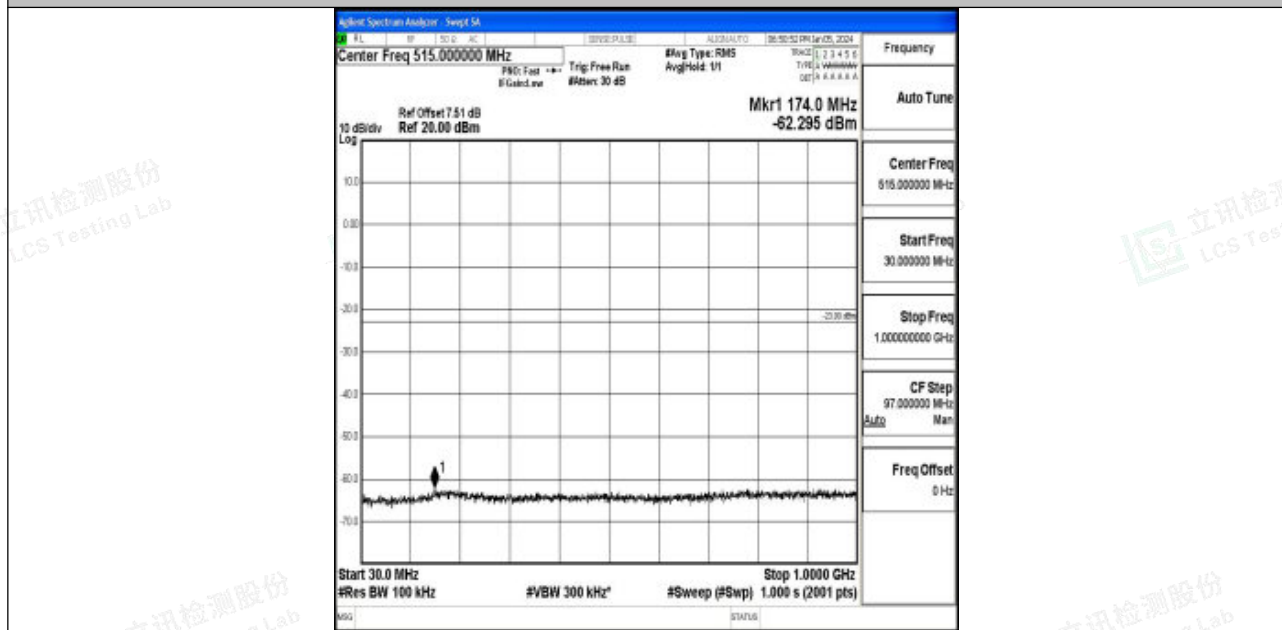
Band4_3MHz_QPSK_19965_1RB#0_30~1000_30~1000
