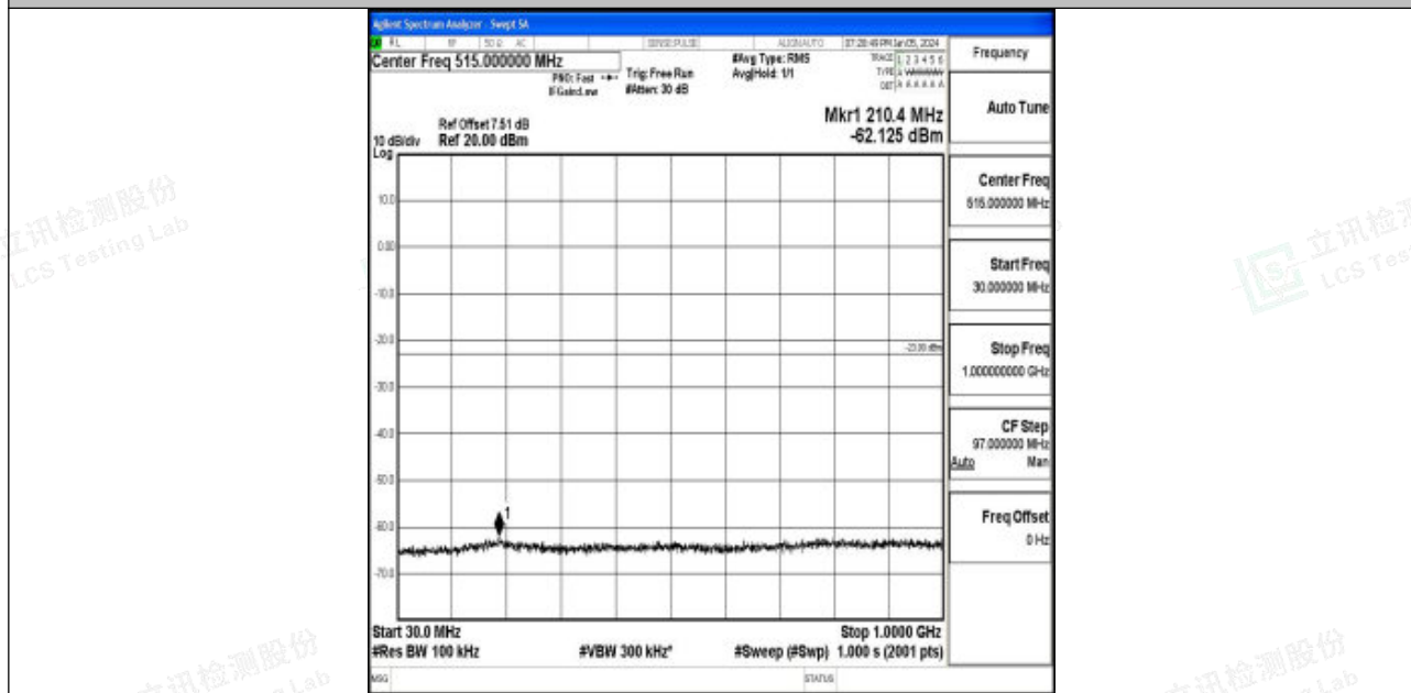
Band4_10MHz_QPSK_20175_1RB#0_30~1000_30~1000
