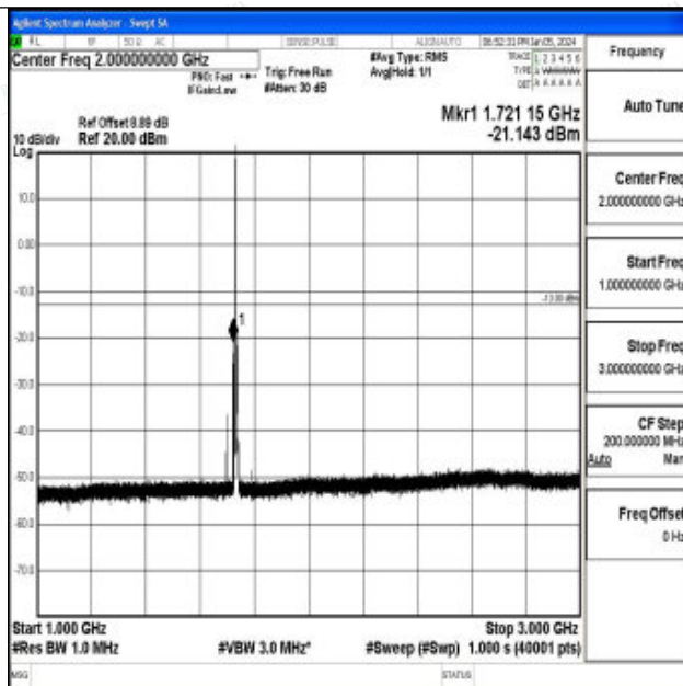
Band4_3MHz_QPSK_20175_1RB#0_1000~3000_1000~3000
