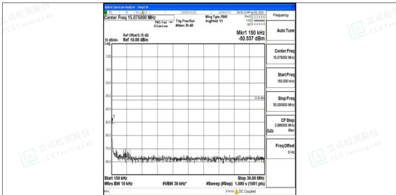
Band4_3MHz_QPSK_20175_1RB#0_0.15~30_0.15~30
