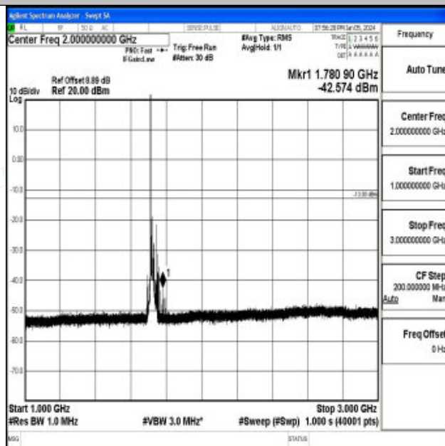
Band4_20MHz_16QAM_20050_1RB#0_1000~3000_1000~3000
