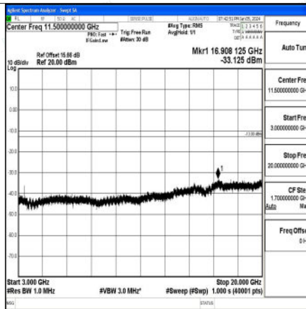
Band4_15MHz_16QAM_20025_1RB#0_3000~20000_3000~20000
