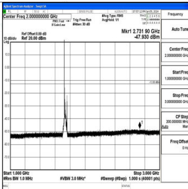
Band4_20MHz_QPSK_20175_1RB#0_1000~3000_1000~3000
