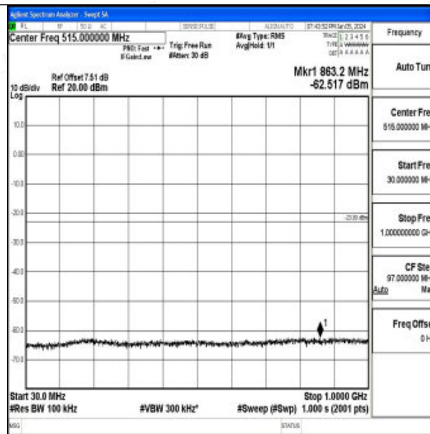
Band4_15MHz_16QAM_20175_1RB#0_30~1000_30~1000
