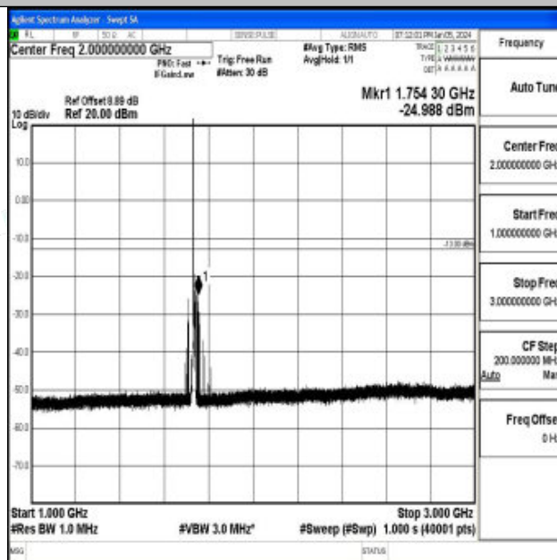
Band4_5MHz_16QAM_20175_1RB#0_1000~3000_1000~3000
