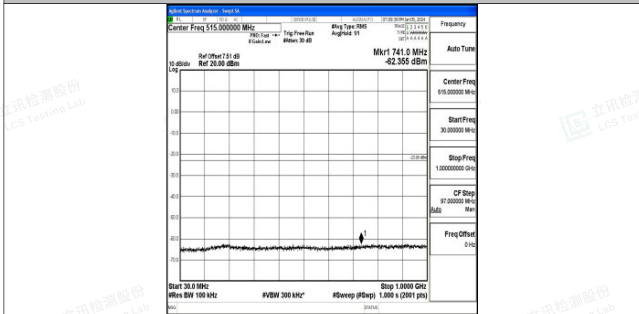
Band4_5MHz_QPSK_19975_1RB#0_30~1000_30~1000
