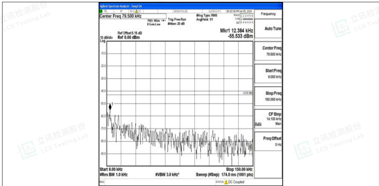
Band4_3MHz_16QAM_20175_1RB#0_0.009~0.15_0.009~0.15
