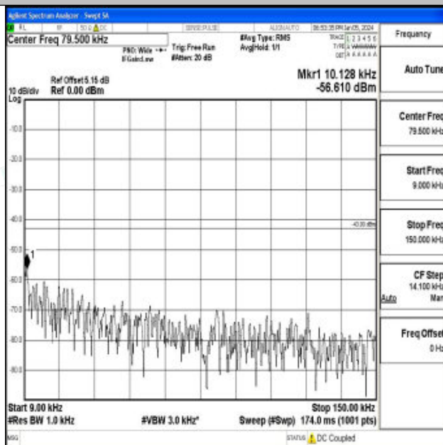
Band4_3MHz_QPSK_20385_1RB#0_0.009~0.15_0.009~0.15
