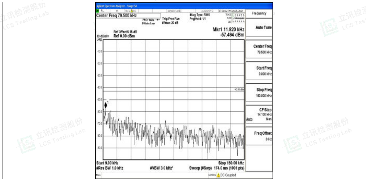
Band4_5MHz_16QAM_19975_1RB#0_0.009~0.15_0.009~0.15
