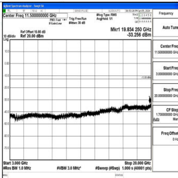
Band4_3MHz_16QAM_20175_1RB#0_3000~20000_3000~20000
