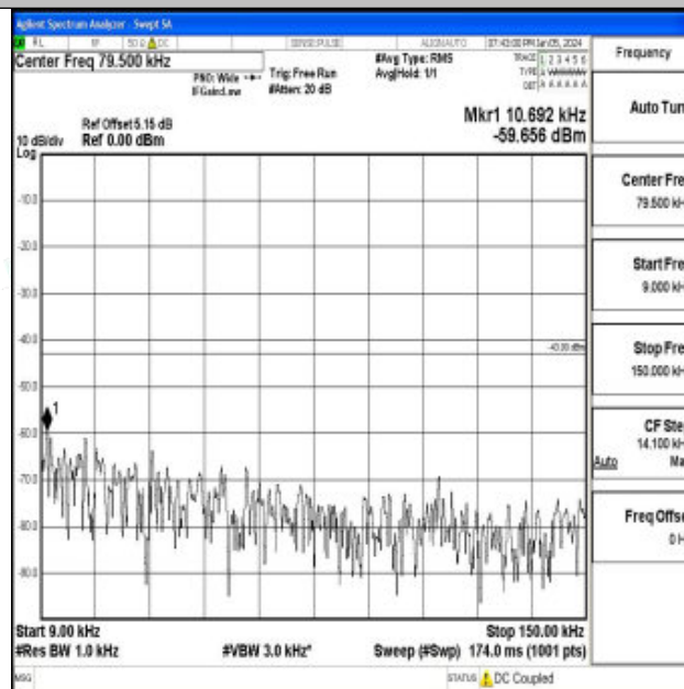
Band4_15MHz_QPSK_20175_1RB#0_0.009~0.15_0.009~0.15
