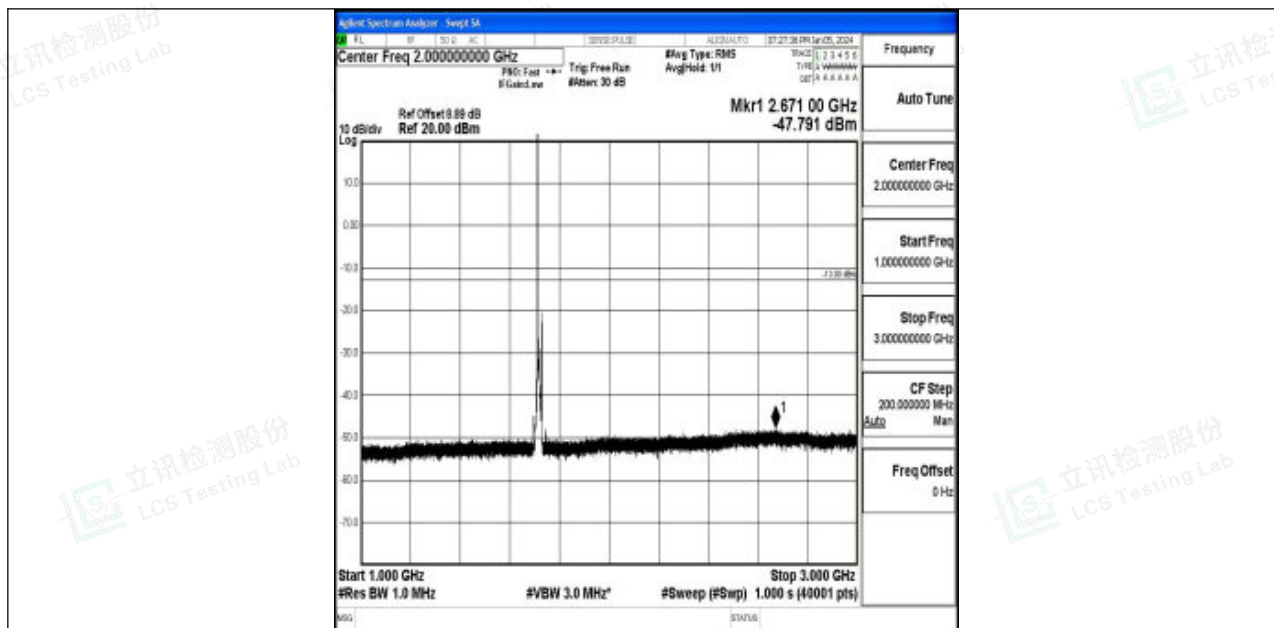
Band4_10MHz_QPSK_20000_1RB#0_1000~3000_1000~3000
