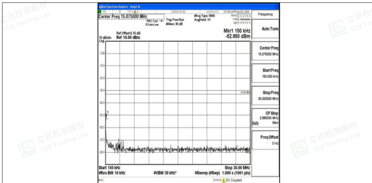
Band4_10MHz_QPSK_20350_1RB#0_0.15~30_0.15~30
