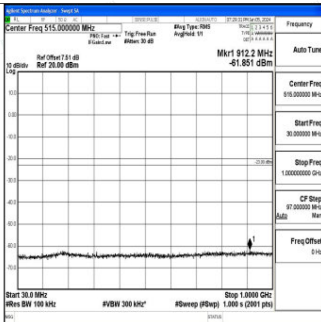
Band4_10MHz_16QAM_20175_1RB#0_30~1000_30~1000
