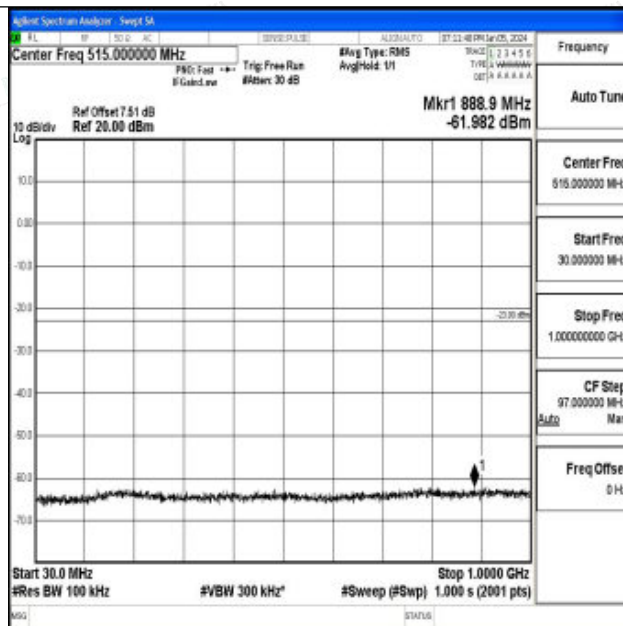
Band4_5MHz_16QAM_20175_1RB#0_30~1000_30~1000
