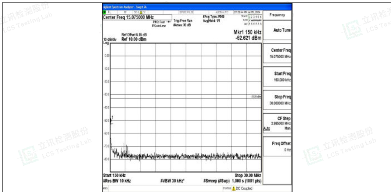
Band4_10MHz_QPSK_20175_1RB#0_0.15~30_0.15~30
