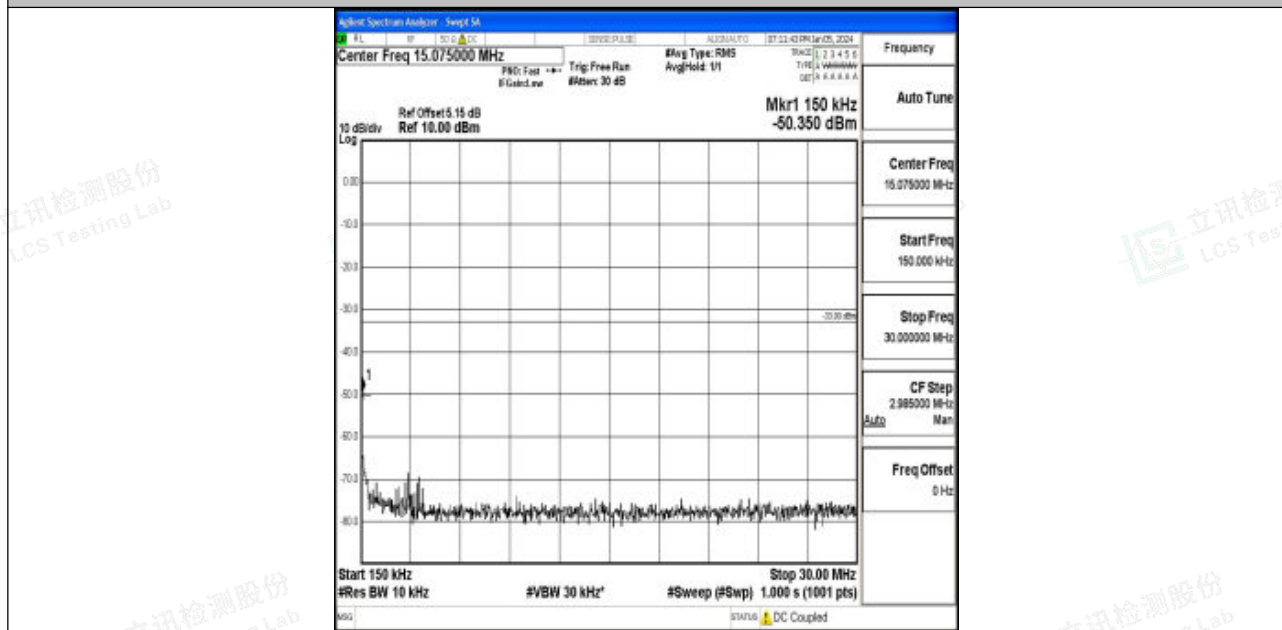
Band4_5MHz_16QAM_20175_1RB#0_0.15~30_0.15~30
