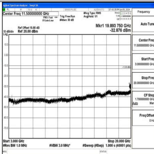
Band4_15MHz_QPSK_20175_1RB#0_3000~20000_3000~20000
