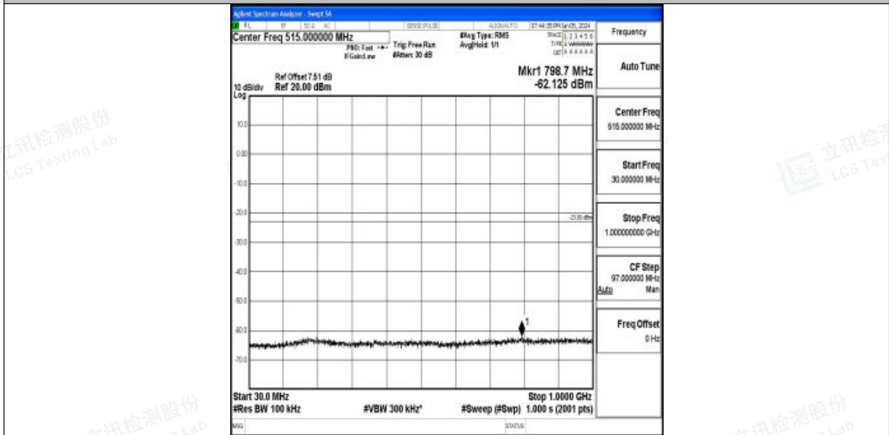
Band4_15MHz_QPSK_20325_1RB#0_30~1000_30~1000
