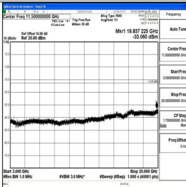
Band4_20MHz_QPSK_20175_1RB#0_3000~20000_3000~20000
