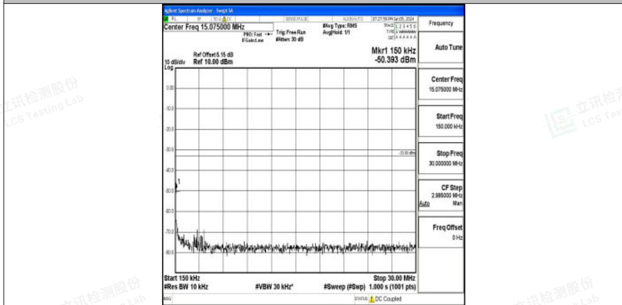
Band4_10MHz_16QAM_20000_1RB#0_0.15~30_0.15~30
