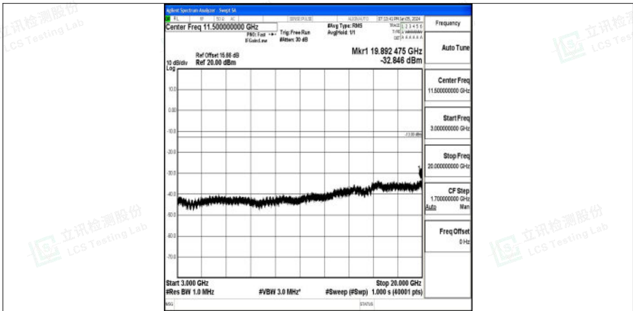
Band4_5MHz_16QAM_20375_1RB#0_3000~20000_3000~20000
