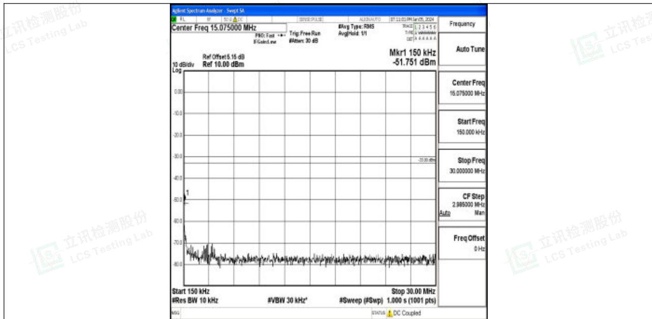
Band4_5MHz_QPSK_20175_1RB#0_0.15~30_0.15~30
