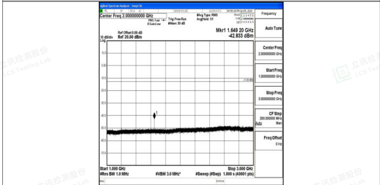
Band5_10MHz_QPSK_20450_1RB#0_1000~3000_1000~3000
