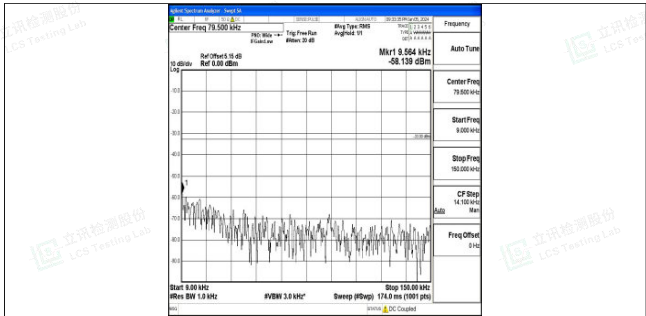
Band5_5MHz_QPSK_20525_1RB#0_0.009~0.15_0.009~0.15
