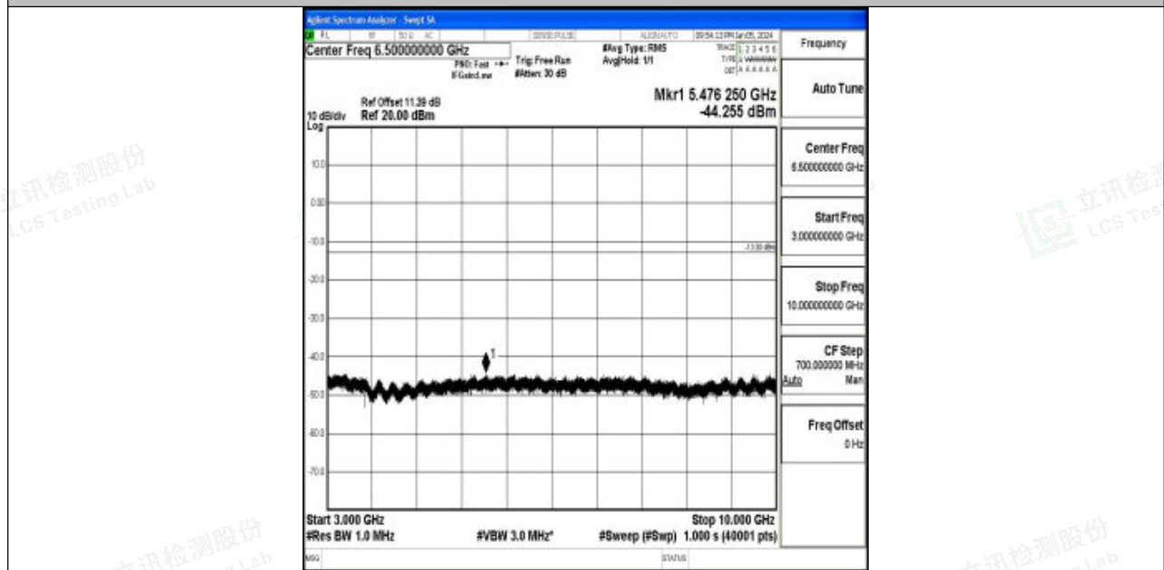
Band5_10MHz_16QAM_20600_1RB#0_3000~10000_3000~10000
