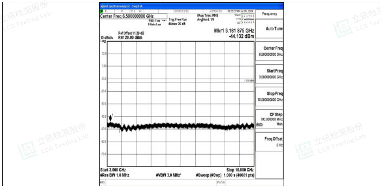
Band5_5MHz_QPSK_20625_1RB#0_3000~10000_3000~10000
