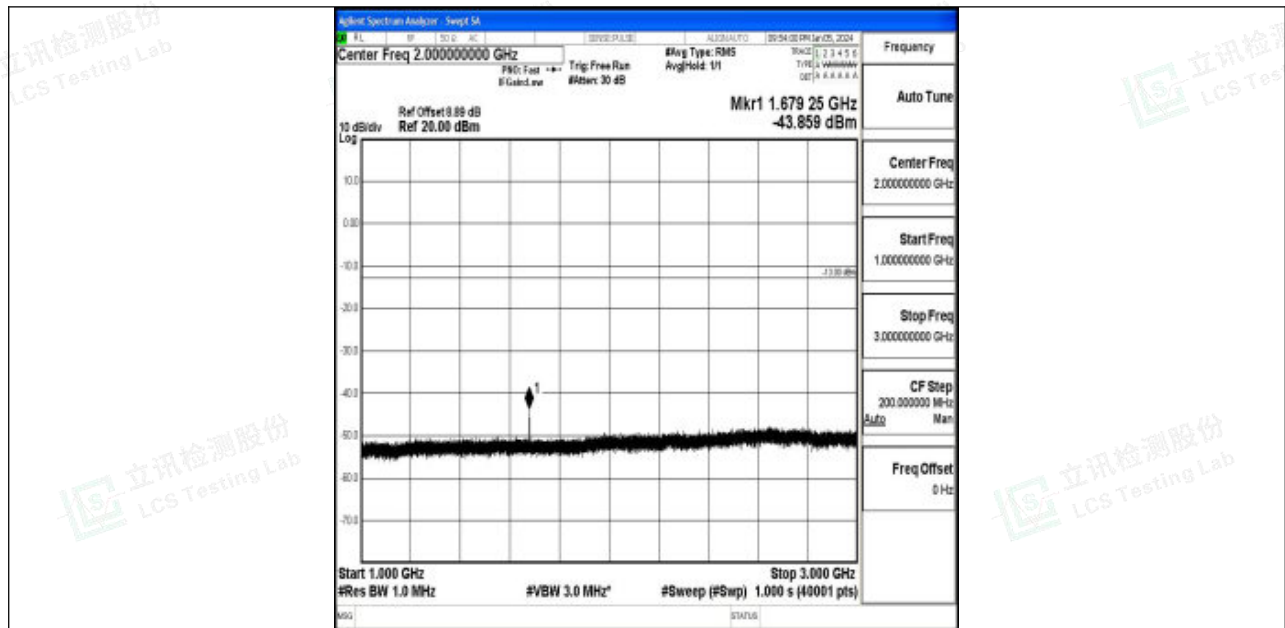
Band5_10MHz_16QAM_20600_1RB#0_1000~3000_1000~3000
