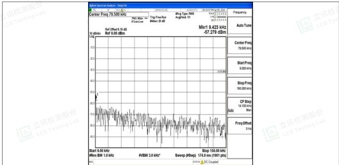
Band5_3MHz_QPSK_20635_1RB#0_0.009~0.15_0.009~0.15
