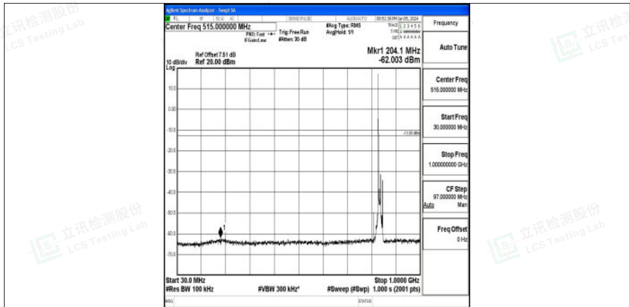
Band5_10MHz_QPSK_20525_1RB#0_30~1000_30~1000
