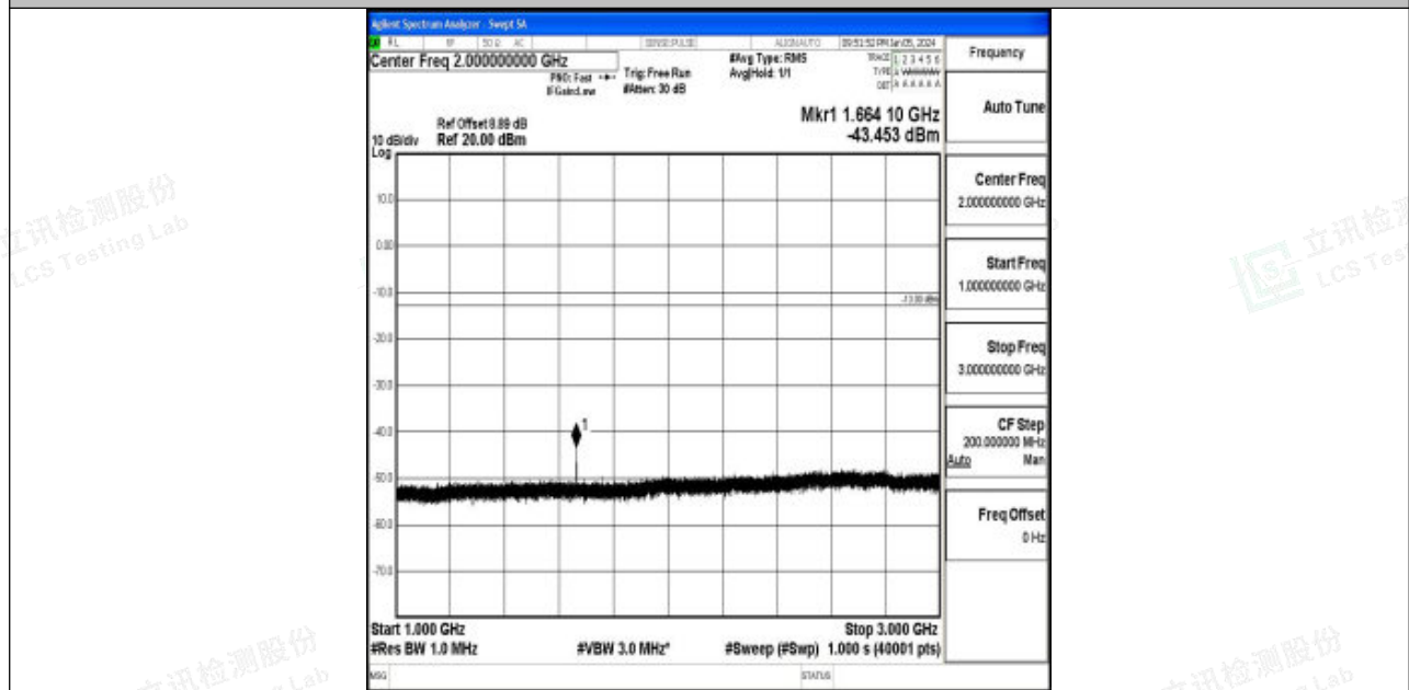
Band5_10MHz_QPSK_20525_1RB#0_1000~3000_1000~3000
