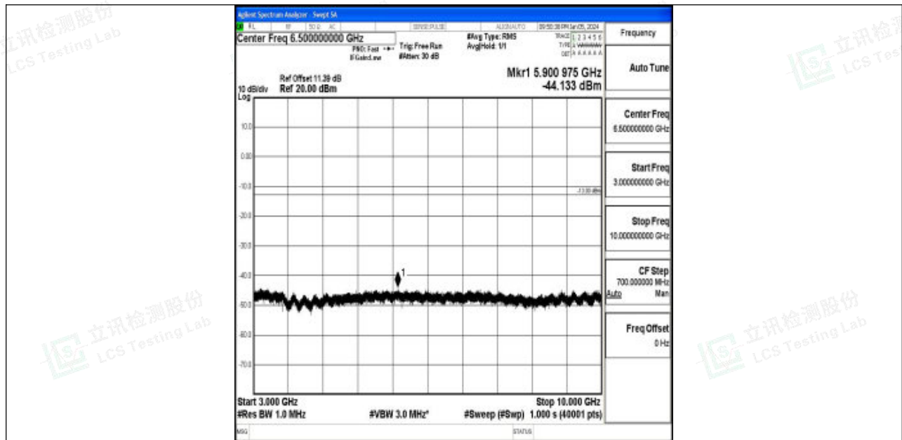
Band5_10MHz_QPSK_20450_1RB#0_3000~10000_3000~10000
