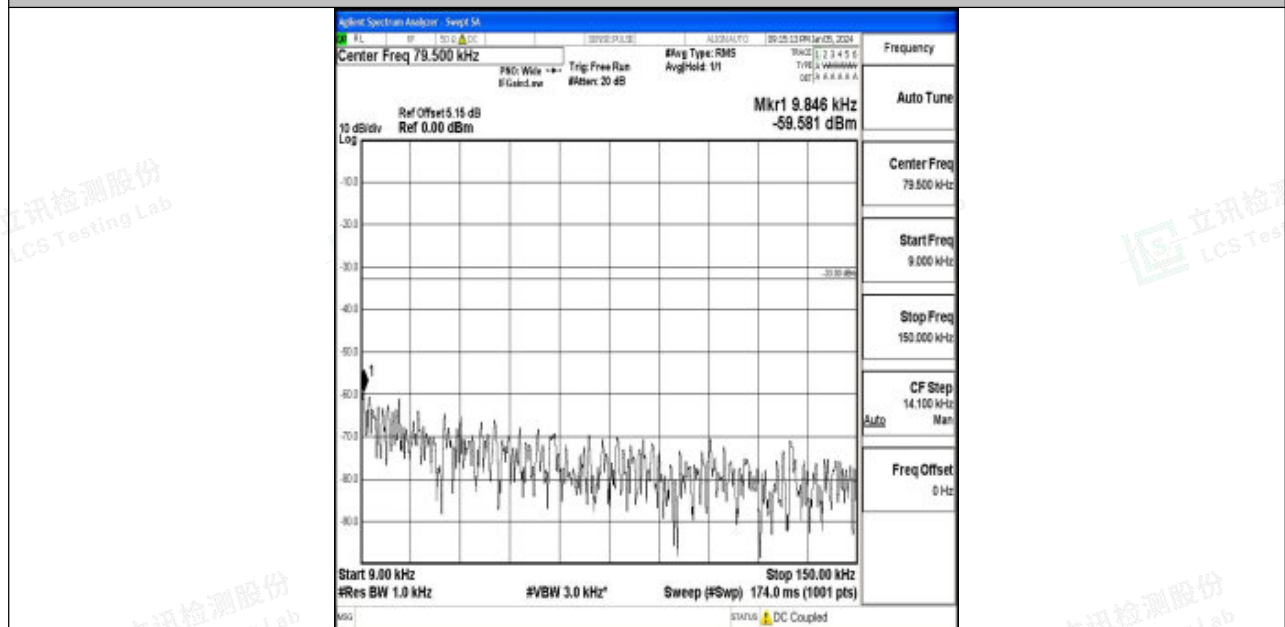
Band5_3MHz_16QAM_20525_1RB#0_0.009~0.15_0.009~0.15
