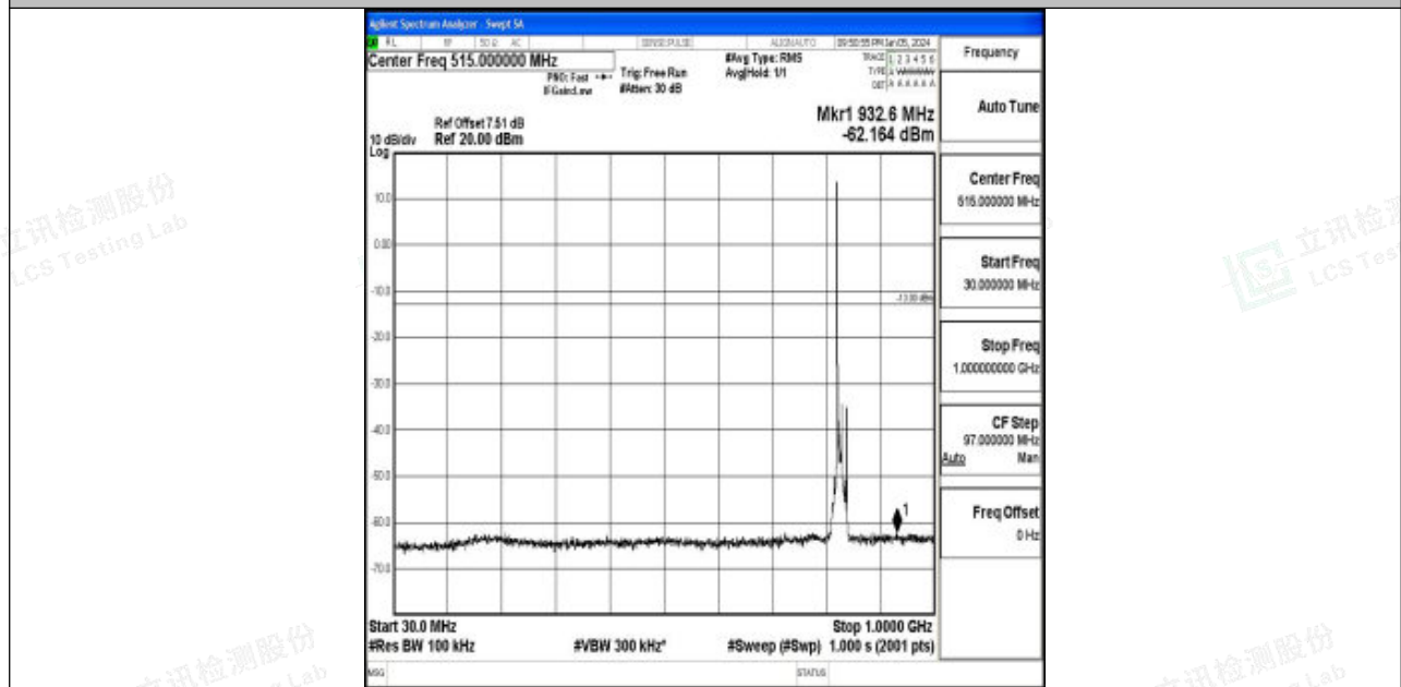
Band5_10MHz_16QAM_20450_1RB#0_30~1000_30~1000
