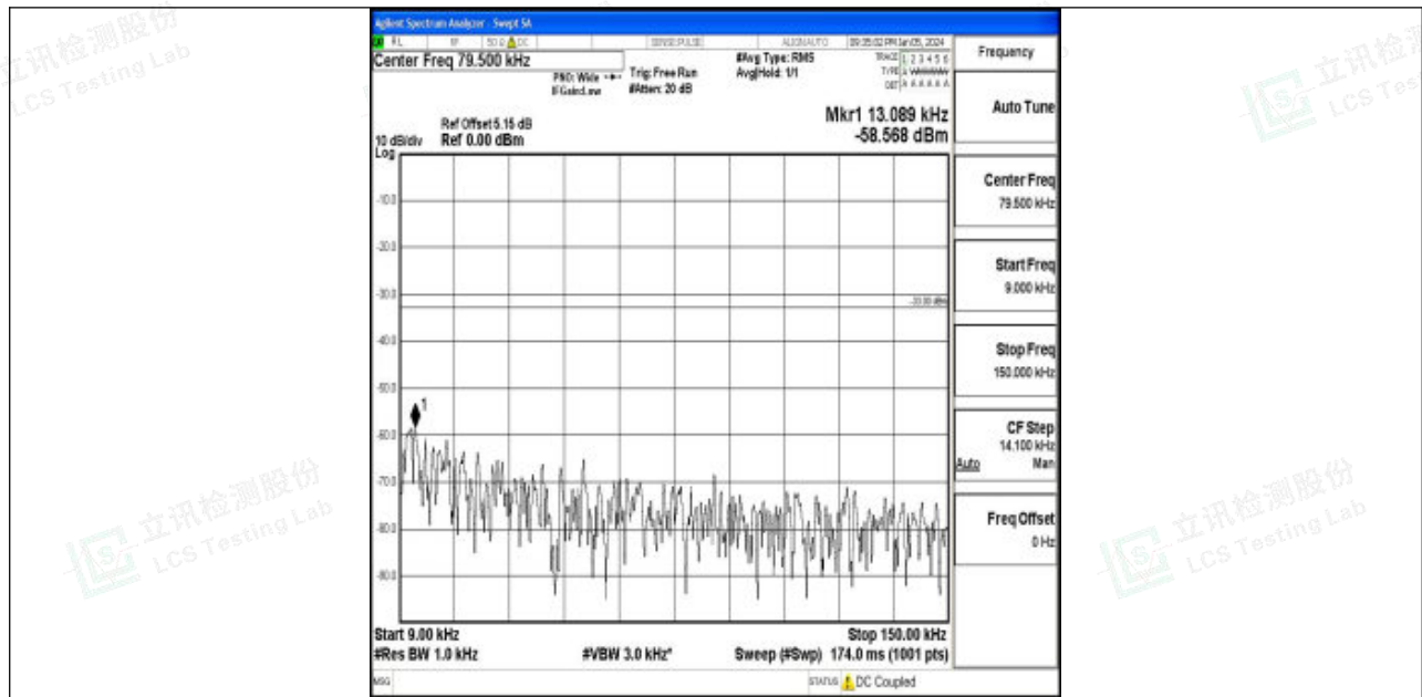
Band5_5MHz_QPSK_20625_1RB#0_0.009~0.15_0.009~0.15
