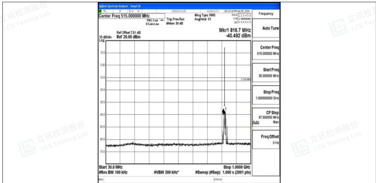
Band5_3MHz_QPSK_20415_1RB#0_30~1000_30~1000
