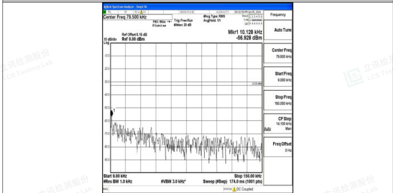
Band5_5MHz_16QAM_20425_1RB#0_0.009~0.15_0.009~0.15
