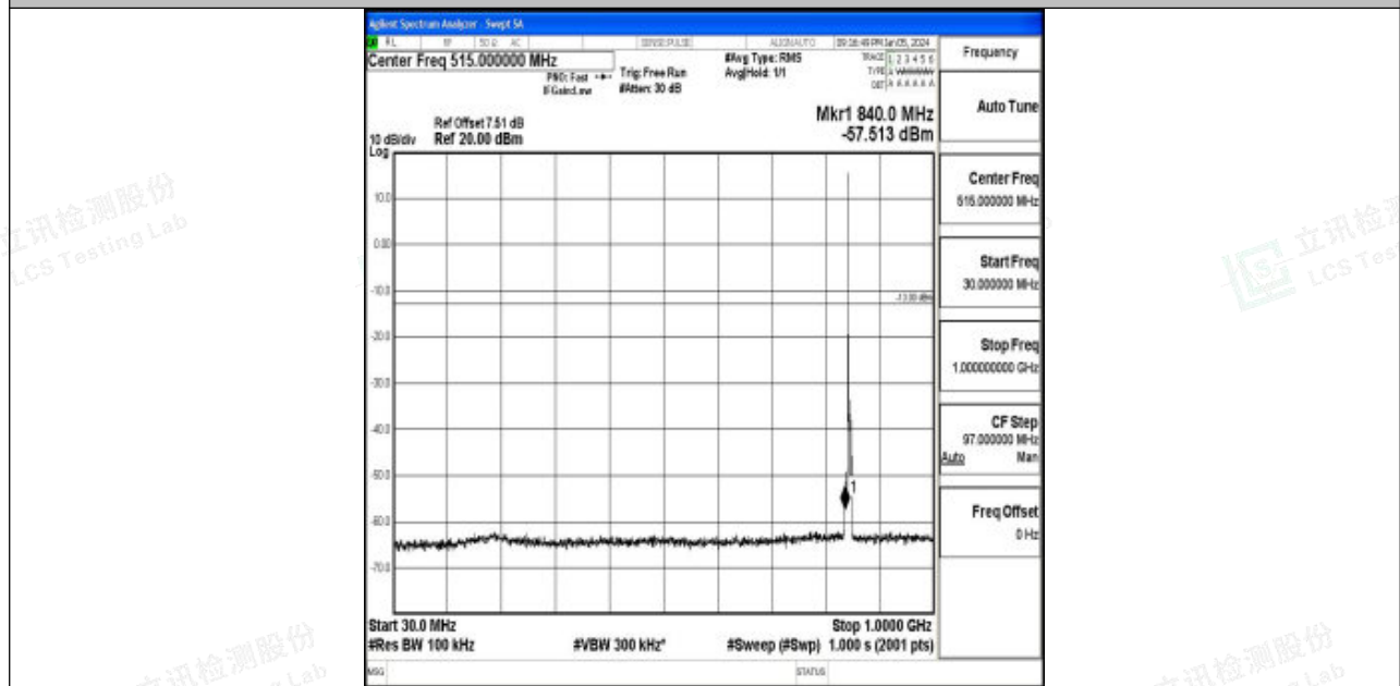
Band5_3MHz_16QAM_20635_1RB#0_30~1000_30~1000
