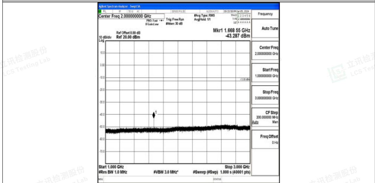
Band5_5MHz_QPSK_20525_1RB#0_1000~3000_1000~3000
