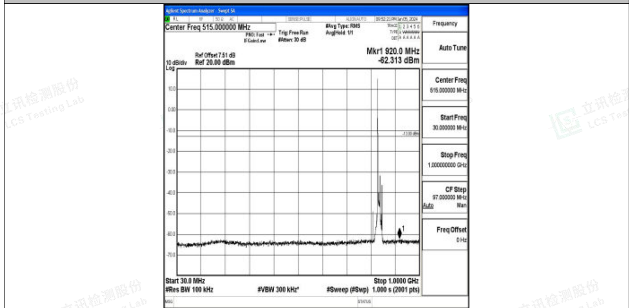
Band5_10MHz_16QAM_20525_1RB#0_30~1000_30~1000
