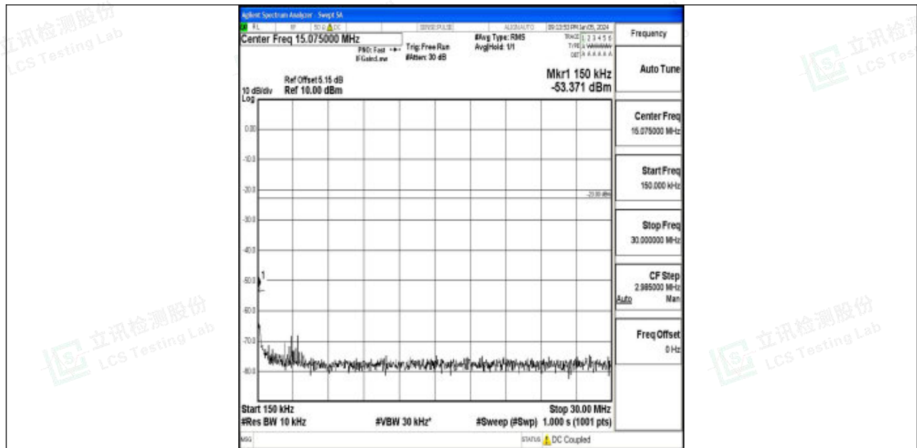
Band5_3MHz_16QAM_20415_1RB#0_0.15~30_0.15~30
