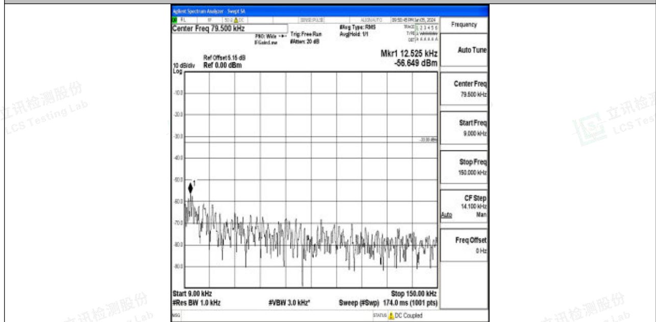
Band5_10MHz_16QAM_20450_1RB#0_0.009~0.15_0.009~0.15
