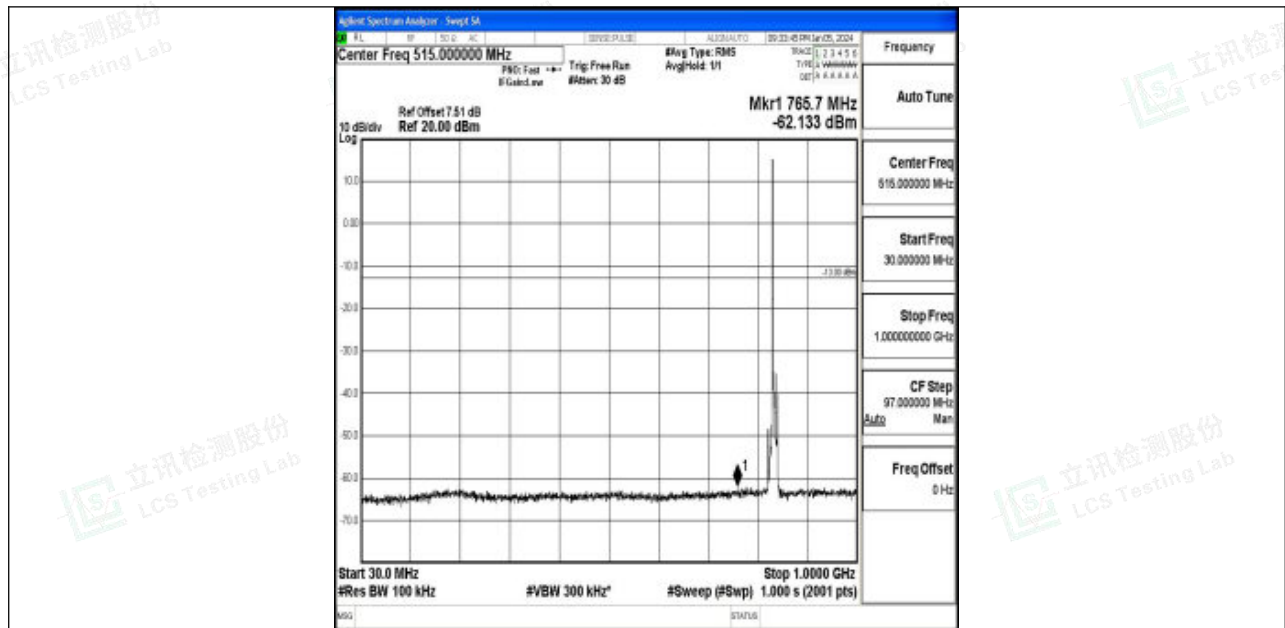
Band5_5MHz_QPSK_20525_1RB#0_30~1000_30~1000
