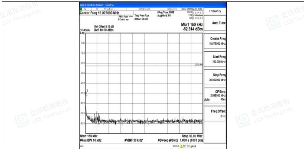
Band5_5MHz_16QAM_20525_1RB#0_0.15~30_0.15~30
