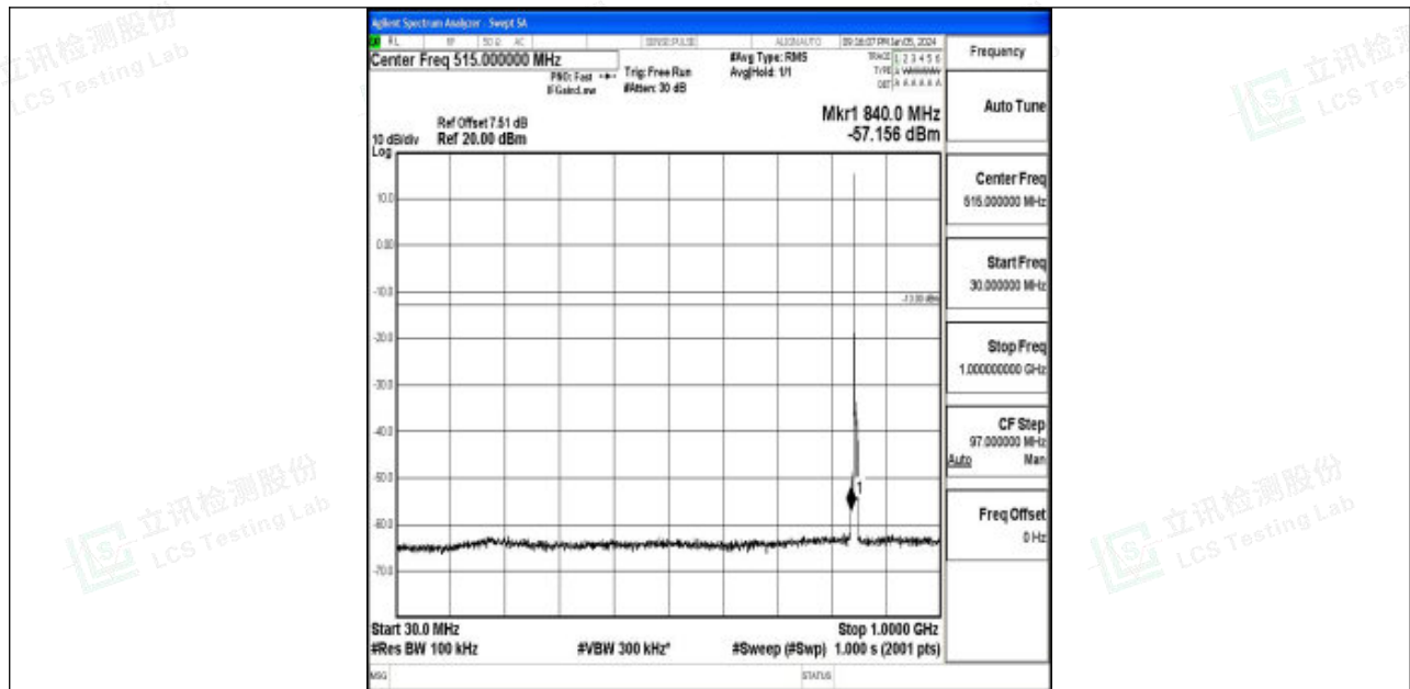
Band5_3MHz_QPSK_20635_1RB#0_30~1000_30~1000
