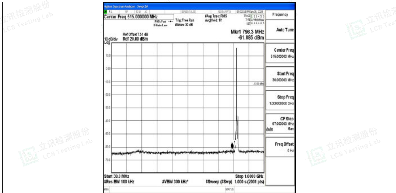
Band5_5MHz_QPSK_20425_1RB#0_30~1000_30~1000
