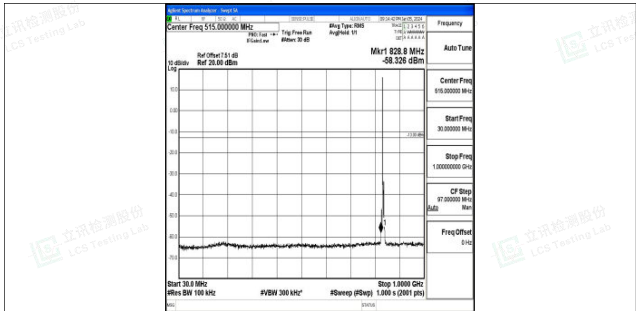
Band5_3MHz_QPSK_20525_1RB#0_30~1000_30~1000
