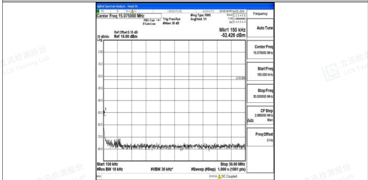
Band5_10MHz_QPSK_20450_1RB#0_0.15~30_0.15~30
