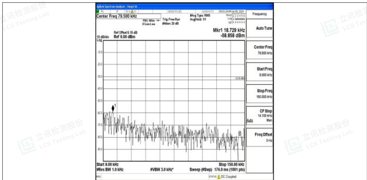
Band5_10MHz_QPSK_20525_1RB#0_0.009~0.15_0.009~0.15
