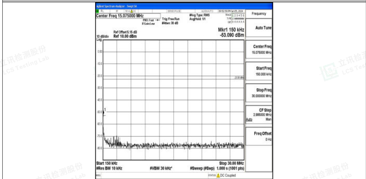
Band5_10MHz_QPSK_20600_1RB#0_0.15~30_0.15~30
