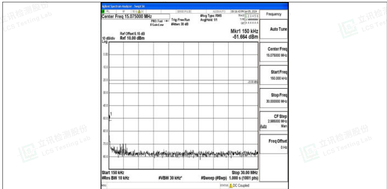
Band5_3MHz_16QAM_20635_1RB#0_0.15~30_0.15~30
