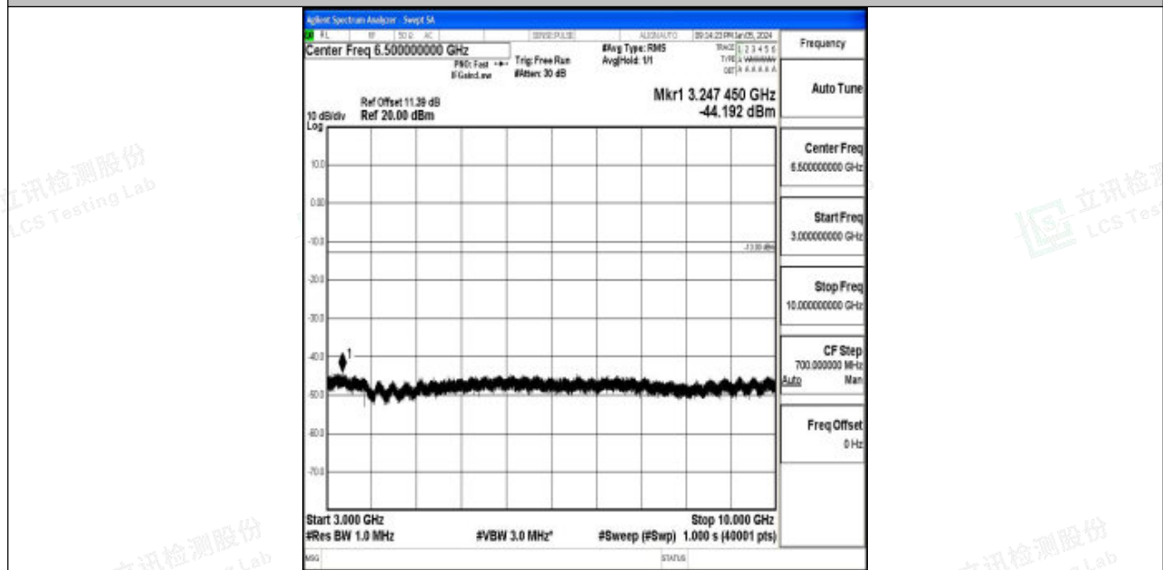
Band5_3MHz_16QAM_20415_1RB#0_3000~10000_3000~10000
