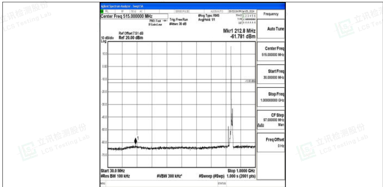
Band5_10MHz_QPSK_20600_1RB#0_30~1000_30~1000
