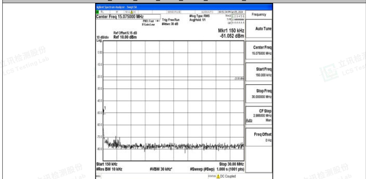
Band5_10MHz_QPSK_20525_1RB#0_0.15~30_0.15~30
