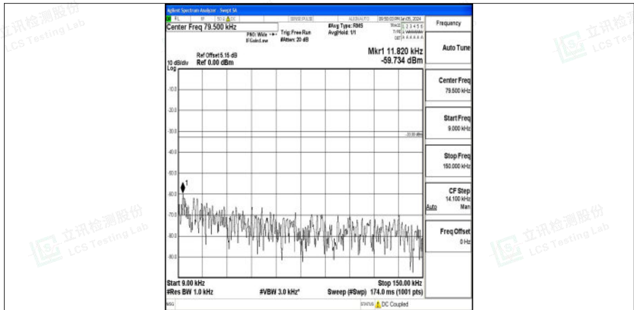
Band5_10MHz_QPSK_20450_1RB#0_0.009~0.15_0.009~0.15
