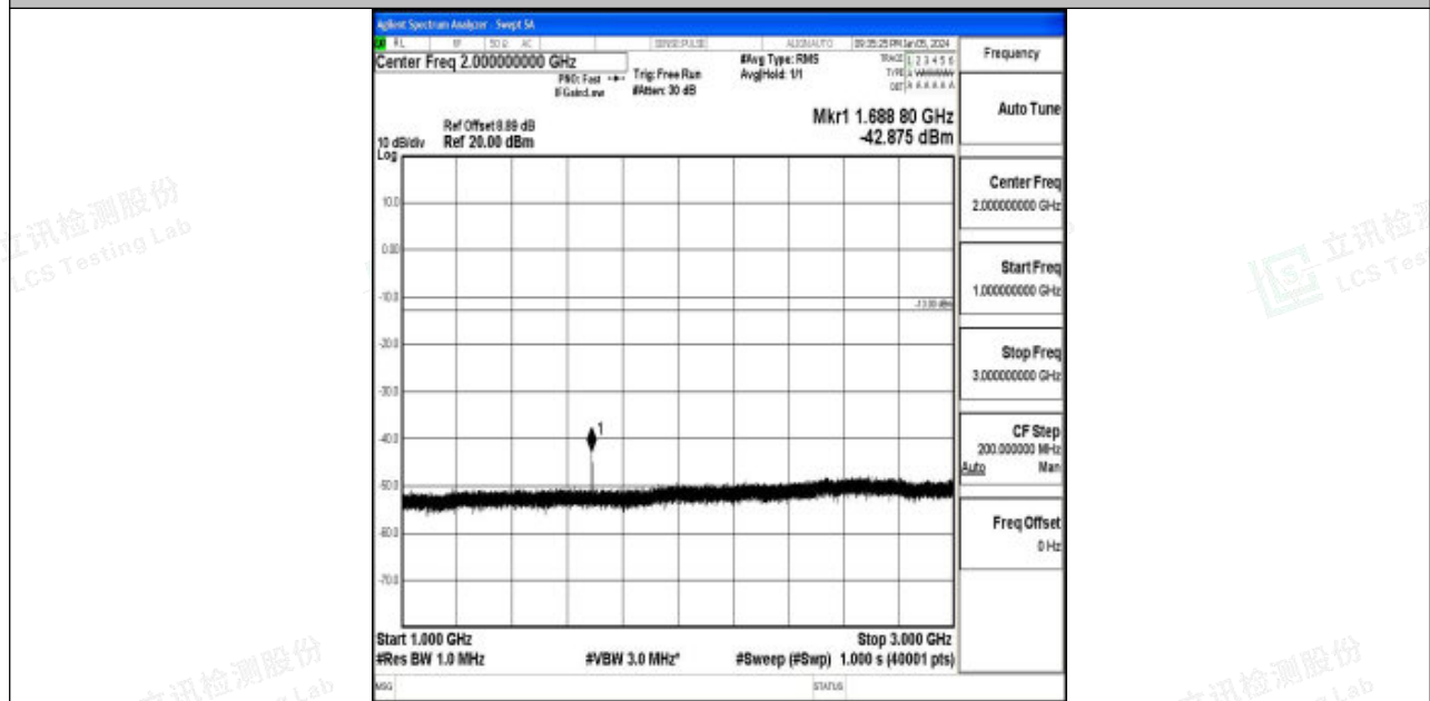
Band5_5MHz_QPSK_20625_1RB#0_1000~3000_1000~3000
