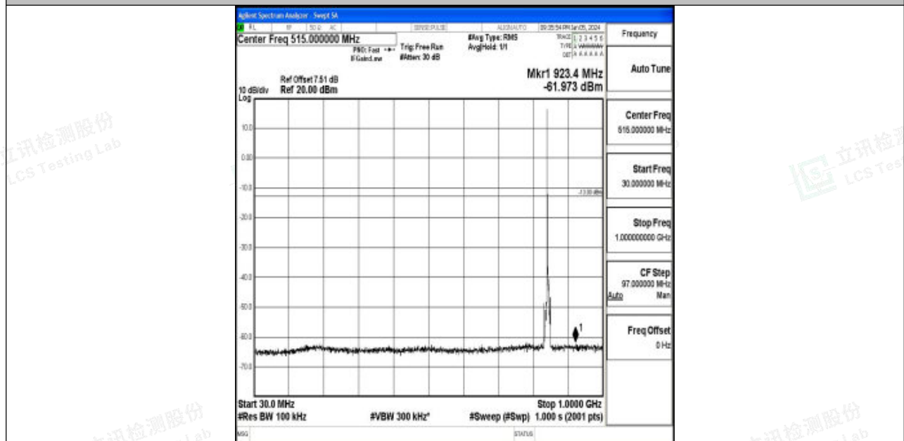
Band5_5MHz_16QAM_20625_1RB#0_30~1000_30~1000
