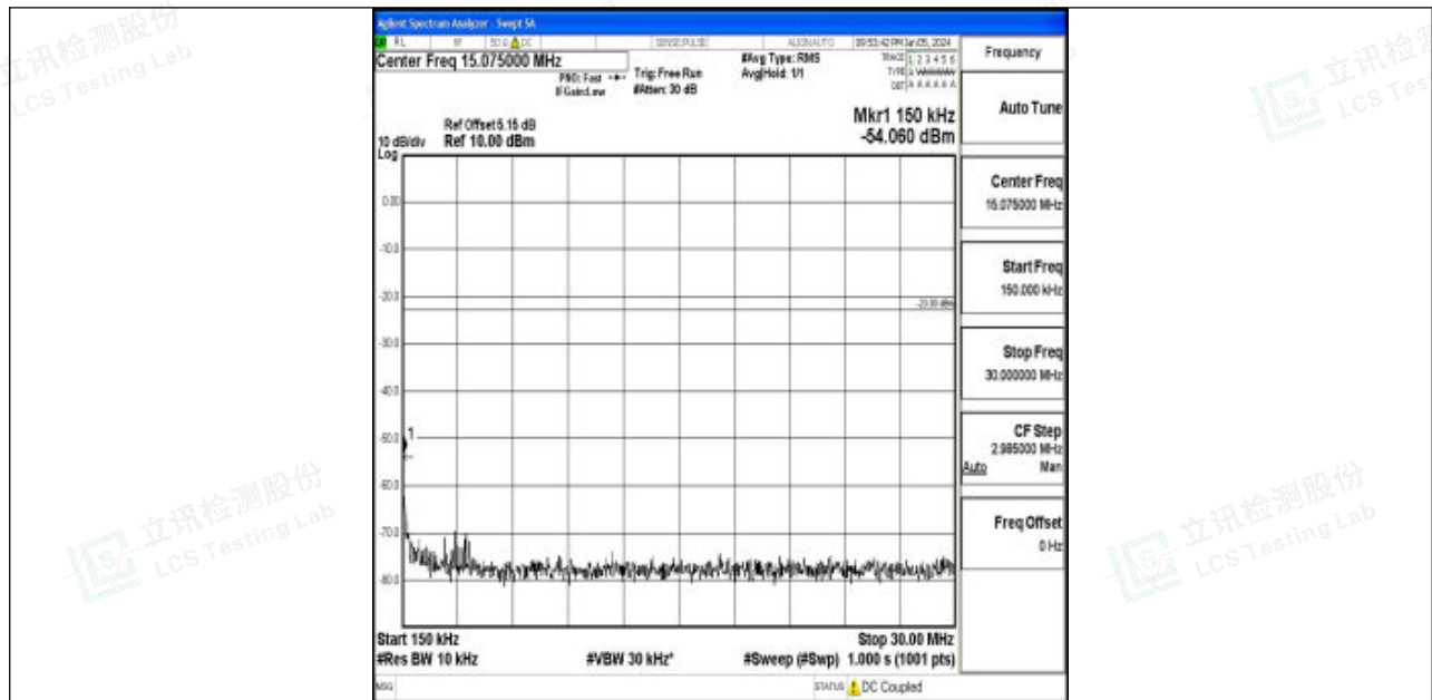
Band5_10MHz_16QAM_20600_1RB#0_0.15~30_0.15~30
