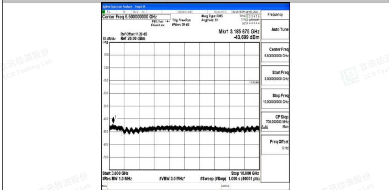
Band5_3MHz_16QAM_20525_1RB#0_3000~10000_3000~10000
