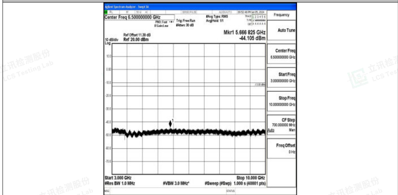
Band5_10MHz_16QAM_20525_1RB#0_3000~10000_3000~10000
