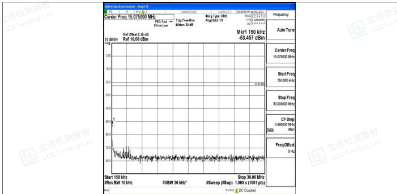
Band5_10MHz_16QAM_20450_1RB#0_0.15~30_0.15~30
