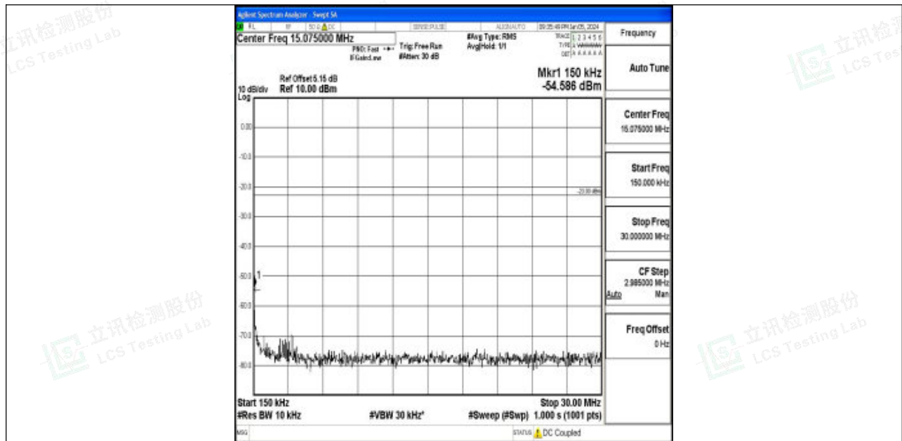
Band5_5MHz_16QAM_20625_1RB#0_0.15~30_0.15~30
