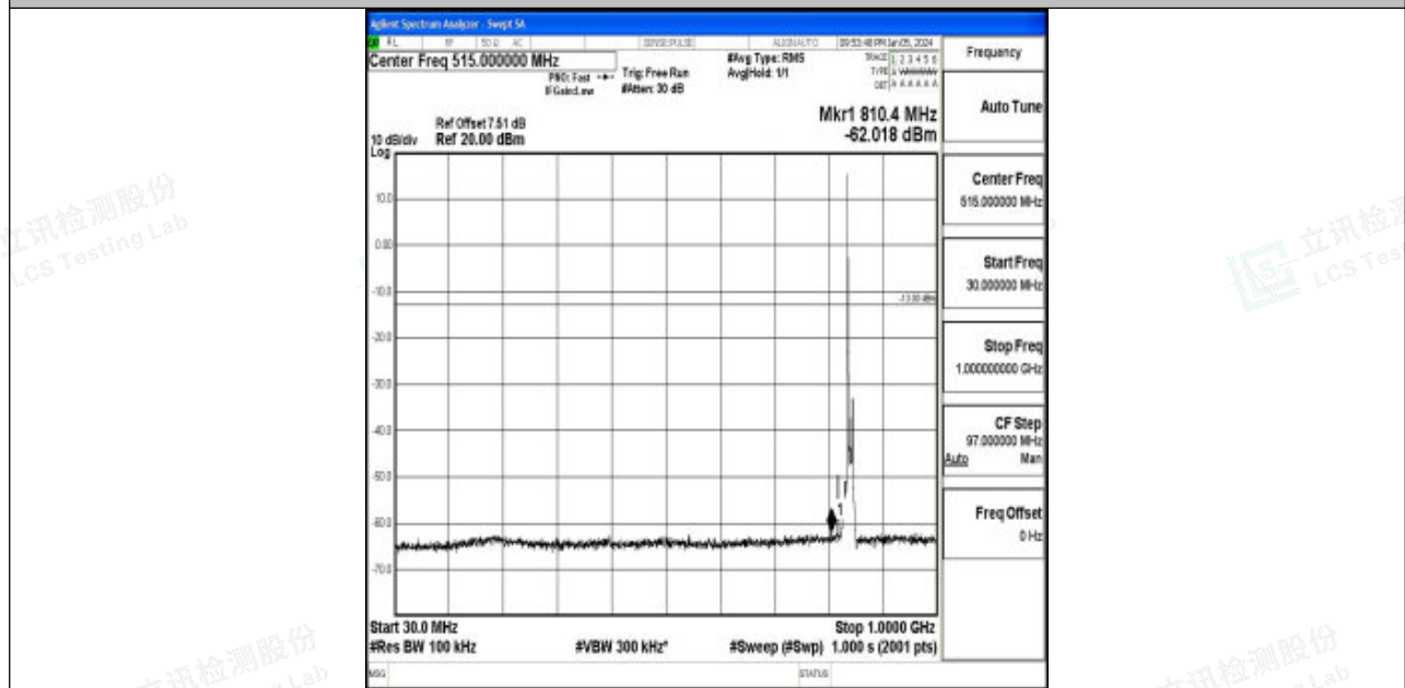
Band5_10MHz_16QAM_20600_1RB#0_30~1000_30~1000
