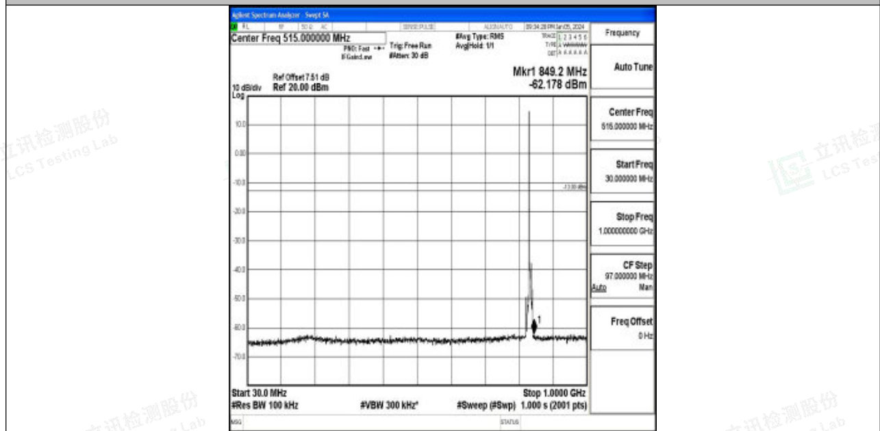
Band5_5MHz_16QAM_20525_1RB#0_30~1000_30~1000
