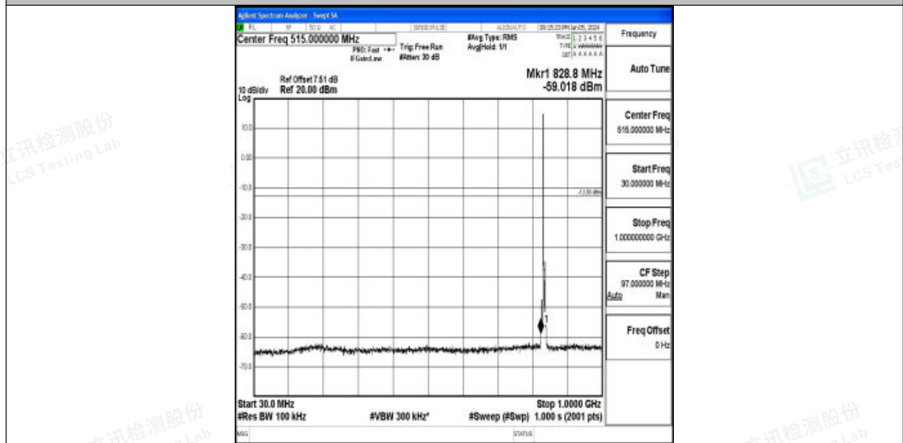
Band5_3MHz_16QAM_20525_1RB#0_30~1000_30~1000
