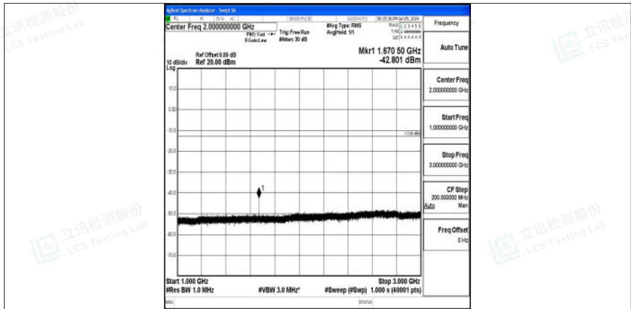
Band5_3MHz_16QAM_20525_1RB#0_1000~3000_1000~3000
