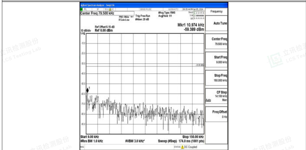
Band5_5MHz_16QAM_20625_1RB#0_0.009~0.15_0.009~0.15
