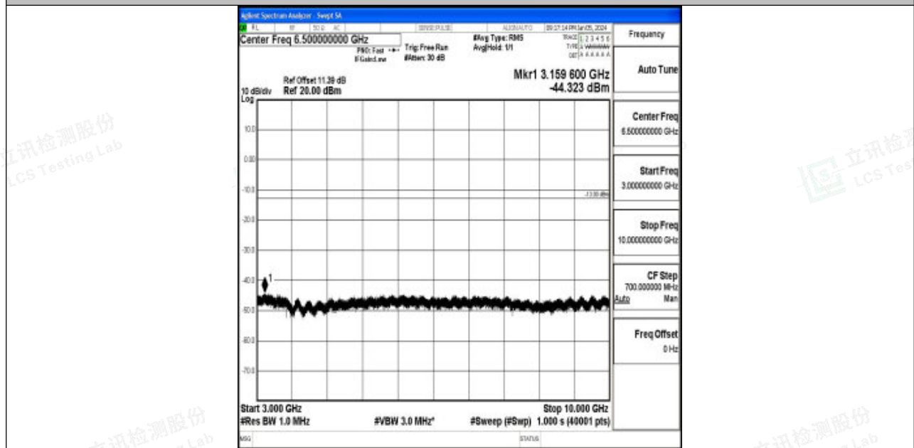
Band5_3MHz_16QAM_20635_1RB#0_3000~10000_3000~10000
