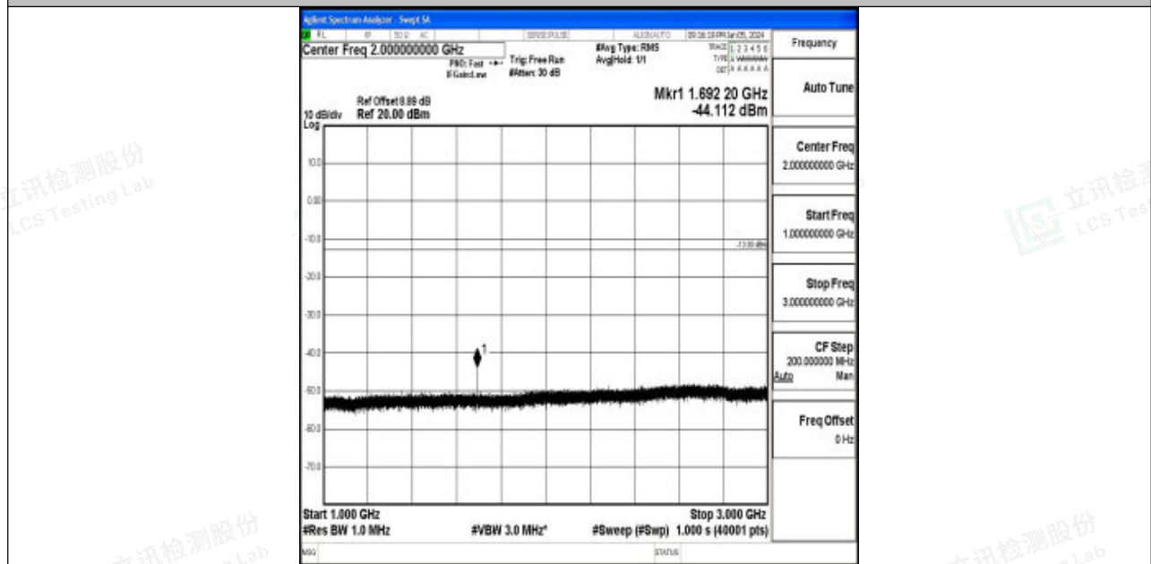
Band5_3MHz_QPSK_20635_1RB#0_1000~3000_1000~3000
