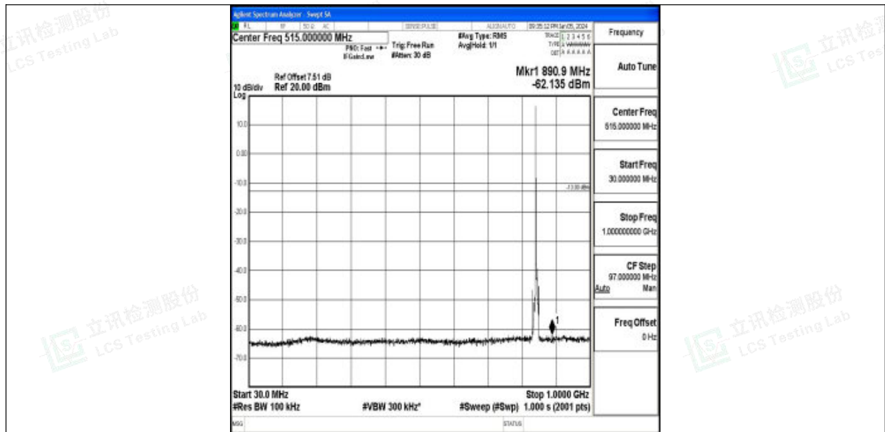
Band5_5MHz_QPSK_20625_1RB#0_30~1000_30~1000
