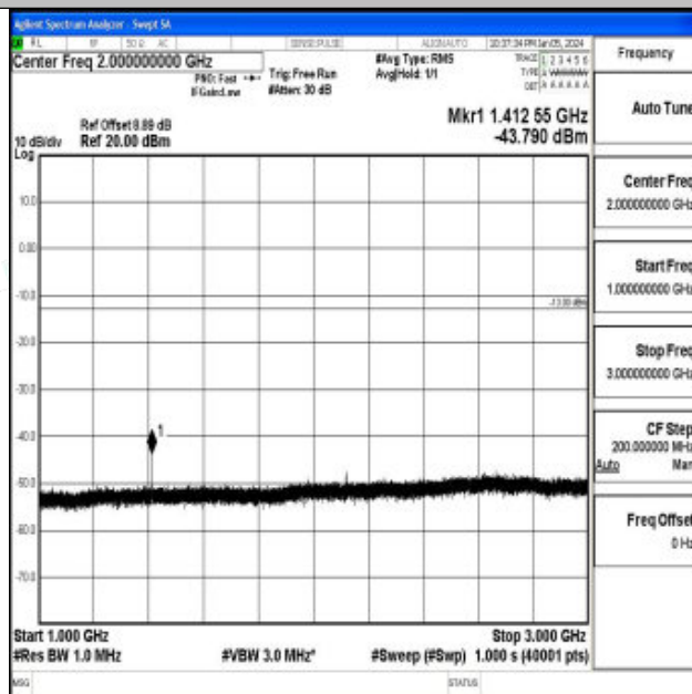
Band12_3MHz_16QAM_23095_1RB#0_1000~3000_1000~3000
