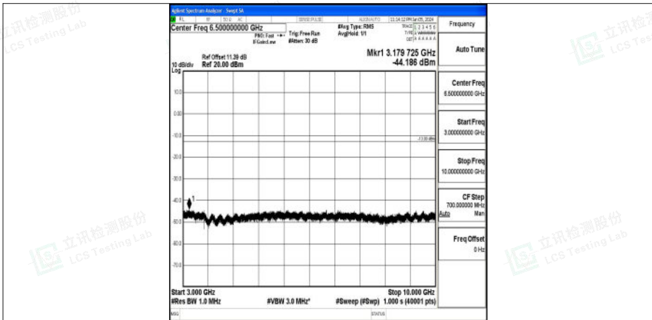
Band12_10MHz_16QAM_23060_1RB#0_3000~10000_3000~10000
