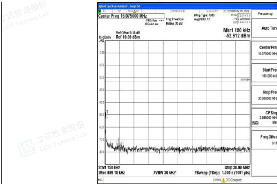
Band12_10MHz_QPSK_23130_1RB#0_0.15~30_0.15~30
