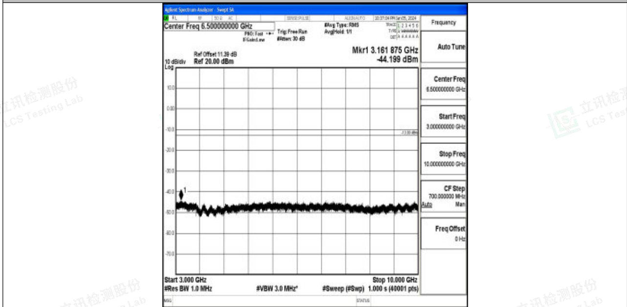
Band12_3MHz_QPSK_23095_1RB#0_3000~10000_3000~10000
