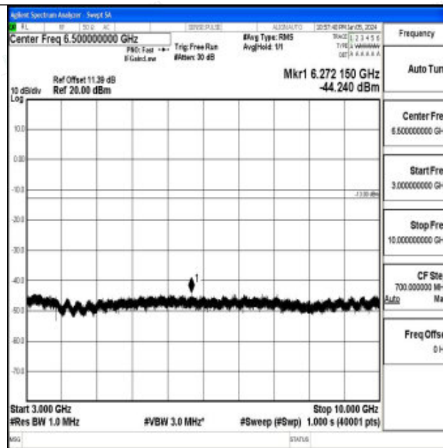
Band12_5MHz_16QAM_23095_1RB#0_3000~10000_3000~10000
