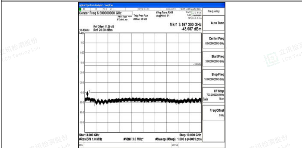
Band12_1.4MHz_QPSK_23173_1RB#0_3000~10000_3000~10000
