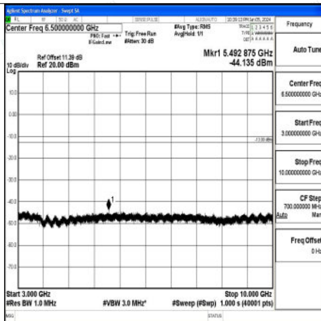
Band12_3MHz_16QAM_23165_1RB#0_3000~10000_3000~10000
