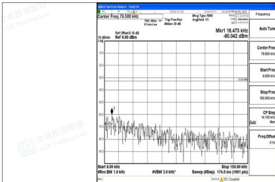
Band12_10MHz_16QAM_23060_1RB#0_0.009~0.15_0.009~0.15
