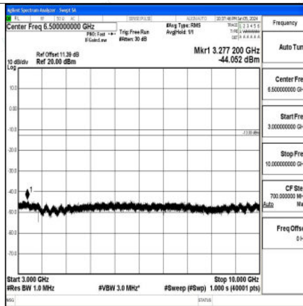
Band12_3MHz_16QAM_23095_1RB#0_3000~10000_3000~10000
