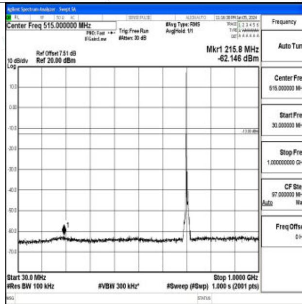
Band12_10MHz_16QAM_23130_1RB#0_30~1000_30~1000
