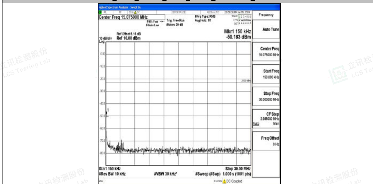
Band12_5MHz_16QAM_23155_1RB#0_0.15~30_0.15~30
