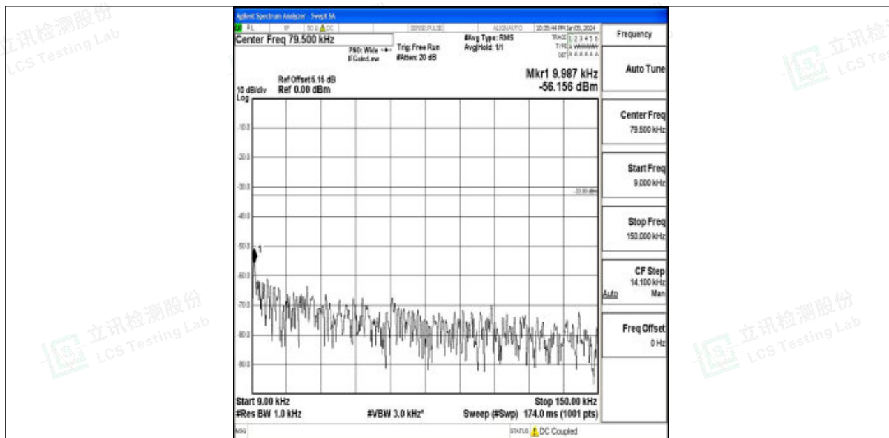
Band12_3MHz_16QAM_23025_1RB#0_0.009~0.15_0.009~0.15
