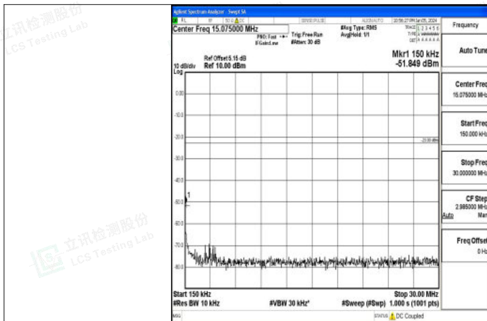
Band12_5MHz_QPSK_23095_1RB#0_0.15~30_0.15~30
