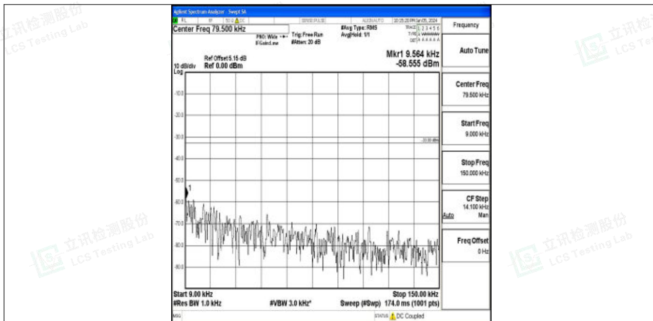
Band12_1.4MHz_16QAM_23173_1RB#0_0.009~0.15_0.009~0.15
