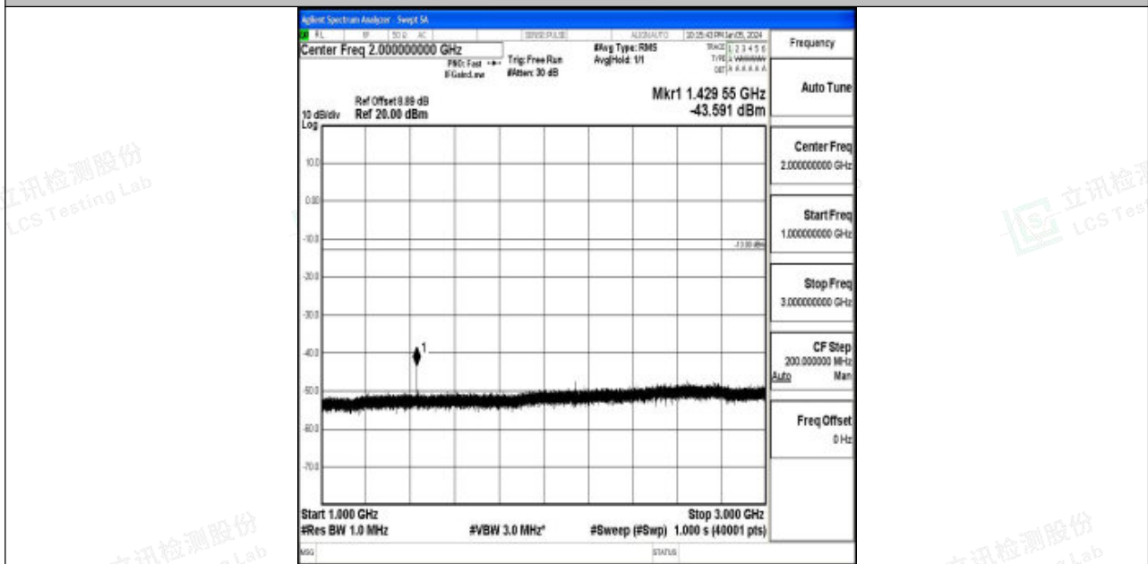
Band12_1.4MHz_16QAM_23173_1RB#0_1000~3000_1000~3000
