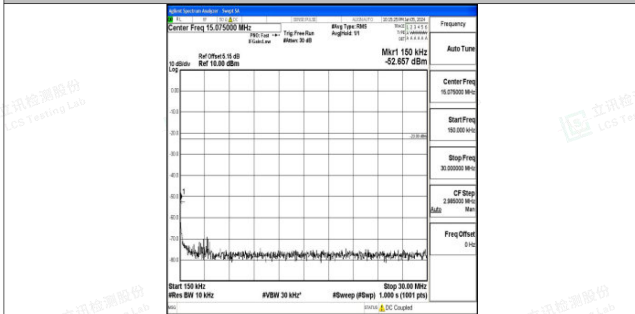
Band12_1.4MHz_16QAM_23173_1RB#0_0.15~30_0.15~30
