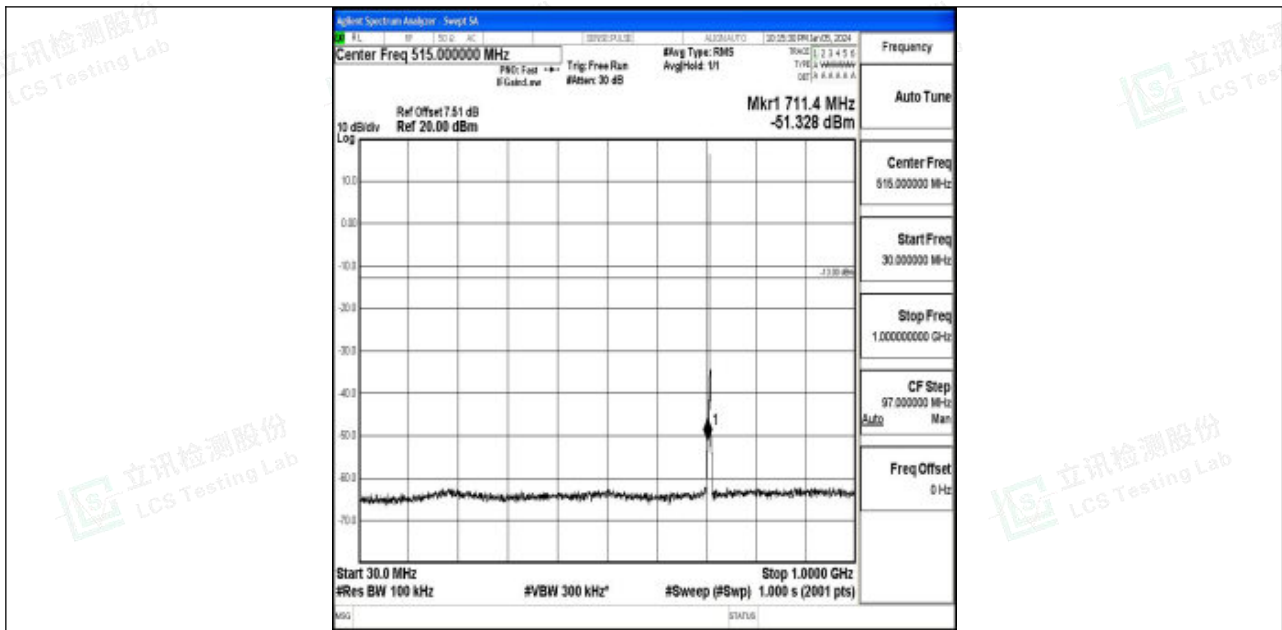
Band12_1.4MHz_16QAM_23173_1RB#0_30~1000_30~1000
