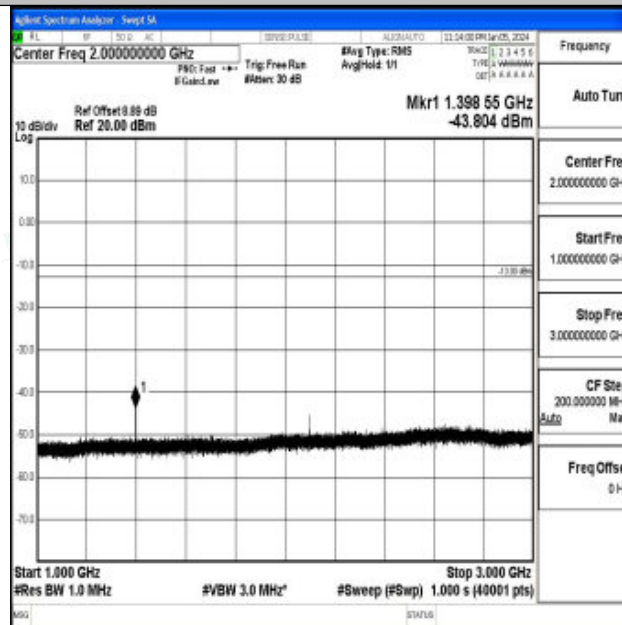
Band12_10MHz_16QAM_23060_1RB#0_1000~3000_1000~3000
