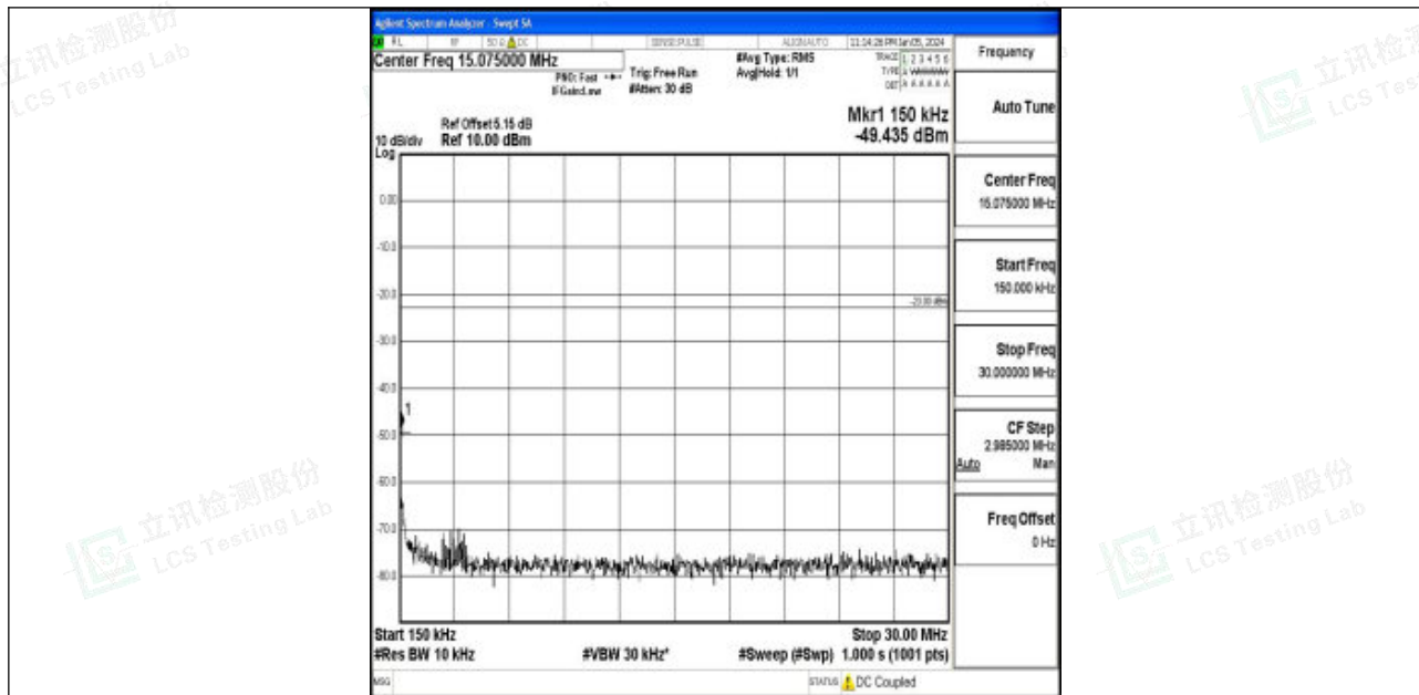
Band12_10MHz_QPSK_23095_1RB#0_0.15~30_0.15~30
