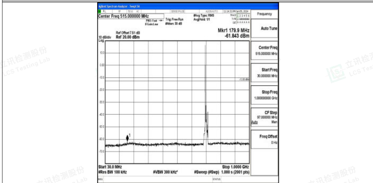
Band12_10MHz_QPSK_23095_1RB#0_30~1000_30~1000
