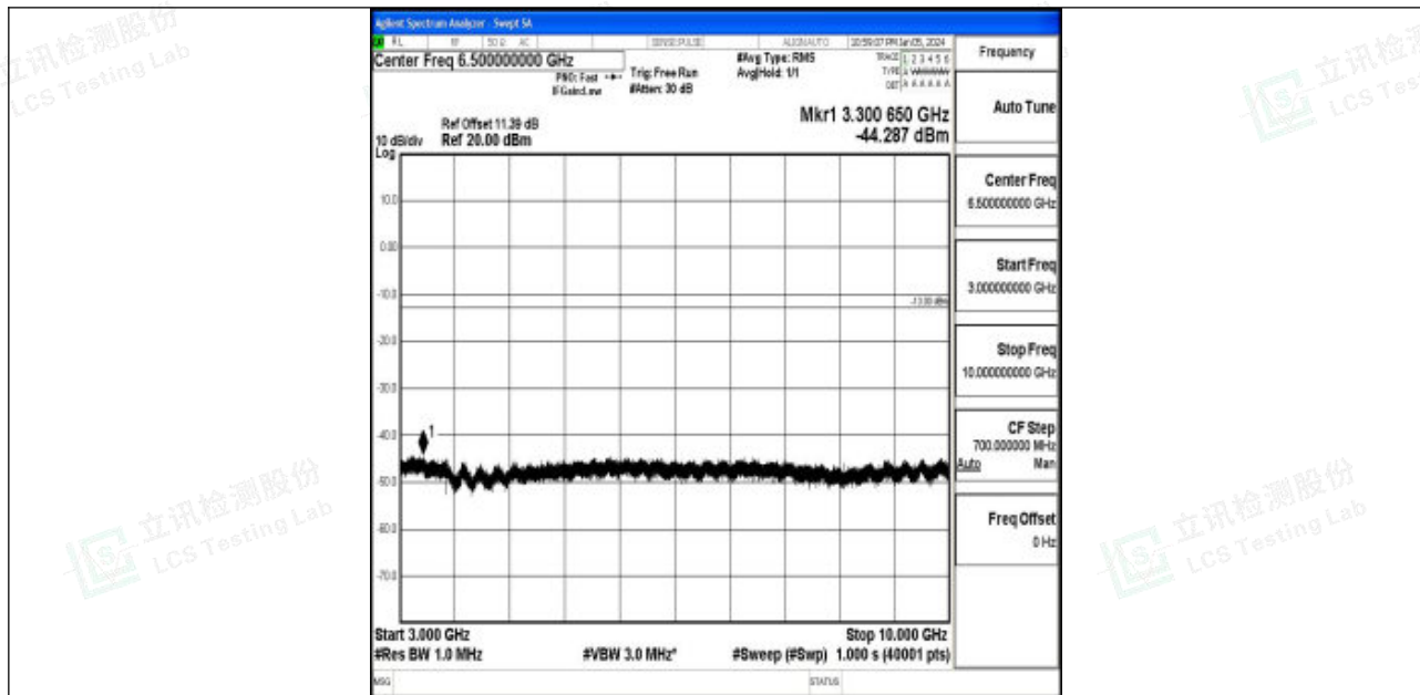
Band12_5MHz_16QAM_23155_1RB#0_3000~10000_3000~10000
