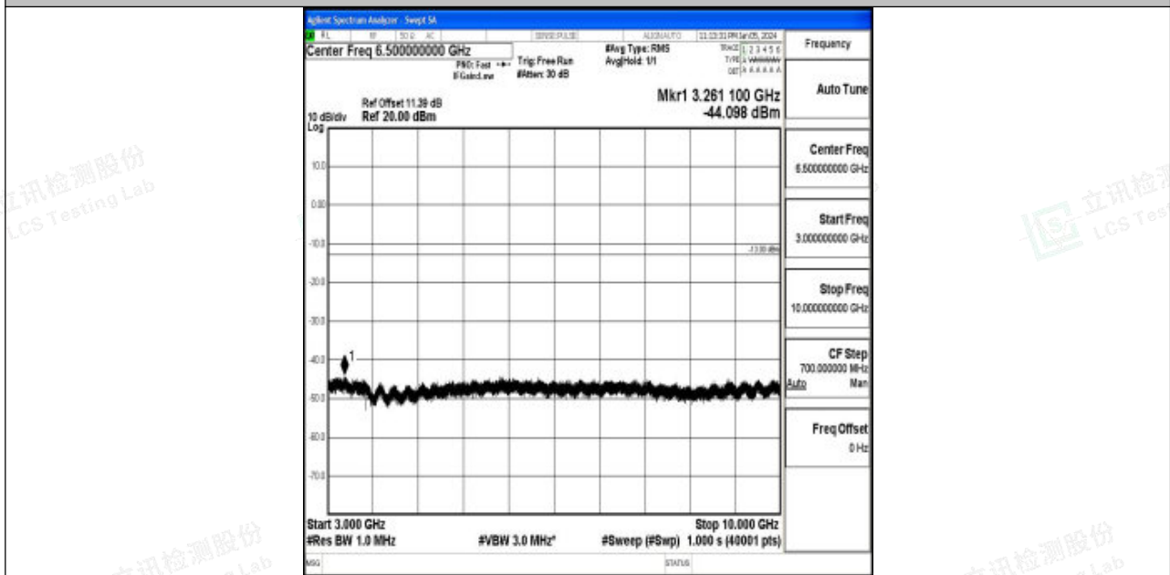
Band12_10MHz_QPSK_23060_1RB#0_3000~10000_3000~10000
