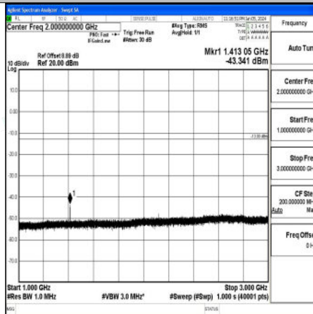
Band12_10MHz_16QAM_23130_1RB#0_1000~3000_1000~3000
