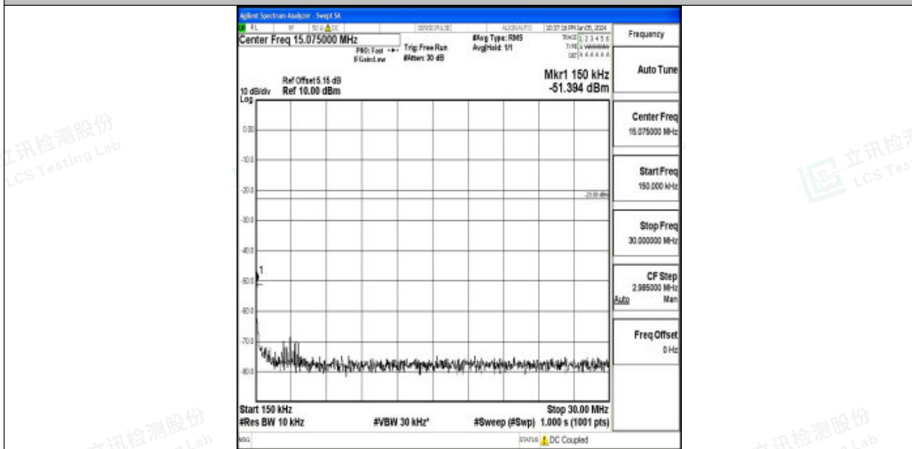
Band12_3MHz_16QAM_23095_1RB#0_0.15~30_0.15~30
