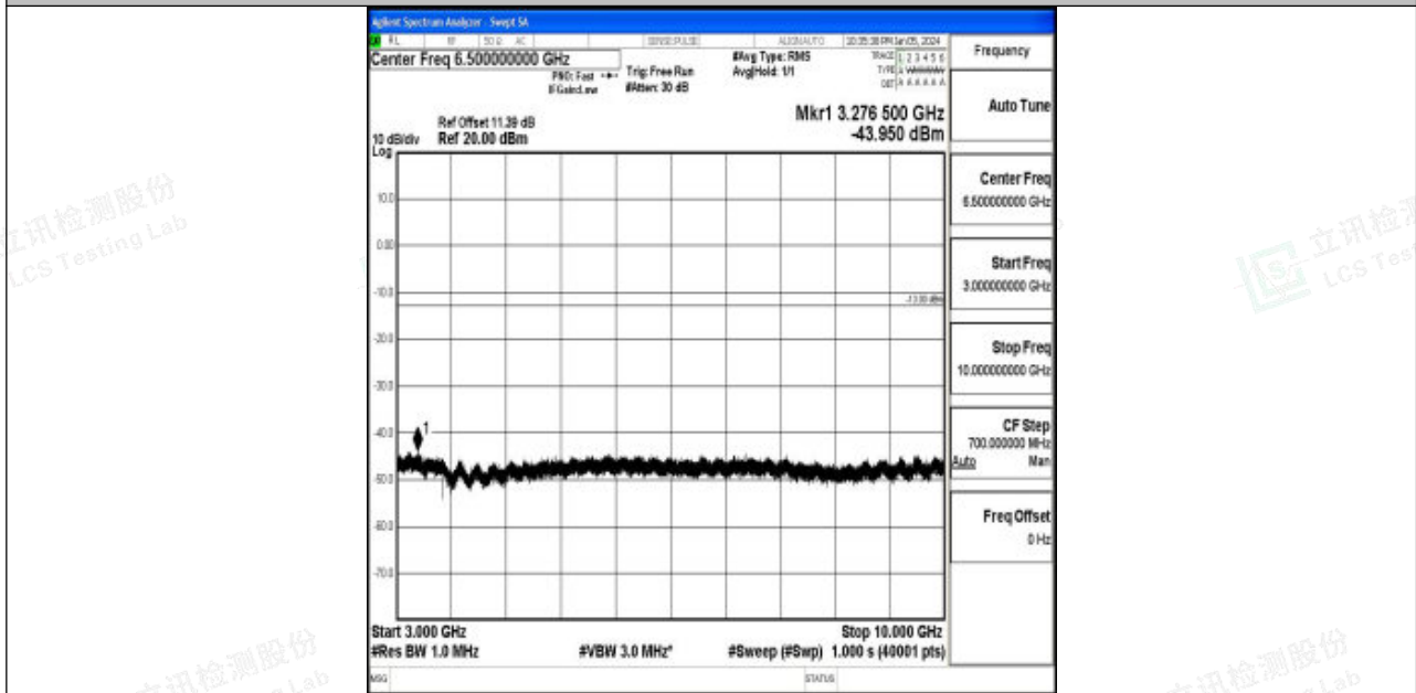
Band12_3MHz_QPSK_23025_1RB#0_3000~10000_3000~10000
