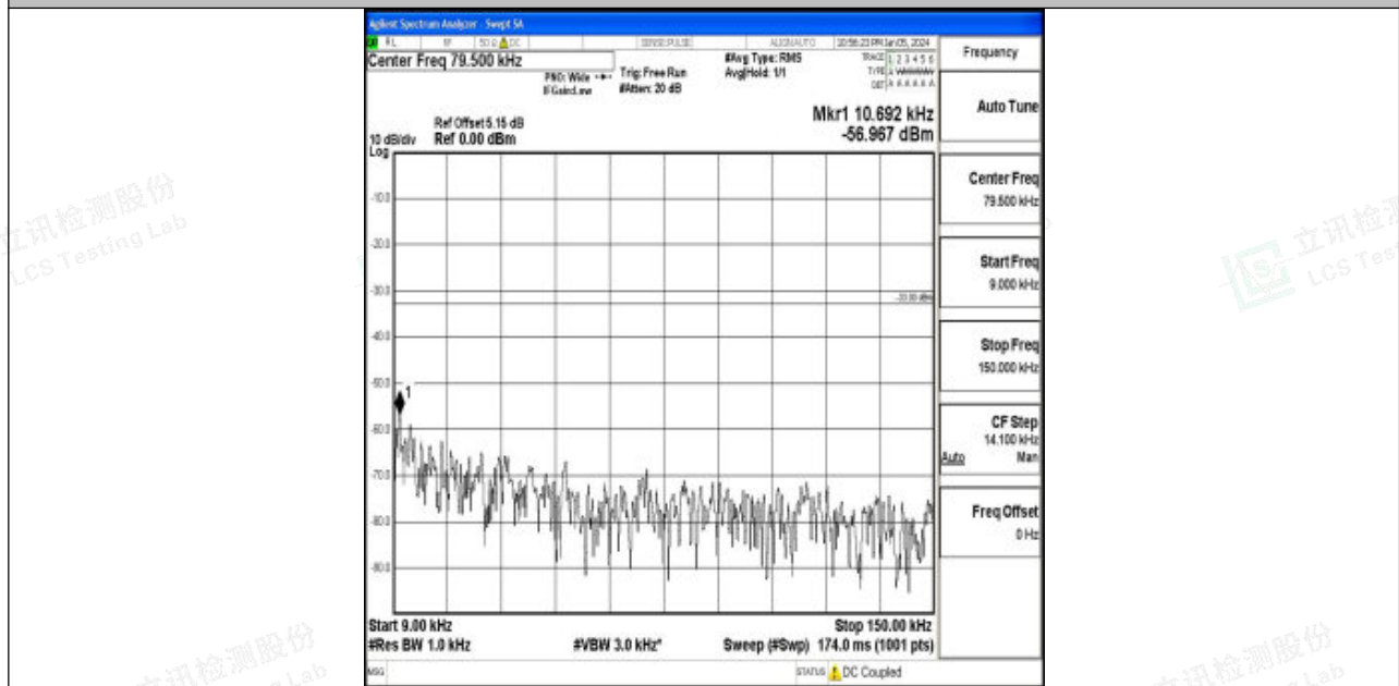
Band12_5MHz_QPSK_23095_1RB#0_0.009~0.15_0.009~0.15
