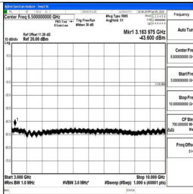
Band12_3MHz_16QAM_23025_1RB#0_3000~10000_3000~10000
