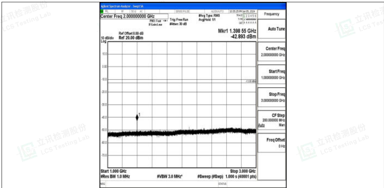
Band12_3MHz_QPSK_23025_1RB#0_1000~3000_1000~3000
