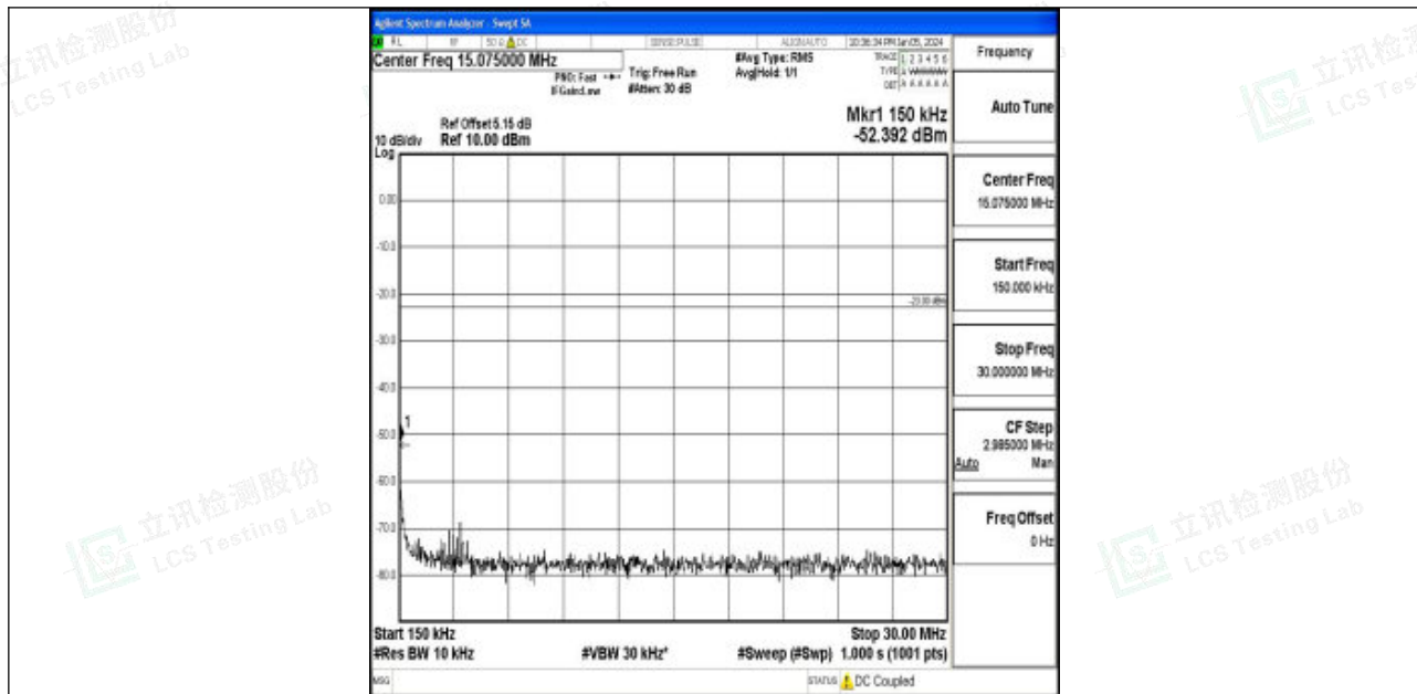
Band12_3MHz_QPSK_23095_1RB#0_0.15~30_0.15~30
