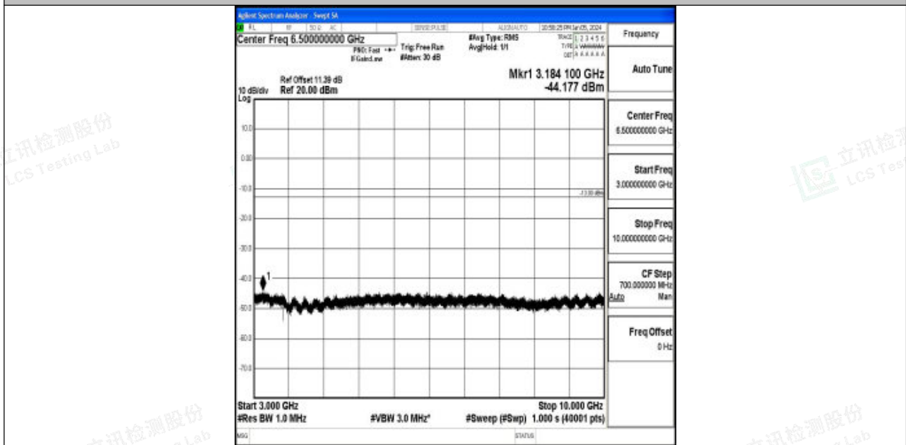
Band12_5MHz_QPSK_23155_1RB#0_3000~10000_3000~10000
