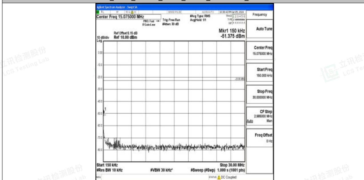
Band12_3MHz_16QAM_23165_1RB#0_0.15~30_0.15~30
