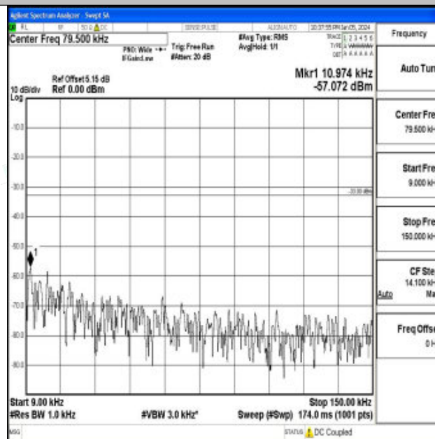
Band12_3MHz_QPSK_23165_1RB#0_0.009~0.15_0.009~0.15
