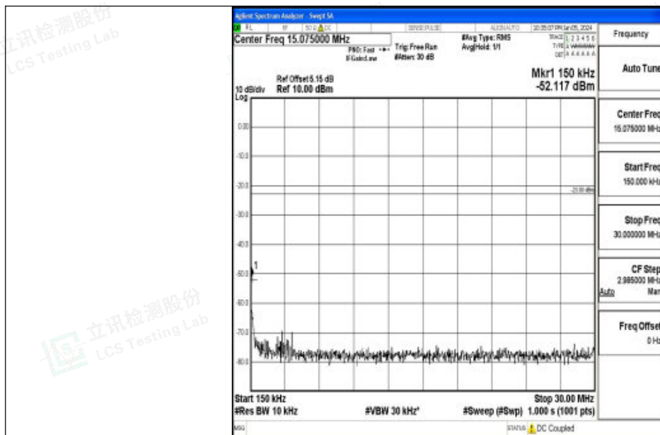
Band12_3MHz_QPSK_23025_1RB#0_0.15~30_0.15~30
