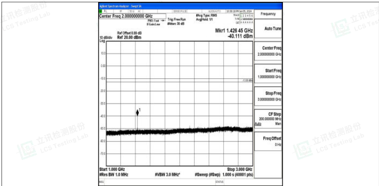
Band12_3MHz_QPSK_23165_1RB#0_1000~3000_1000~3000
