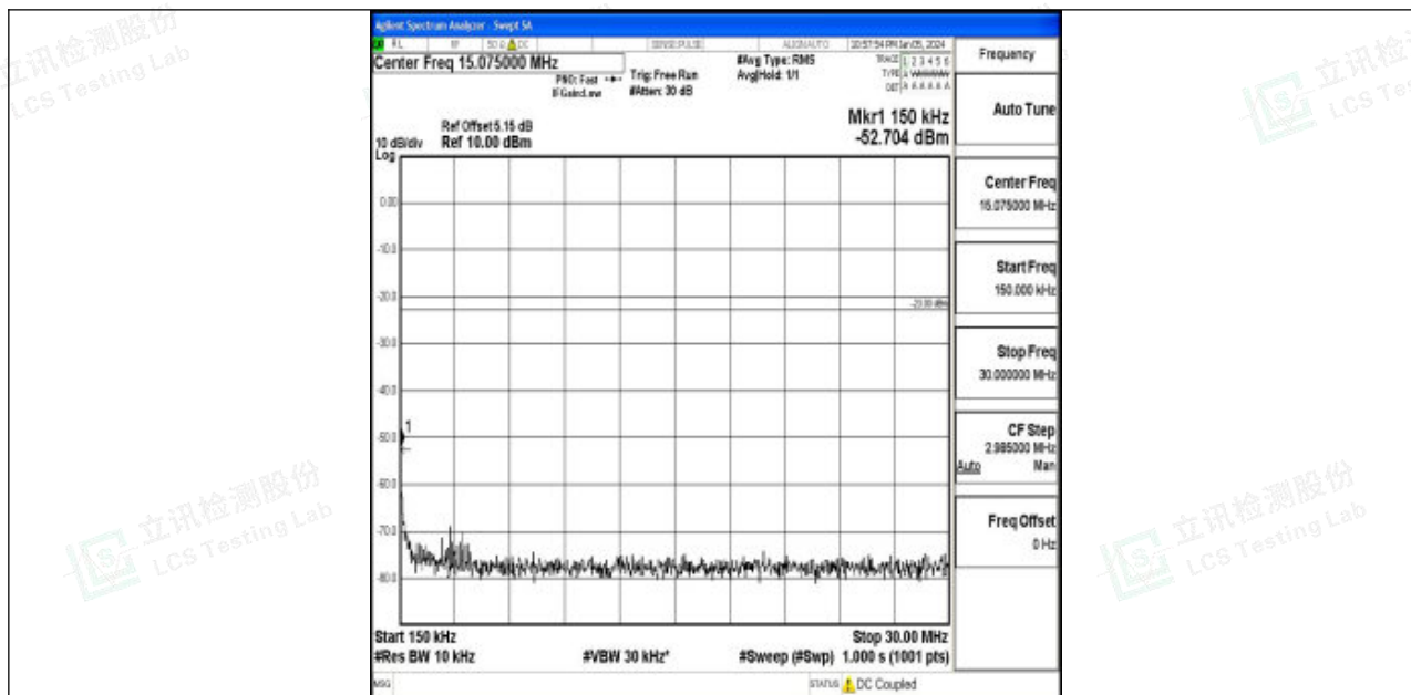
Band12_5MHz_QPSK_23155_1RB#0_0.15~30_0.15~30
