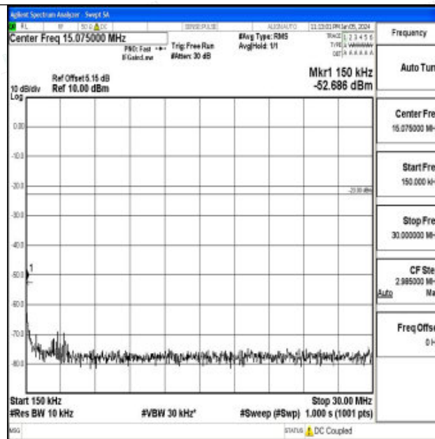
Band12_10MHz_QPSK_23060_1RB#0_0.15~30_0.15~30
