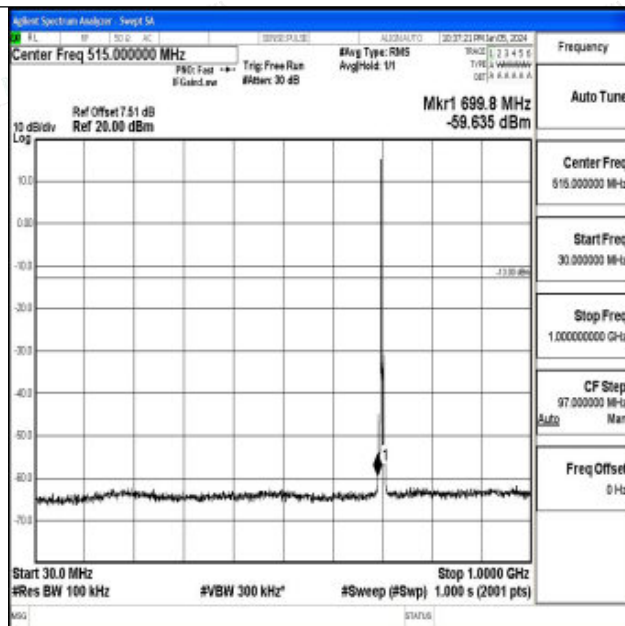
Band12_3MHz_16QAM_23095_1RB#0_30~1000_30~1000
