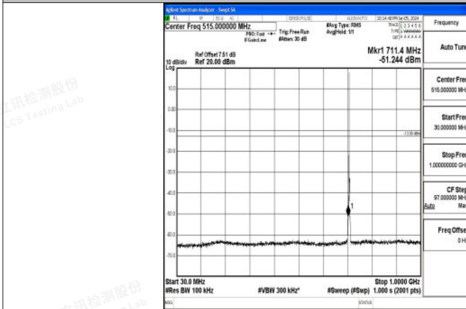
Band12_1.4MHz_QPSK_23173_1RB#0_30~1000_30~1000
