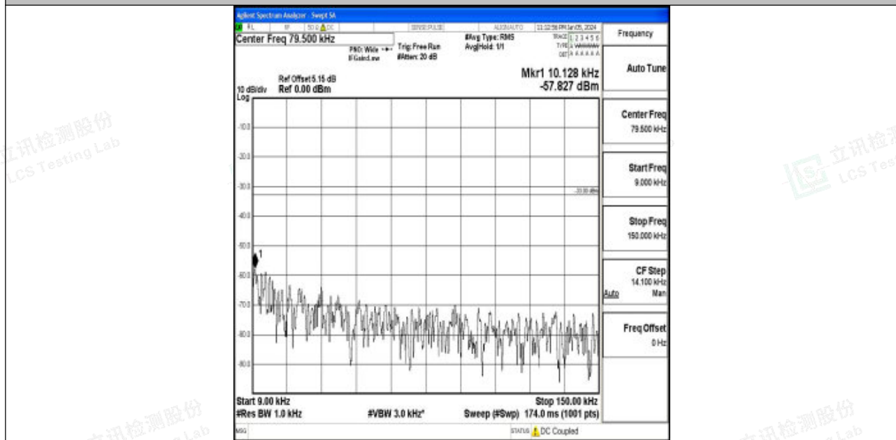
Band12_10MHz_QPSK_23060_1RB#0_0.009~0.15_0.009~0.15
