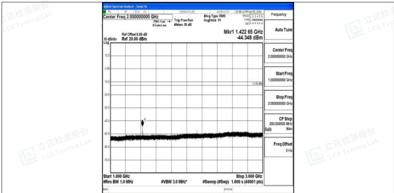
Band12_5MHz_QPSK_23155_1RB#0_1000~3000_1000~3000
