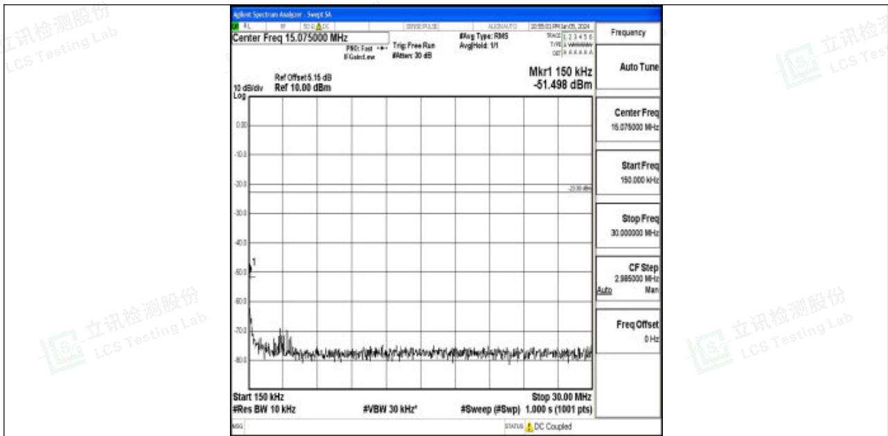
Band12_5MHz_QPSK_23035_1RB#0_0.15~30_0.15~30
