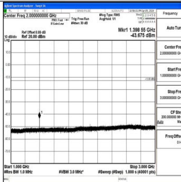
Band12_5MHz_16QAM_23035_1RB#0_1000~3000_1000~3000
