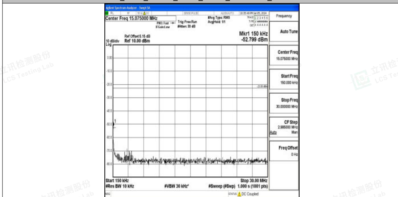
Band12_3MHz_16QAM_23025_1RB#0_0.15~30_0.15~30
