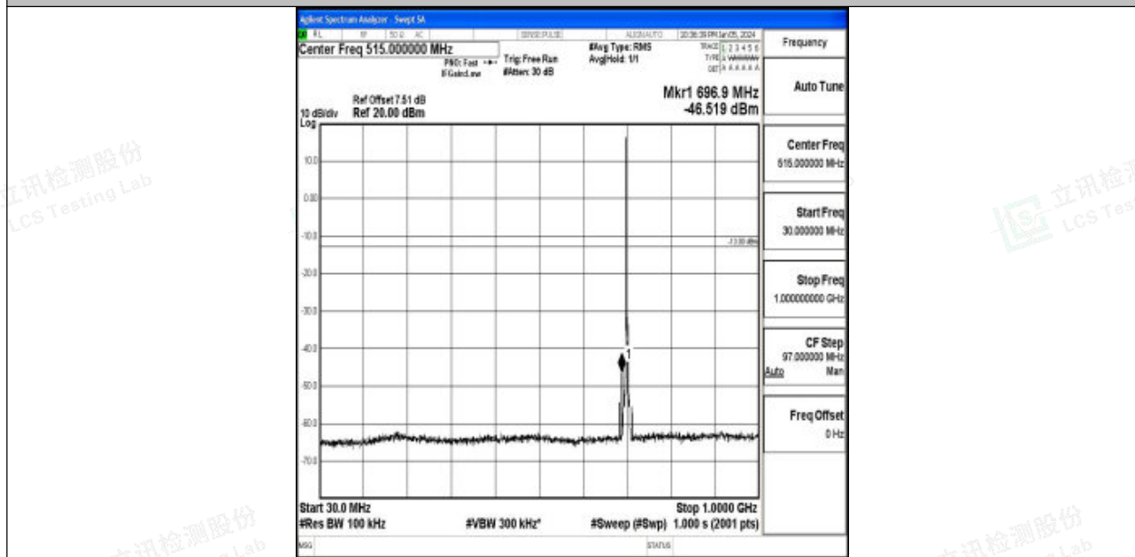
Band12_3MHz_QPSK_23095_1RB#0_30~1000_30~1000
