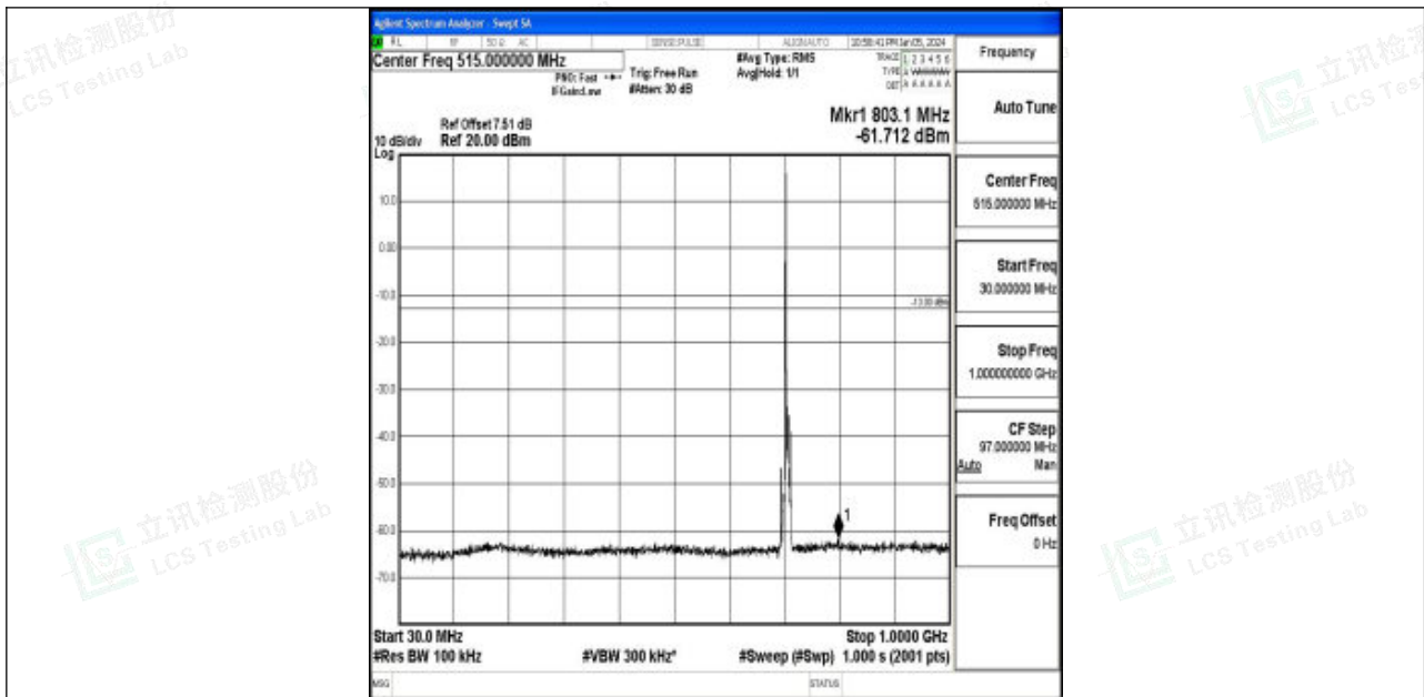
Band12_5MHz_16QAM_23155_1RB#0_30~1000_30~1000
