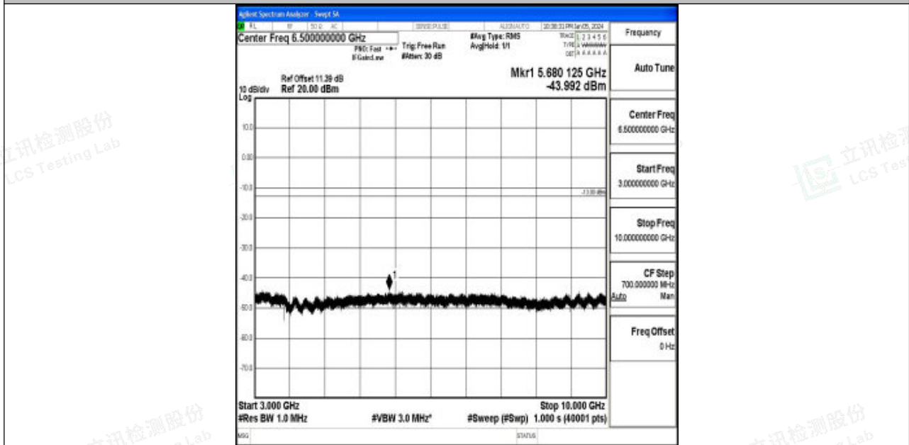
Band12_3MHz_QPSK_23165_1RB#0_3000~10000_3000~10000
