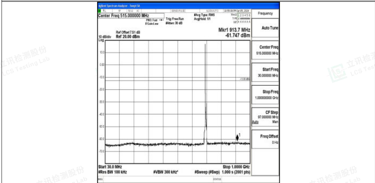
Band12_5MHz_QPSK_23035_1RB#0_30~1000_30~1000
