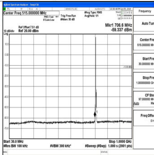
Band12_3MHz_16QAM_23165_1RB#0_30~1000_30~1000
