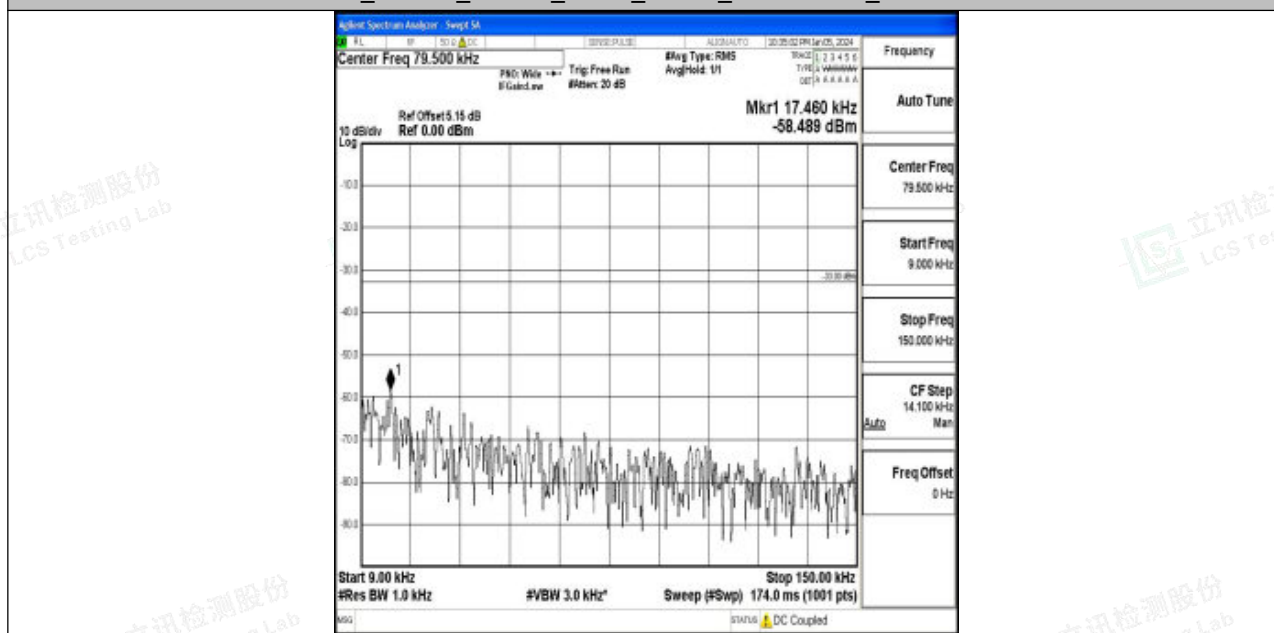
Band12_3MHz_QPSK_23025_1RB#0_0.009~0.15_0.009~0.15
