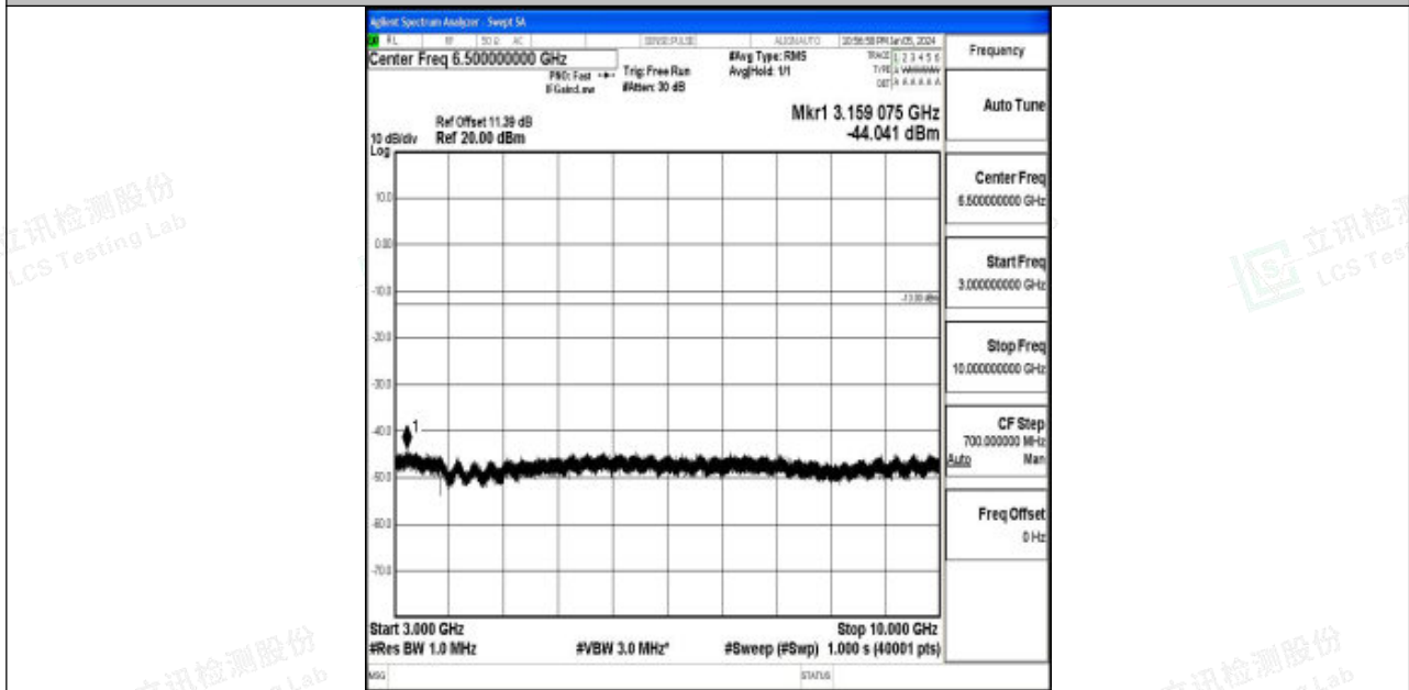
Band12_5MHz_QPSK_23095_1RB#0_3000~10000_3000~10000
