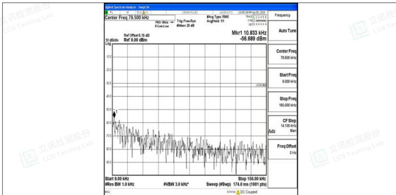
Band12_5MHz_16QAM_23035_1RB#0_0.009~0.15_0.009~0.15
