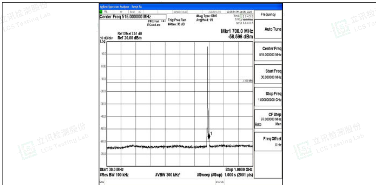
Band12_3MHz_16QAM_23025_1RB#0_30~1000_30~1000
