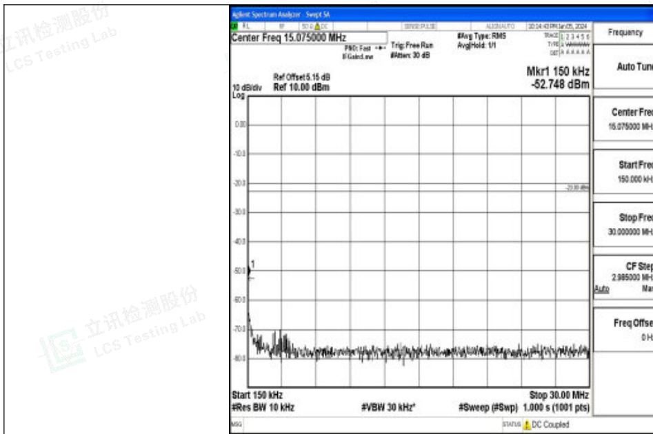
Band12_1.4MHz_QPSK_23173_1RB#0_0.15~30_0.15~30
