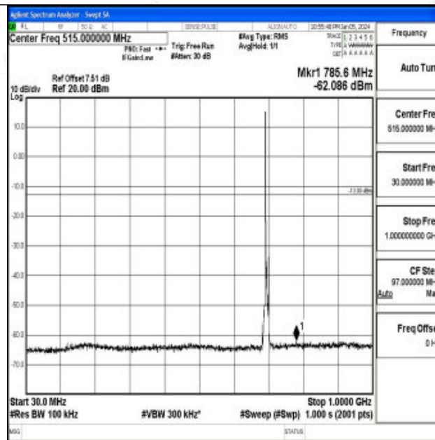
Band12_5MHz_16QAM_23035_1RB#0_30~1000_30~1000
