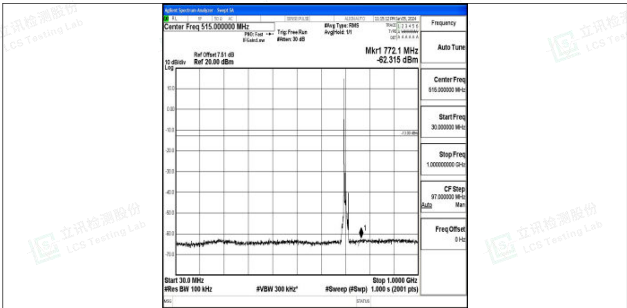
Band12_10MHz_16QAM_23095_1RB#0_30~1000_30~1000
