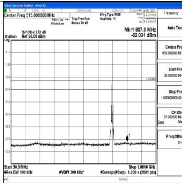
Band12_10MHz_16QAM_23060_1RB#0_30~1000_30~1000
