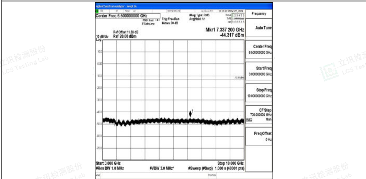
Band12_10MHz_QPSK_23130_1RB#0_3000~10000_3000~10000
