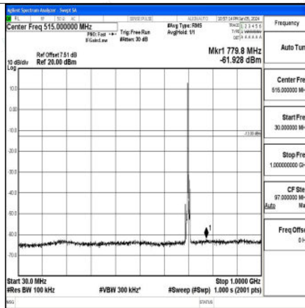
Band12_5MHz_16QAM_23095_1RB#0_30~1000_30~1000
