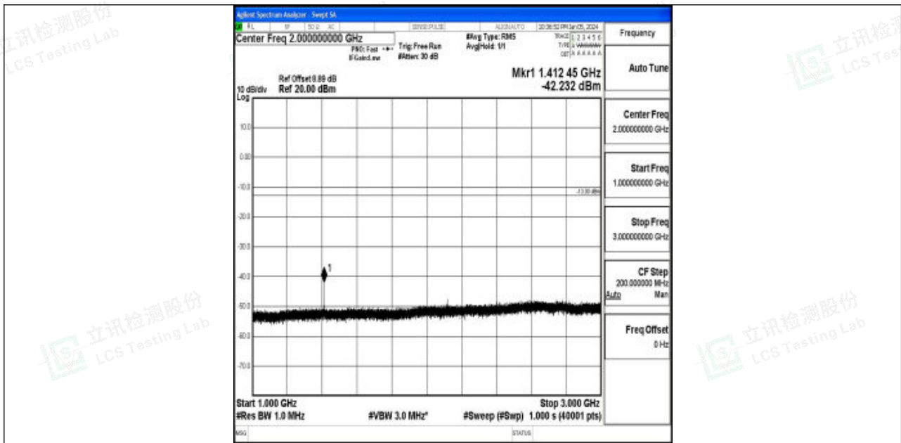
Band12_3MHz_QPSK_23095_1RB#0_1000~3000_1000~3000
