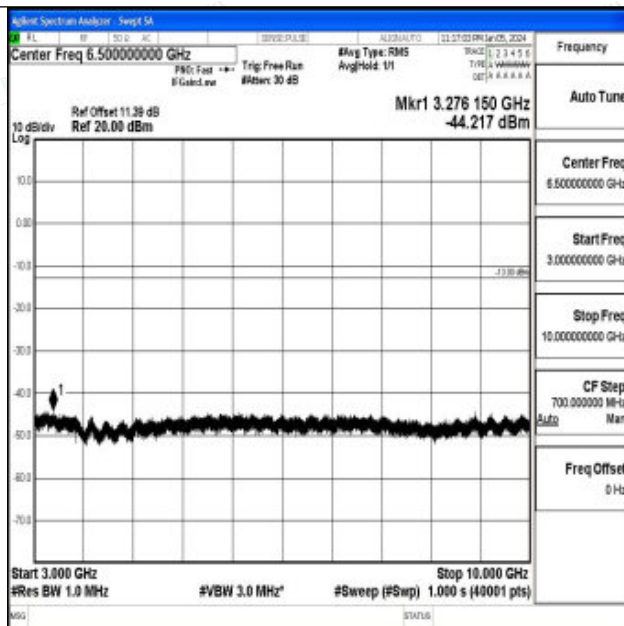
Band12_10MHz_16QAM_23130_1RB#0_3000~10000_3000~10000
