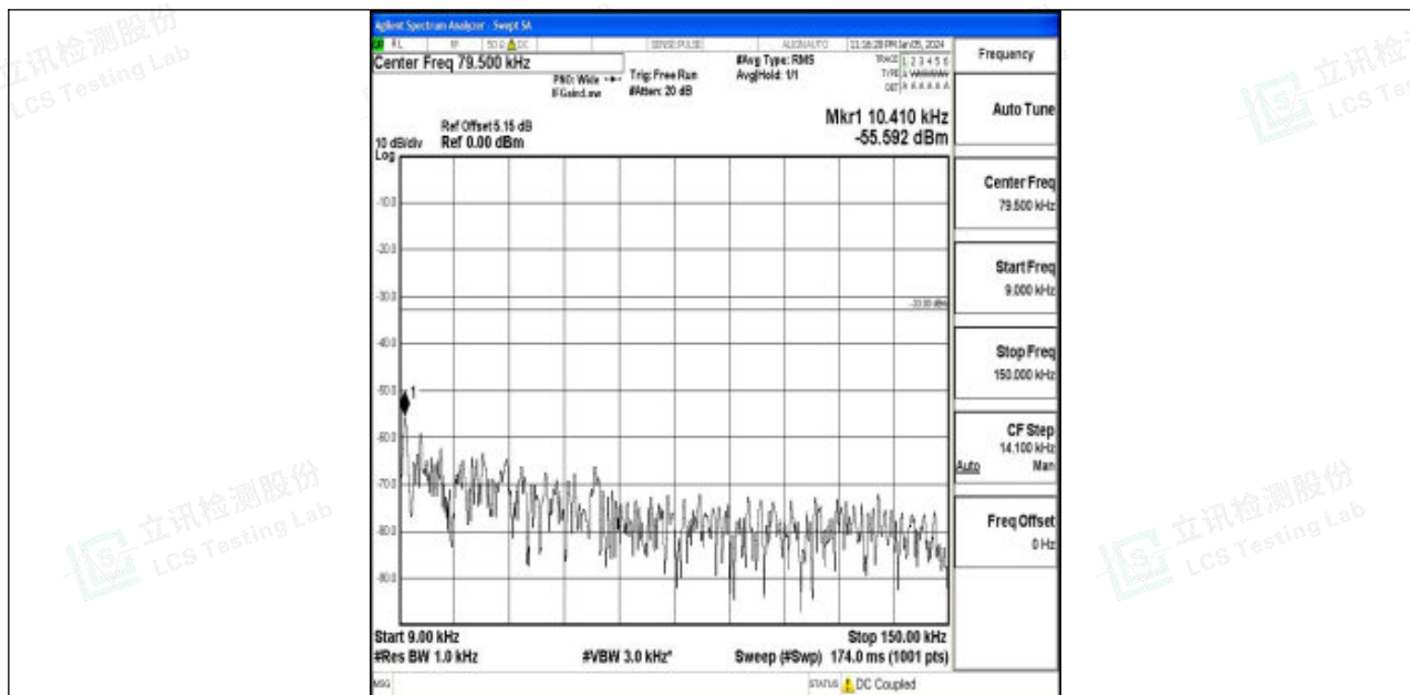
Band12_10MHz_16QAM_23130_1RB#0_0.009~0.15_0.009~0.15
