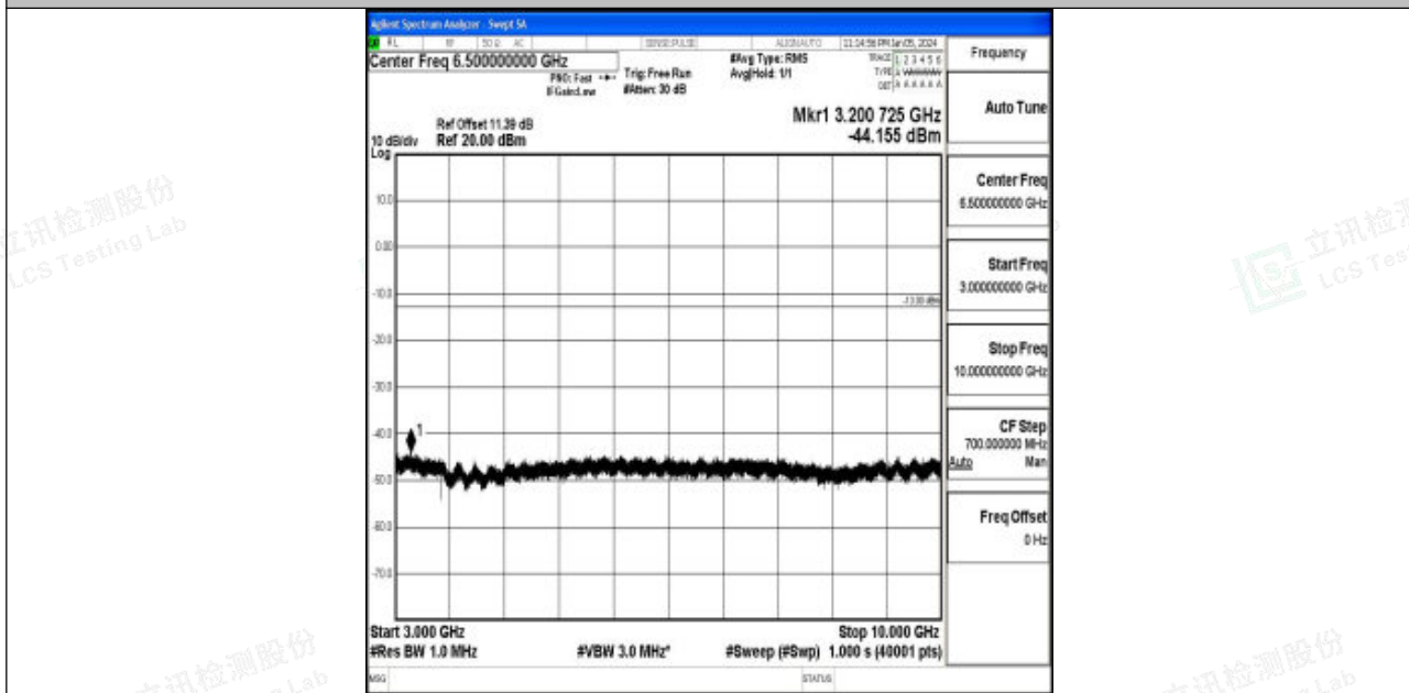
Band12_10MHz_QPSK_23095_1RB#0_3000~10000_3000~10000
