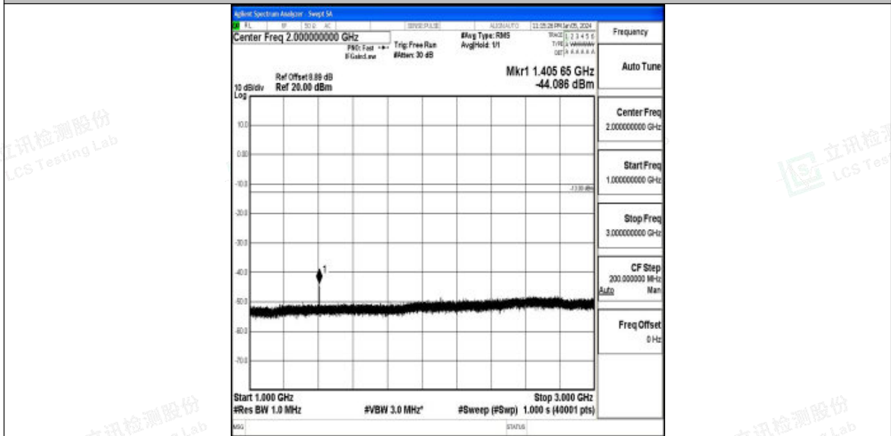
Band12_10MHz_16QAM_23095_1RB#0_1000~3000_1000~3000
