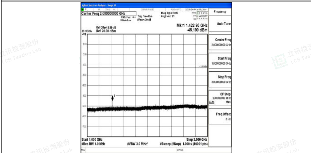
Band12_5MHz_16QAM_23155_1RB#0_1000~3000_1000~3000
