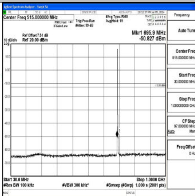
Band12_1.4MHz_16QAM_23017_1RB#0_30~1000_30~1000
