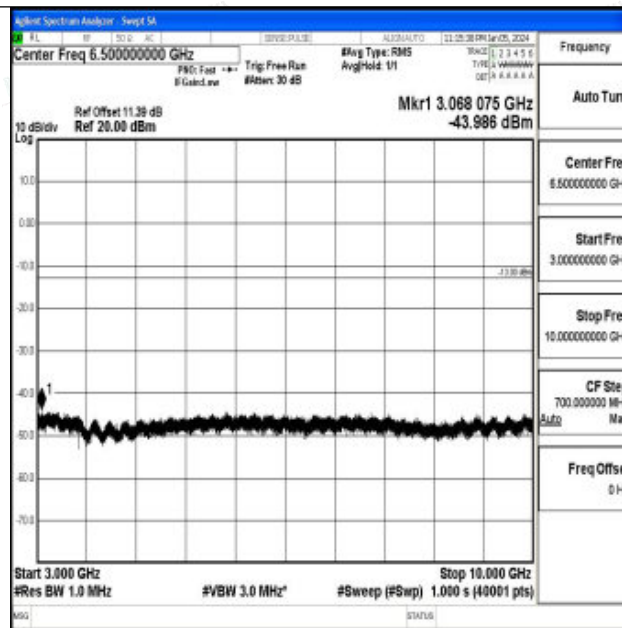
Band12_10MHz_16QAM_23095_1RB#0_3000~10000_3000~10000
