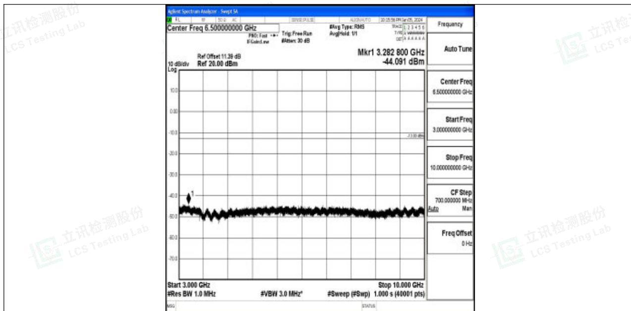
Band12_1.4MHz_16QAM_23173_1RB#0_3000~10000_3000~10000
