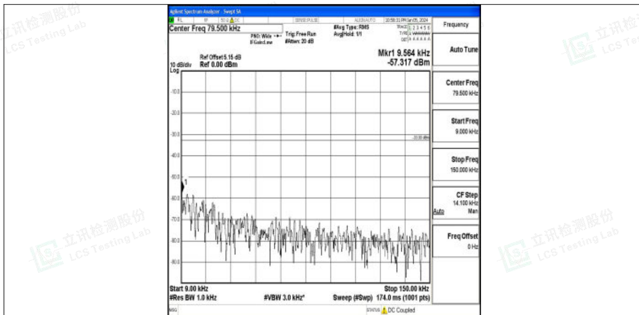
Band12_5MHz_16QAM_23155_1RB#0_0.009~0.15_0.009~0.15
