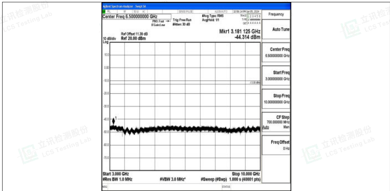
Band12_5MHz_16QAM_23035_1RB#0_3000~10000_3000~10000
