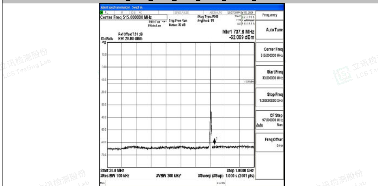
Band12_5MHz_QPSK_23155_1RB#0_30~1000_30~1000
