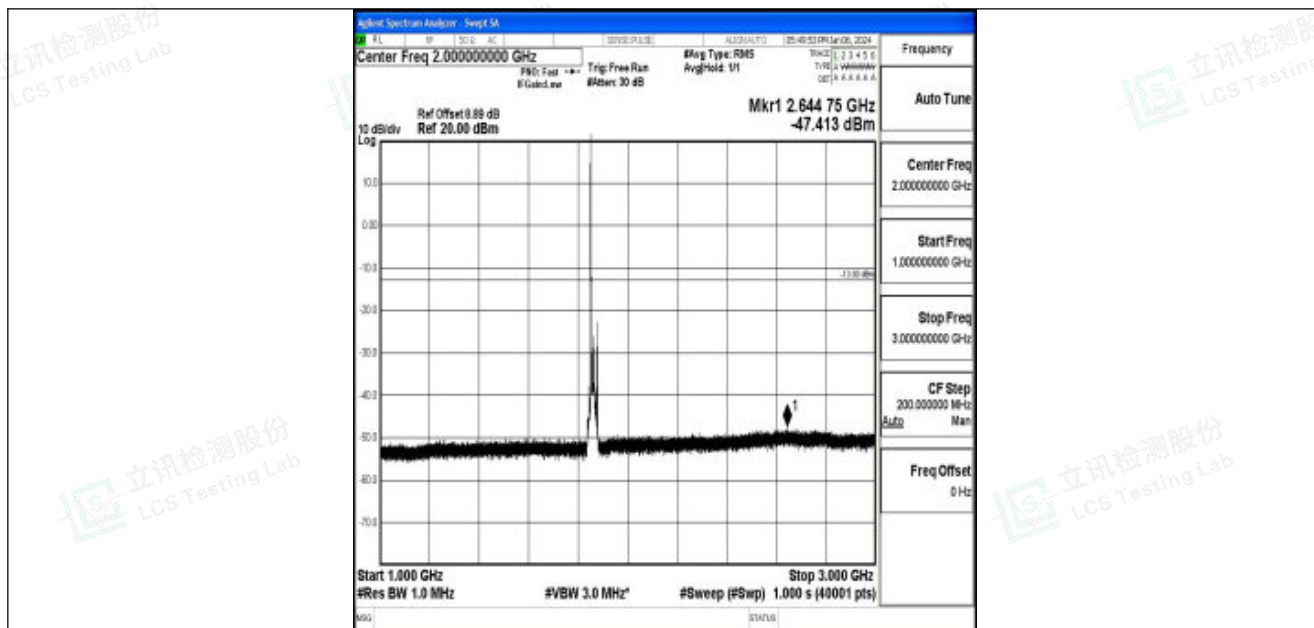
Band25_15MHz_QPSK_26115_1RB#0_1000~3000_1000~3000
