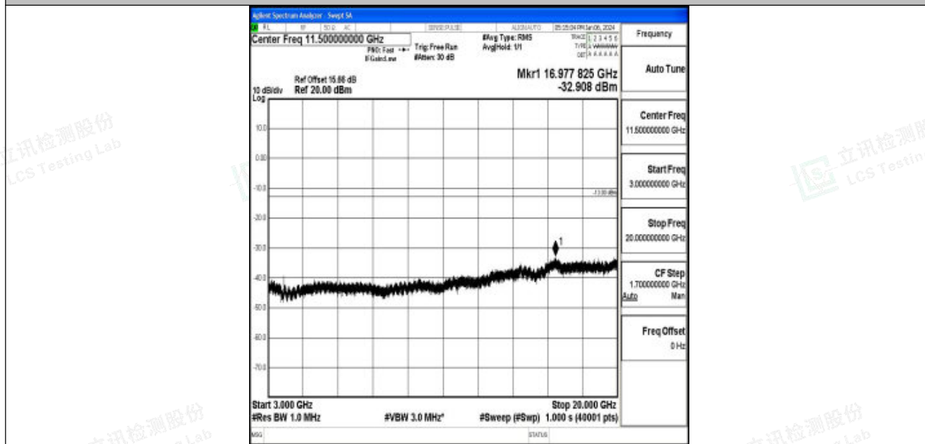
Band25_5MHz_QPSK_26365_1RB#0_3000~20000_3000~20000
