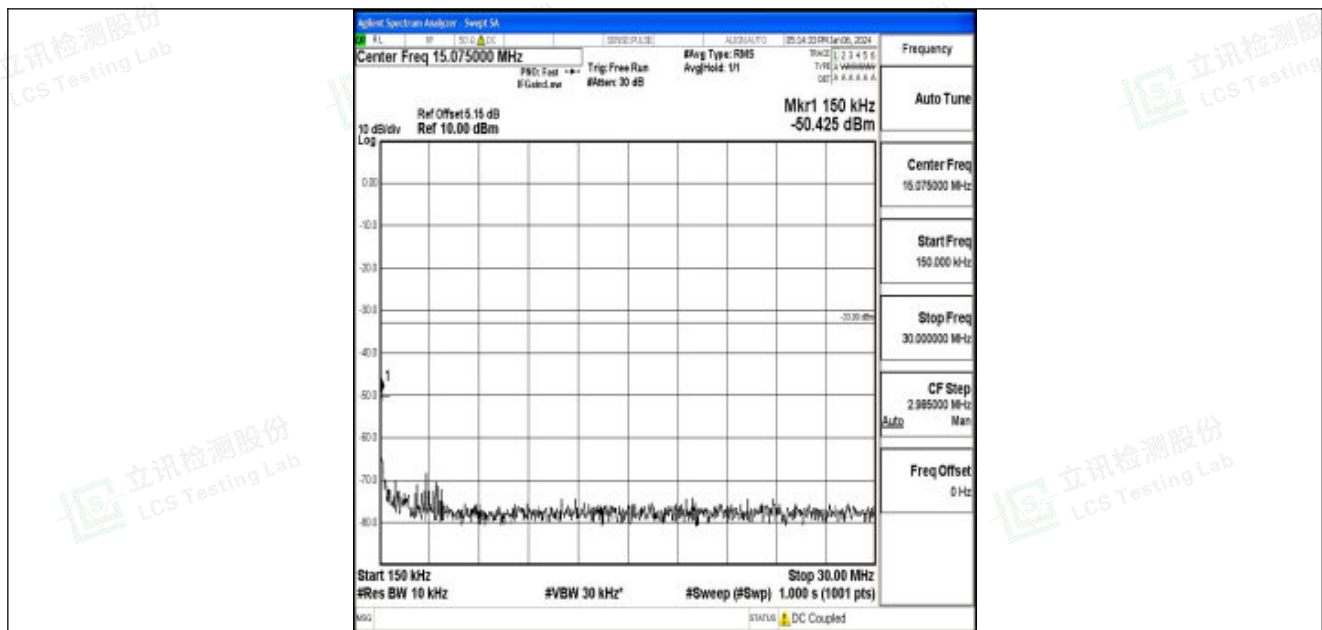
Band25_5MHz_QPSK_26365_1RB#0_0.15~30_0.15~30
