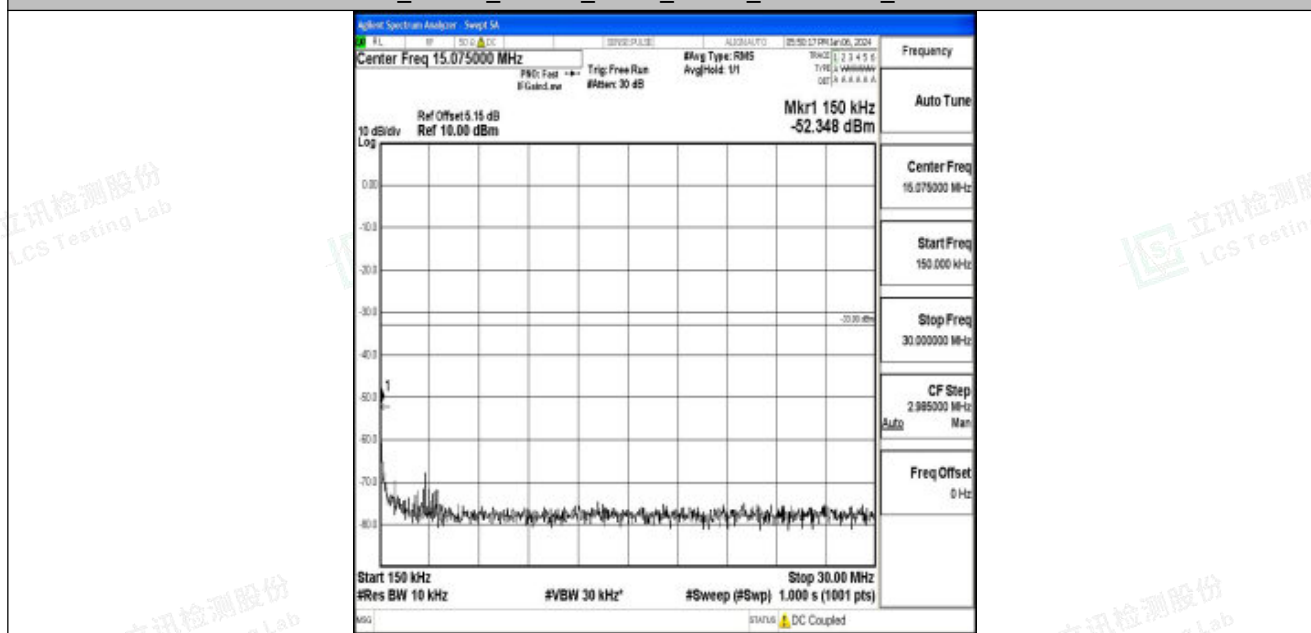
Band25_15MHz_16QAM_26115_1RB#0_0.15~30_0.15~30
