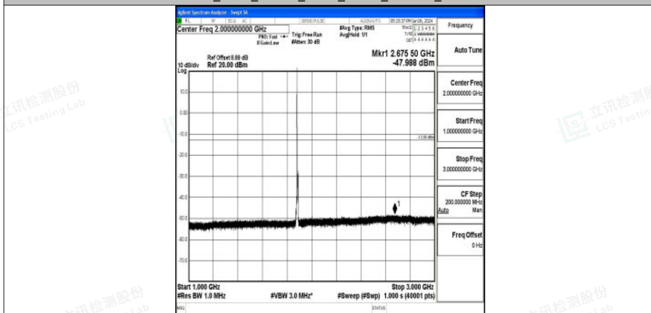
Band25_5MHz_16QAM_26365_1RB#0_1000~3000_1000~3000
