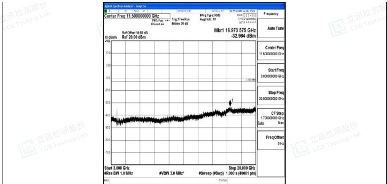
Band25_3MHz_16QAM_26055_1RB#0_3000~20000_3000~20000
