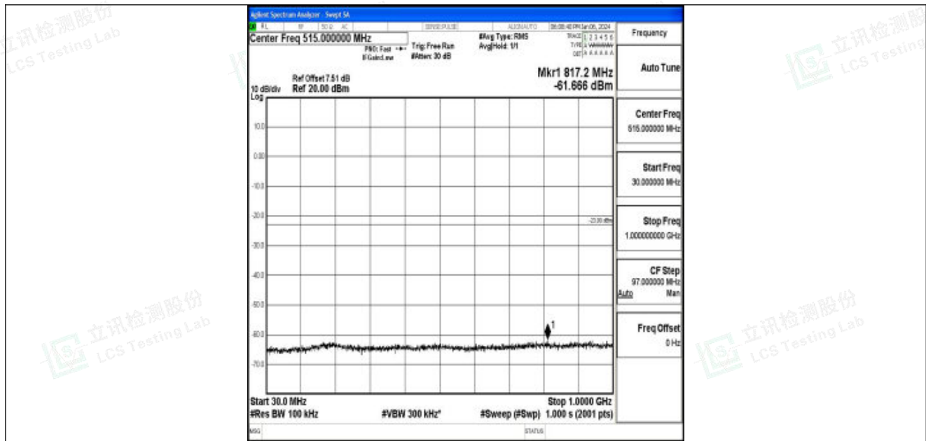
Band25_20MHz_16QAM_26590_1RB#0_30~1000_30~1000
