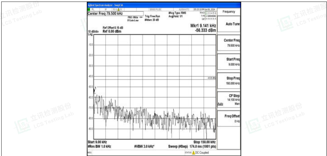
Band25_5MHz_16QAM_26365_1RB#0_0.009~0.15_0.009~0.15
