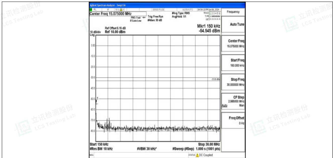
Band25_3MHz_QPSK_26055_1RB#0_0.15~30_0.15~30
