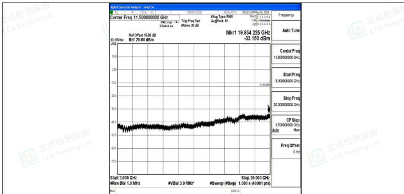
Band25_15MHz_16QAM_26365_1RB#0_3000~20000_3000~20000
