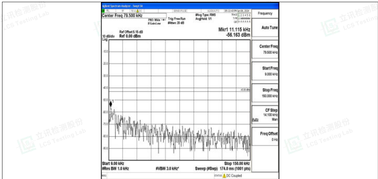
Band25_5MHz_16QAM_26065_1RB#0_0.009~0.15_0.009~0.15
