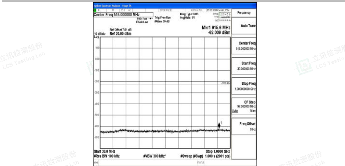
Band25_15MHz_QPSK_26615_1RB#0_30~1000_30~1000
