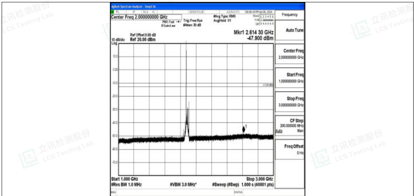
Band25_20MHz_QPSK_26365_1RB#0_1000~3000_1000~3000
