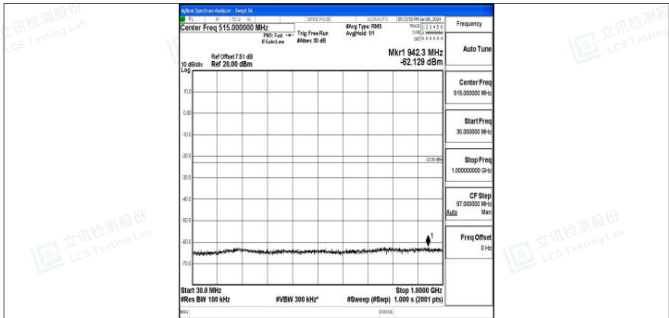
Band25_5MHz_16QAM_26065_1RB#0_30~1000_30~1000
