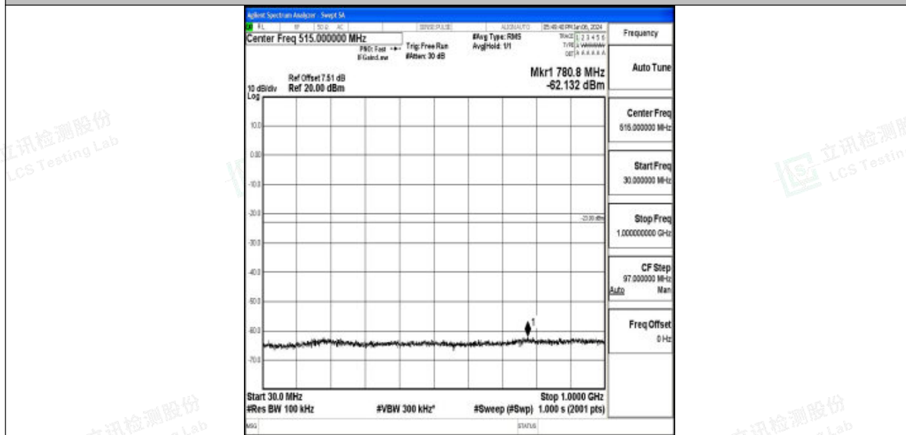
Band25_15MHz_QPSK_26115_1RB#0_30~1000_30~1000
