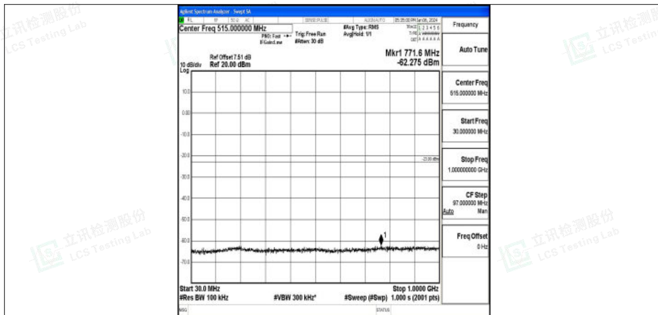
Band25_10MHz_16QAM_26365_1RB#0_30~1000_30~1000
