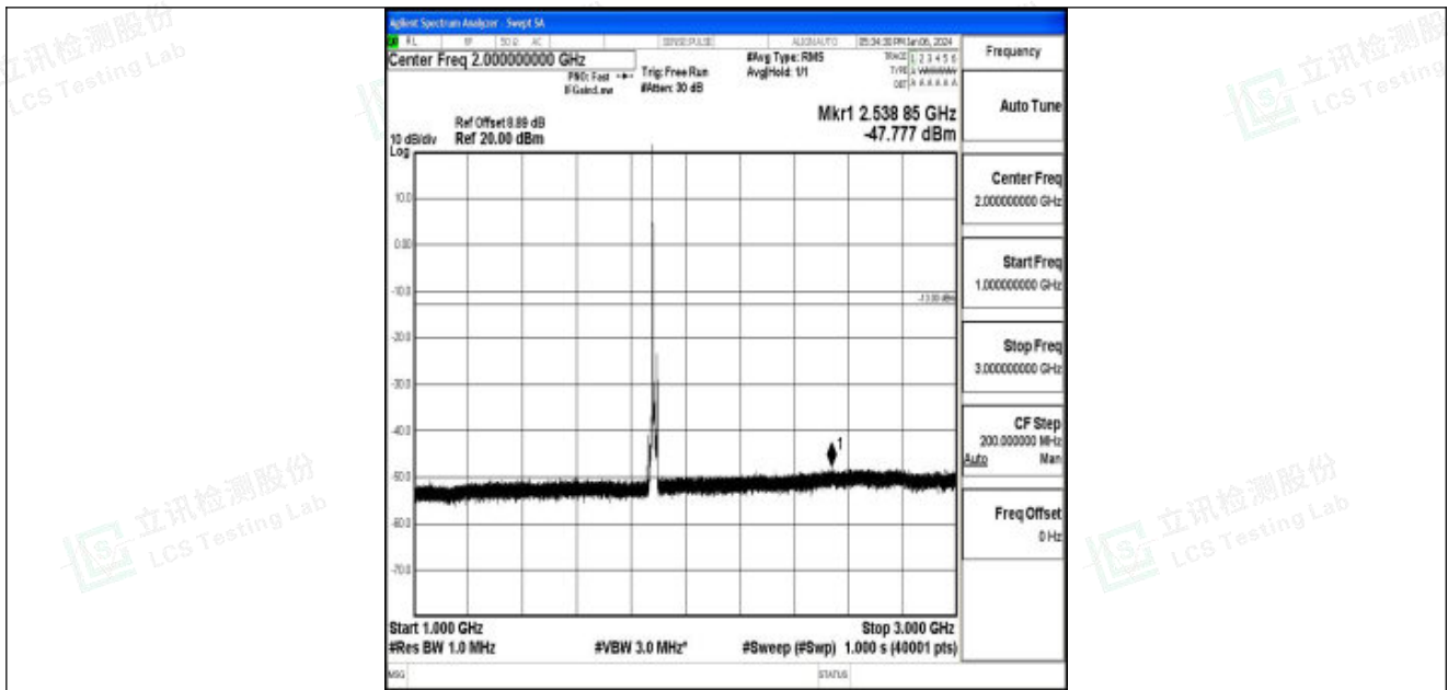
Band25_10MHz_QPSK_26365_1RB#0_1000~3000_1000~3000
