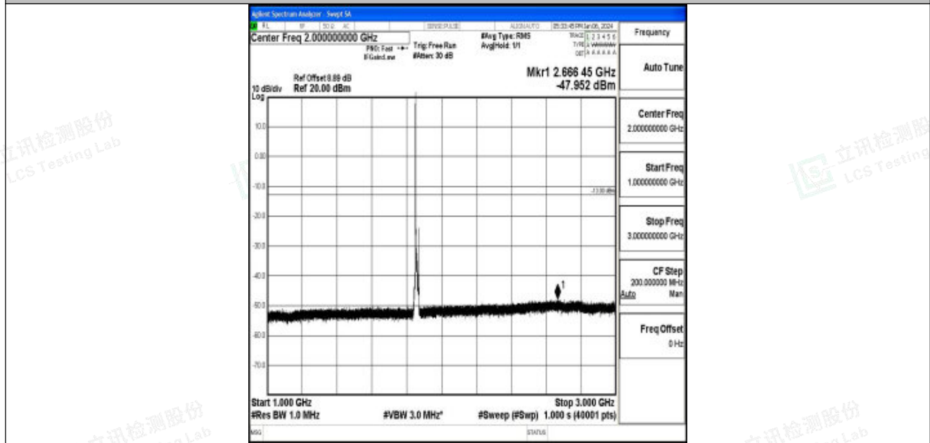
Band25_10MHz_16QAM_26090_1RB#0_1000~3000_1000~3000
