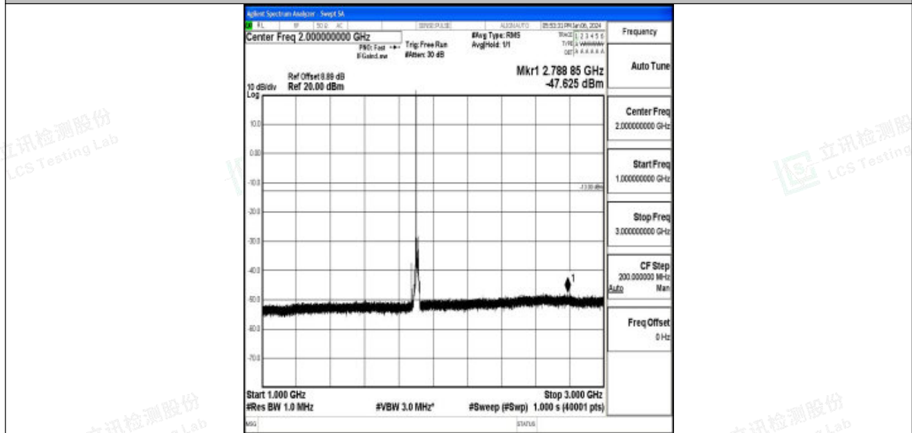
Band25_15MHz_16QAM_26615_1RB#0_1000~3000_1000~3000
