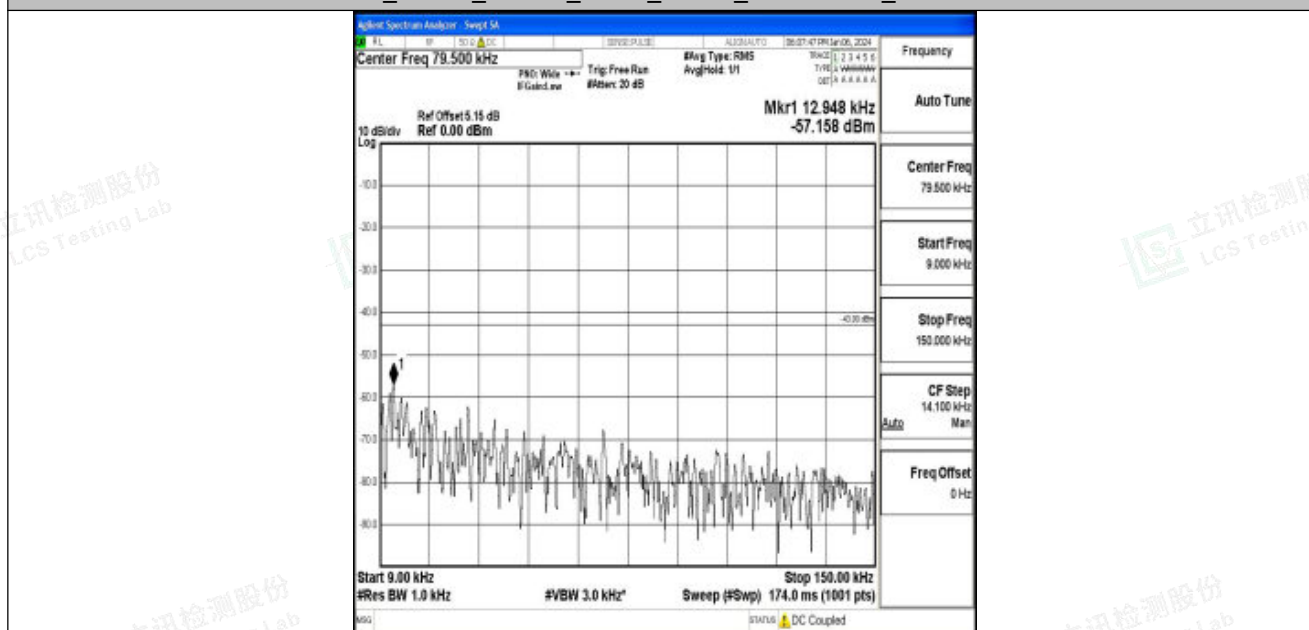
Band25_20MHz_QPSK_26590_1RB#0_0.009~0.15_0.009~0.15
