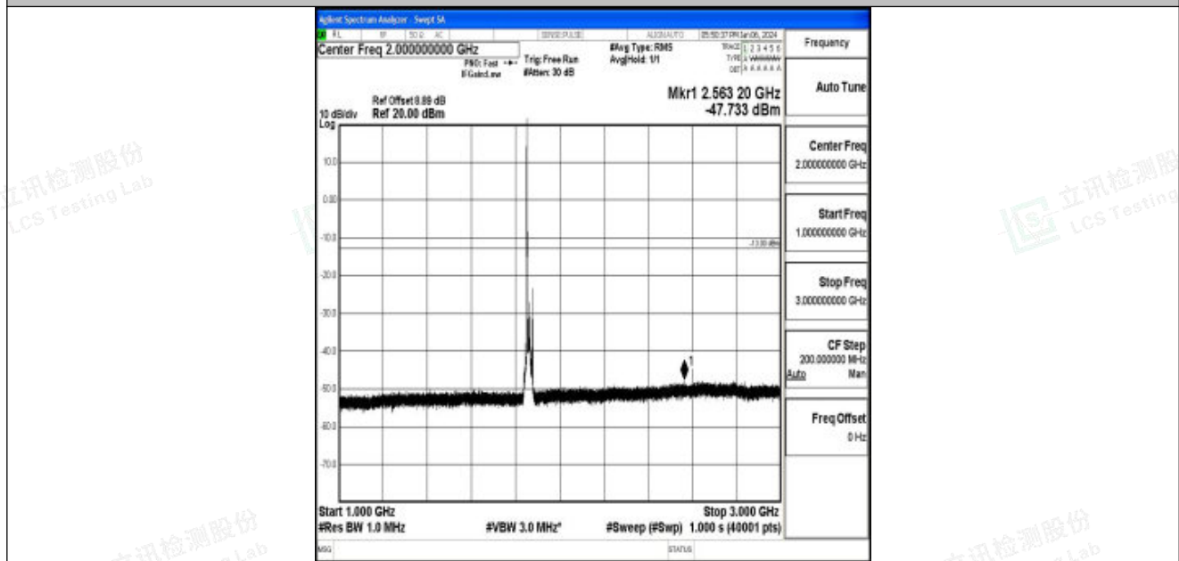
Band25_15MHz_16QAM_26115_1RB#0_1000~3000_1000~3000
