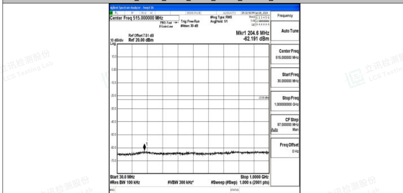
Band25_10MHz_QPSK_26090_1RB#0_30~1000_30~1000
