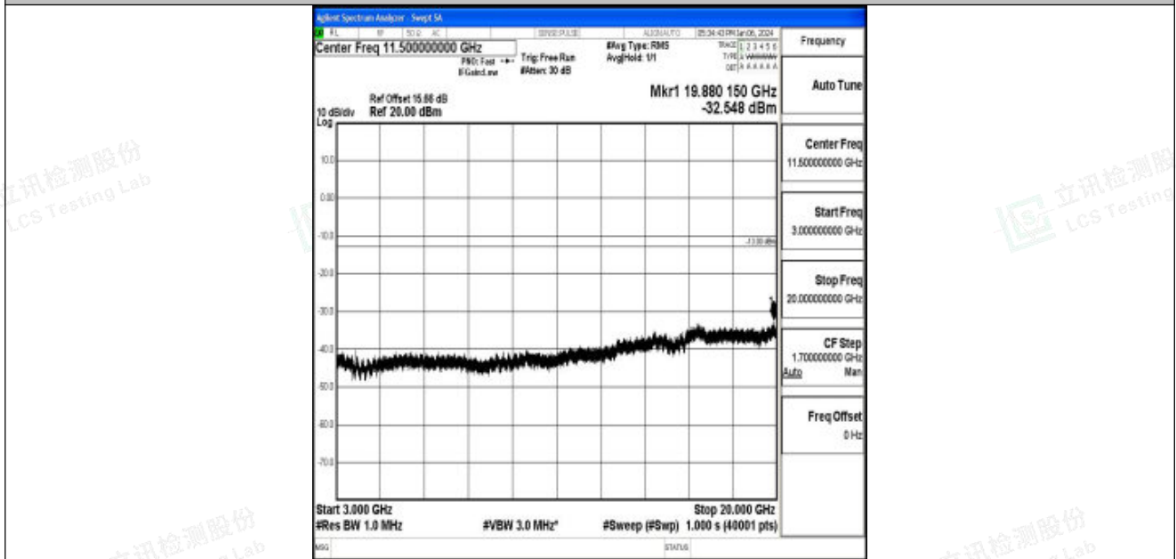
Band25_10MHz_QPSK_26365_1RB#0_3000~20000_3000~20000
