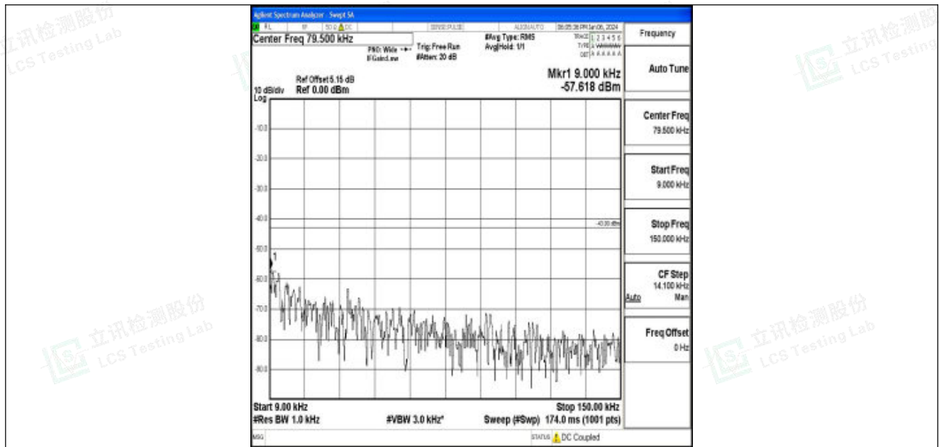
Band25_20MHz_16QAM_26140_1RB#0_0.009~0.15_0.009~0.15
