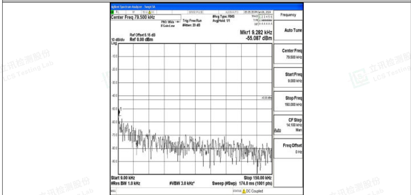
Band25_10MHz_QPSK_26640_1RB#0_0.009~0.15_0.009~0.15
