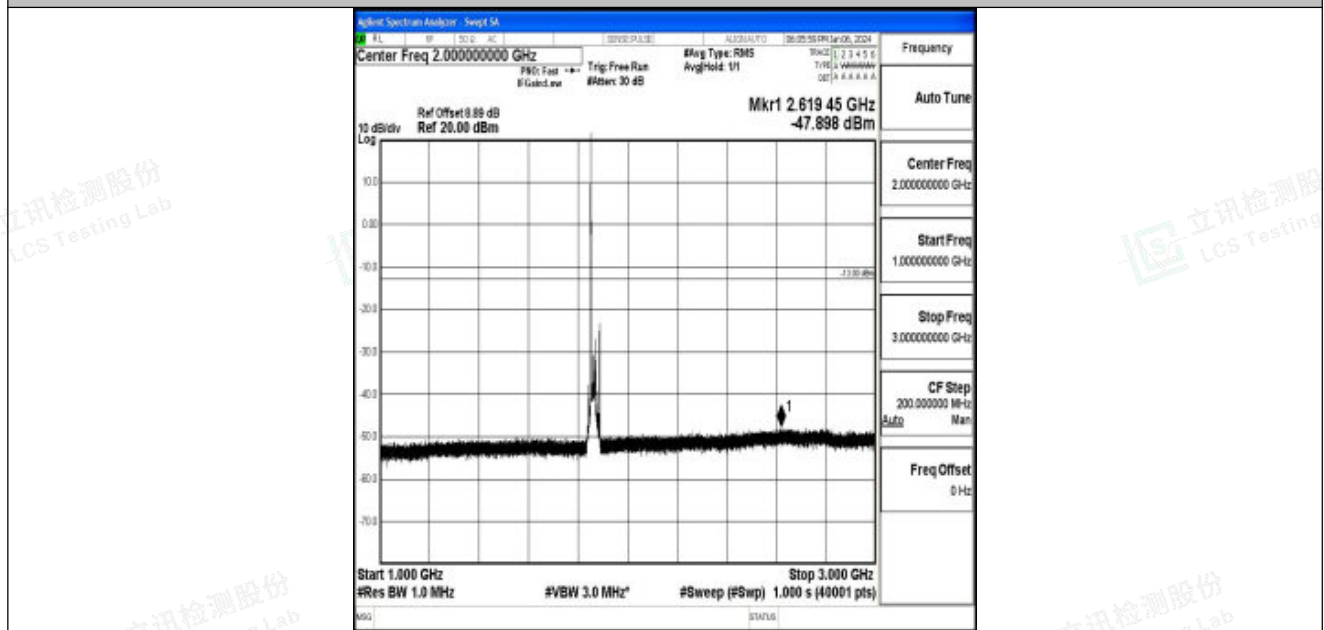
Band25_20MHz_16QAM_26140_1RB#0_1000~3000_1000~3000
