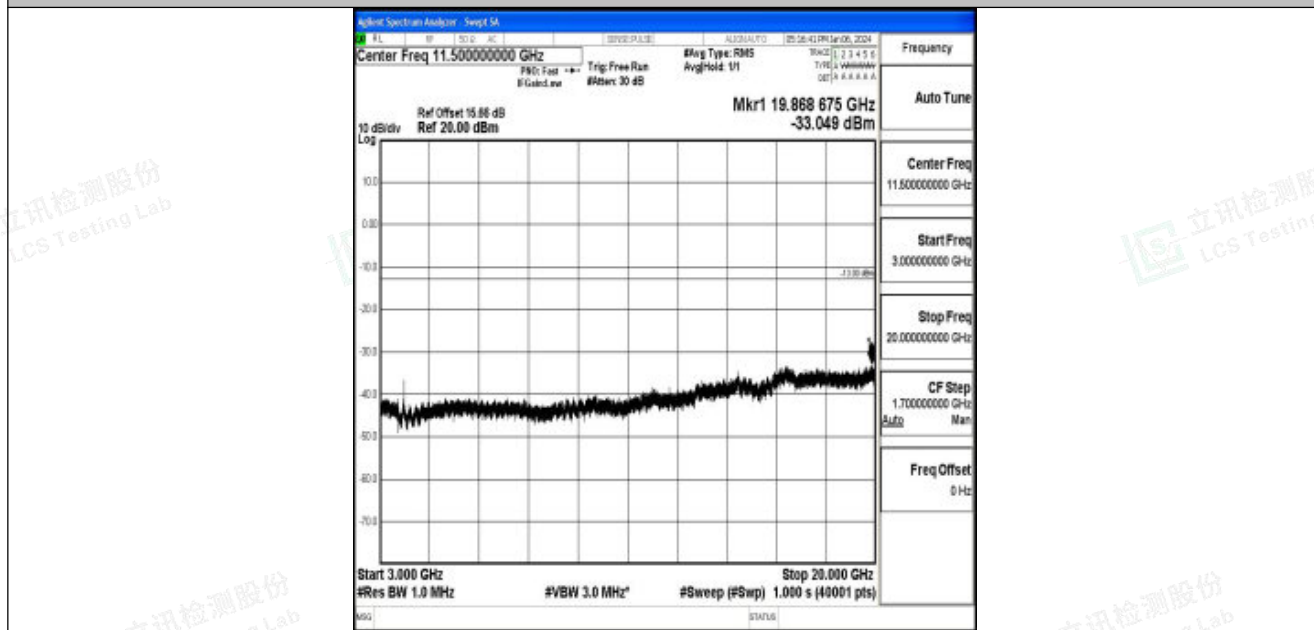
Band25_5MHz_QPSK_26665_1RB#0_3000~20000_3000~20000
