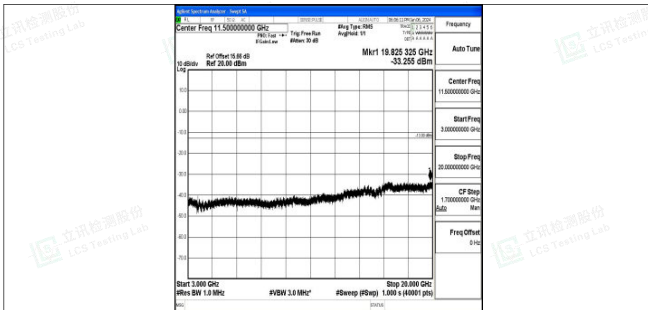
Band25_20MHz_16QAM_26140_1RB#0_3000~20000_3000~20000
