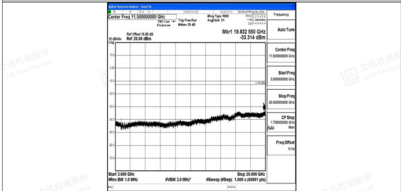
Band25_20MHz_QPSK_26140_1RB#0_3000~20000_3000~20000
