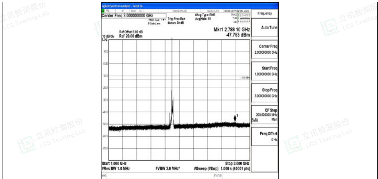
Band25_20MHz_QPSK_26590_1RB#0_1000~3000_1000~3000
