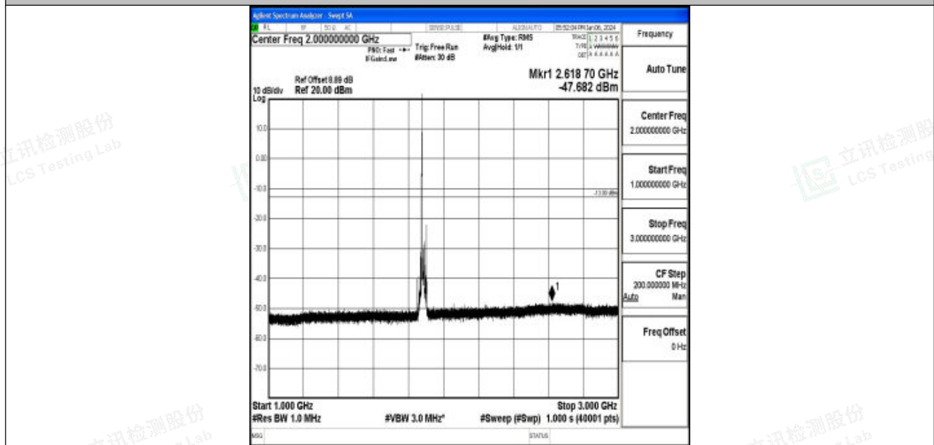
Band25_15MHz_16QAM_26365_1RB#0_1000~3000_1000~3000
