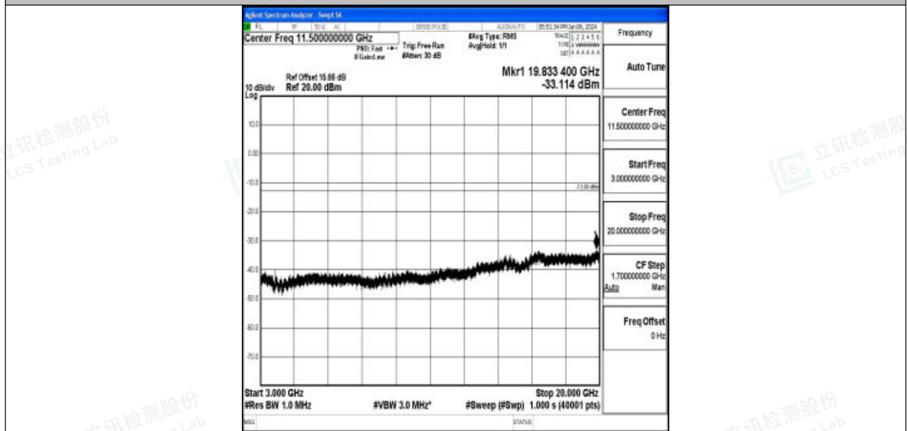
Band25_15MHz_QPSK_26365_1RB#0_3000~20000_3000~20000
