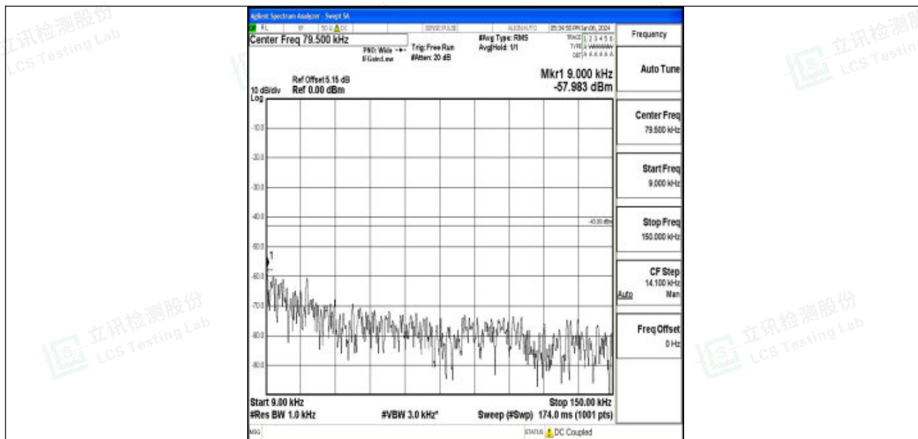
Band25_10MHz_16QAM_26365_1RB#0_0.009~0.15_0.009~0.15
