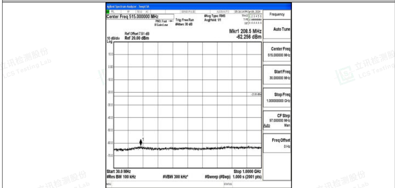
Band25_5MHz_QPSK_26665_1RB#0_30~1000_30~1000
