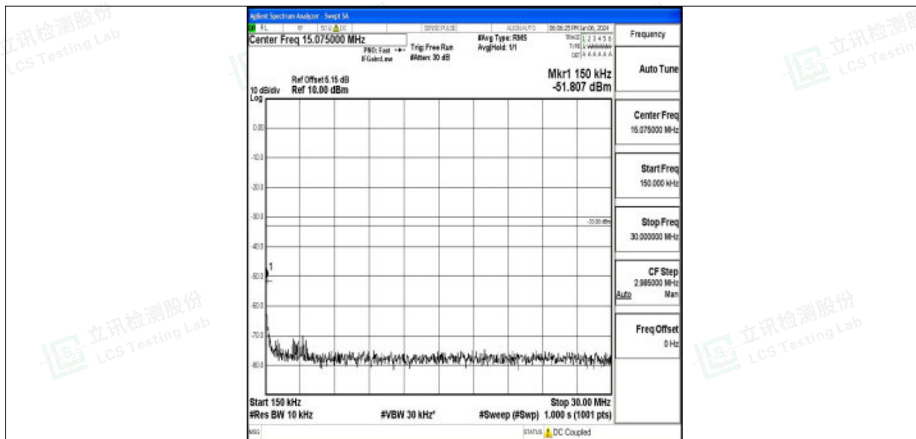
Band25_20MHz_QPSK_26365_1RB#0_0.15~30_0.15~30
