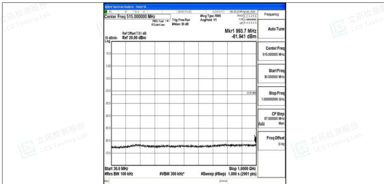
Band25_5MHz_16QAM_26365_1RB#0_30~1000_30~1000
