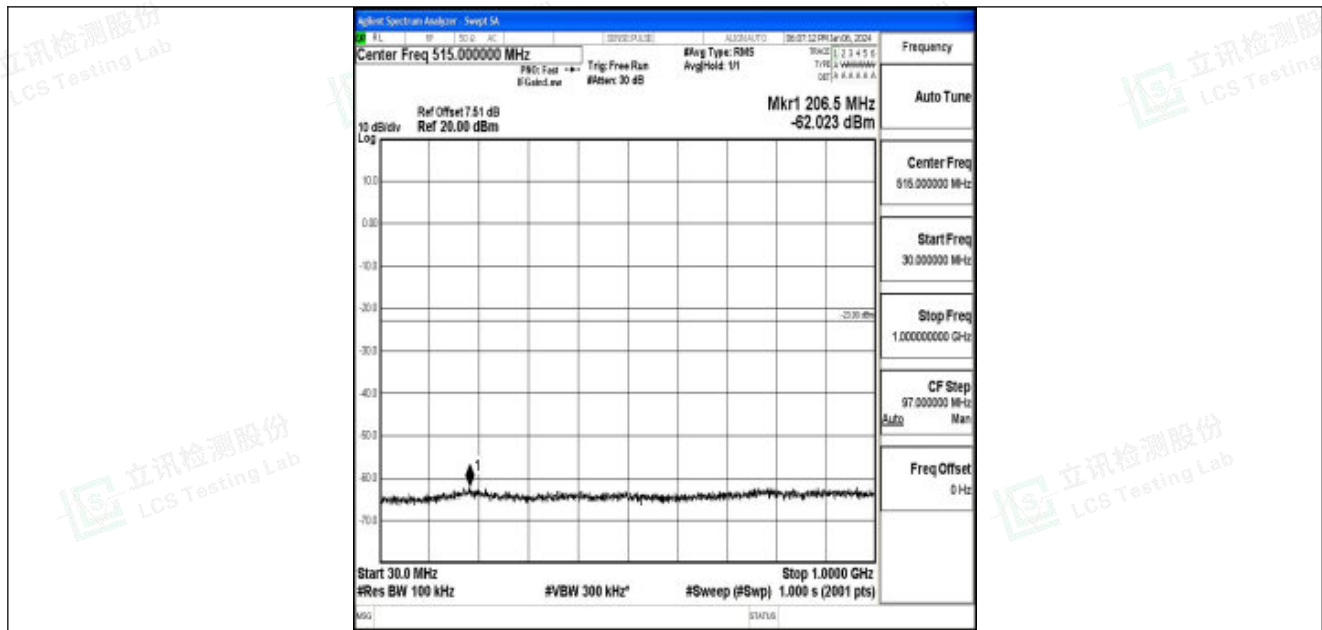
Band25_20MHz_16QAM_26365_1RB#0_30~1000_30~1000
