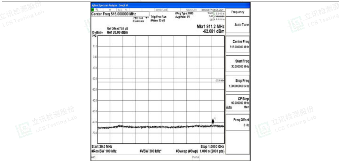
Band25_15MHz_16QAM_26615_1RB#0_30~1000_30~1000
