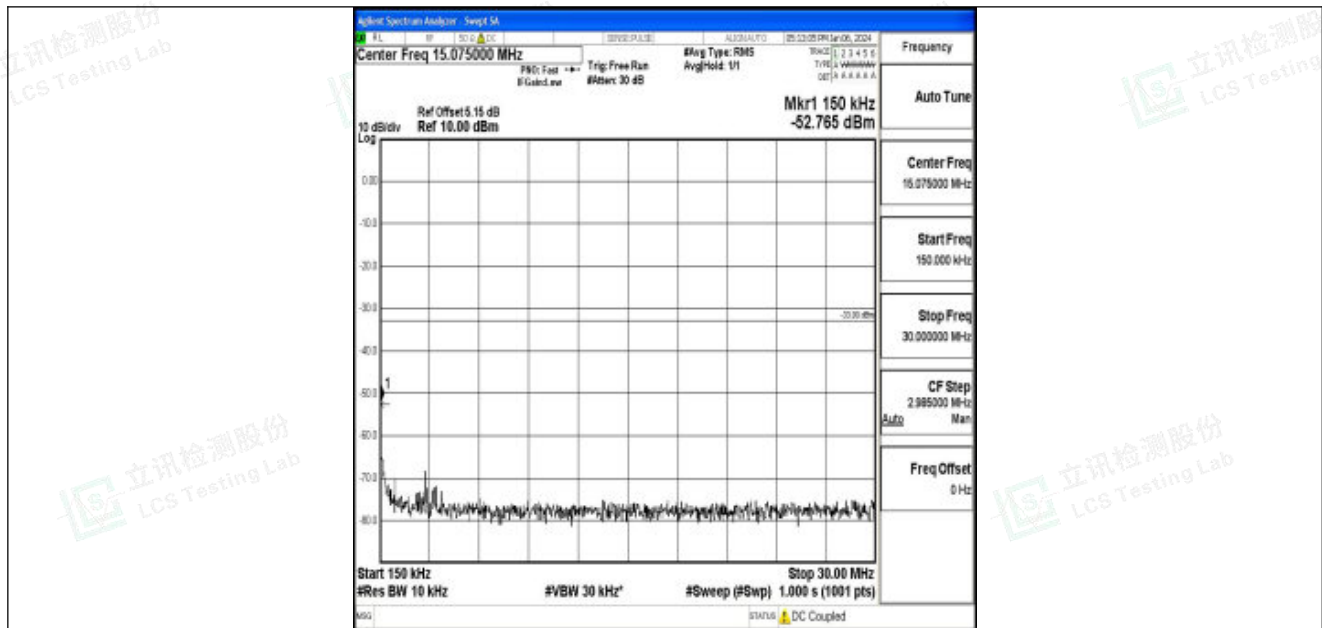
Band25_5MHz_QPSK_26065_1RB#0_0.15~30_0.15~30
