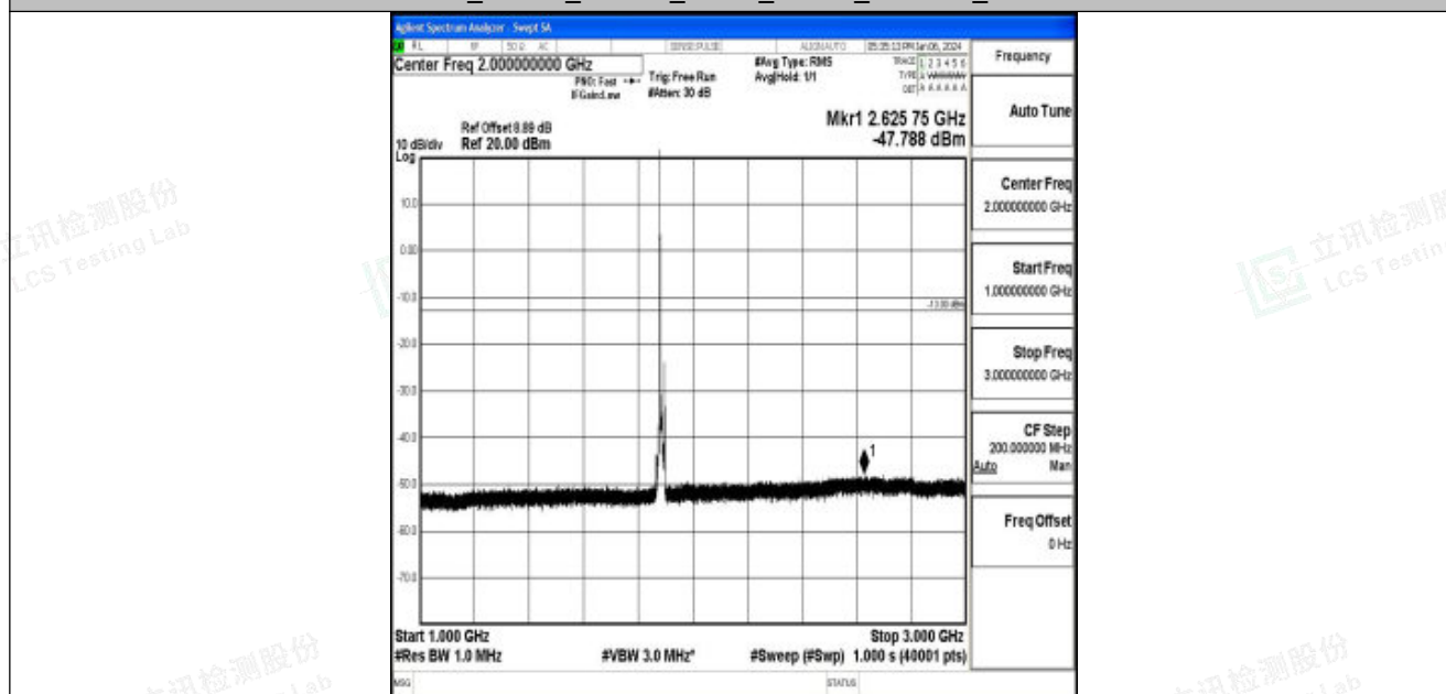
Band25_10MHz_16QAM_26365_1RB#0_1000~3000_1000~3000
