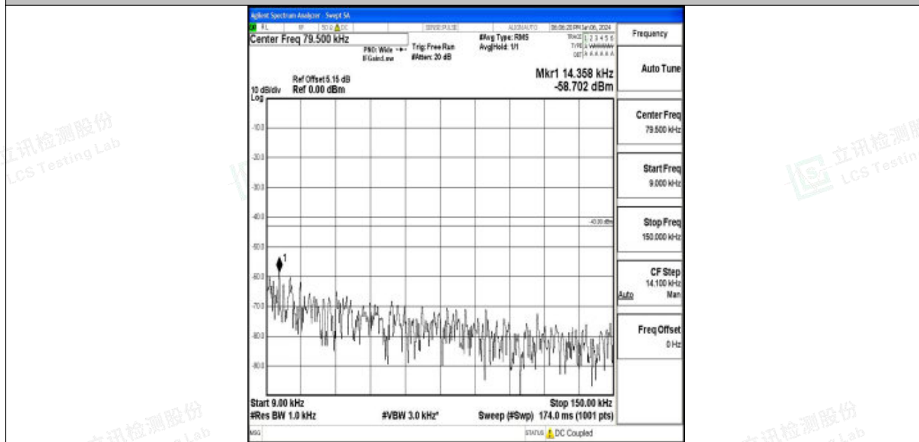
Band25_20MHz_QPSK_26365_1RB#0_0.009~0.15_0.009~0.15
