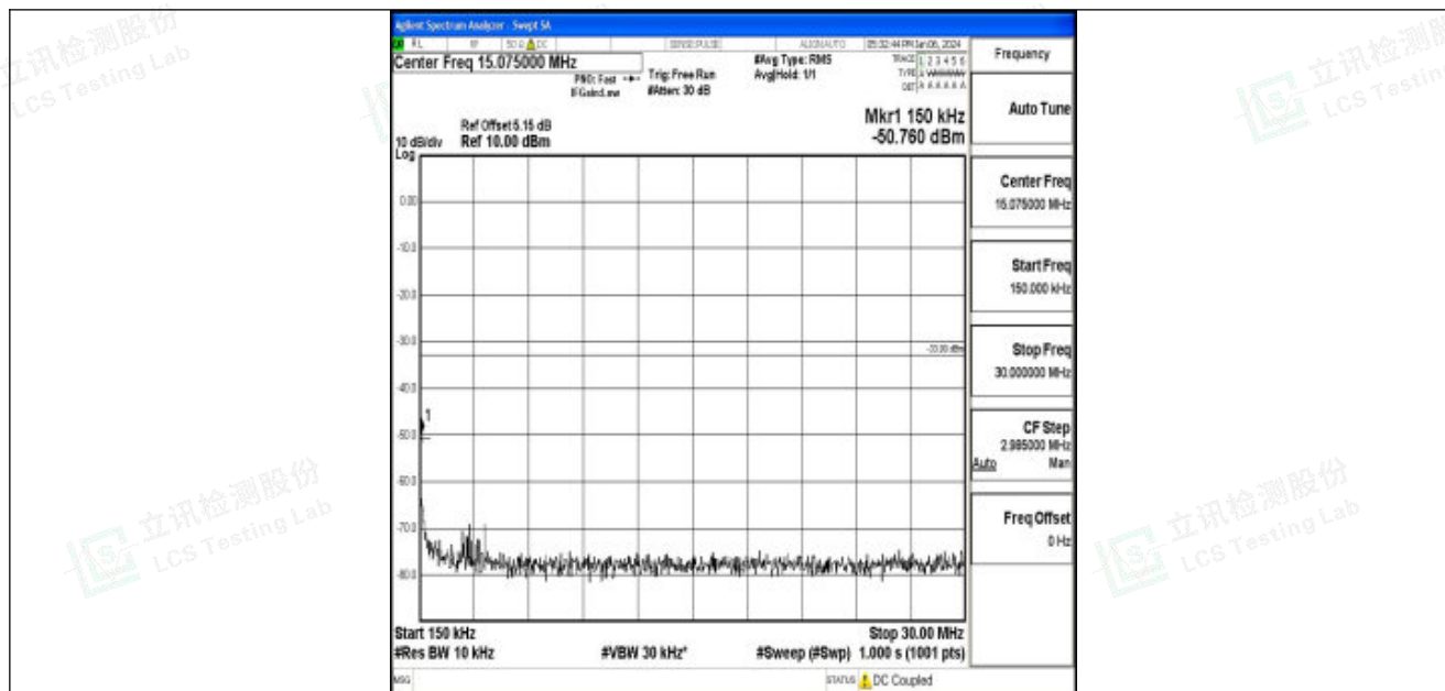
Band25_10MHz_QPSK_26090_1RB#0_0.15~30_0.15~30
