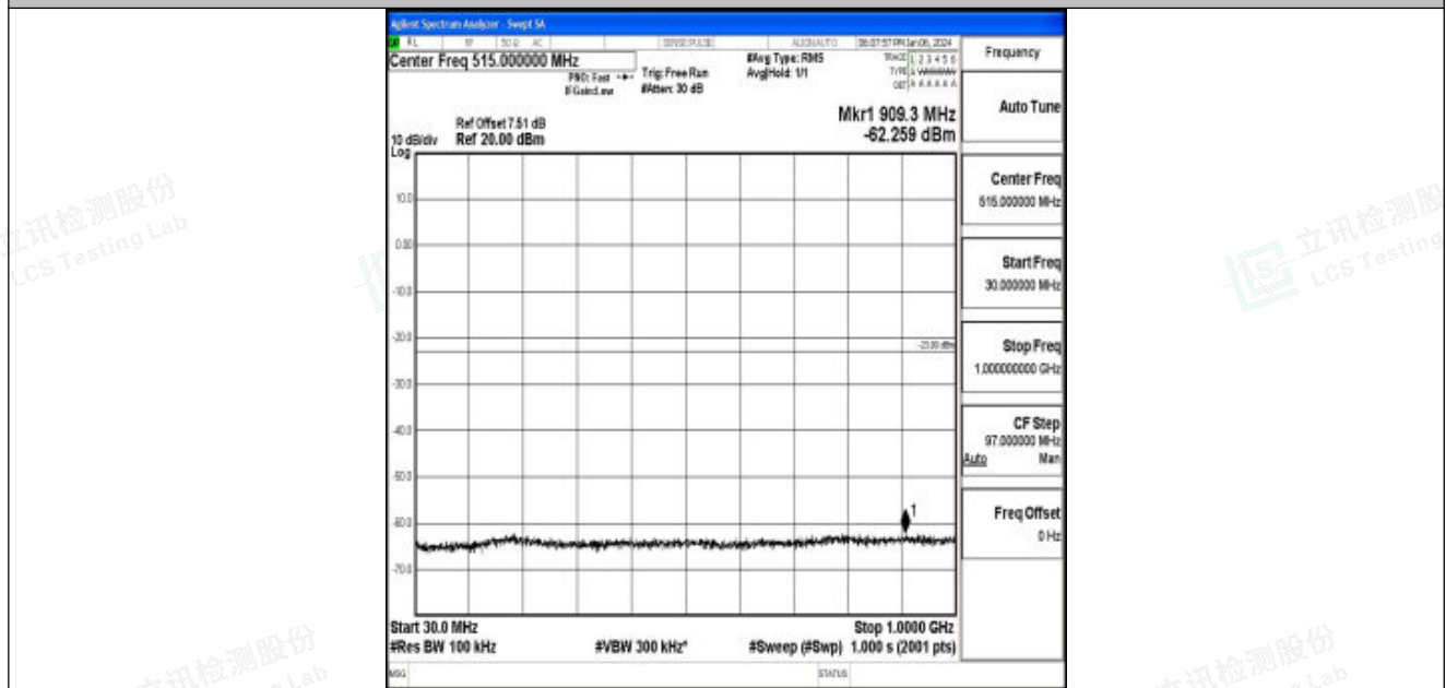
Band25_20MHz_QPSK_26590_1RB#0_30~1000_30~1000
