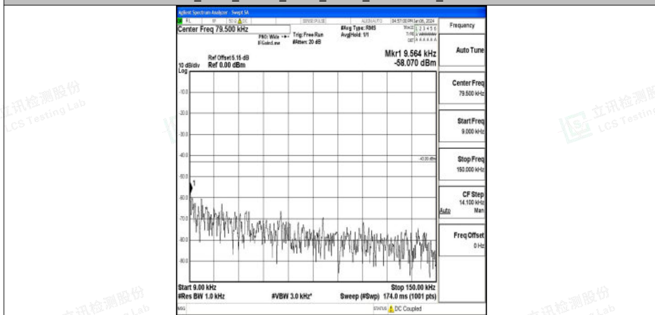
Band25_3MHz_QPSK_26675_1RB#0_0.009~0.15_0.009~0.15
