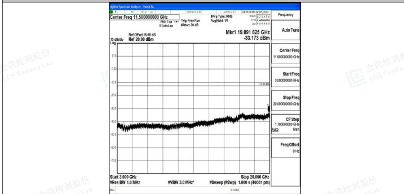
Band25_3MHz_QPSK_26365_1RB#0_3000~20000_3000~20000
