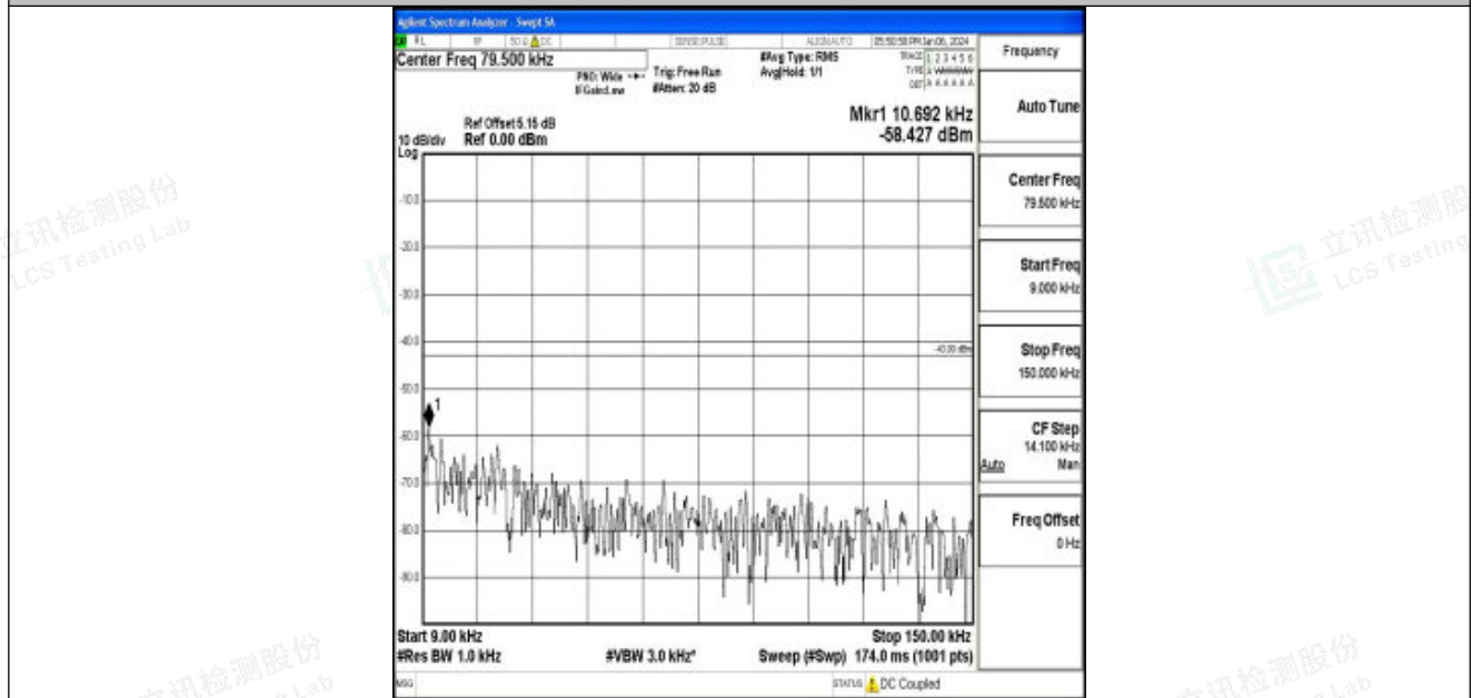
Band25_15MHz_QPSK_26365_1RB#0_0.009~0.15_0.009~0.15
