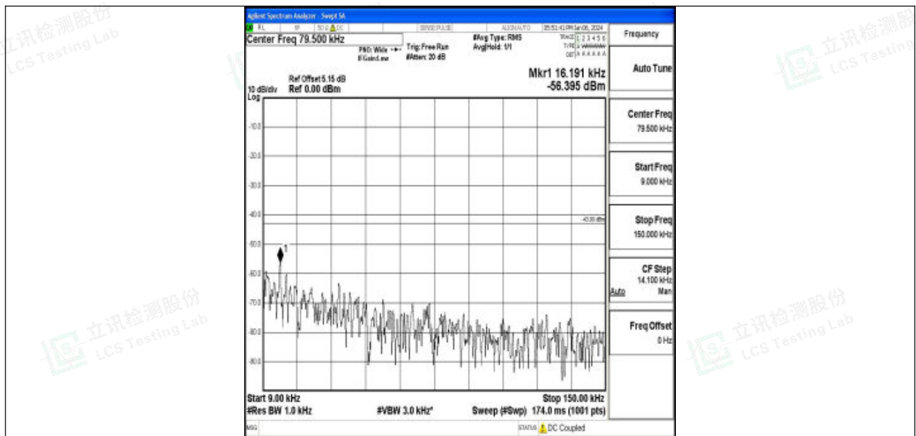
Band25_15MHz_16QAM_26365_1RB#0_0.009~0.15_0.009~0.15
