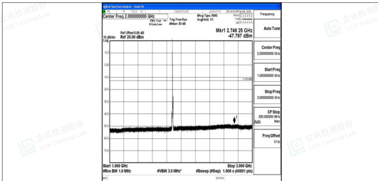
Band25_5MHz_QPSK_26365_1RB#0_1000~3000_1000~3000
