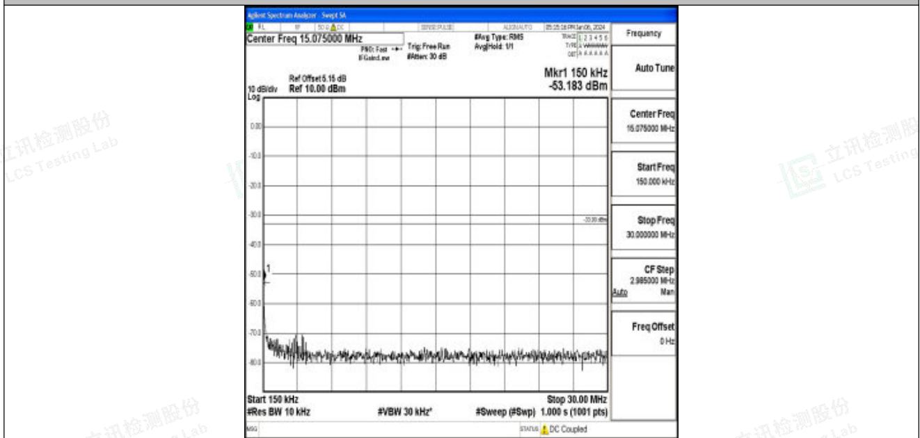
Band25_5MHz_16QAM_26365_1RB#0_0.15~30_0.15~30
