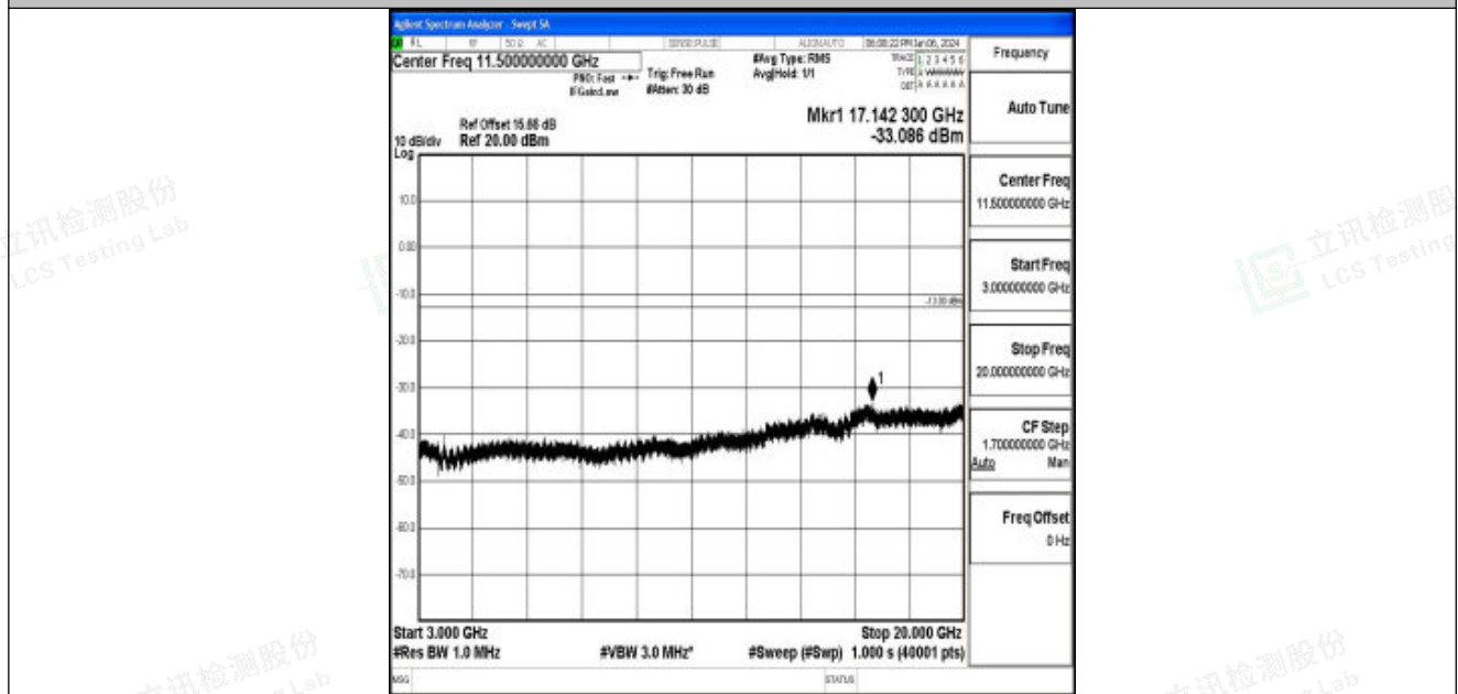
Band25_20MHz_QPSK_26590_1RB#0_3000~20000_3000~20000
