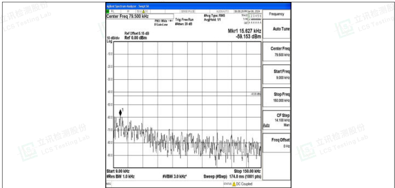
Band25_20MHz_16QAM_26590_1RB#0_0.009~0.15_0.009~0.15
