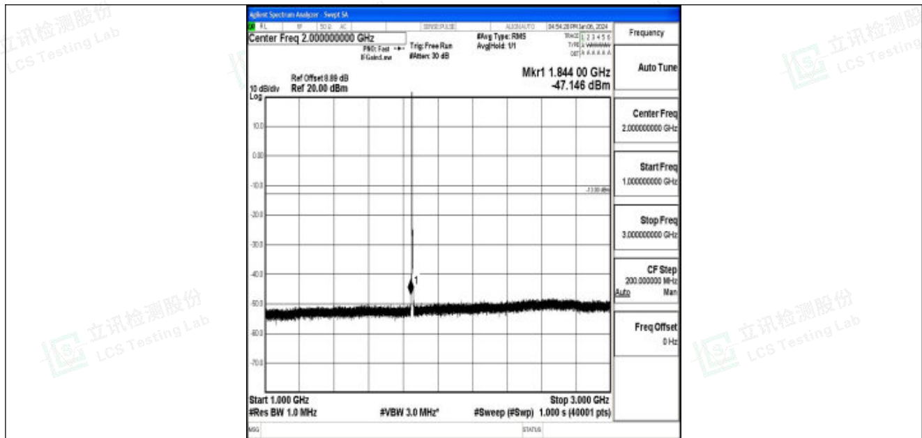
Band25_3MHz_QPSK_26055_1RB#0_1000~3000_1000~3000
