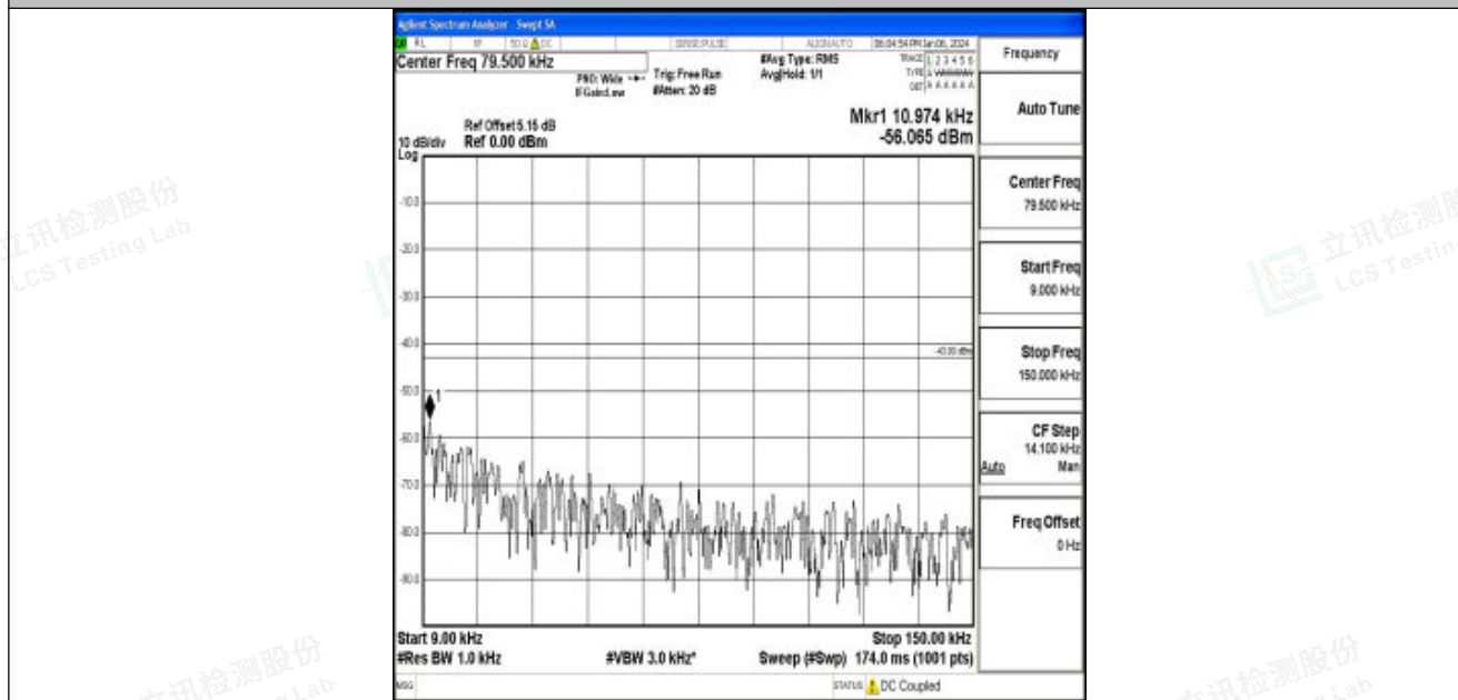
Band25_20MHz_QPSK_26140_1RB#0_0.009~0.15_0.009~0.15
