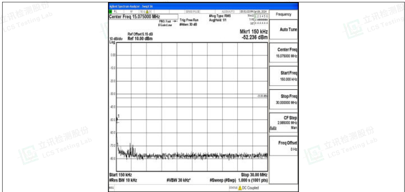
Band25_15MHz_QPSK_26365_1RB#0_0.15~30_0.15~30
