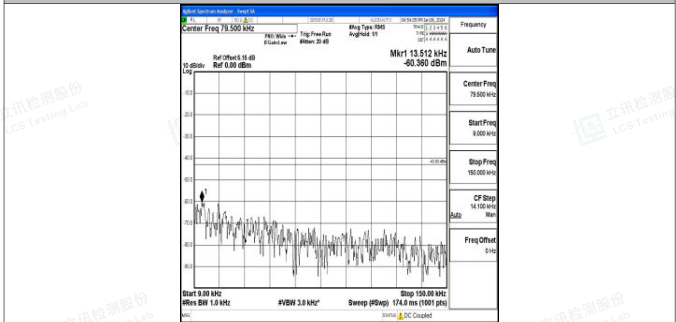
Band25_3MHz_QPSK_26055_1RB#0_0.009~0.15_0.009~0.15
