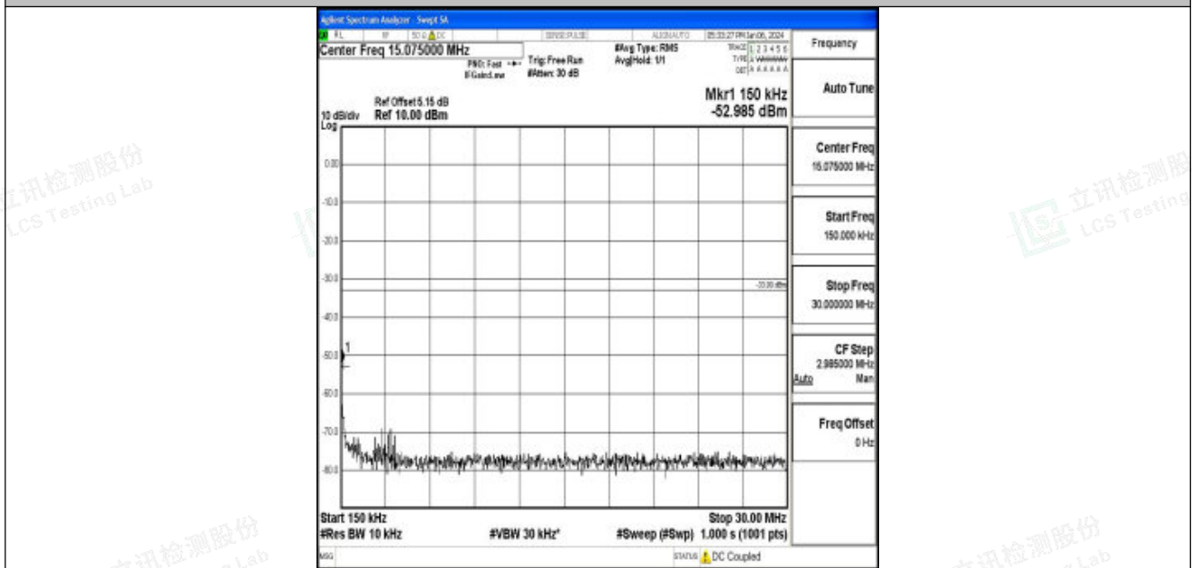
Band25_10MHz_16QAM_26090_1RB#0_0.15~30_0.15~30
