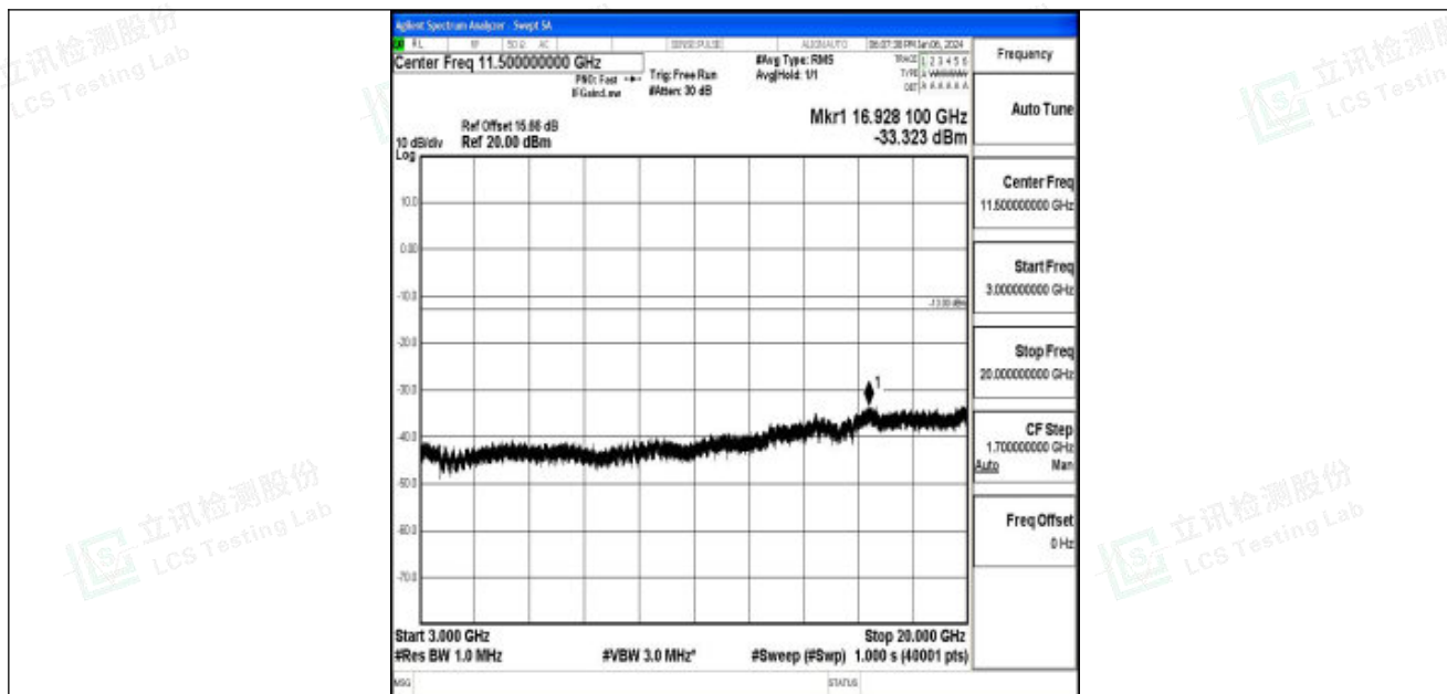
Band25_20MHz_16QAM_26365_1RB#0_3000~20000_3000~20000
