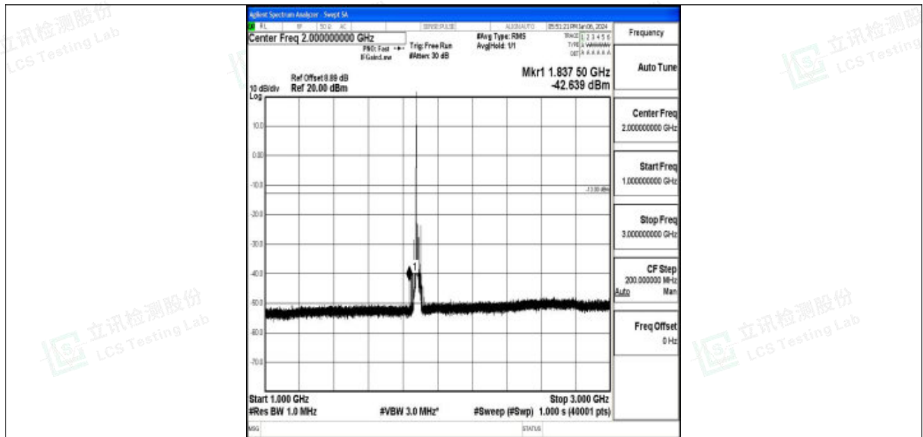
Band25_15MHz_QPSK_26365_1RB#0_1000~3000_1000~3000
