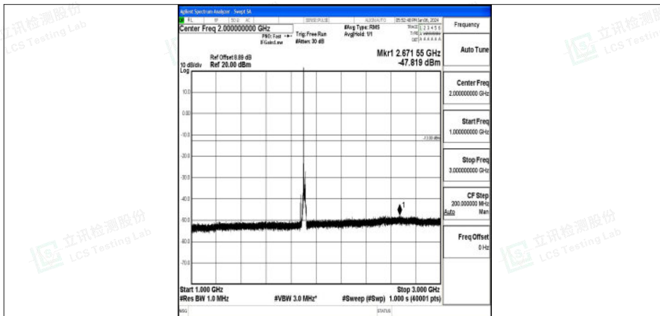
Band25_15MHz_QPSK_26615_1RB#0_1000~3000_1000~3000
