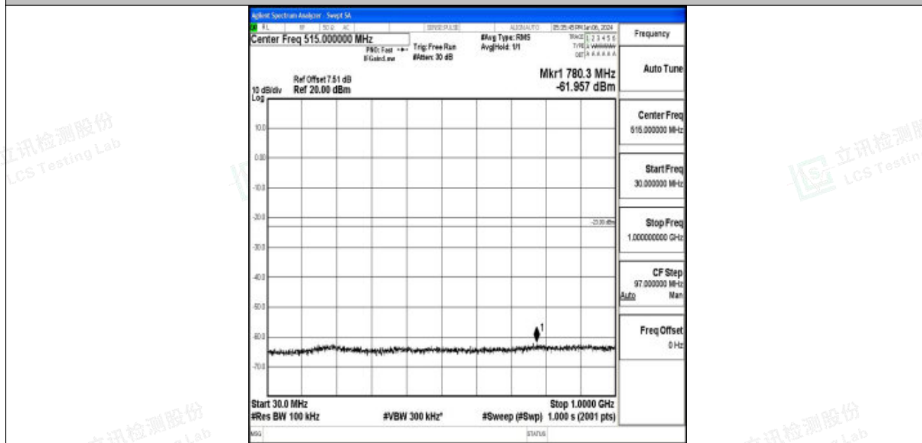
Band25_10MHz_QPSK_26640_1RB#0_30~1000_30~1000
