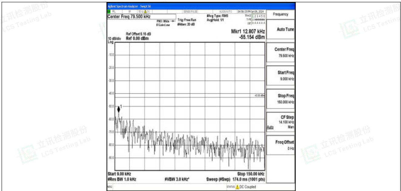
Band25_3MHz_16QAM_26365_1RB#0_0.009~0.15_0.009~0.15
