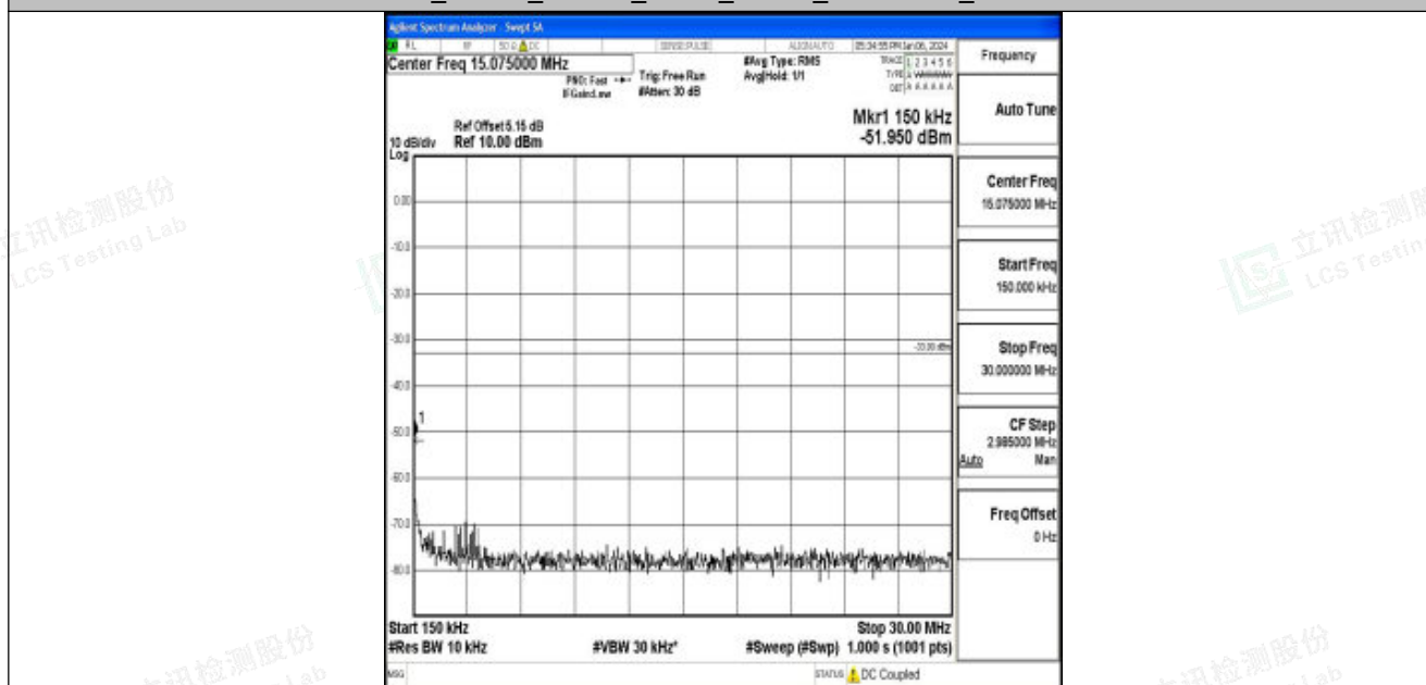
Band25_10MHz_16QAM_26365_1RB#0_0.15~30_0.15~30
