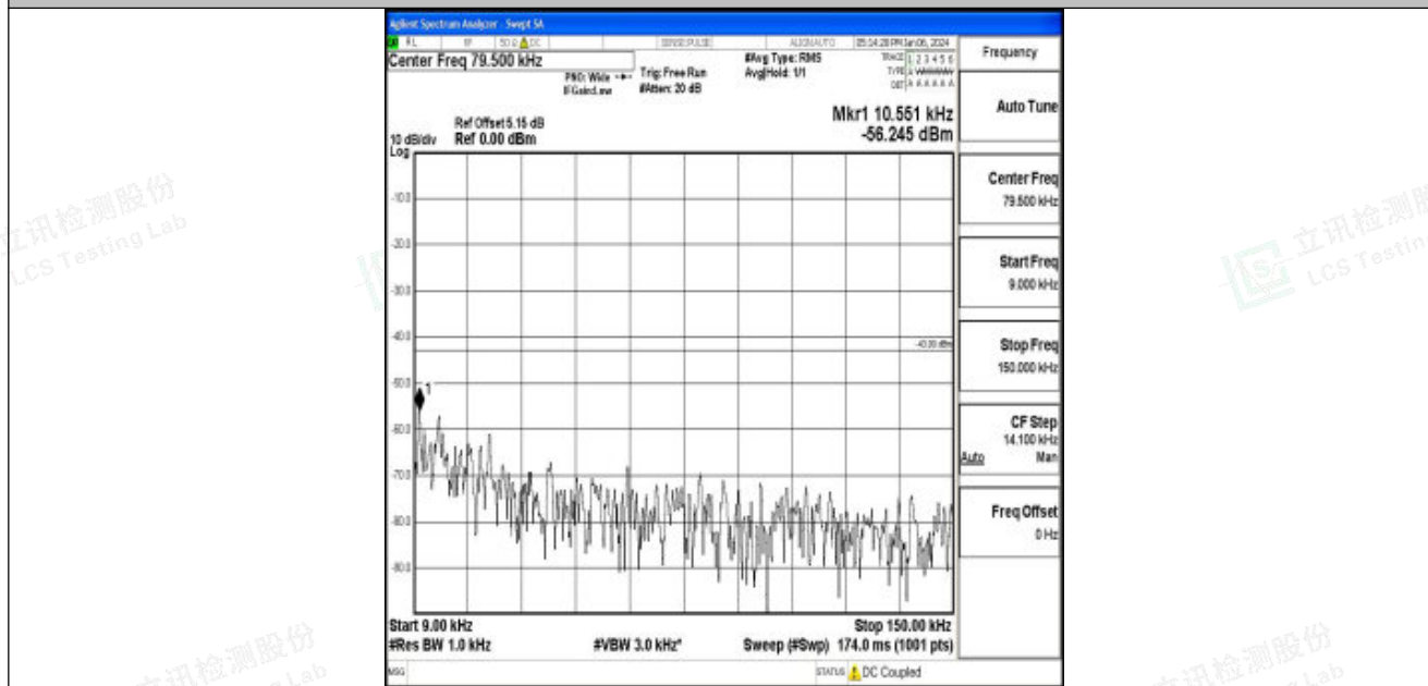
Band25_5MHz_QPSK_26365_1RB#0_0.009~0.15_0.009~0.15
