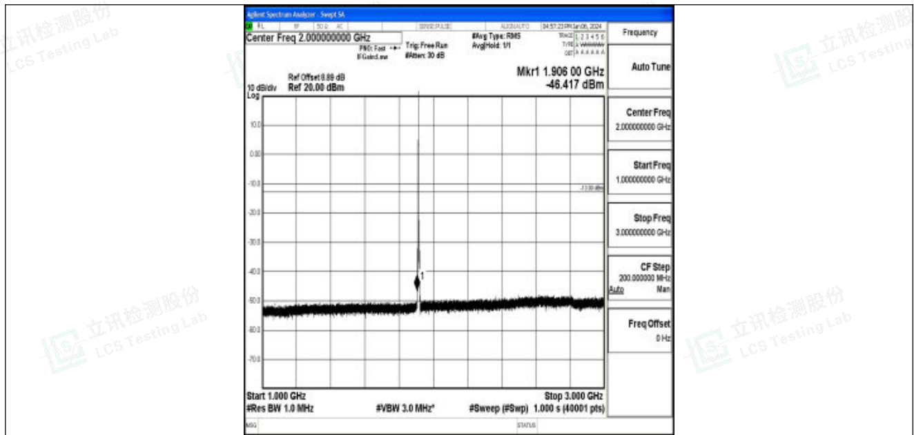
Band25_3MHz_QPSK_26675_1RB#0_1000~3000_1000~3000
