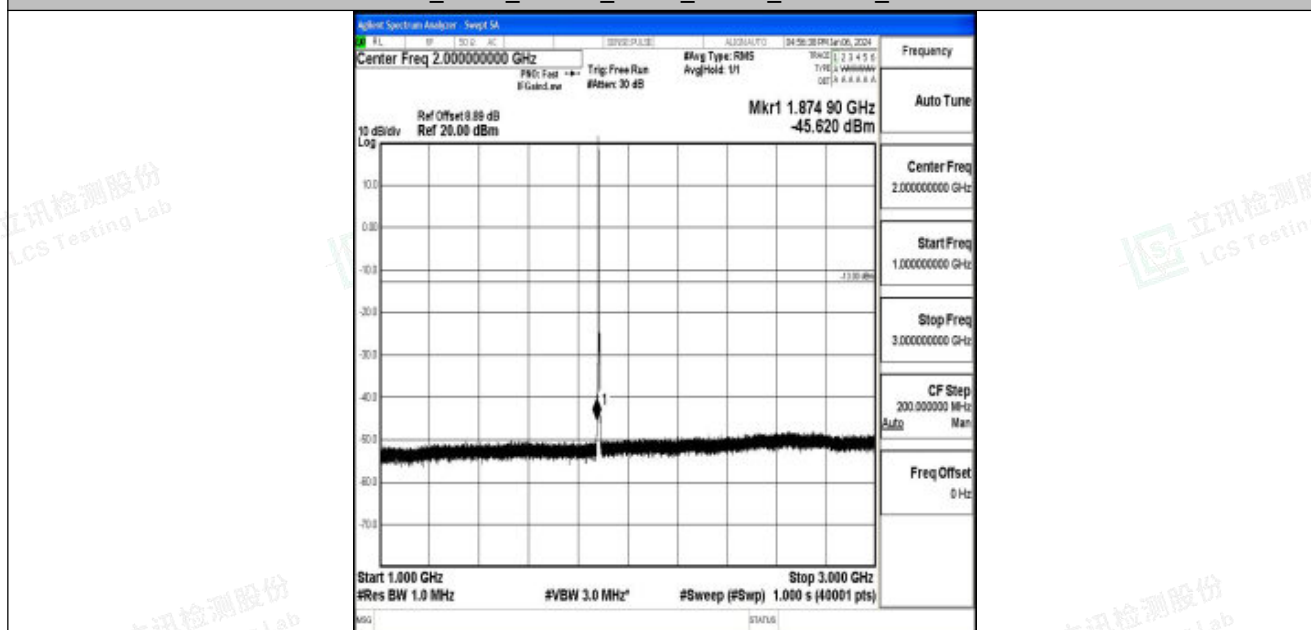
Band25_3MHz_16QAM_26365_1RB#0_1000~3000_1000~3000
