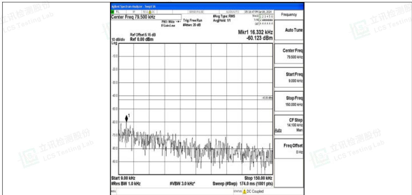
Band25_5MHz_16QAM_26665_1RB#0_0.009~0.15_0.009~0.15
