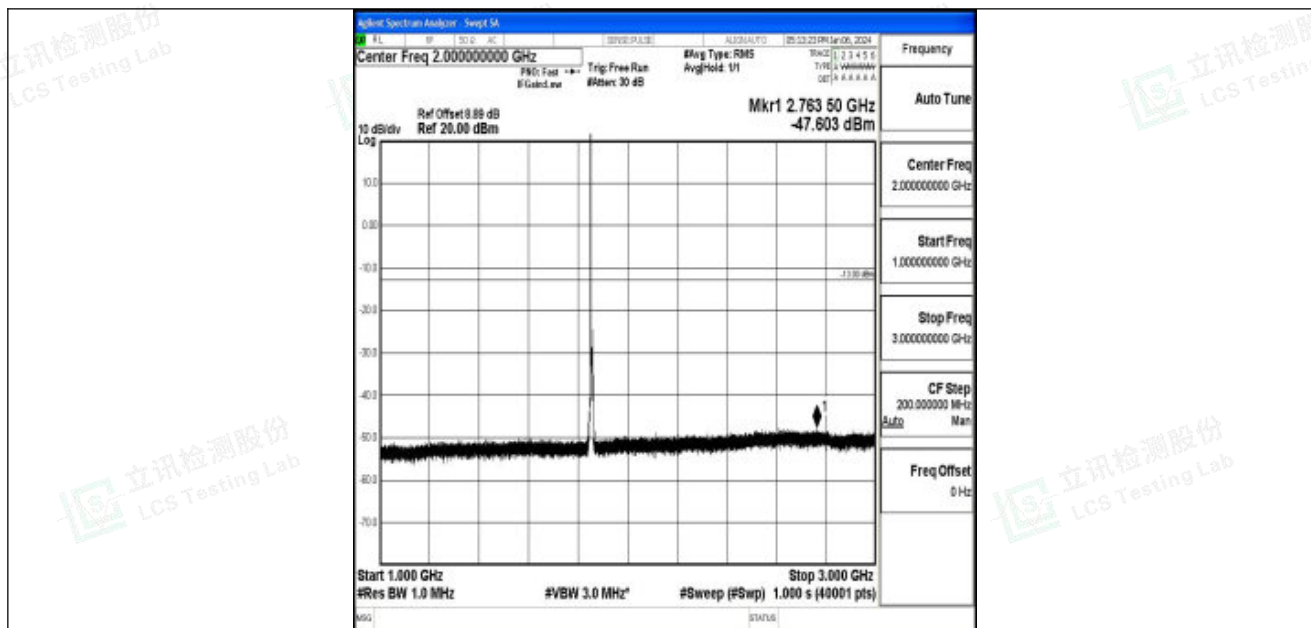
Band25_5MHz_QPSK_26065_1RB#0_1000~3000_1000~3000
