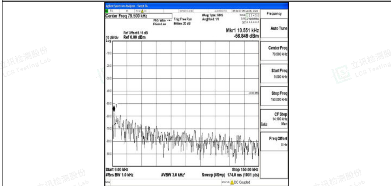
Band25_10MHz_QPSK_26365_1RB#0_0.009~0.15_0.009~0.15
