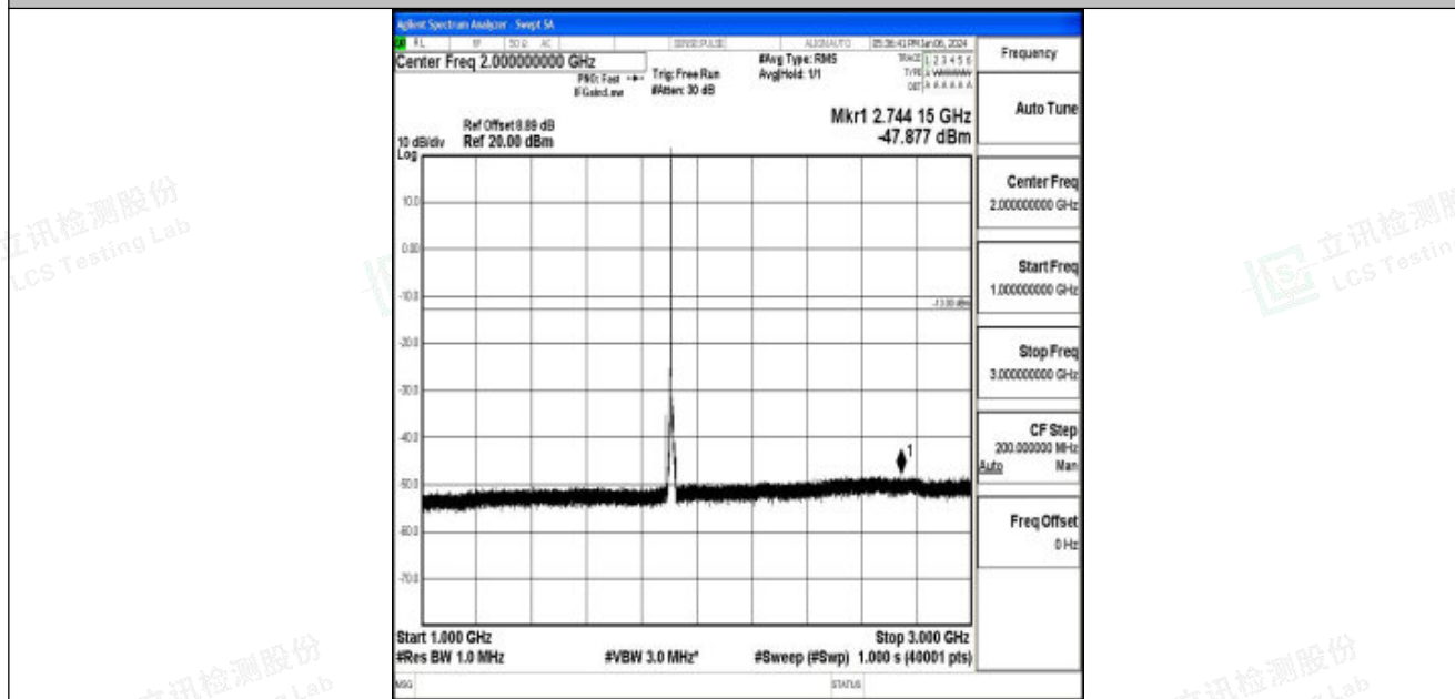
Band25_10MHz_16QAM_26640_1RB#0_1000~3000_1000~3000
