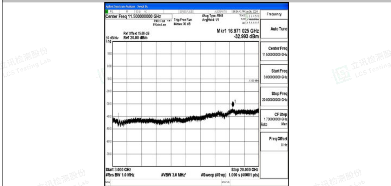
Band25_3MHz_QPSK_26055_1RB#0_3000~20000_3000~20000
