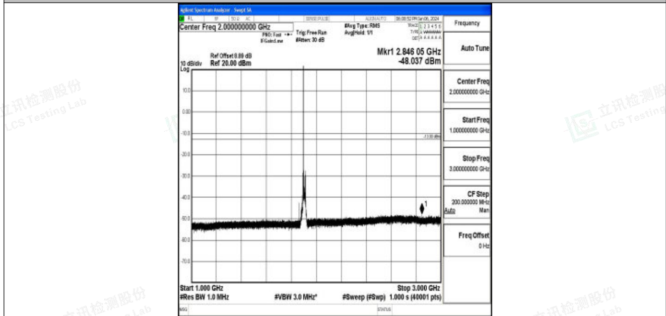
Band25_20MHz_16QAM_26590_1RB#0_1000~3000_1000~3000
