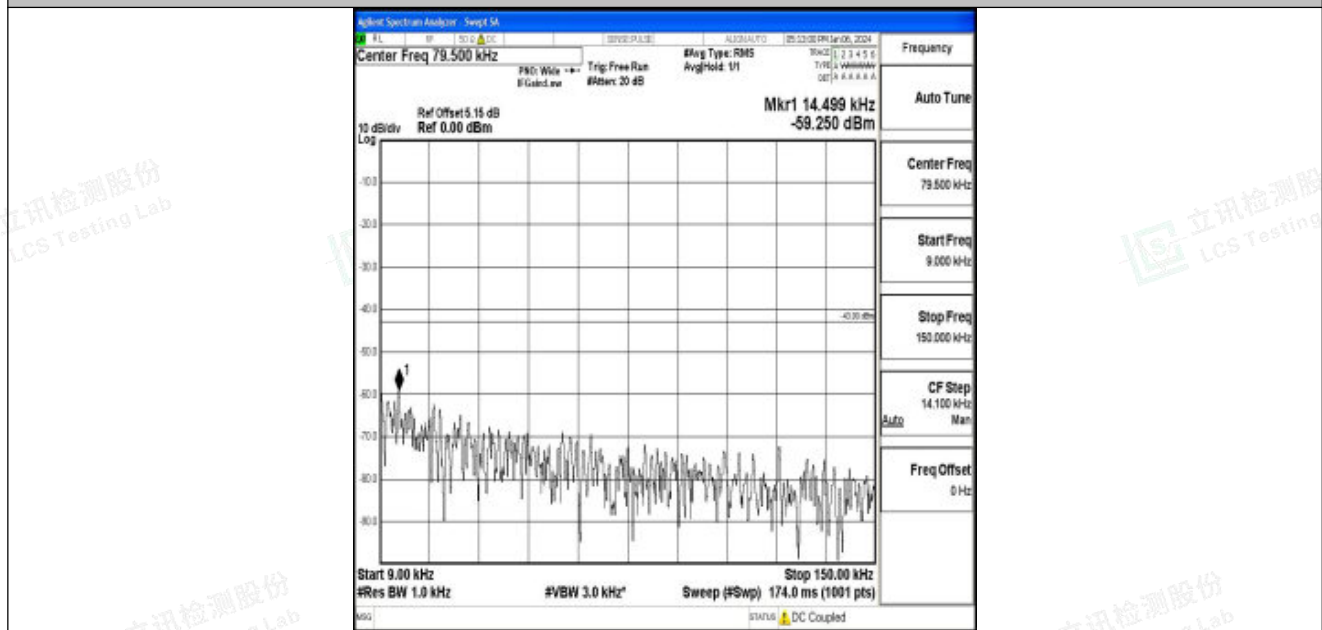
Band25_5MHz_QPSK_26065_1RB#0_0.009~0.15_0.009~0.15
