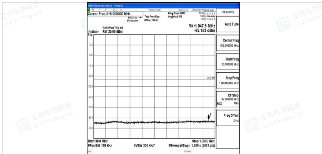
Band25_5MHz_16QAM_26665_1RB#0_30~1000_30~1000
