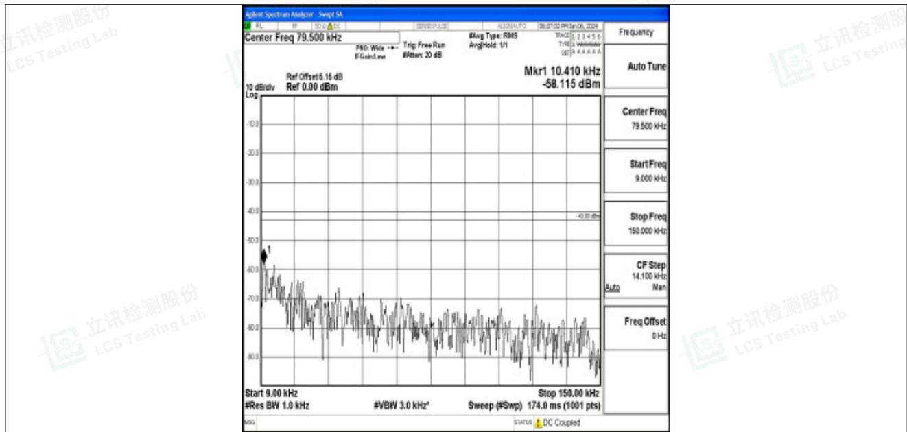
Band25_20MHz_16QAM_26365_1RB#0_0.009~0.15_0.009~0.15
