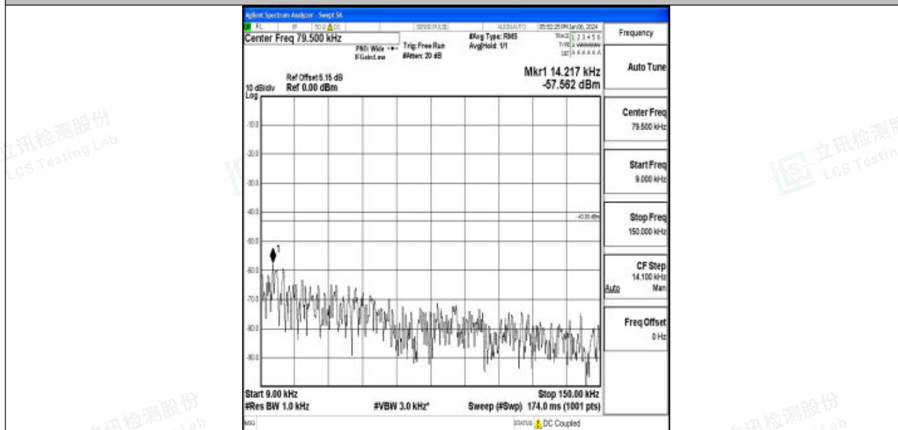
Band25_15MHz_QPSK_26615_1RB#0_0.009~0.15_0.009~0.15
