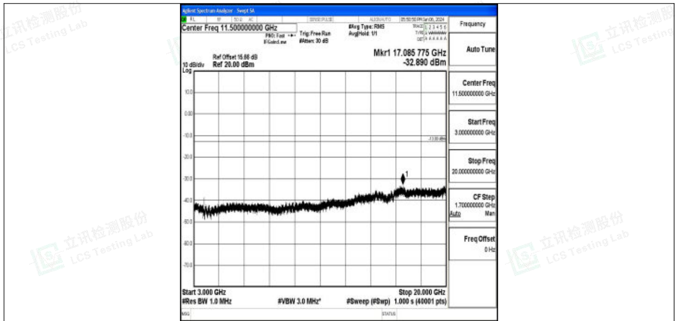
Band25_15MHz_16QAM_26115_1RB#0_3000~20000_3000~20000
