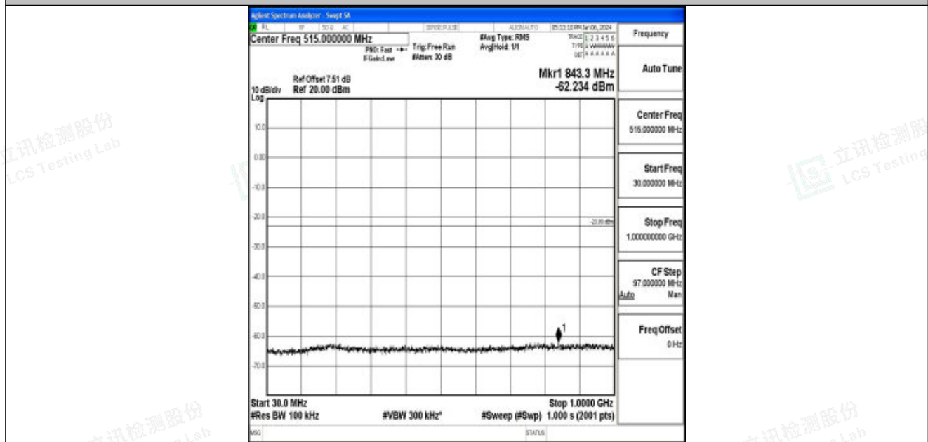
Band25_5MHz_QPSK_26065_1RB#0_30~1000_30~1000
