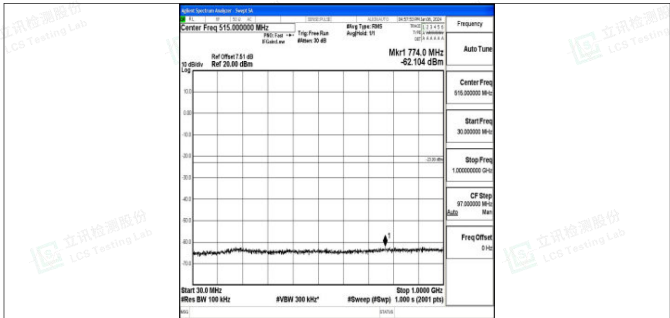
Band25_3MHz_16QAM_26675_1RB#0_30~1000_30~1000
