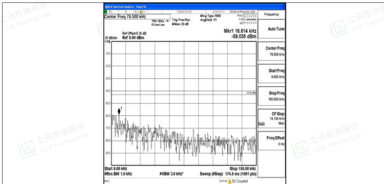
Band25_15MHz_16QAM_26115_1RB#0_0.009~0.15_0.009~0.15
