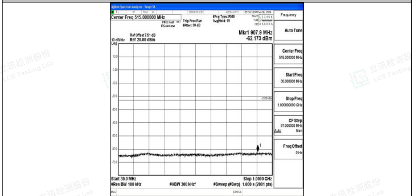
Band25_10MHz_QPSK_26365_1RB#0_30~1000_30~1000
