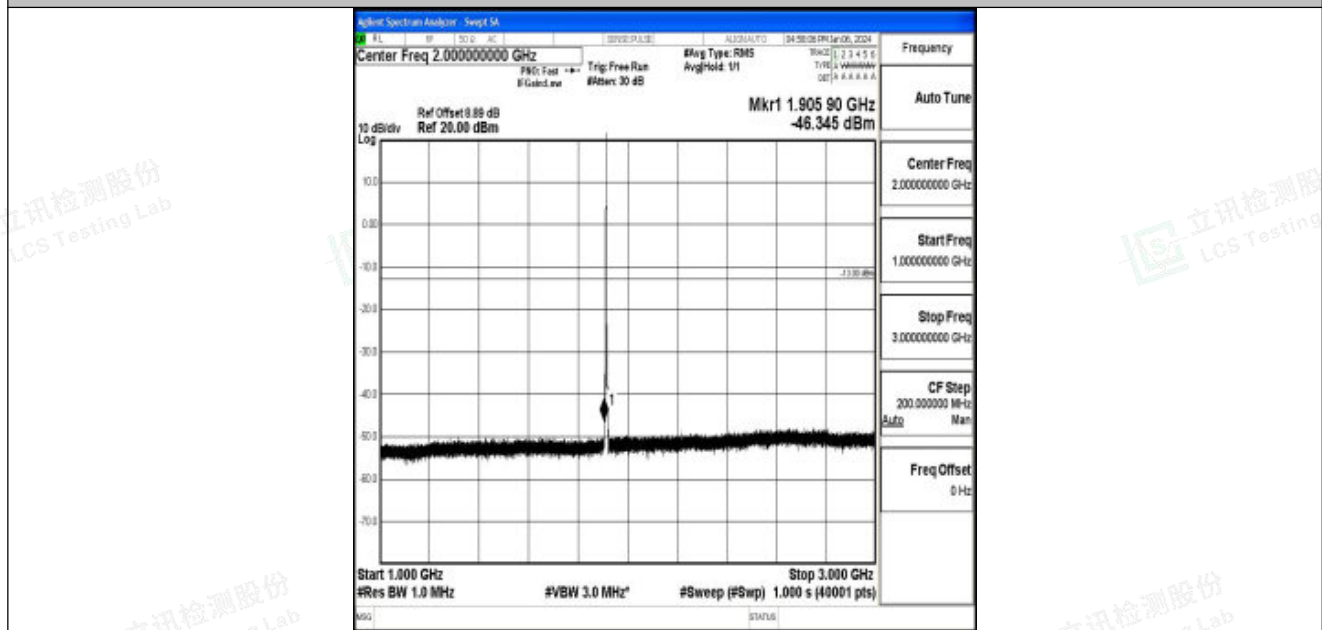
Band25_3MHz_16QAM_26675_1RB#0_1000~3000_1000~3000
