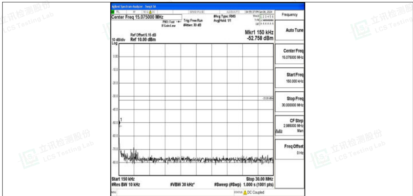
Band25_3MHz_QPSK_26365_1RB#0_0.15~30_0.15~30
