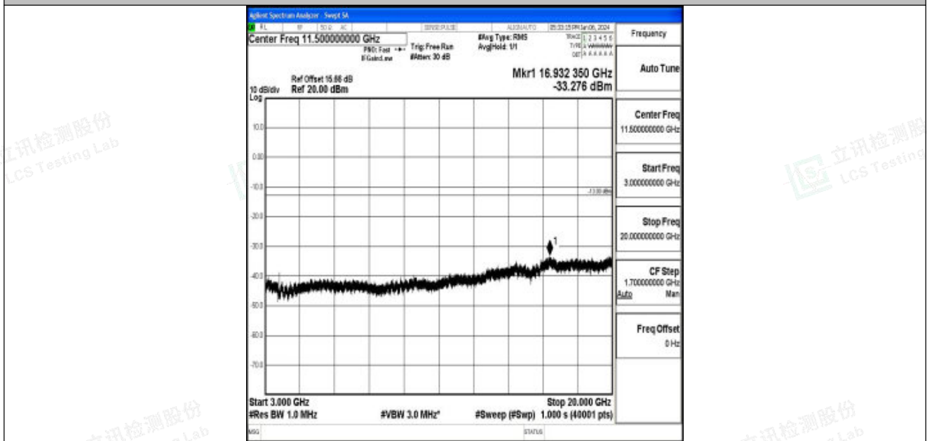
Band25_10MHz_QPSK_26090_1RB#0_3000~20000_3000~20000
