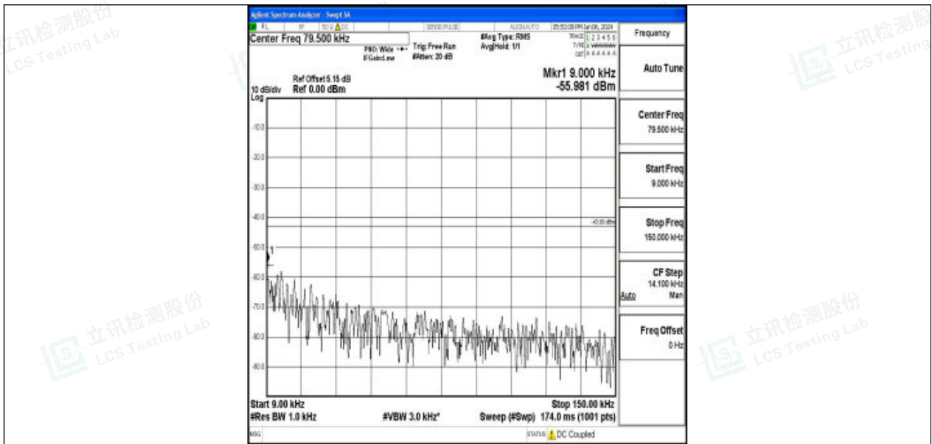
Band25_15MHz_16QAM_26615_1RB#0_0.009~0.15_0.009~0.15
