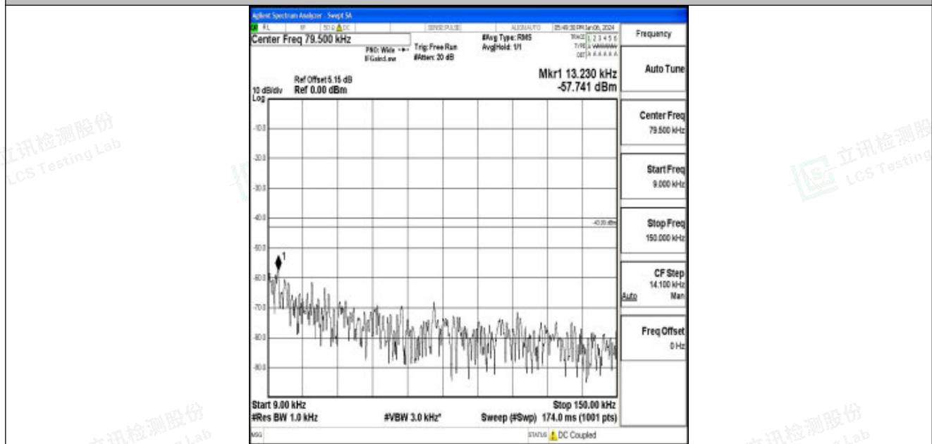
Band25_15MHz_QPSK_26115_1RB#0_0.009~0.15_0.009~0.15
