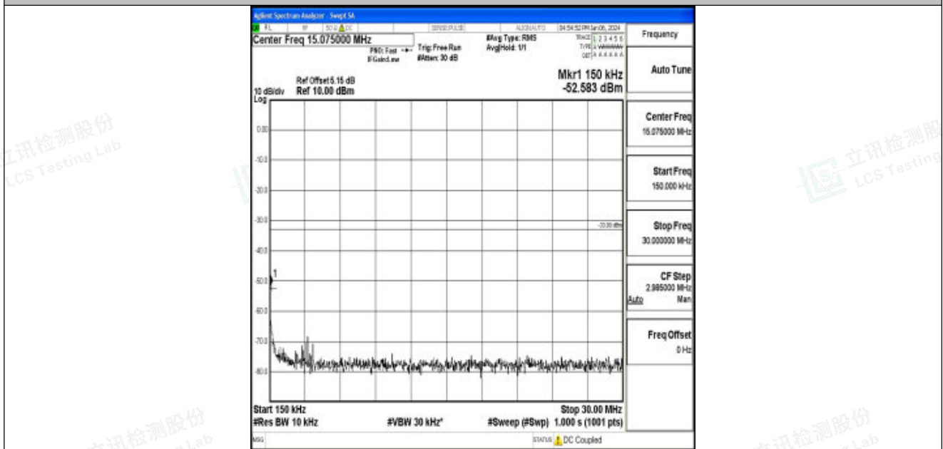
Band25_3MHz_16QAM_26055_1RB#0_0.15~30_0.15~30
