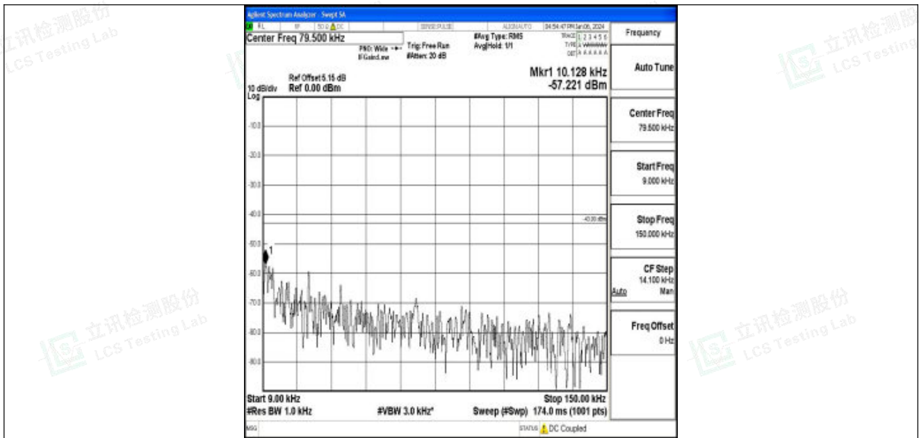
Band25_3MHz_16QAM_26055_1RB#0_0.009~0.15_0.009~0.15
