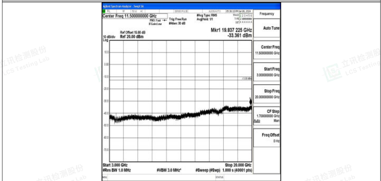
Band25_10MHz_QPSK_26640_1RB#0_3000~20000_3000~20000
