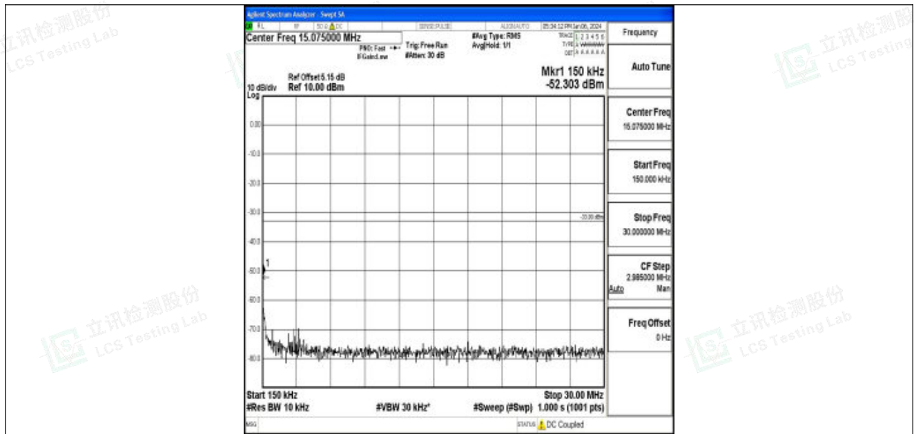
Band25_10MHz_QPSK_26365_1RB#0_0.15~30_0.15~30
