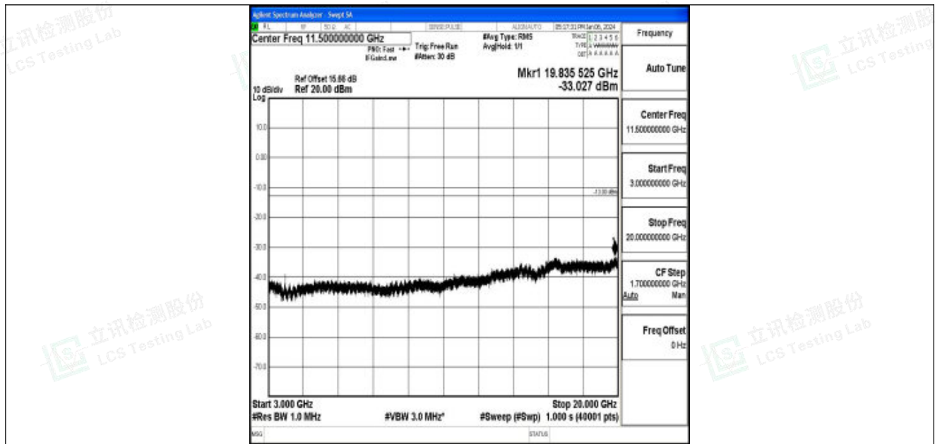
Band25_5MHz_16QAM_26665_1RB#0_3000~20000_3000~20000
