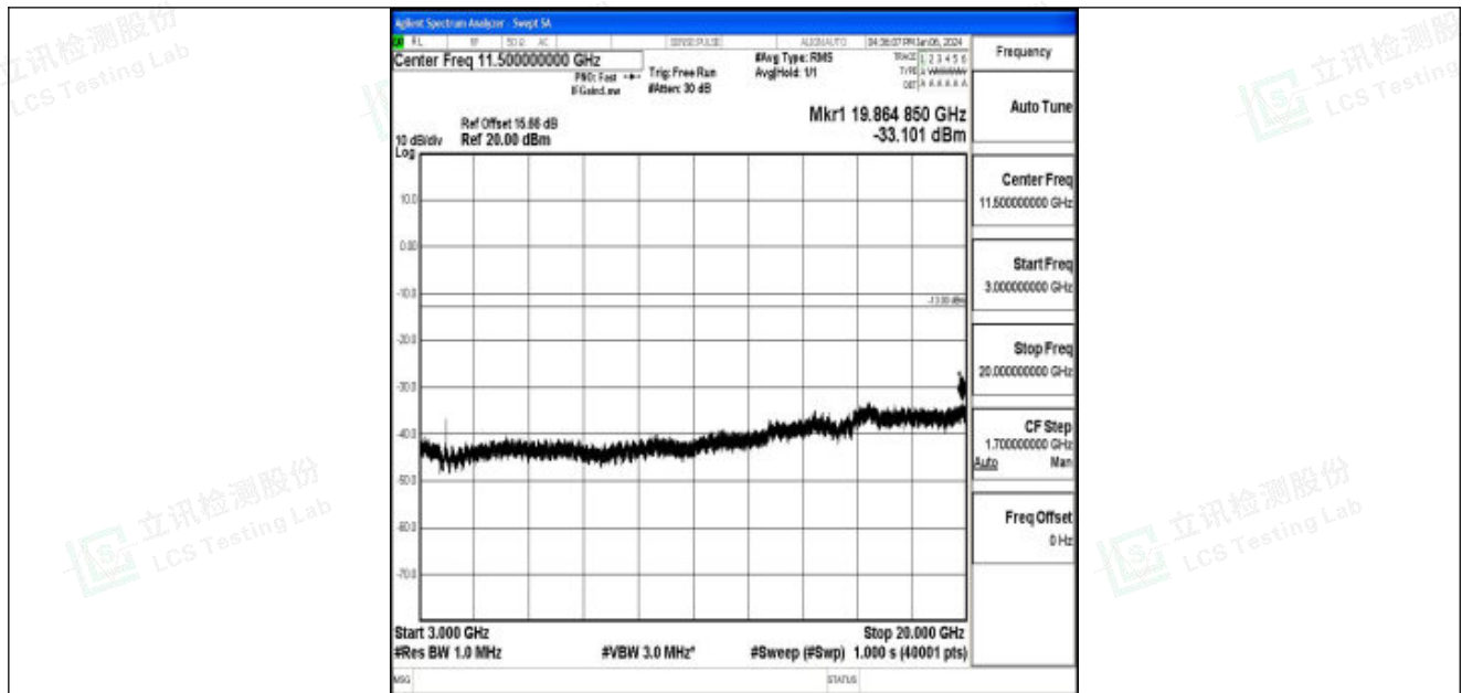
Band25_1.4MHz_16QAM_26683_1RB#0_3000~20000_3000~20000
