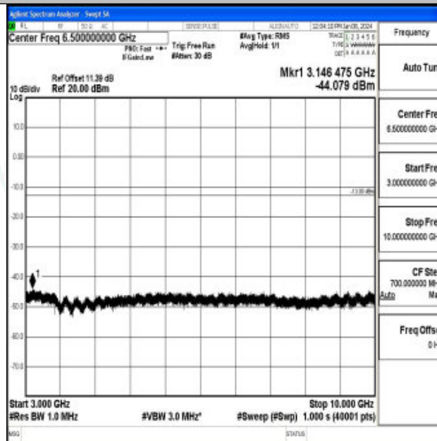
Band26_1.4MHz_16QAM_26697_1RB#0_3000~10000_3000~10000
