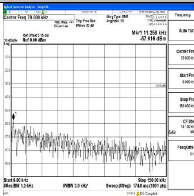
Band26_1.4MHz_16QAM_26740_1RB#0_0.009~0.15_0.009~0.15
