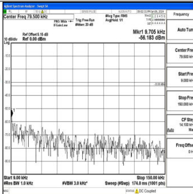
Band26_5MHz_16QAM_26740_1RB#0_0.009~0.15_0.009~0.15
