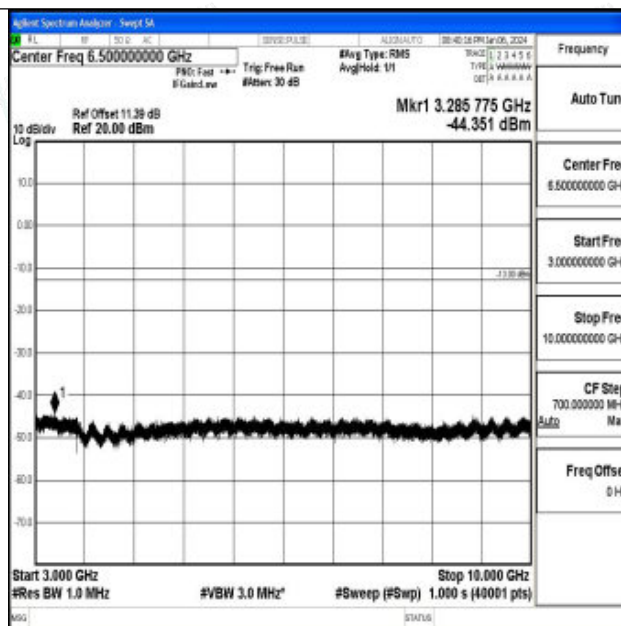
Band26_3MHz_QPSK_26705_1RB#0_3000~10000_3000~10000
