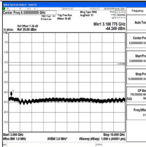
Band26_3MHz_16QAM_26705_1RB#0_3000~10000_3000~10000
