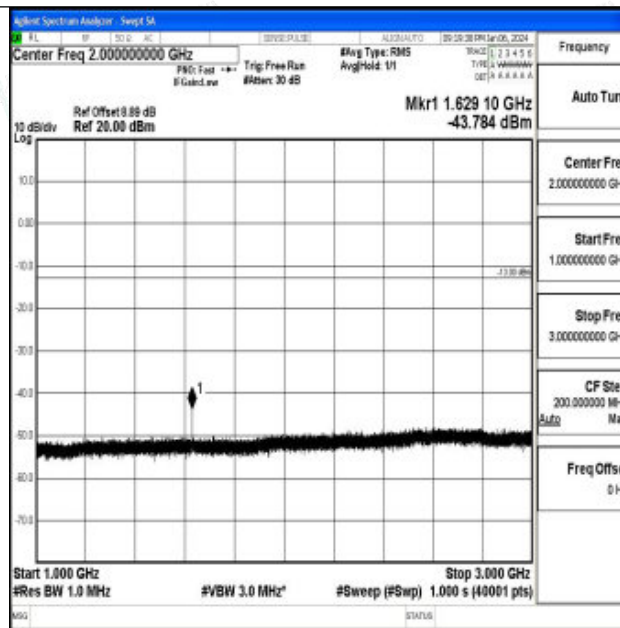
Band26_10MHz_16QAM_26740_1RB#0_1000~3000_1000~3000
