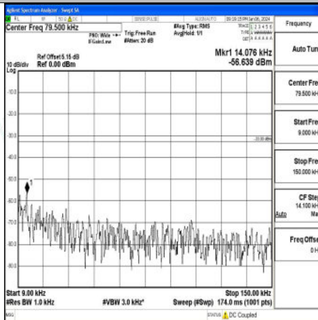
Band26_10MHz_16QAM_26740_1RB#0_0.009~0.15_0.009~0.15
