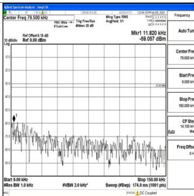
Band26_1.4MHz_QPSK_26740_1RB#0_0.009~0.15_0.009~0.15
