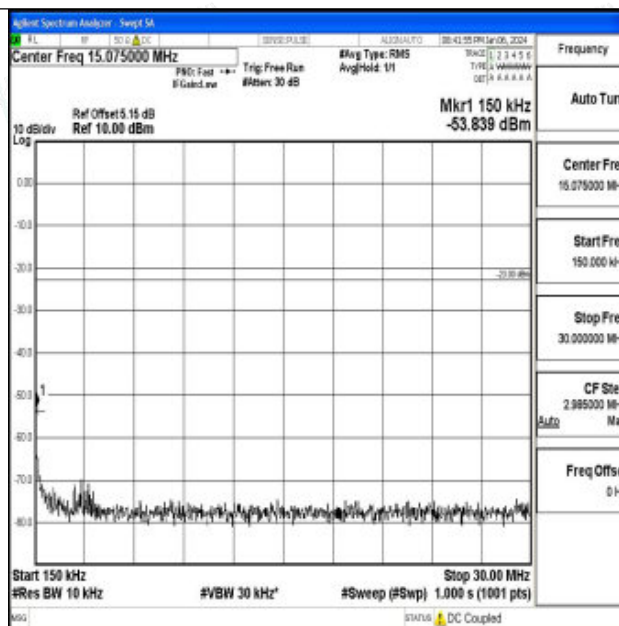
Band26_3MHz_16QAM_26740_1RB#0_0.15~30_0.15~30
