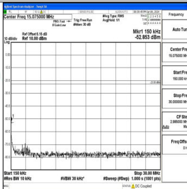
Band26_3MHz_QPSK_26705_1RB#0_0.15~30_0.15~30
