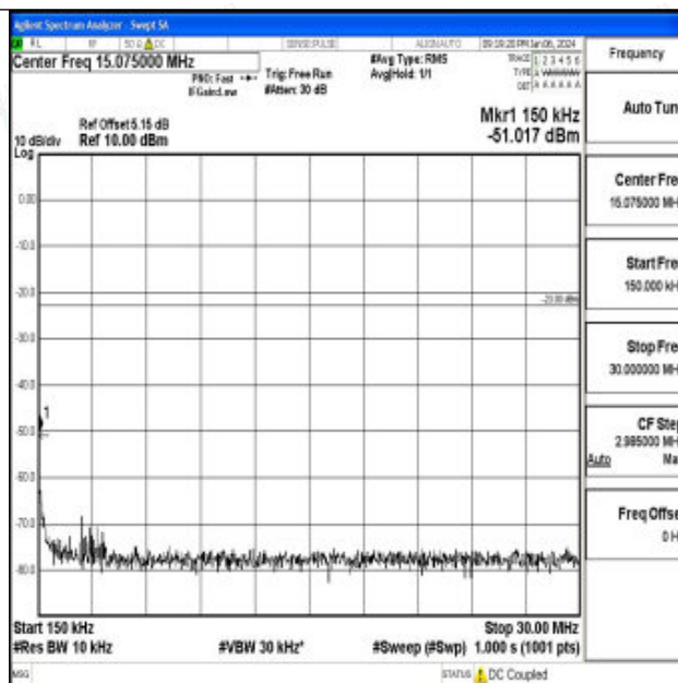
Band26_10MHz_16QAM_26740_1RB#0_0.15~30_0.15~30
