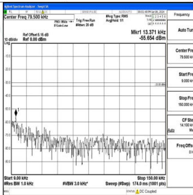
Band26_5MHz_QPSK_26740_1RB#0_0.009~0.15_0.009~0.15
