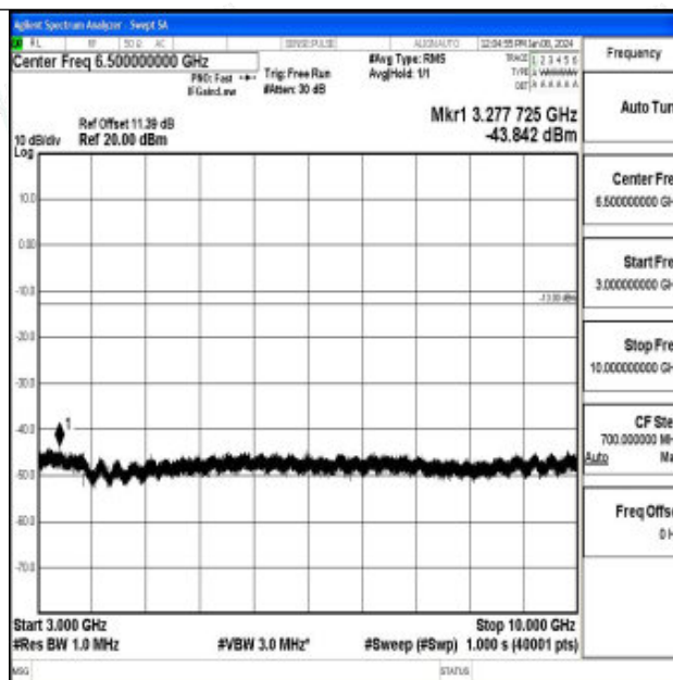
Band26_1.4MHz_QPSK_26740_1RB#0_3000~10000_3000~10000
