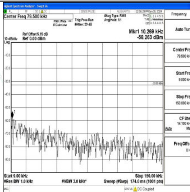
Band26_1.4MHz_16QAM_26783_1RB#0_0.009~0.15_0.009~0.15
