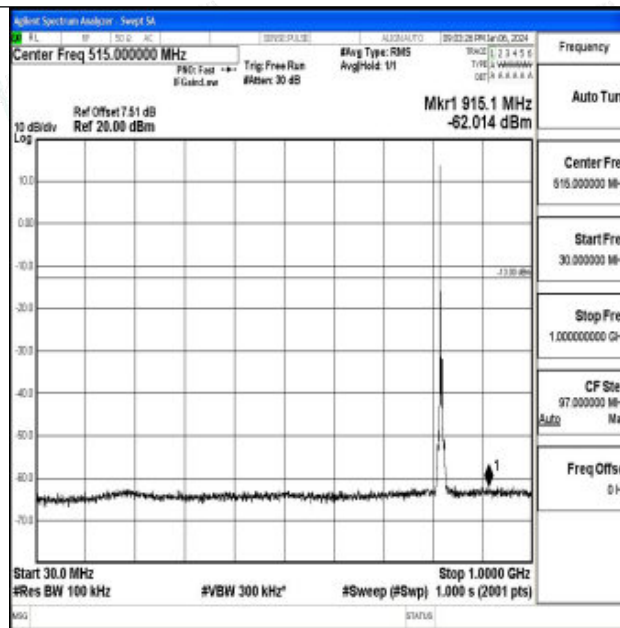
Band26_5MHz_QPSK_26765_1RB#0_30~1000_30~1000
