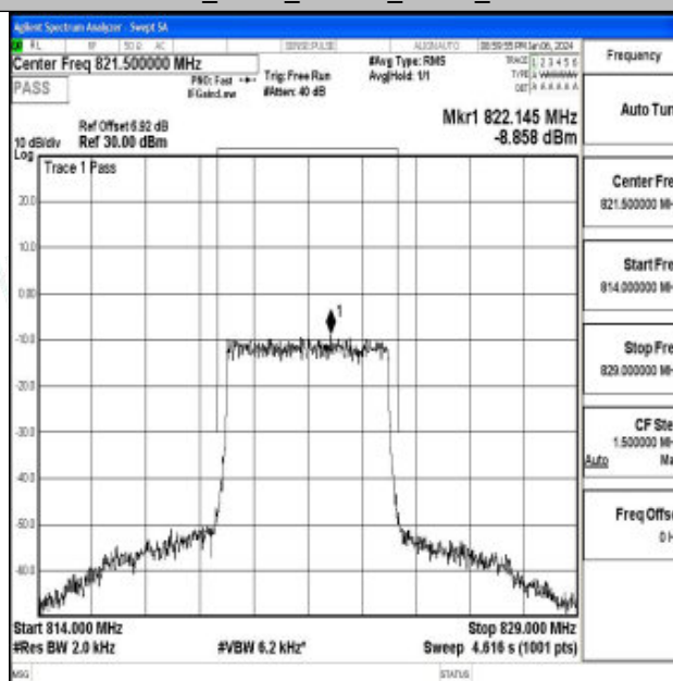
Band26_5MHz_QPSK_26765_25RB#0
