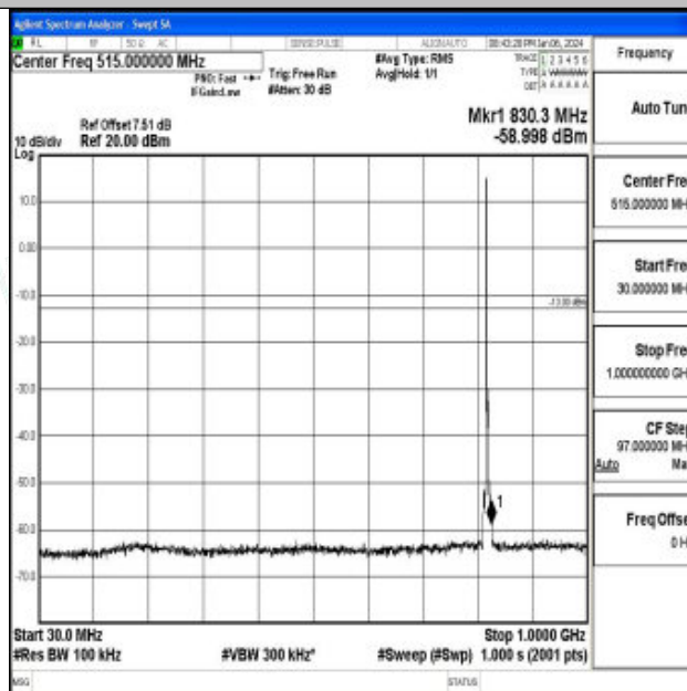
Band26_3MHz_16QAM_26775_1RB#0_30~1000_30~1000
