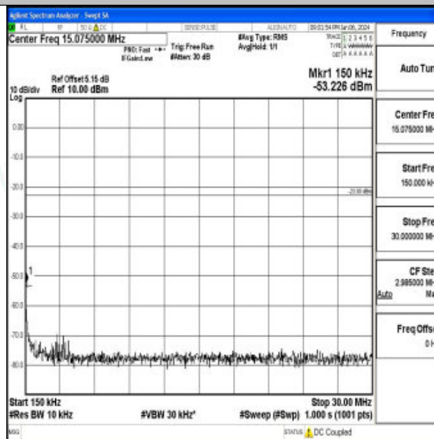
Band26_5MHz_QPSK_26740_1RB#0_0.15~30_0.15~30
