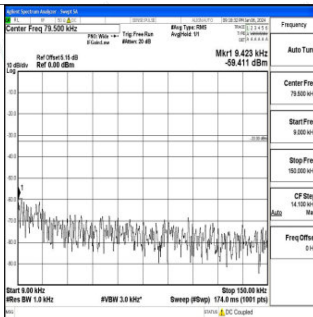
Band26_10MHz_QPSK_26740_1RB#0_0.009~0.15_0.009~0.15
