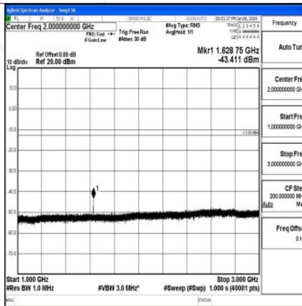
Band26_5MHz_16QAM_26715_1RB#0_1000~3000_1000~3000
