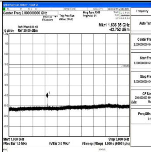
Band26_1.4MHz_QPSK_26740_1RB#0_1000~3000_1000~3000
