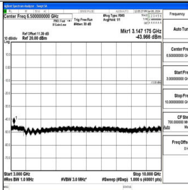
Band26_1.4MHz_16QAM_26740_1RB#0_3000~10000_3000~10000
