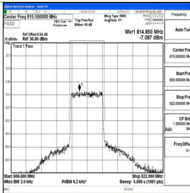
Band26_3MHz_QPSK_26705_15RB#0
