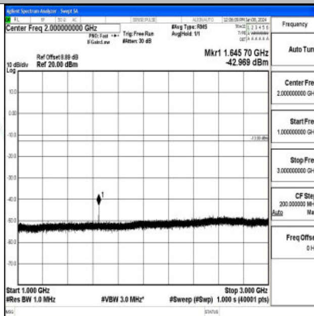
Band26_1.4MHz_QPSK_26783_1RB#0_1000~3000_1000~3000
