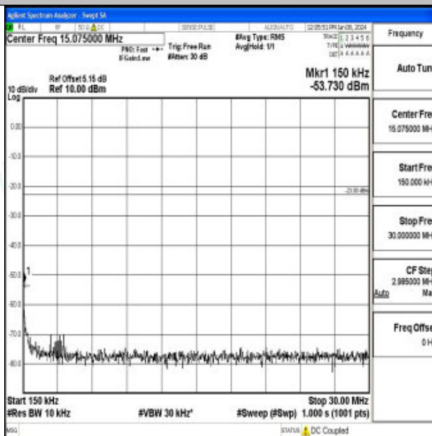
Band26_1.4MHz_QPSK_26783_1RB#0_0.15~30_0.15~30
