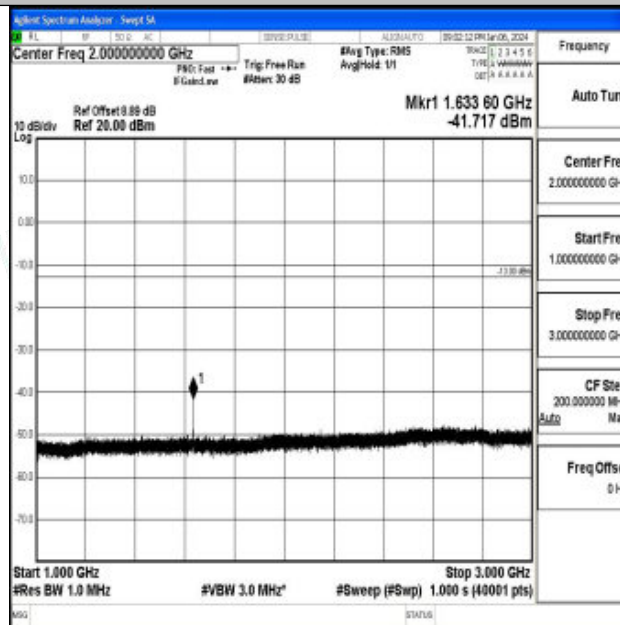
Band26_5MHz_QPSK_26740_1RB#0_1000~3000_1000~3000
