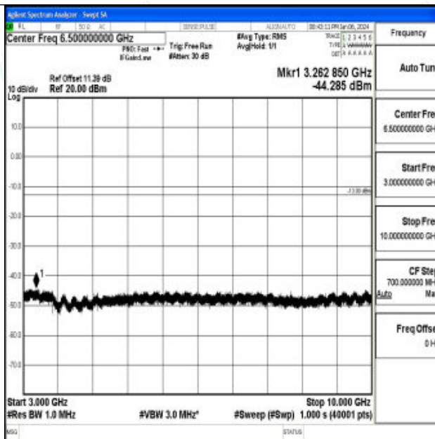
Band26_3MHz_QPSK_26775_1RB#0_3000~10000_3000~10000
