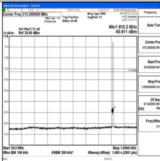
Band26_1.4MHz_16QAM_26740_1RB#0_30~1000_30~1000
