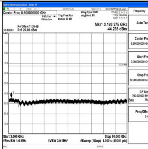
Band26_10MHz_16QAM_26740_1RB#0_3000~10000_3000~10000
