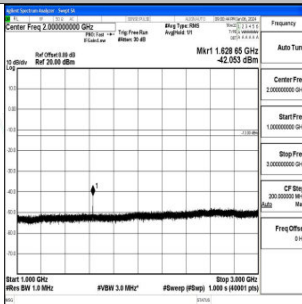
Band26_5MHz_QPSK_26715_1RB#0_1000~3000_1000~3000
