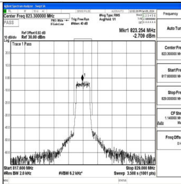
Band26_1.4MHz_QPSK_26783_6RB#0
