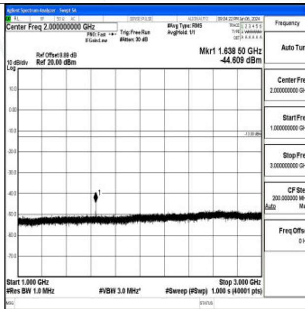
Band26_5MHz_16QAM_26765_1RB#0_1000~3000_1000~3000
