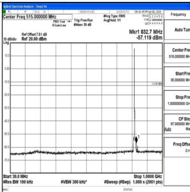
Band26_3MHz_QPSK_26775_1RB#0_30~1000_30~1000
