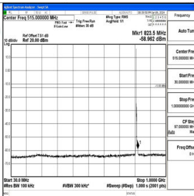
Band26_3MHz_QPSK_26705_1RB#0_30~1000_30~1000
