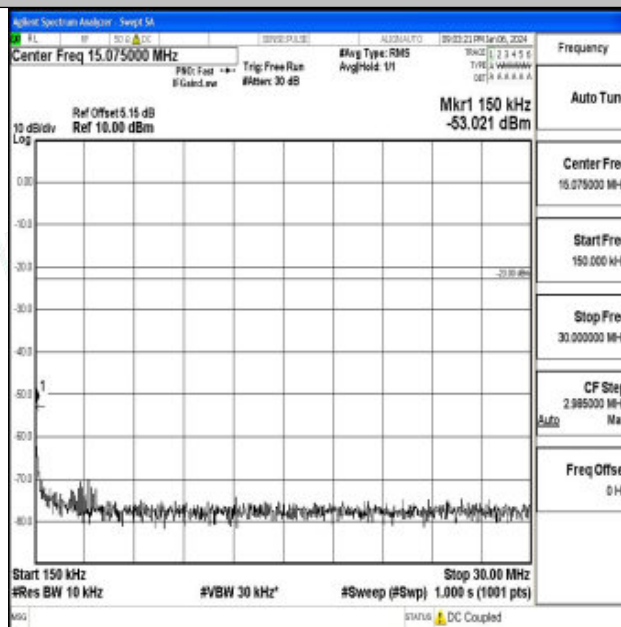
Band26_5MHz_QPSK_26765_1RB#0_0.15~30_0.15~30
