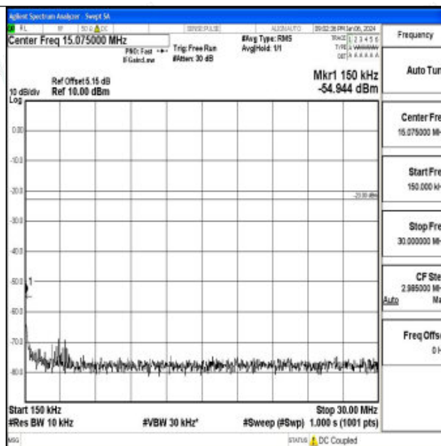
Band26_5MHz_16QAM_26740_1RB#0_0.15~30_0.15~30
