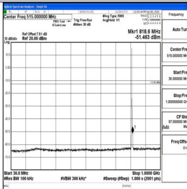
Band26_1.4MHz_16QAM_26697_1RB#0_30~1000_30~1000
