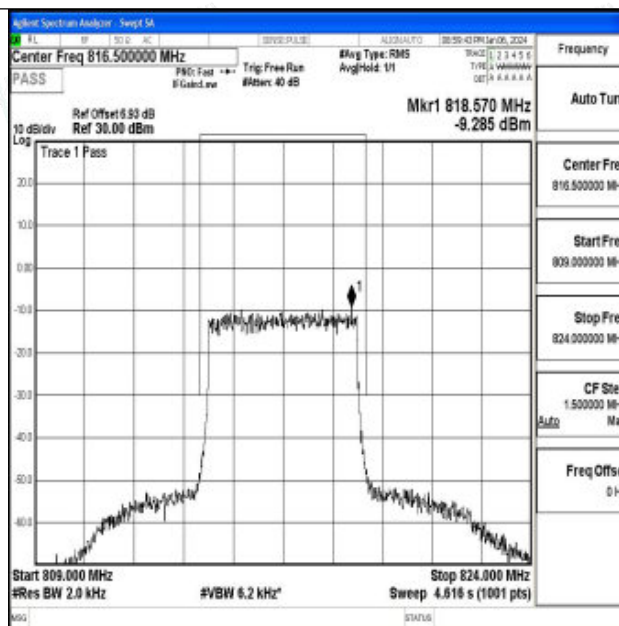
Band26_5MHz_16QAM_26715_25RB#0
