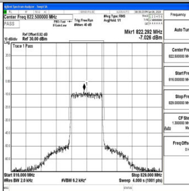
Band26_3MHz_16QAM_26775_15RB#0
