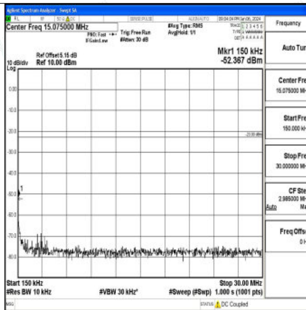
Band26_5MHz_16QAM_26765_1RB#0_0.15~30_0.15~30
