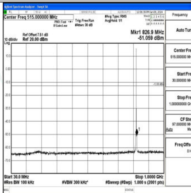
Band26_1.4MHz_16QAM_26783_1RB#0_30~1000_30~1000
