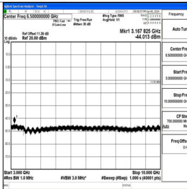
Band26_5MHz_QPSK_26715_1RB#0_3000~10000_3000~10000
