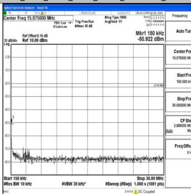
Band26_3MHz_QPSK_26740_1RB#0_0.15~30_0.15~30
