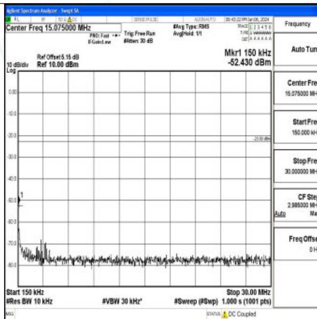
Band26_3MHz_16QAM_26775_1RB#0_0.15~30_0.15~30
