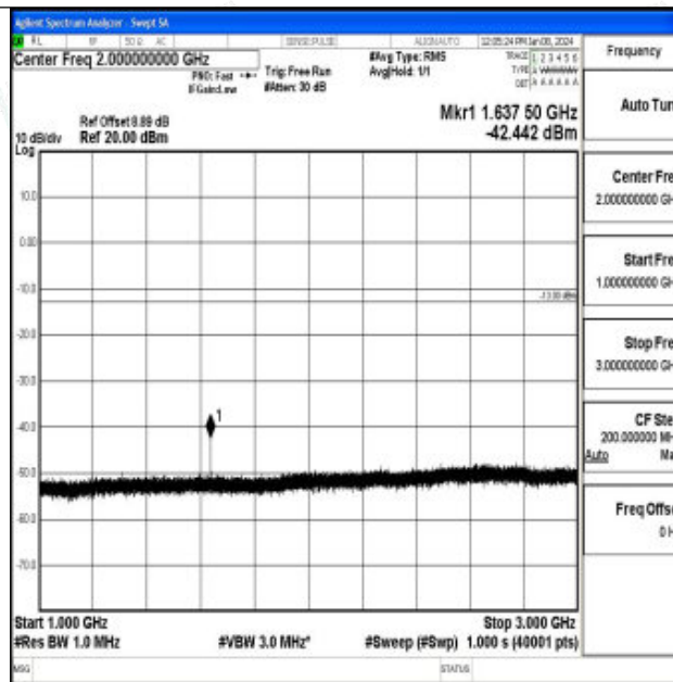
Band26_1.4MHz_16QAM_26740_1RB#0_1000~3000_1000~3000
