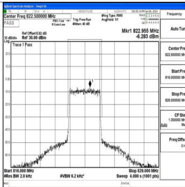
Band26_3MHz_QPSK_26775_15RB#0
