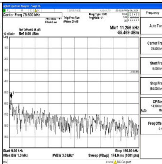
Band26_3MHz_QPSK_26740_1RB#0_0.009~0.15_0.009~0.15
