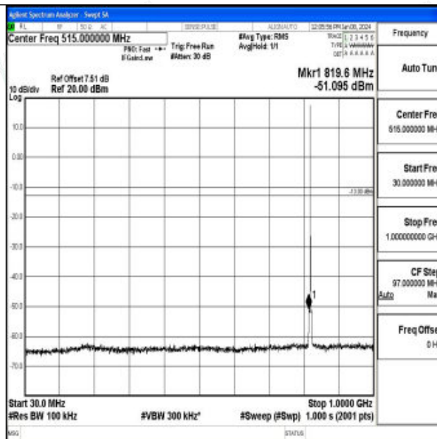
Band26_1.4MHz_QPSK_26783_1RB#0_30~1000_30~1000
