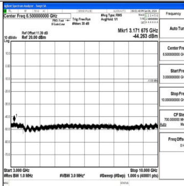
Band26_5MHz_16QAM_26715_1RB#0_3000~10000_3000~10000
