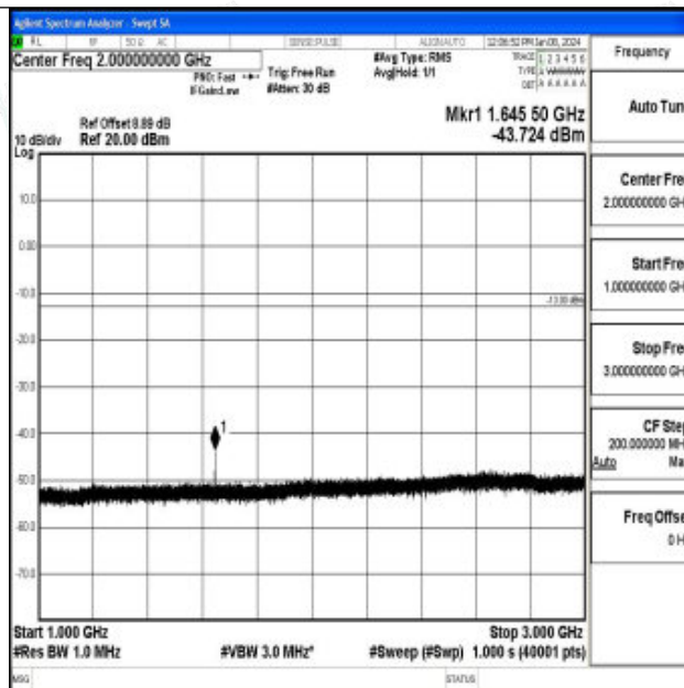
Band26_1.4MHz_16QAM_26783_1RB#0_1000~3000_1000~3000
