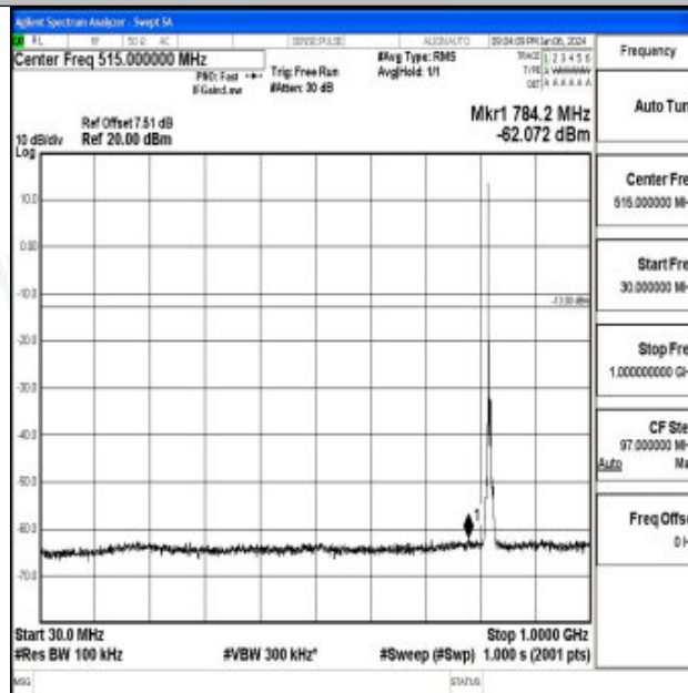
Band26_5MHz_16QAM_26765_1RB#0_30~1000_30~1000
