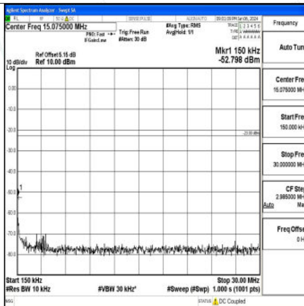
Band26_5MHz_16QAM_26715_1RB#0_0.15~30_0.15~30
