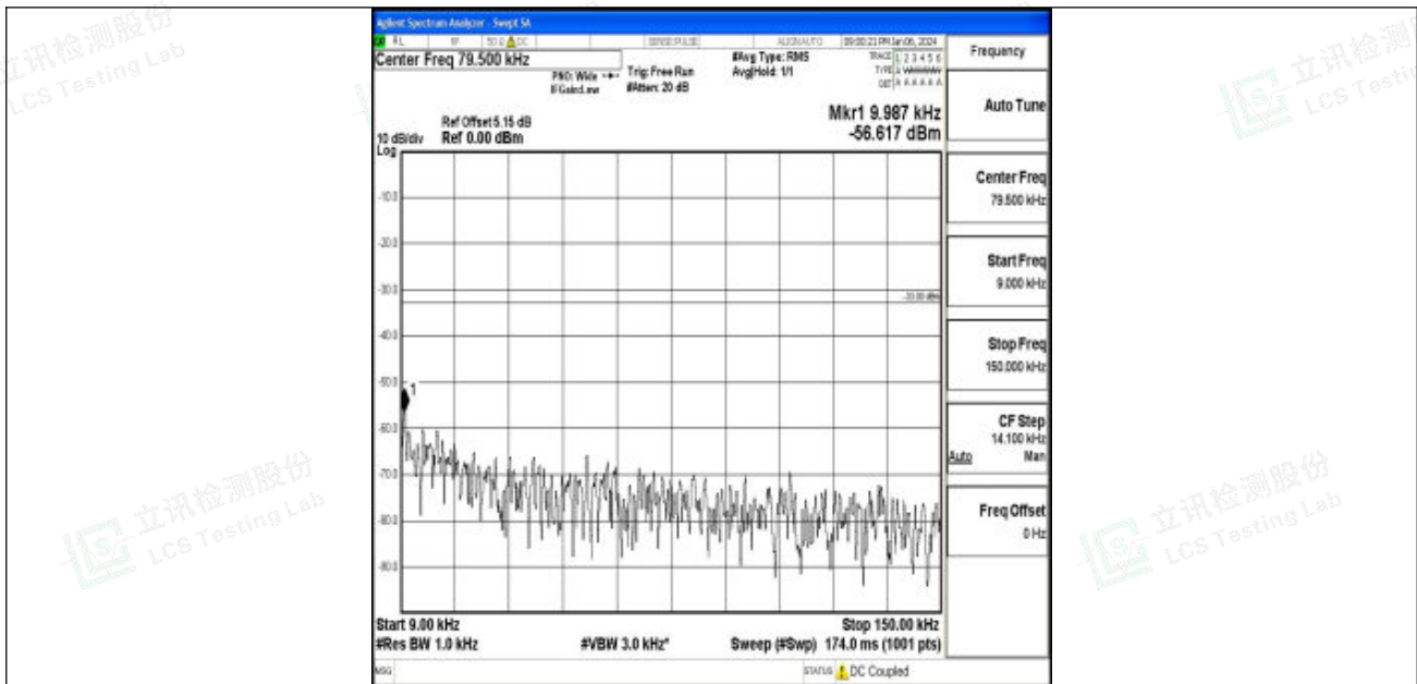
Band26_5MHz_QPSK_26715_1RB#0_0.009~0.15_0.009~0.15
