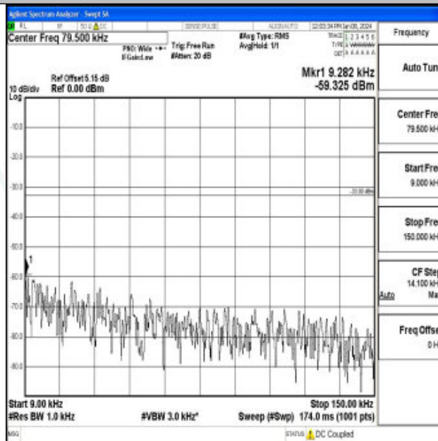
Band26_1.4MHz_16QAM_26697_1RB#0_0.009~0.15_0.009~0.15
