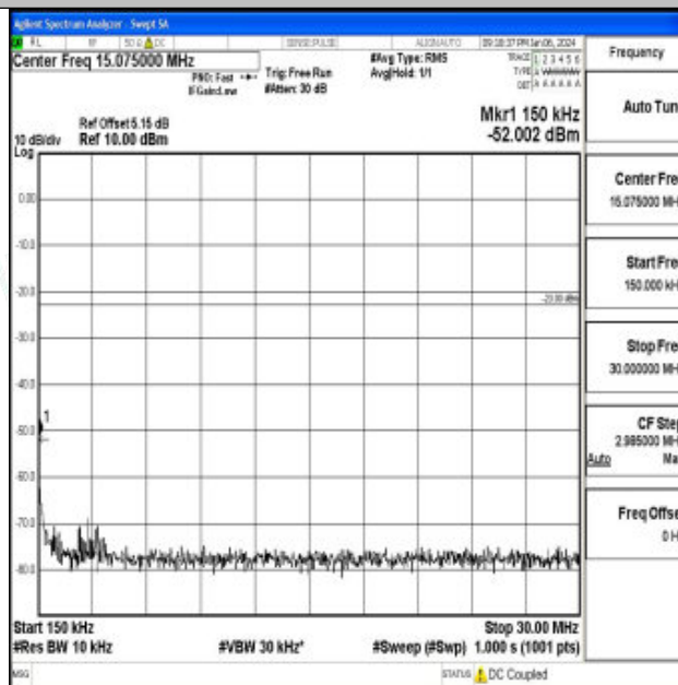
Band26_10MHz_QPSK_26740_1RB#0_0.15~30_0.15~30
