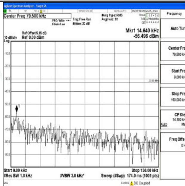
Band26_5MHz_16QAM_26765_1RB#0_0.009~0.15_0.009~0.15
