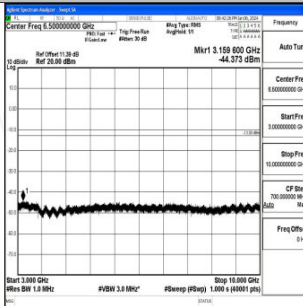
Band26_3MHz_16QAM_26740_1RB#0_3000~10000_3000~10000
