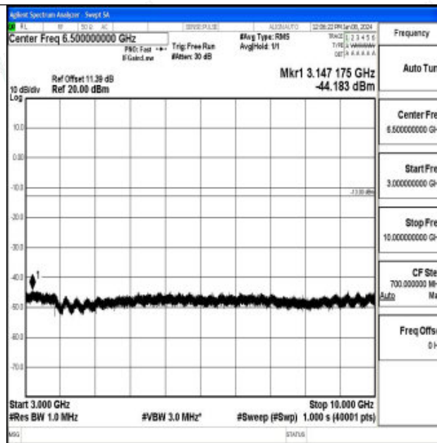
Band26_1.4MHz_QPSK_26783_1RB#0_3000~10000_3000~10000
