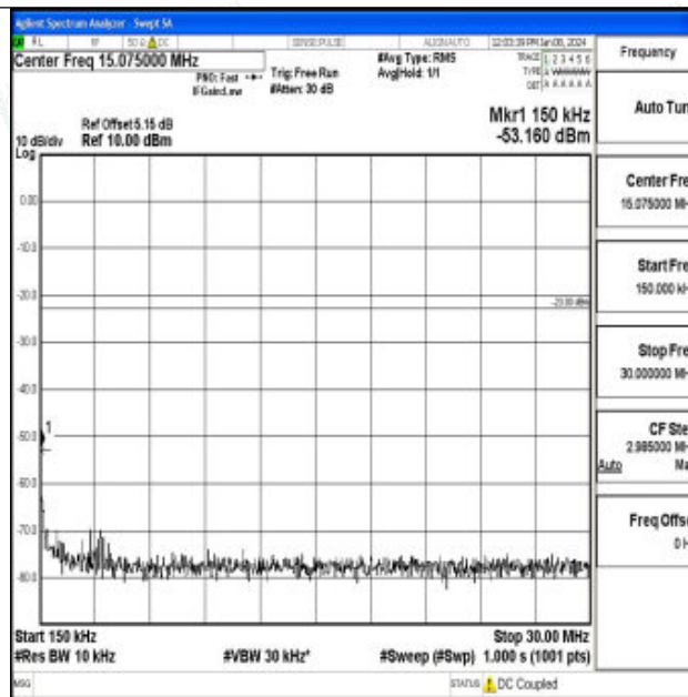
Band26_1.4MHz_16QAM_26697_1RB#0_0.15~30_0.15~30
