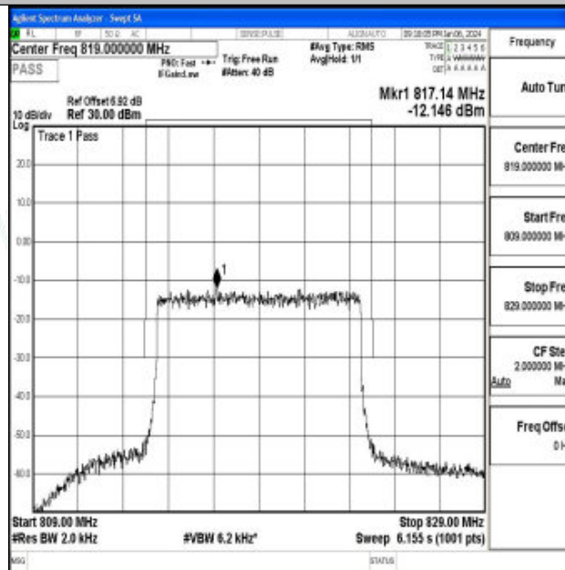
Band26_10MHz_QPSK_26740_50RB#0
