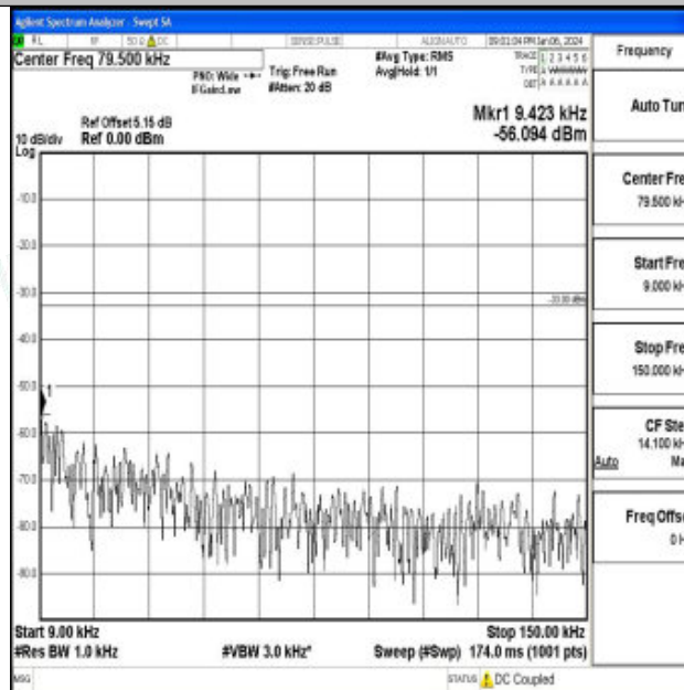
Band26_5MHz_16QAM_26715_1RB#0_0.009~0.15_0.009~0.15
