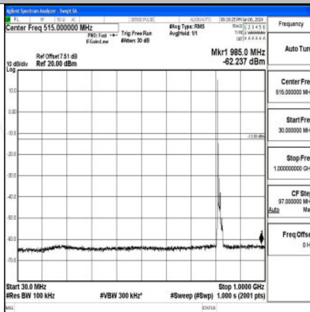
Band26_10MHz_16QAM_26740_1RB#0_30~1000_30~1000
