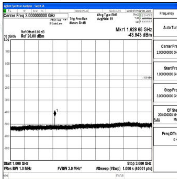
Band26_1.4MHz_16QAM_26697_1RB#0_1000~3000_1000~3000
