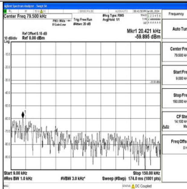
Band26_3MHz_16QAM_26740_1RB#0_0.009~0.15_0.009~0.15
