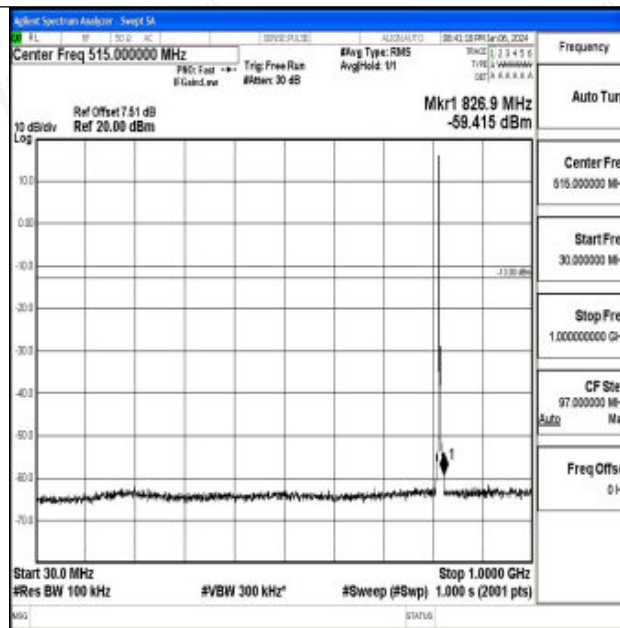
Band26_3MHz_QPSK_26740_1RB#0_30~1000_30~1000
