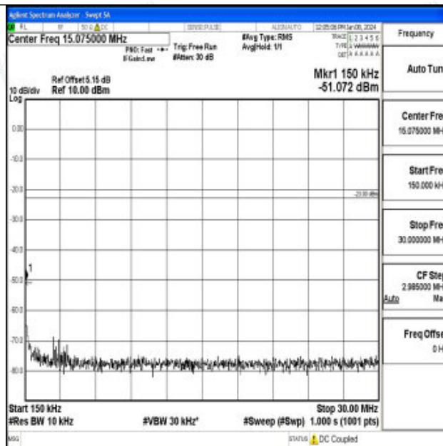
Band26_1.4MHz_16QAM_26740_1RB#0_0.15~30_0.15~30
