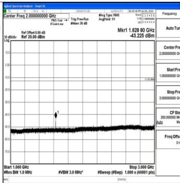
Band26_3MHz_16QAM_26705_1RB#0_1000~3000_1000~3000
