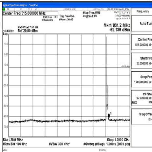
Band26_5MHz_QPSK_26715_1RB#0_30~1000_30~1000
