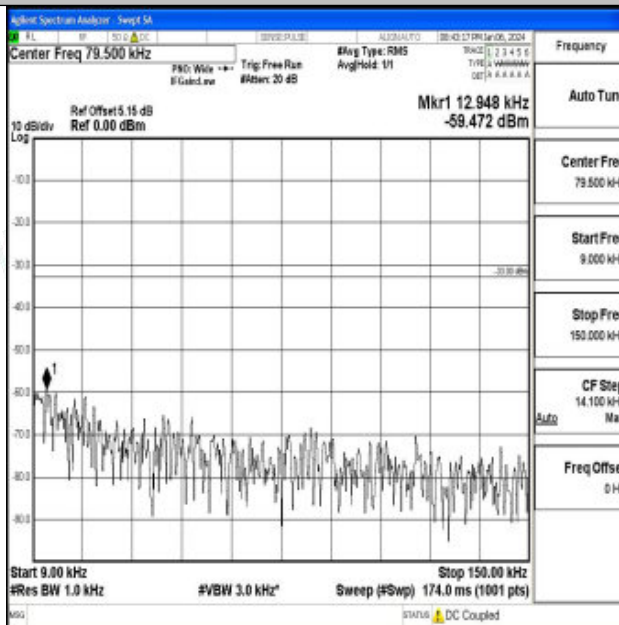
Band26_3MHz_16QAM_26775_1RB#0_0.009~0.15_0.009~0.15
