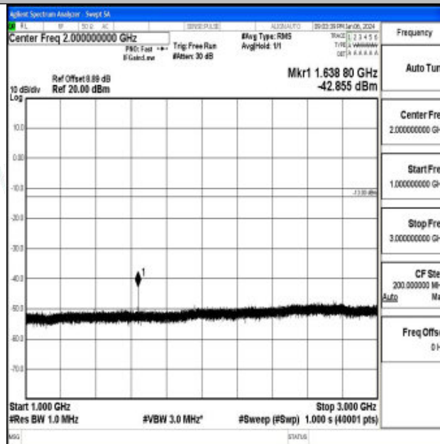
Band26_5MHz_QPSK_26765_1RB#0_1000~3000_1000~3000
