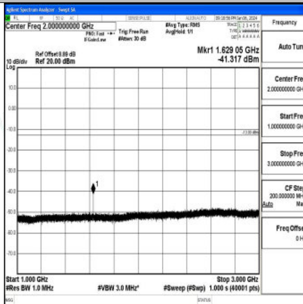
Band26_10MHz_QPSK_26740_1RB#0_1000~3000_1000~3000
