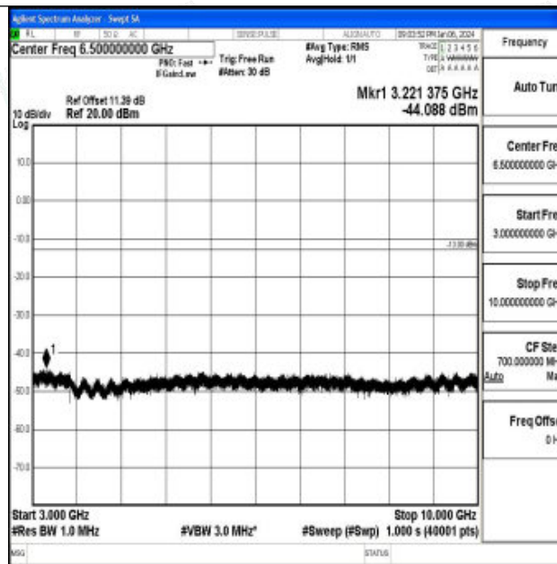
Band26_5MHz_QPSK_26765_1RB#0_3000~10000_3000~10000
