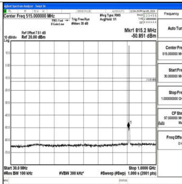
Band26_1.4MHz_QPSK_26740_1RB#0_30~1000_30~1000
