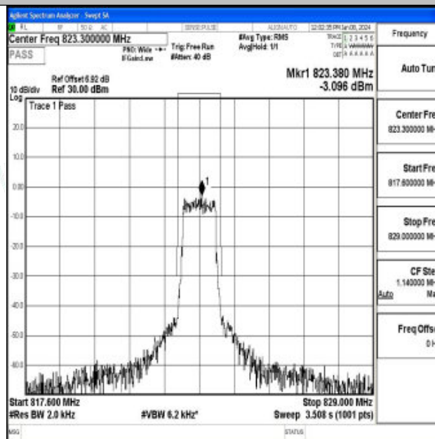
Band26_1.4MHz_16QAM_26783_6RB#0
