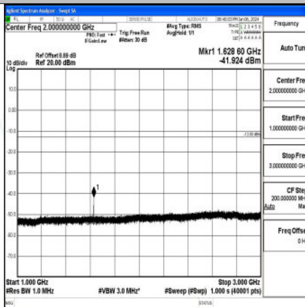
Band26_3MHz_QPSK_26705_1RB#0_1000~3000_1000~3000
