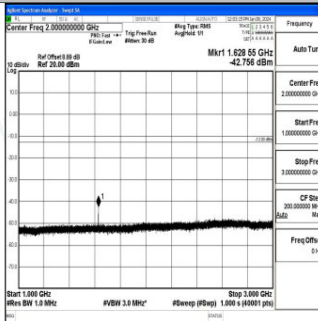
Band26_1.4MHz_QPSK_26697_1RB#0_1000~3000_1000~3000
