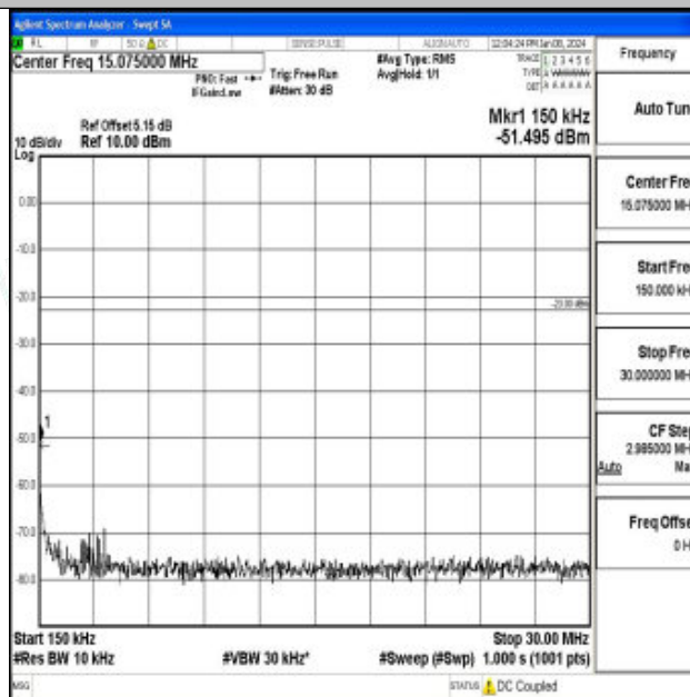
Band26_1.4MHz_QPSK_26740_1RB#0_0.15~30_0.15~30
