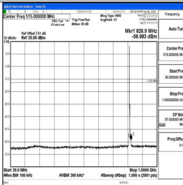
Band26_3MHz_16QAM_26740_1RB#0_30~1000_30~1000
