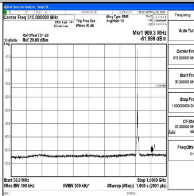
Band26_5MHz_16QAM_26740_1RB#0_30~1000_30~1000
