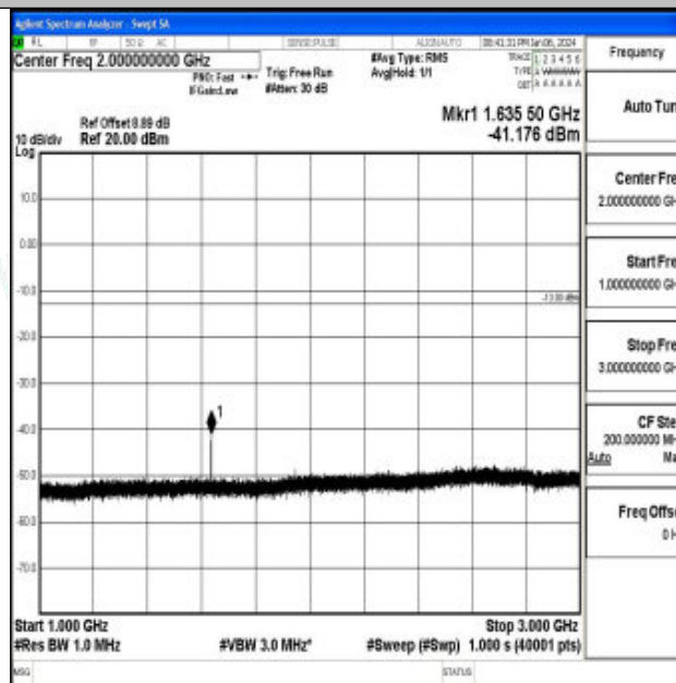
Band26_3MHz_QPSK_26740_1RB#0_1000~3000_1000~3000
