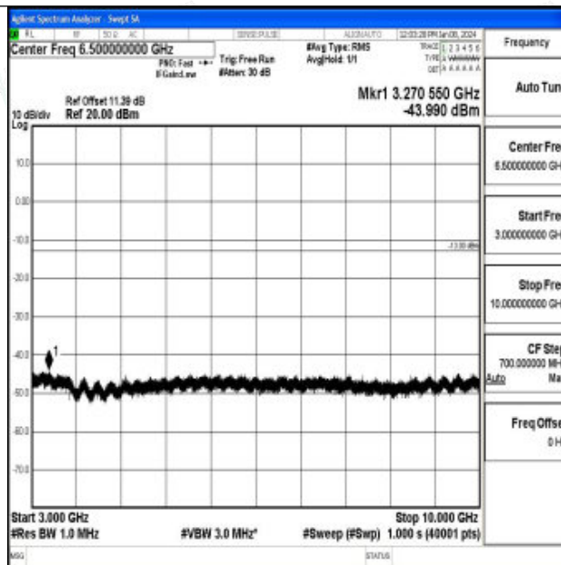
Band26_1.4MHz_QPSK_26697_1RB#0_3000~10000_3000~10000
