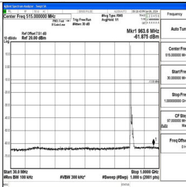
Band26_10MHz_QPSK_26740_1RB#0_30~1000_30~1000
