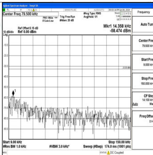
Band26_5MHz_QPSK_26765_1RB#0_0.009~0.15_0.009~0.15
