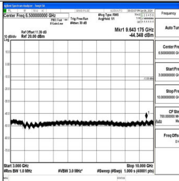
Band26_5MHz_16QAM_26740_1RB#0_3000~10000_3000~10000
