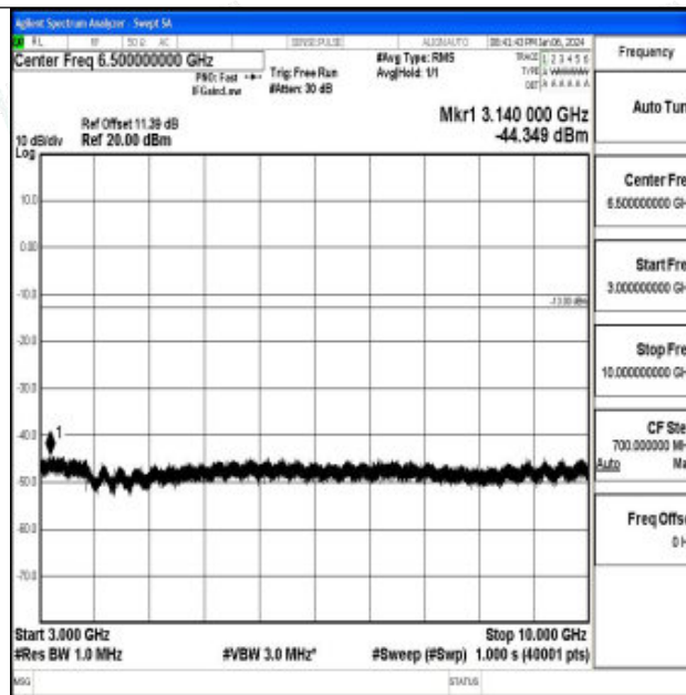
Band26_3MHz_QPSK_26740_1RB#0_3000~10000_3000~10000
