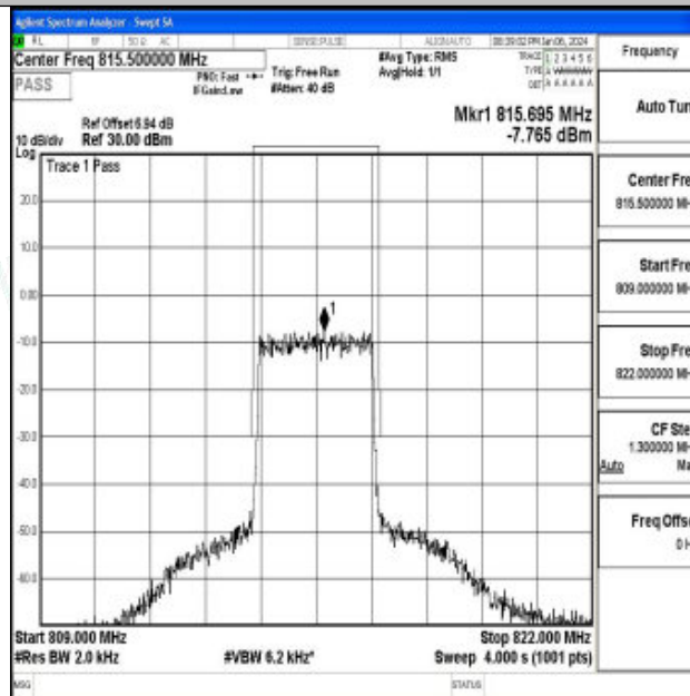
Band26_3MHz_16QAM_26705_15RB#0
