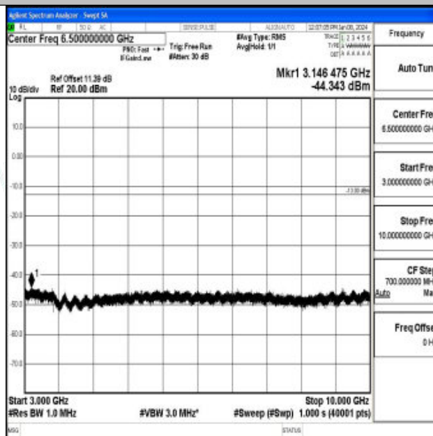
Band26_1.4MHz_16QAM_26783_1RB#0_3000~10000_3000~10000
