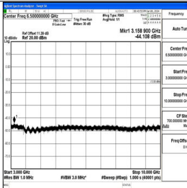
Band26_3MHz_16QAM_26775_1RB#0_3000~10000_3000~10000
