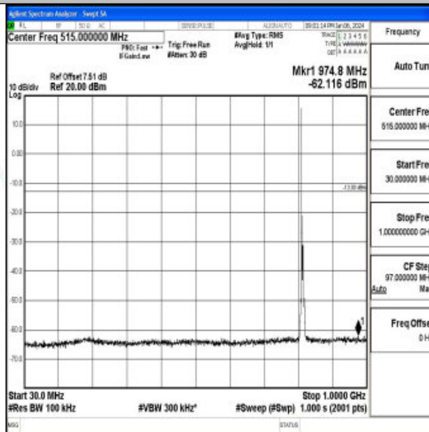
Band26_5MHz_16QAM_26715_1RB#0_30~1000_30~1000
