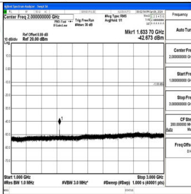
Band26_5MHz_16QAM_26740_1RB#0_1000~3000_1000~3000
