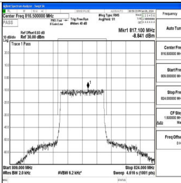
Band26_5MHz_QPSK_26715_25RB#0
