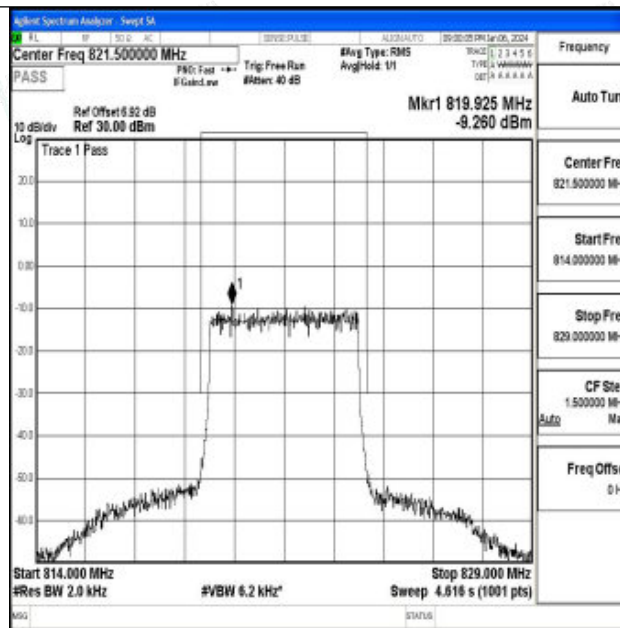
Band26_5MHz_16QAM_26765_25RB#0
