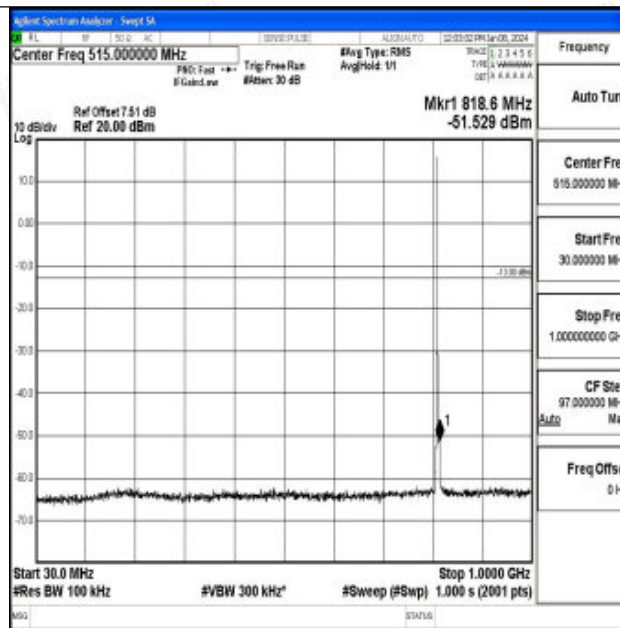
Band26_1.4MHz_QPSK_26697_1RB#0_30~1000_30~1000
