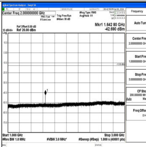
Band26_3MHz_QPSK_26775_1RB#0_1000~3000_1000~3000
