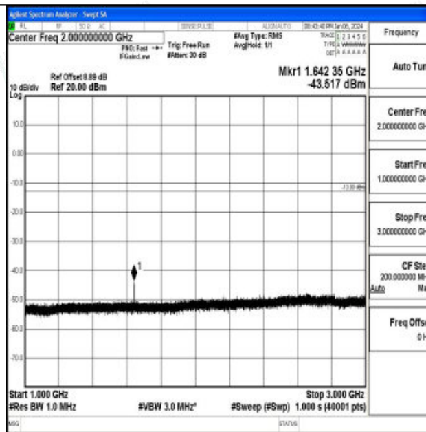
Band26_3MHz_16QAM_26775_1RB#0_1000~3000_1000~3000
