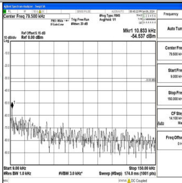
Band26_3MHz_16QAM_26705_1RB#0_0.009~0.15_0.009~0.15
