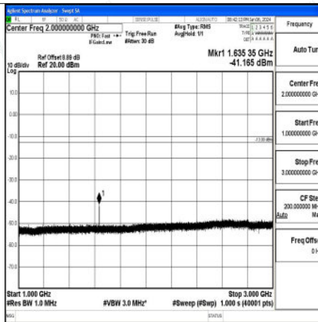
Band26_3MHz_16QAM_26740_1RB#0_1000~3000_1000~3000
