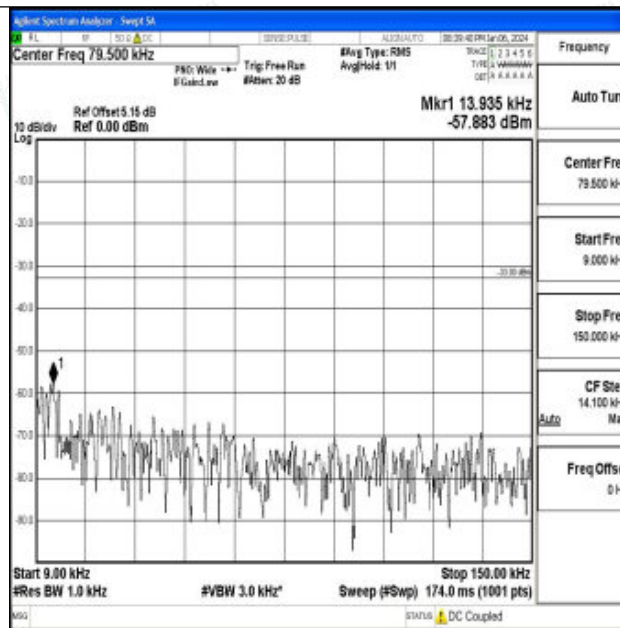
Band26_3MHz_QPSK_26705_1RB#0_0.009~0.15_0.009~0.15
