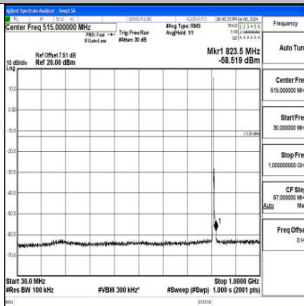
Band26_3MHz_16QAM_26705_1RB#0_30~1000_30~1000
