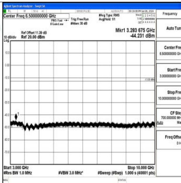
Band26_10MHz_QPSK_26740_1RB#0_3000~10000_3000~10000
