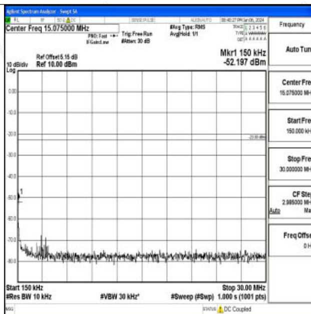
Band26_3MHz_16QAM_26705_1RB#0_0.15~30_0.15~30
