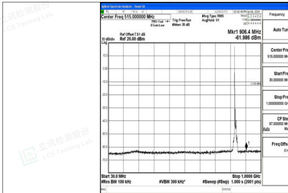
Band26_10MHz_QPSK_26915_1RB#0_30~1000_30~1000
