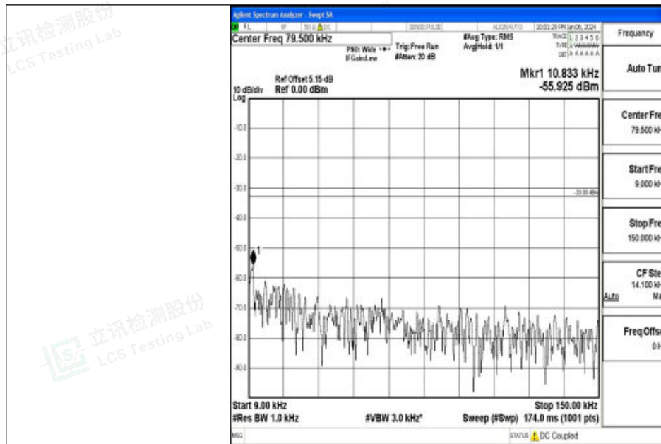
Band26_3MHz_QPSK_26915_1RB#0_0.009~0.15_0.009~0.15
