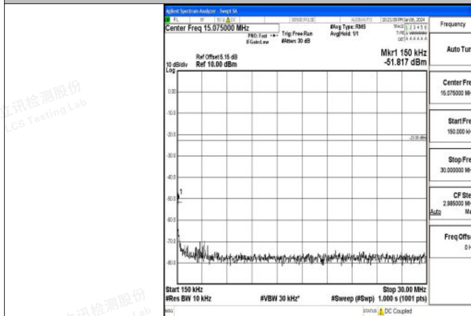
Band26_5MHz_QPSK_26815_1RB#0_0.15~30_0.15~30
