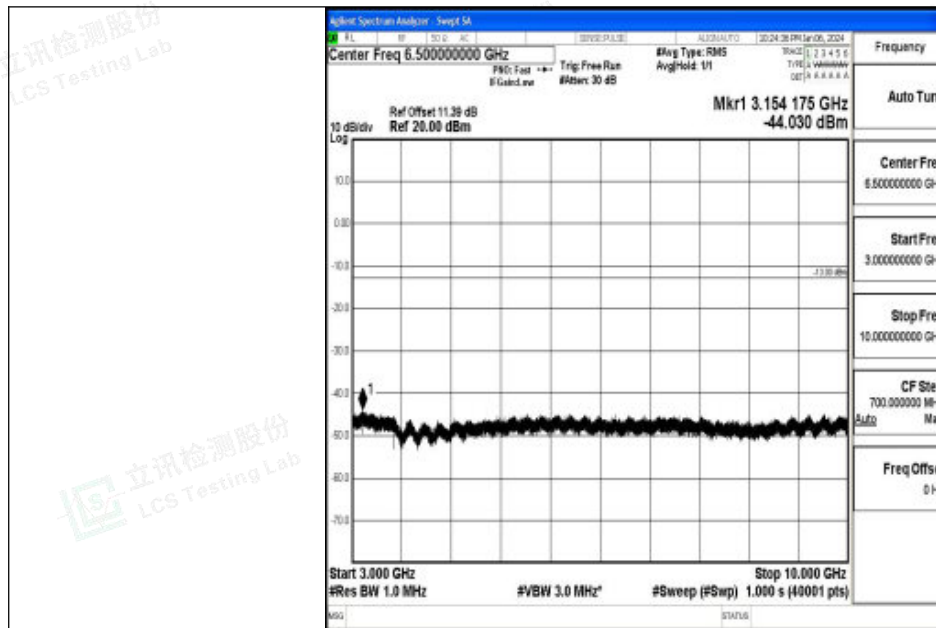
Band26_5MHz_QPSK_27015_1RB#0_3000~10000_3000~10000
