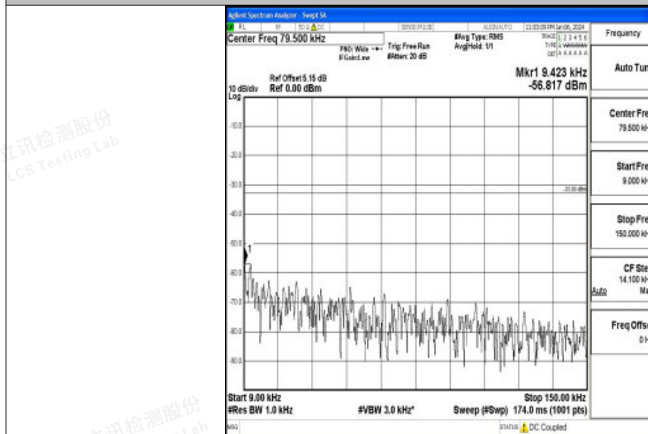
Band26_15MHz_16QAM_26965_1RB#0_0.009~0.15_0.009~0.15
