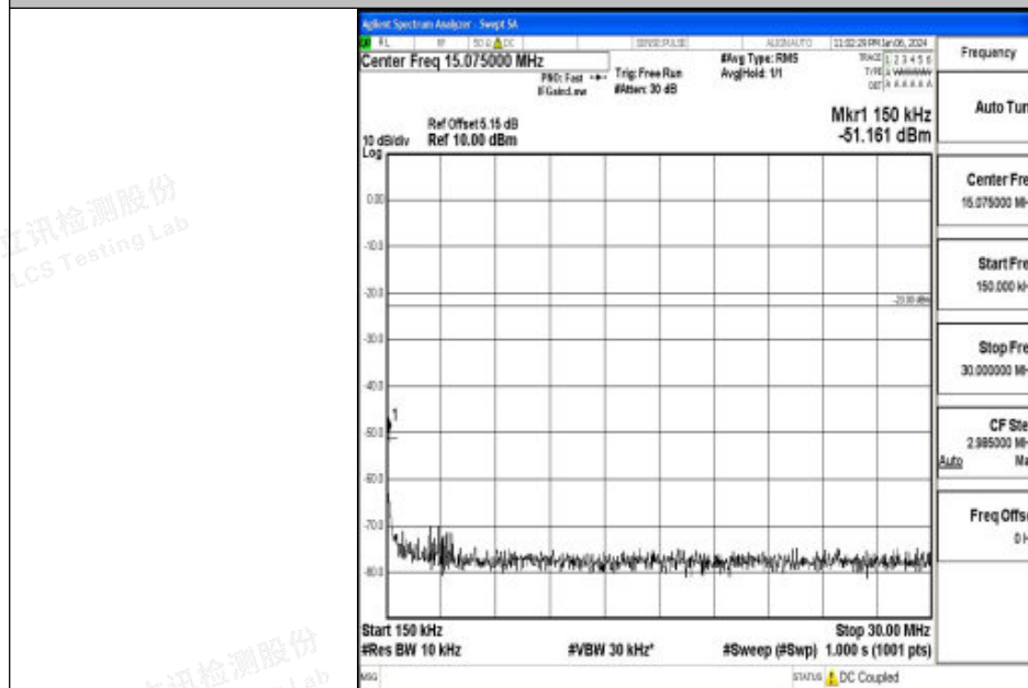
Band26_15MHz_QPSK_26965_1RB#0_0.15~30_0.15~30
