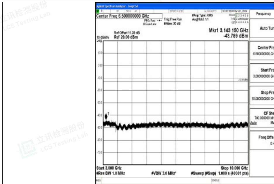
Band26_3MHz_QPSK_26805_1RB#0_3000~10000_3000~10000
