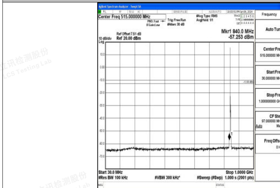
Band26_3MHz_16QAM_27025_1RB#0_30~1000_30~1000
