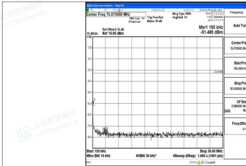
Band26_5MHz_16QAM_26915_1RB#0_0.15~30_0.15~30
