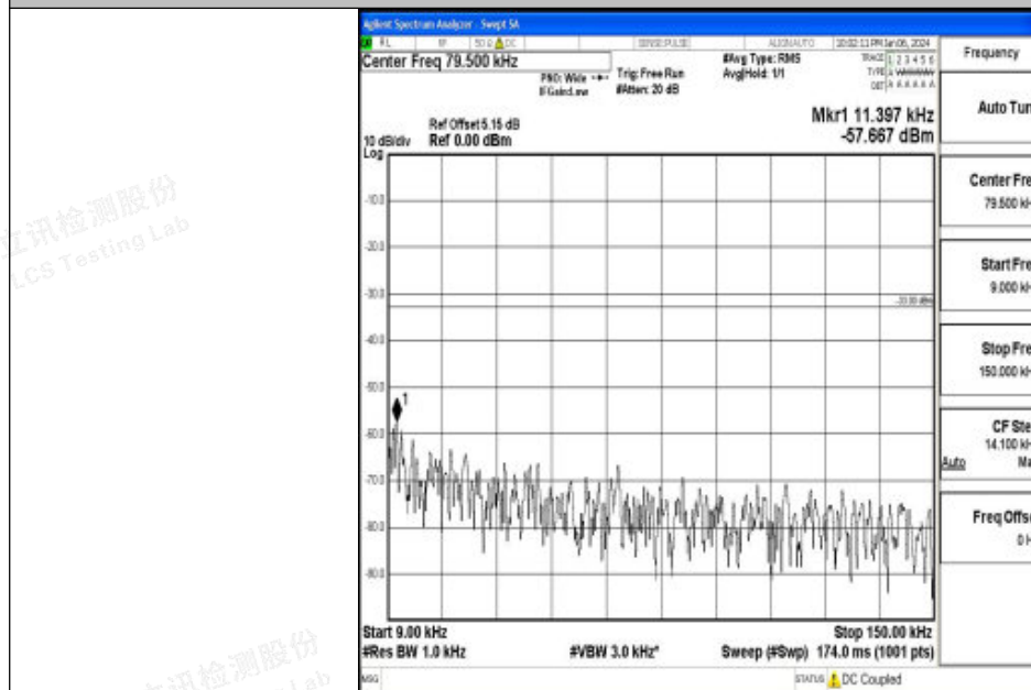
Band26_3MHz_16QAM_26915_1RB#0_0.009~0.15_0.009~0.15
