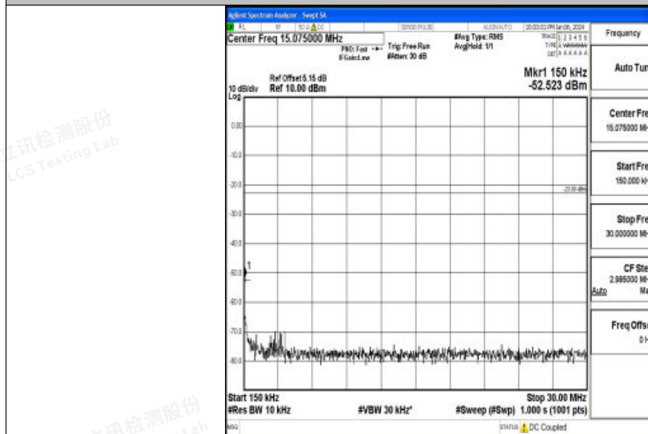
Band26_3MHz_QPSK_27025_1RB#0_0.15~30_0.15~30
