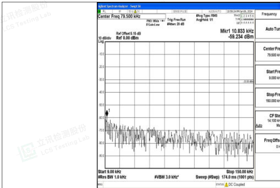
Band26_15MHz_QPSK_26865_1RB#0_0.009~0.15_0.009~0.15
