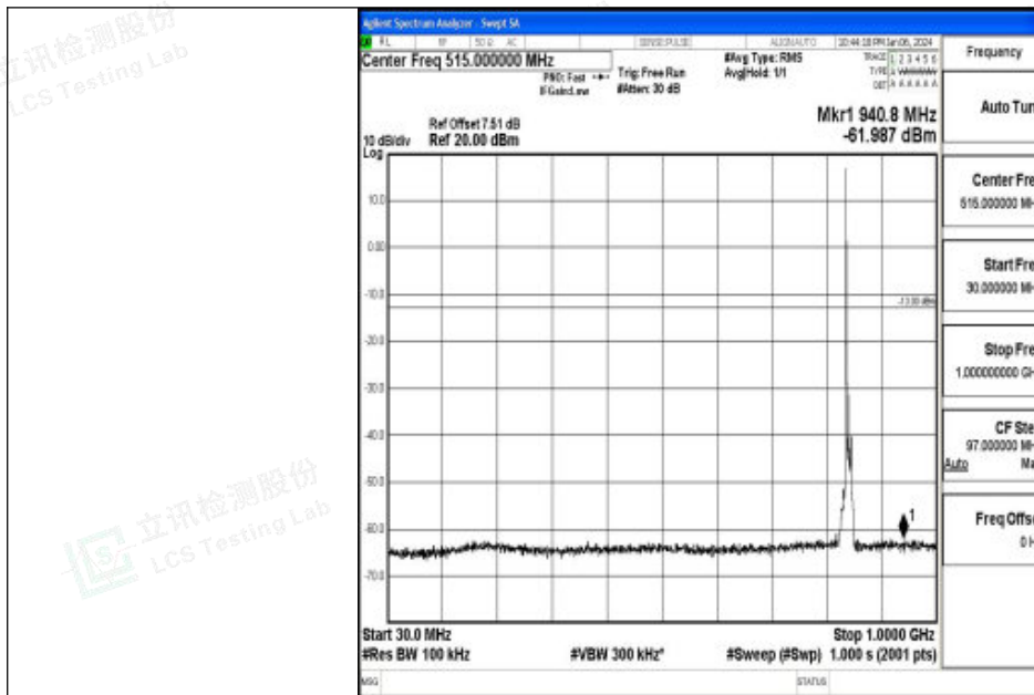
Band26_10MHz_QPSK_26990_1RB#0_30~1000_30~1000
