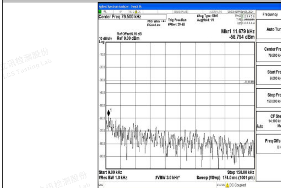
Band26_3MHz_16QAM_27025_1RB#0_0.009~0.15_0.009~0.15
