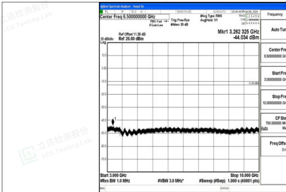
Band26_10MHz_QPSK_26990_1RB#0_3000~10000_3000~10000
