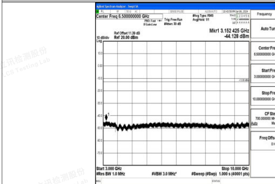
Band26_10MHz_16QAM_26915_1RB#0_3000~10000_3000~10000
