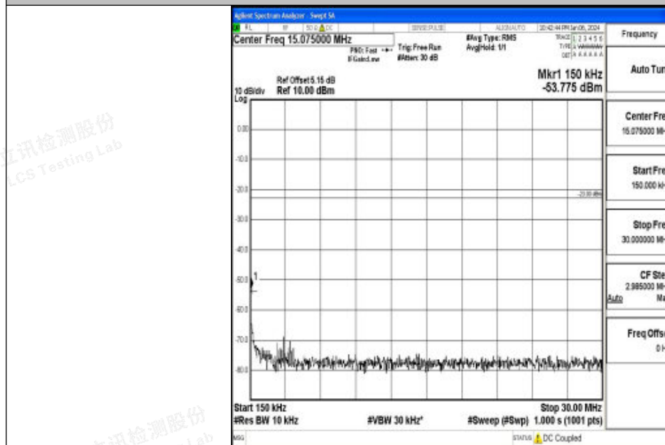
Band26_10MHz_QPSK_26915_1RB#0_0.15~30_0.15~30
