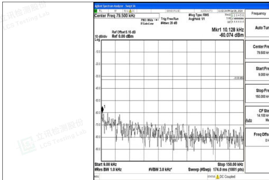
Band26_15MHz_QPSK_26965_1RB#0_0.009~0.15_0.009~0.15
