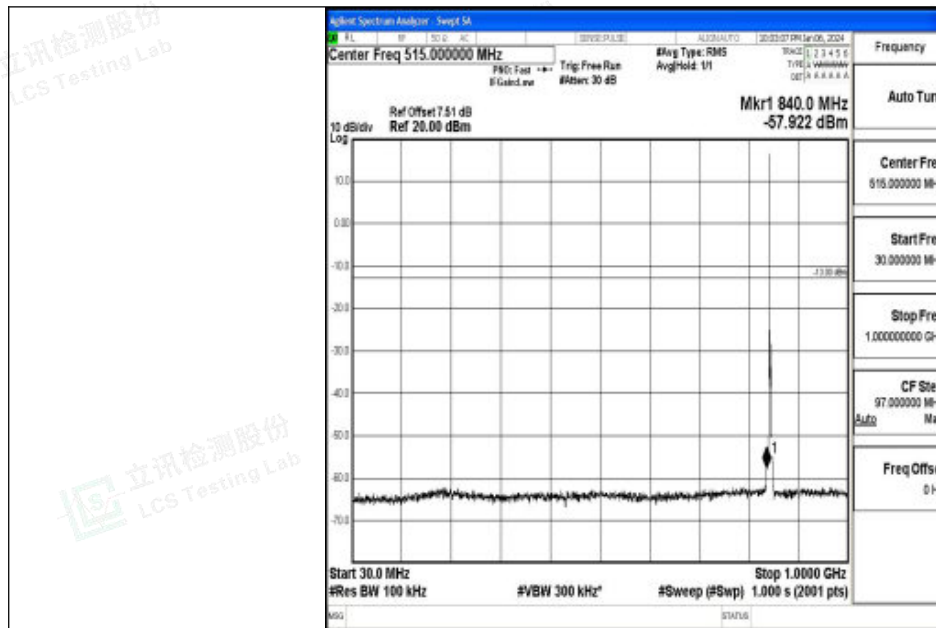
Band26_3MHz_QPSK_27025_1RB#0_30~1000_30~1000
