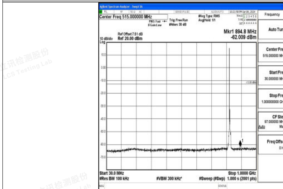
Band26_5MHz_16QAM_26815_1RB#0_30~1000_30~1000
