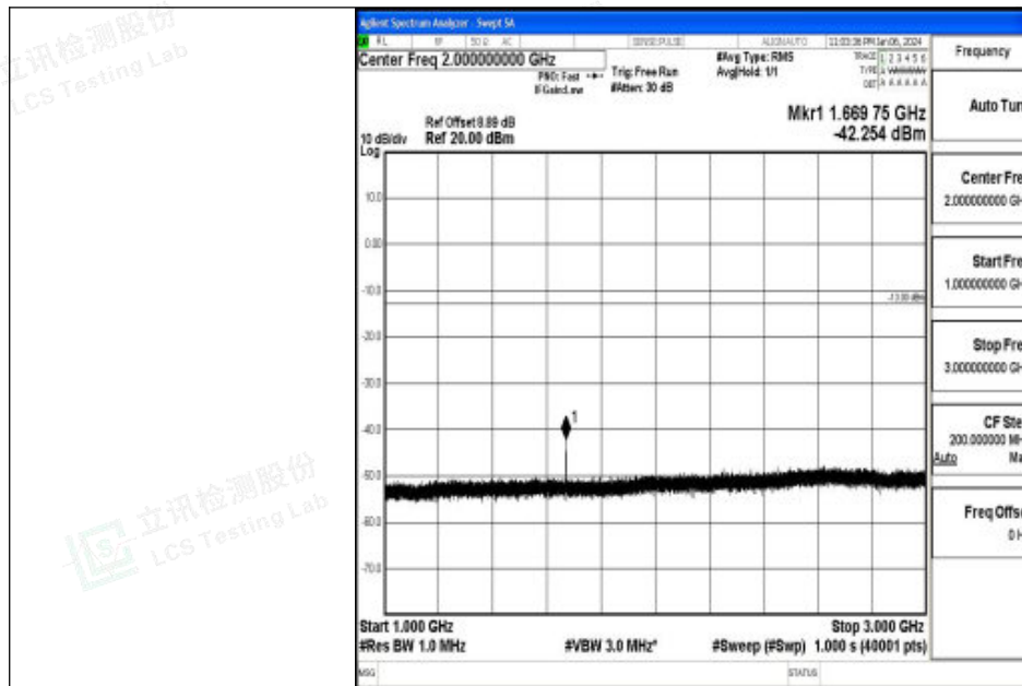
Band26_15MHz_16QAM_26965_1RB#0_1000~3000_1000~3000
