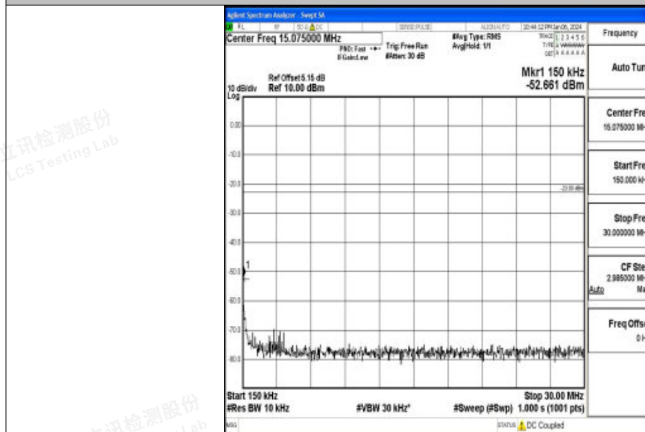
Band26_10MHz_QPSK_26990_1RB#0_0.15~30_0.15~30
