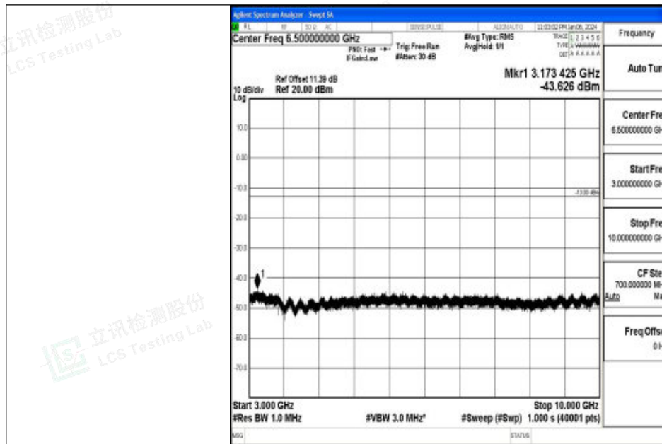
Band26_15MHz_QPSK_26965_1RB#0_3000~10000_3000~10000
