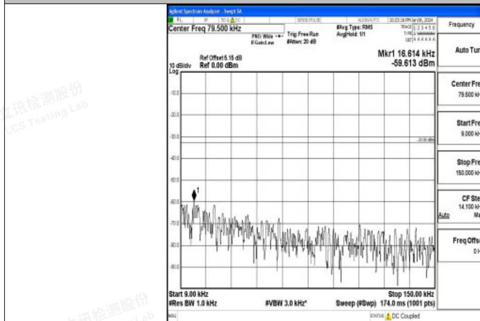
Band26_5MHz_16QAM_26915_1RB#0_0.009~0.15_0.009~0.15
