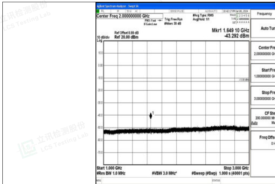
Band26_10MHz_16QAM_26840_1RB#0_1000~3000_1000~3000
