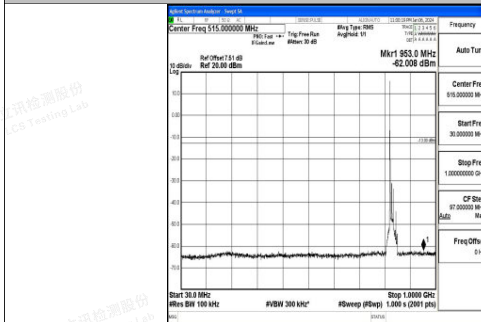
Band26_15MHz_16QAM_26865_1RB#0_30~1000_30~1000
