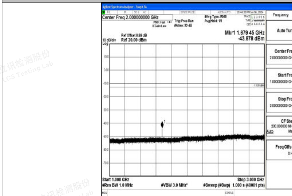
Band26_10MHz_QPSK_26990_1RB#0_1000~3000_1000~3000
