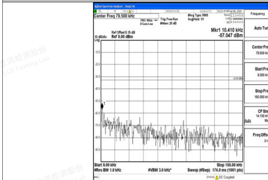
Band26_5MHz_16QAM_26815_1RB#0_0.009~0.15_0.009~0.15
