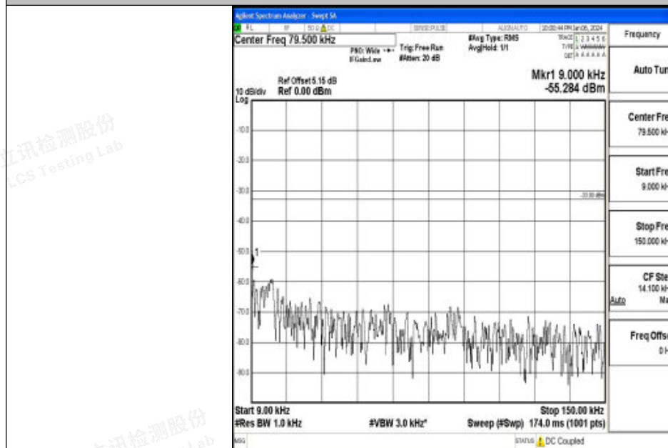
Band26_3MHz_16QAM_26805_1RB#0_0.009~0.15_0.009~0.15
