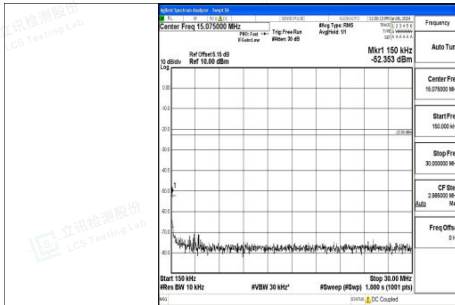
Band26_15MHz_16QAM_26865_1RB#0_0.15~30_0.15~30
