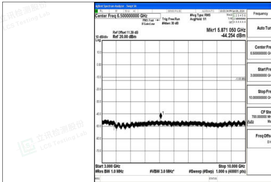
Band26_3MHz_QPSK_27025_1RB#0_3000~10000_3000~10000
