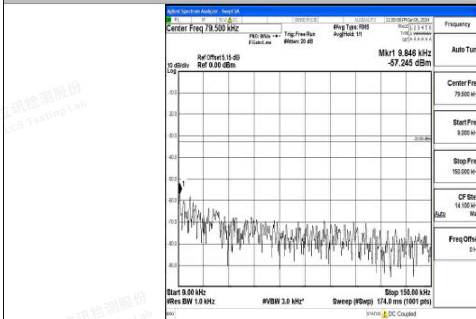
Band26_15MHz_16QAM_26865_1RB#0_0.009~0.15_0.009~0.15
