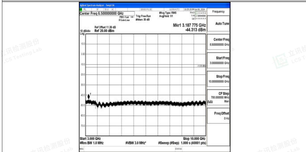
Band26_5MHz_16QAM_27015_1RB#0_3000~10000_3000~10000
