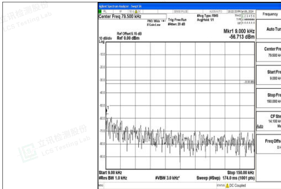
Band26_5MHz_QPSK_26915_1RB#0_0.009~0.15_0.009~0.15
