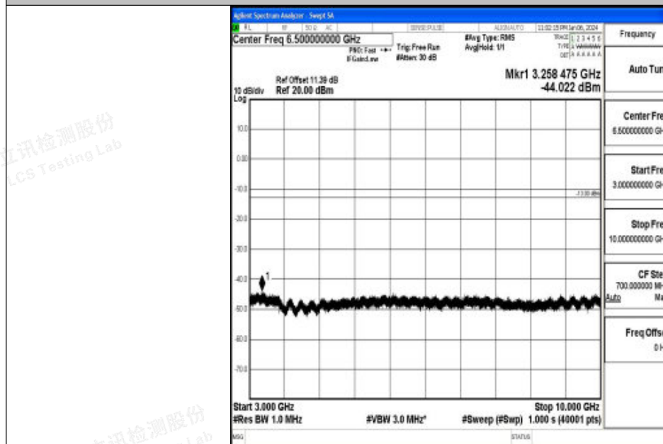
Band26_15MHz_16QAM_26915_1RB#0_3000~10000_3000~10000
