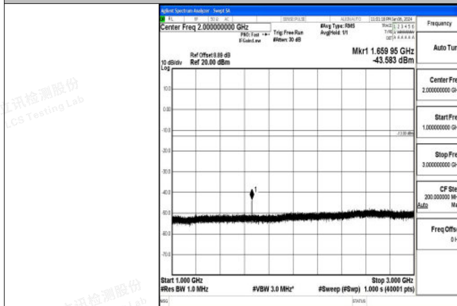
Band26_15MHz_QPSK_26915_1RB#0_1000~3000_1000~3000
