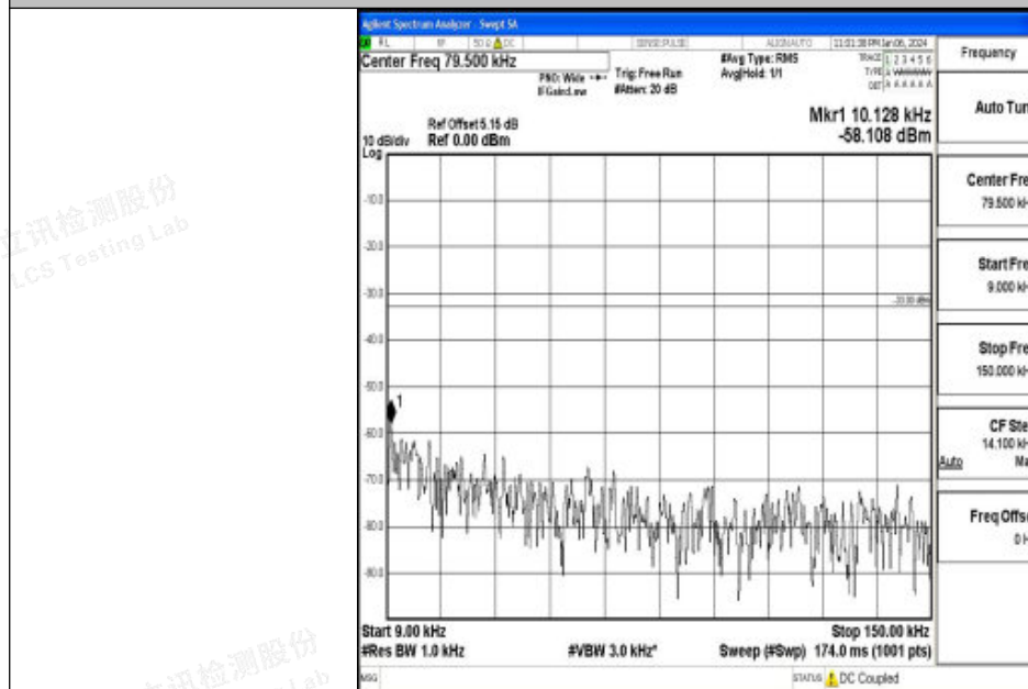
Band26_15MHz_16QAM_26915_1RB#0_0.009~0.15_0.009~0.15
