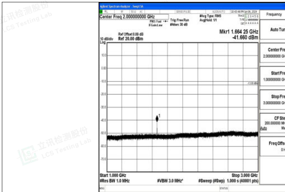
Band26_10MHz_16QAM_26915_1RB#0_1000~3000_1000~3000
