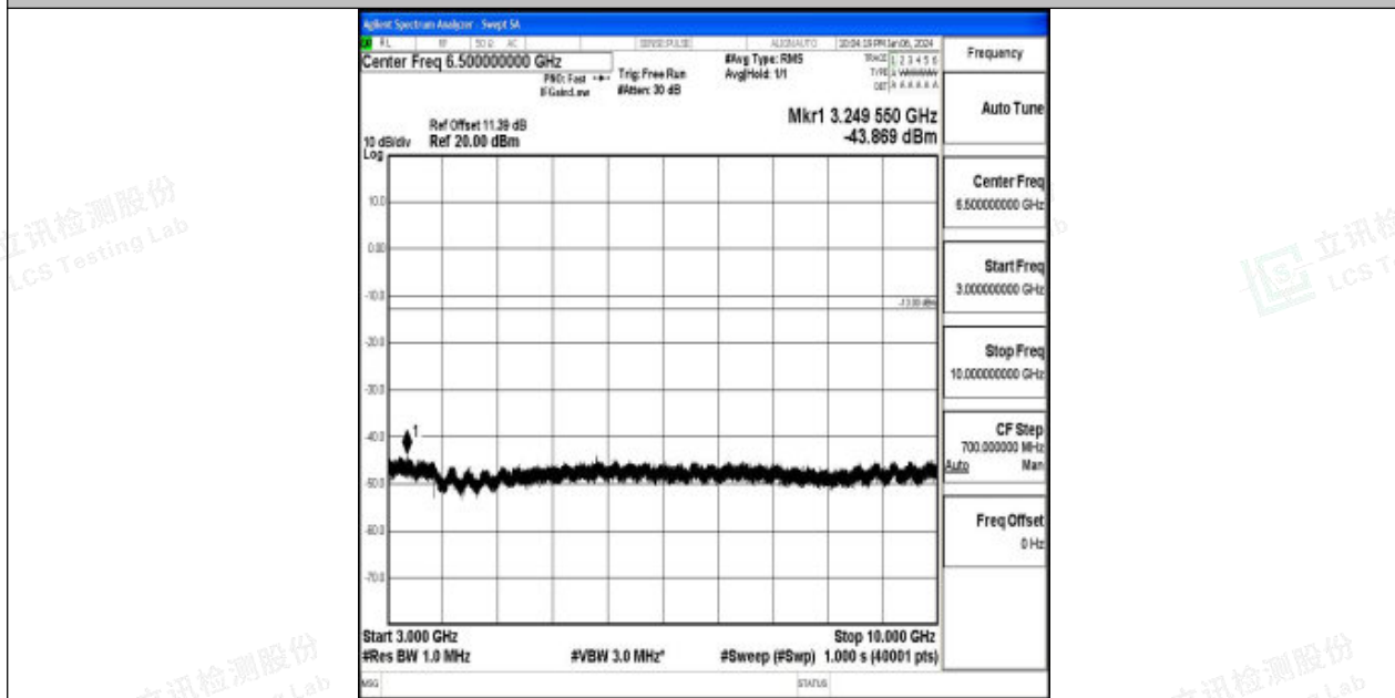
Band26_3MHz_16QAM_27025_1RB#0_3000~10000_3000~10000
