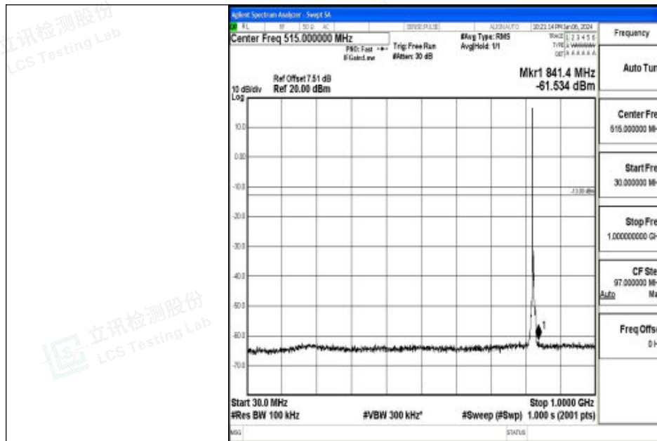
Band26_5MHz_QPSK_26815_1RB#0_30~1000_30~1000
