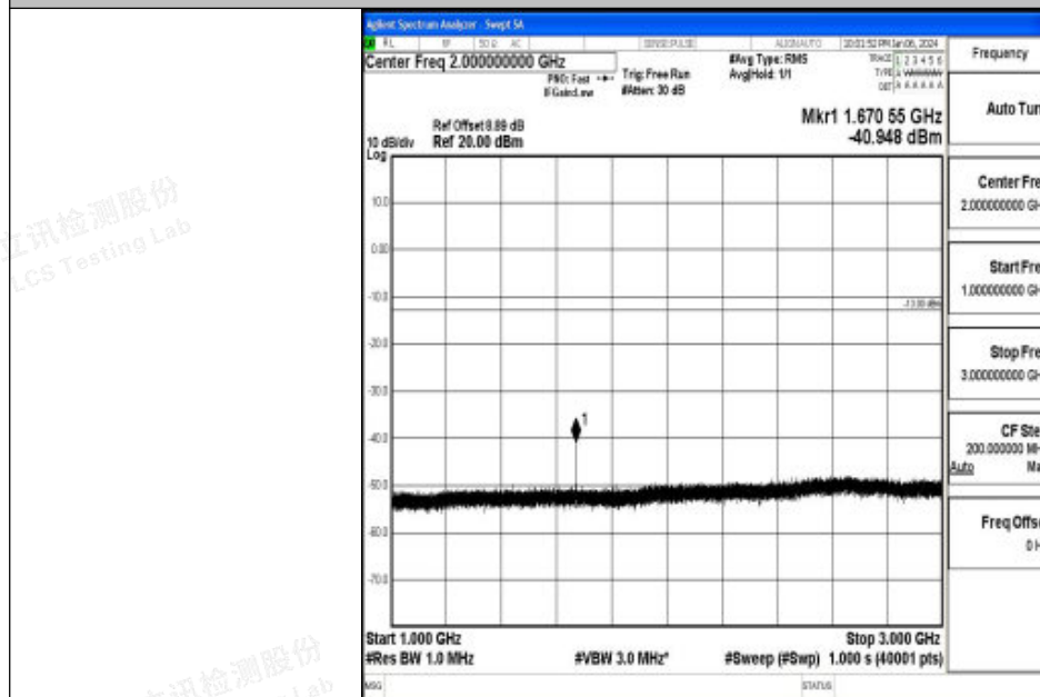
Band26_3MHz_QPSK_26915_1RB#0_1000~3000_1000~3000
