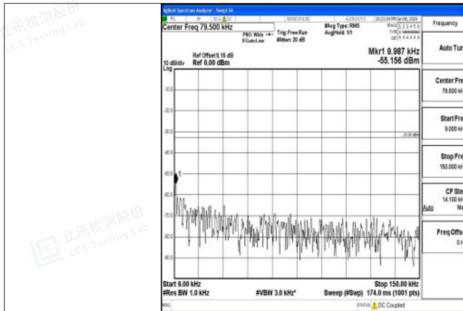
Band26_5MHz_QPSK_26815_1RB#0_0.009~0.15_0.009~0.15
