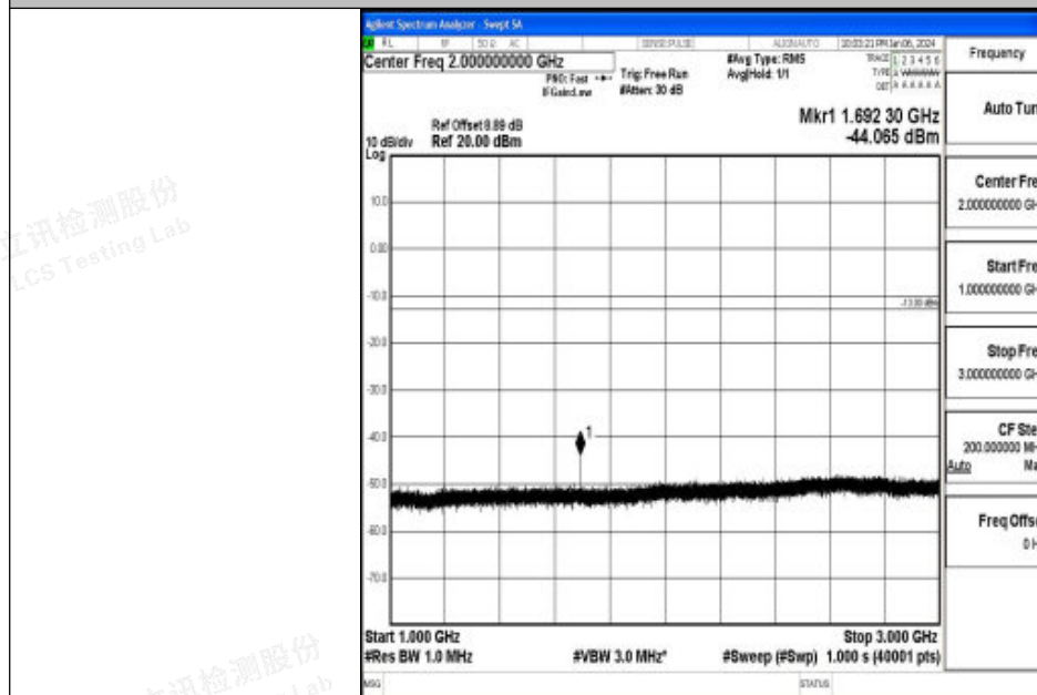
Band26_3MHz_QPSK_27025_1RB#0_1000~3000_1000~3000
