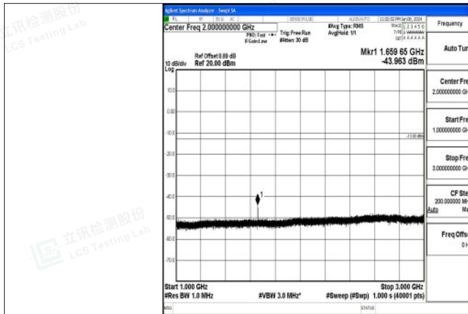
Band26_15MHz_16QAM_26915_1RB#0_1000~3000_1000~3000
