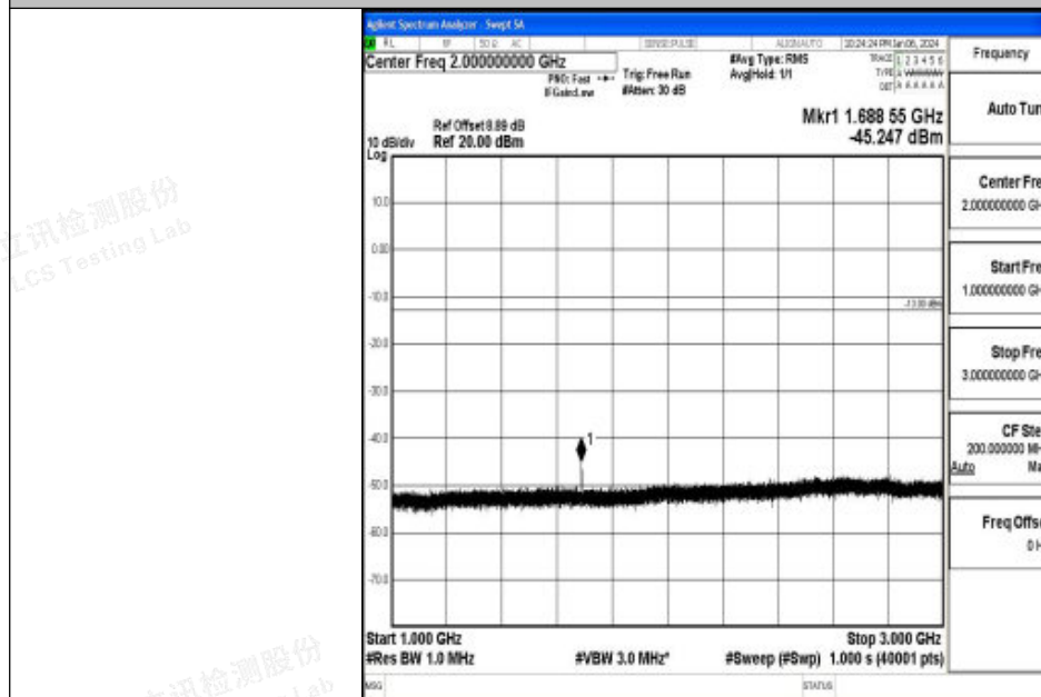
Band26_5MHz_QPSK_27015_1RB#0_1000~3000_1000~3000
