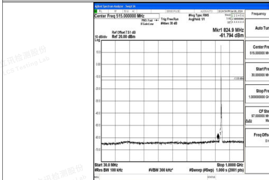
Band26_5MHz_16QAM_27015_1RB#0_30~1000_30~1000
