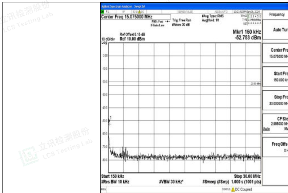
Band26_5MHz_16QAM_26815_1RB#0_0.15~30_0.15~30
