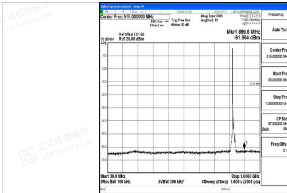
Band26_10MHz_QPSK_26840_1RB#0_30~1000_30~1000
