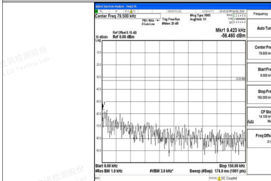
Band26_10MHz_16QAM_26915_1RB#0_0.009~0.15_0.009~0.15
