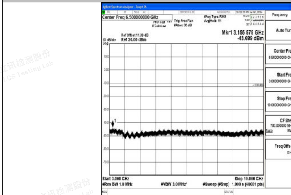
Band26_3MHz_16QAM_26805_1RB#0_3000~10000_3000~10000
