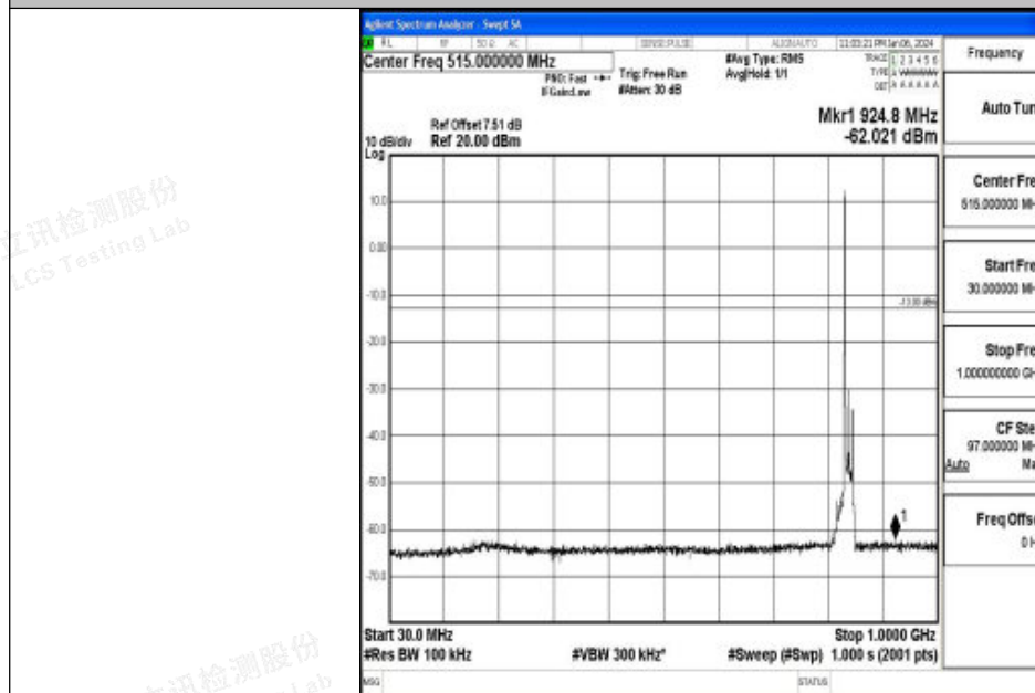
Band26_15MHz_16QAM_26965_1RB#0_30~1000_30~1000
