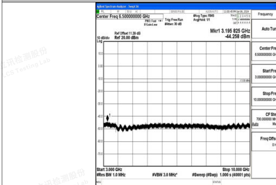
Band26_15MHz_16QAM_26865_1RB#0_3000~10000_3000~10000
