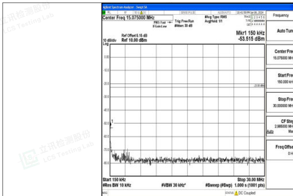
Band26_10MHz_16QAM_26840_1RB#0_0.15~30_0.15~30
