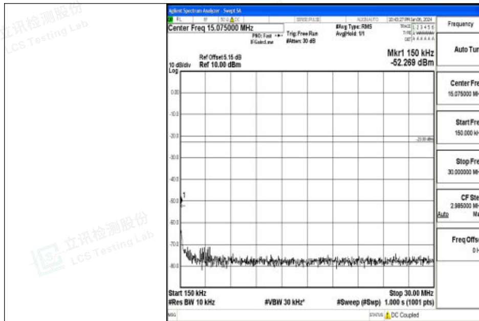
Band26_10MHz_16QAM_26915_1RB#0_0.15~30_0.15~30
