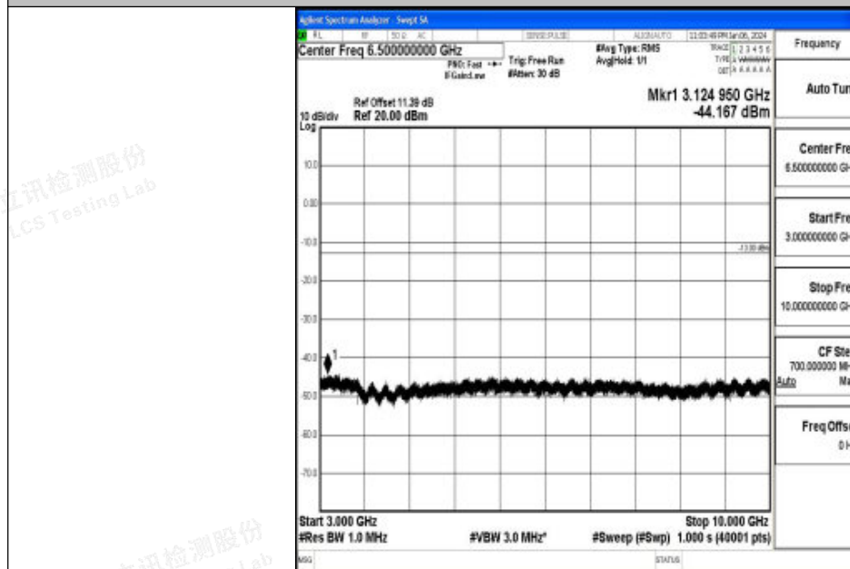
Band26_15MHz_16QAM_26965_1RB#0_3000~10000_3000~10000
