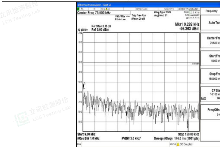
Band26_10MHz_QPSK_26990_1RB#0_0.009~0.15_0.009~0.15
