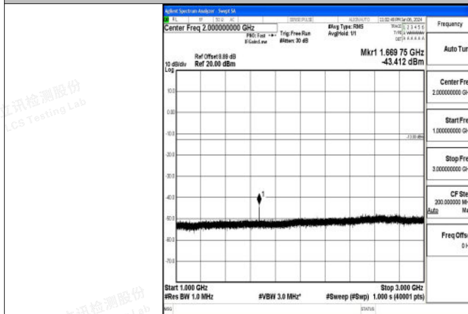
Band26_15MHz_QPSK_26965_1RB#0_1000~3000_1000~3000
