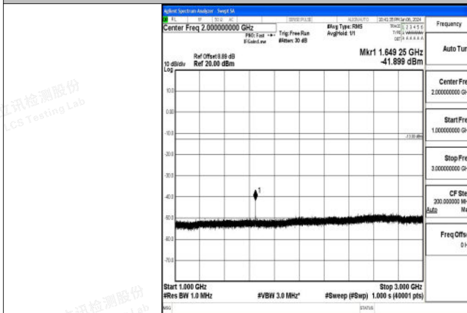
Band26_10MHz_QPSK_26840_1RB#0_1000~3000_1000~3000
