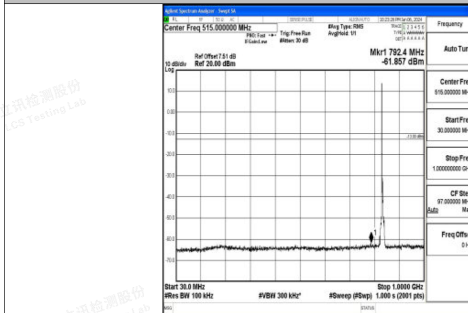
Band26_5MHz_16QAM_26915_1RB#0_30~1000_30~1000
