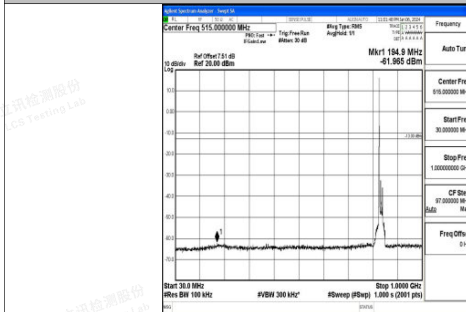
Band26_15MHz_16QAM_26915_1RB#0_30~1000_30~1000
