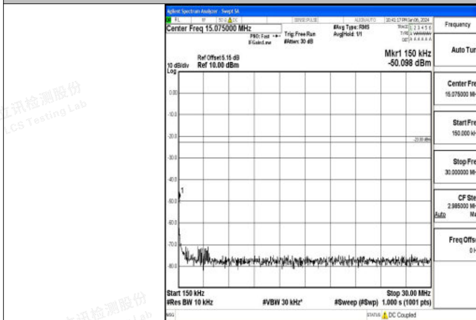
Band26_10MHz_QPSK_26840_1RB#0_0.15~30_0.15~30
