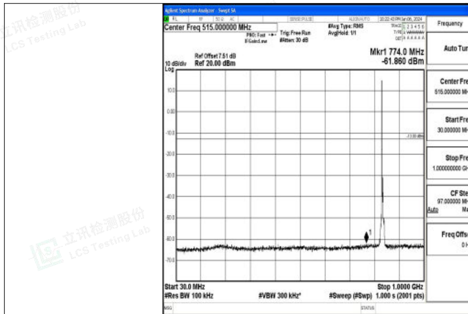
Band26_5MHz_QPSK_26915_1RB#0_30~1000_30~1000
