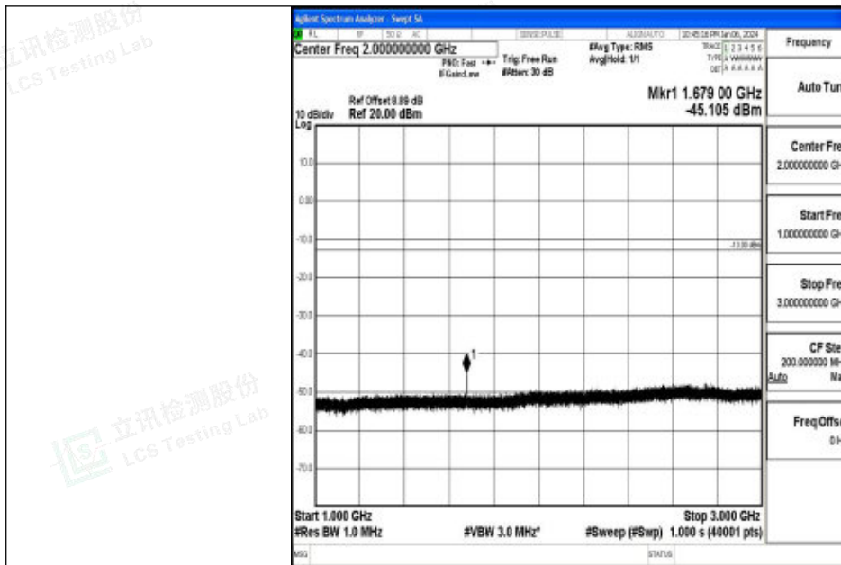
Band26_10MHz_16QAM_26990_1RB#0_1000~3000_1000~3000
