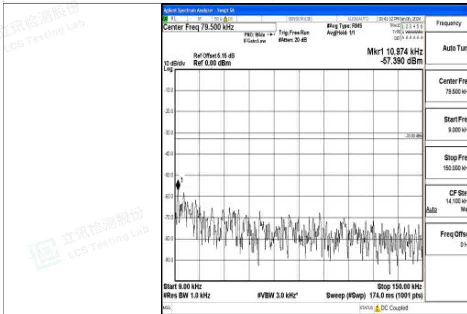
Band26_10MHz_QPSK_26840_1RB#0_0.009~0.15_0.009~0.15
