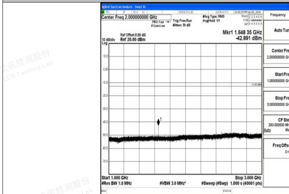
Band26_3MHz_QPSK_26805_1RB#0_1000~3000_1000~3000
