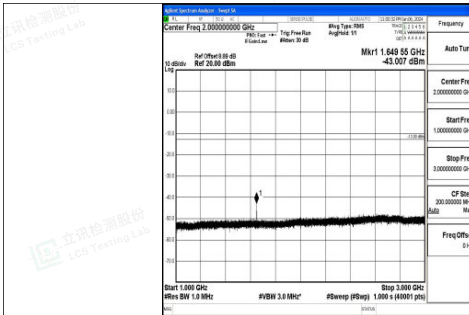
Band26_15MHz_16QAM_26865_1RB#0_1000~3000_1000~3000
