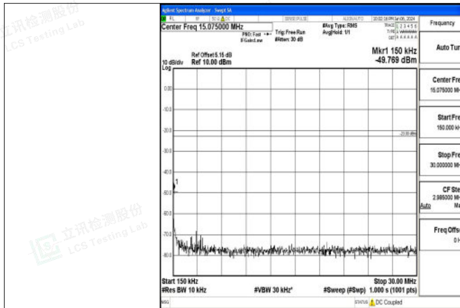
Band26_3MHz_16QAM_26915_1RB#0_0.15~30_0.15~30
