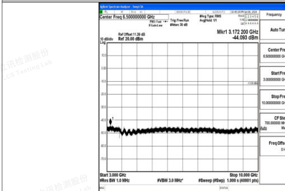
Band26_10MHz_16QAM_26990_1RB#0_3000~10000_3000~10000
