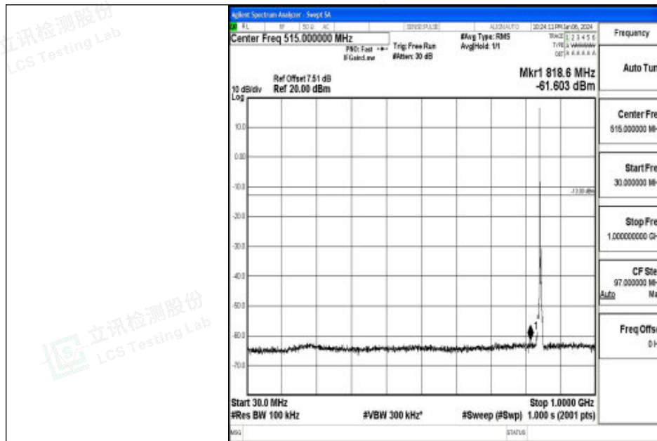
Band26_5MHz_QPSK_27015_1RB#0_30~1000_30~1000
