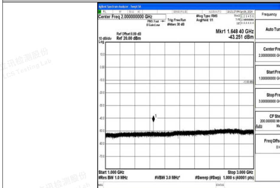
Band26_5MHz_QPSK_26815_1RB#0_1000~3000_1000~3000
