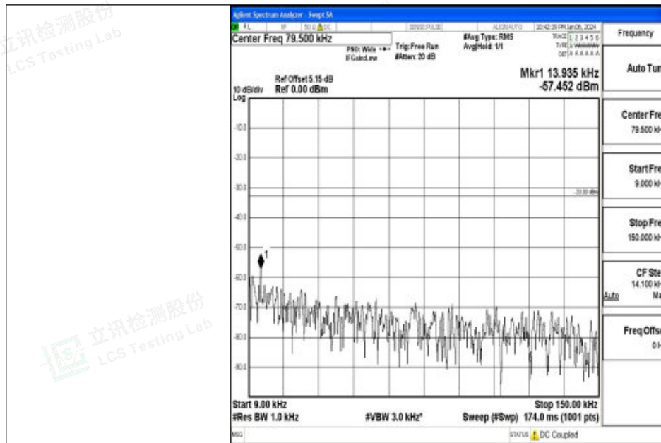
Band26_10MHz_QPSK_26915_1RB#0_0.009~0.15_0.009~0.15
