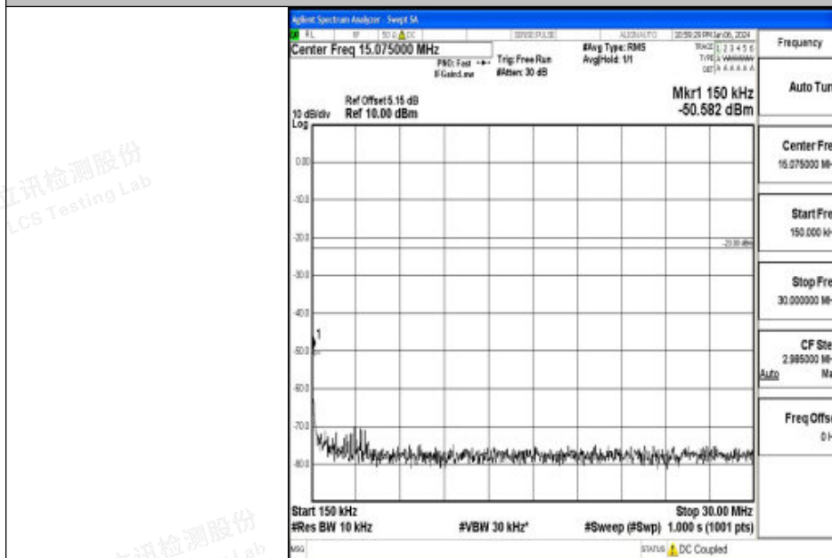
Band26_15MHz_QPSK_26865_1RB#0_0.15~30_0.15~30
