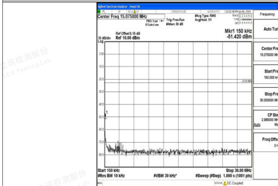
Band26_5MHz_QPSK_26915_1RB#0_0.15~30_0.15~30
