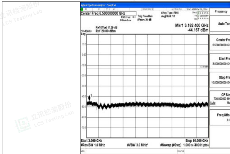
Band26_10MHz_QPSK_26840_1RB#0_3000~10000_3000~10000
