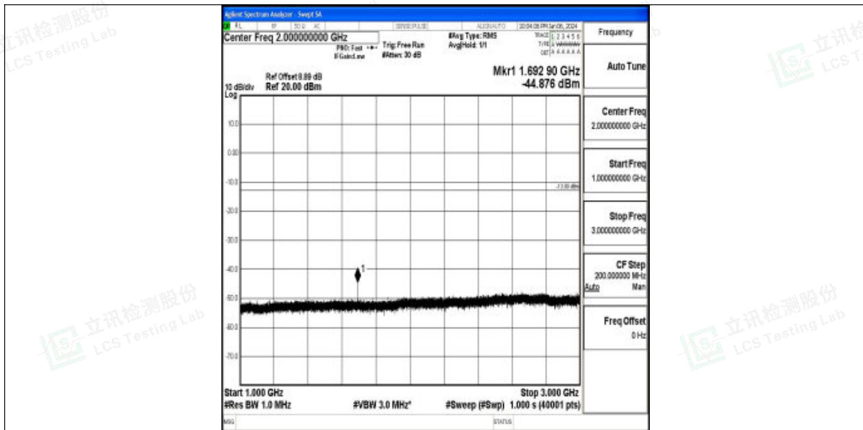
Band26_3MHz_16QAM_27025_1RB#0_1000~3000_1000~3000
