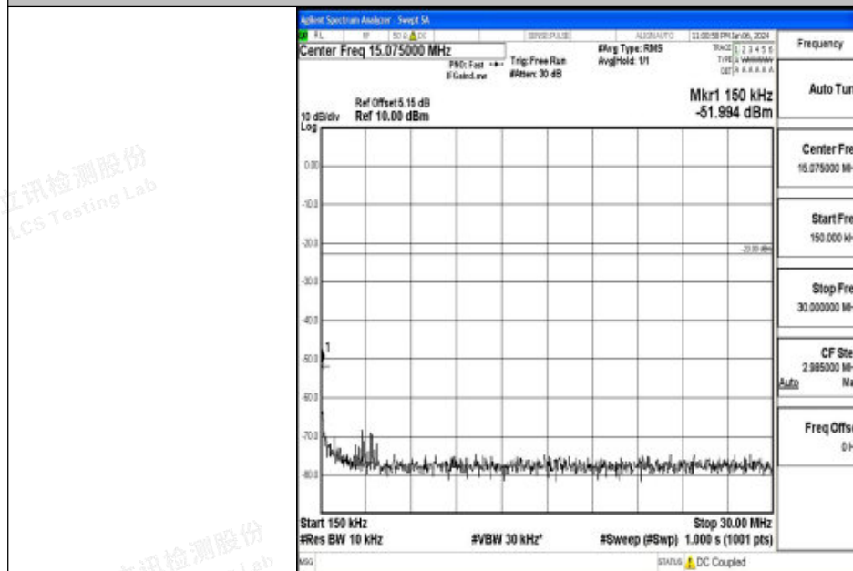
Band26_15MHz_QPSK_26915_1RB#0_0.15~30_0.15~30
