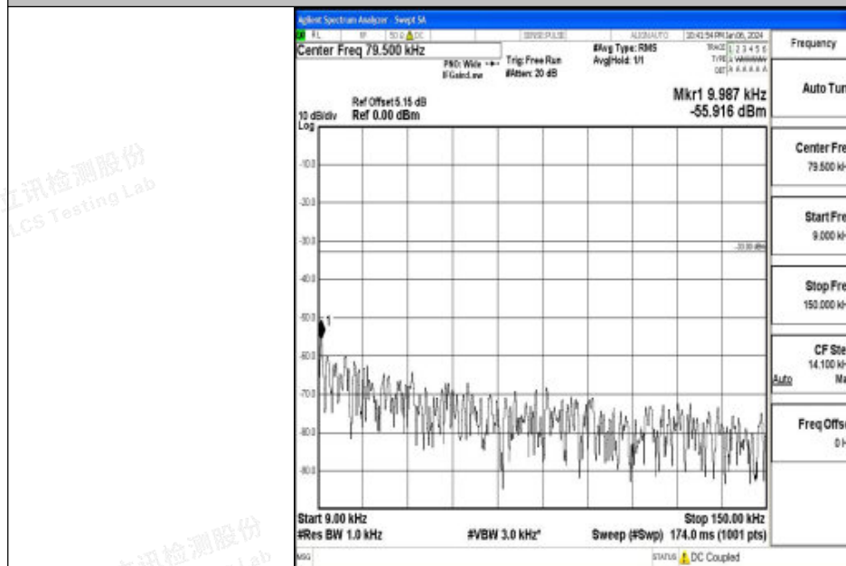
Band26_10MHz_16QAM_26840_1RB#0_0.009~0.15_0.009~0.15
