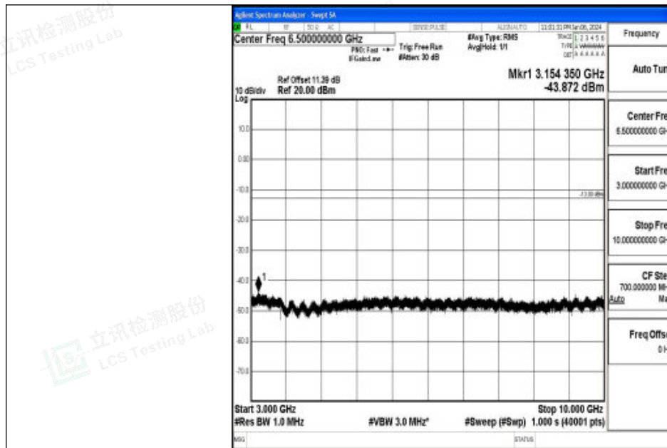
Band26_15MHz_QPSK_26915_1RB#0_3000~10000_3000~10000
