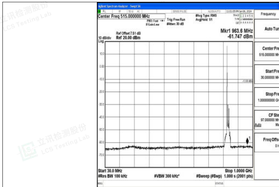
Band26_15MHz_QPSK_26915_1RB#0_30~1000_30~1000
