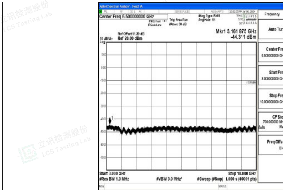
Band26_3MHz_QPSK_26915_1RB#0_3000~10000_3000~10000
