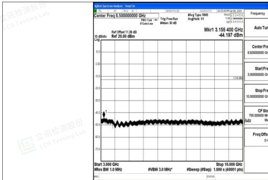
Band26_5MHz_QPSK_26915_1RB#0_3000~10000_3000~10000
