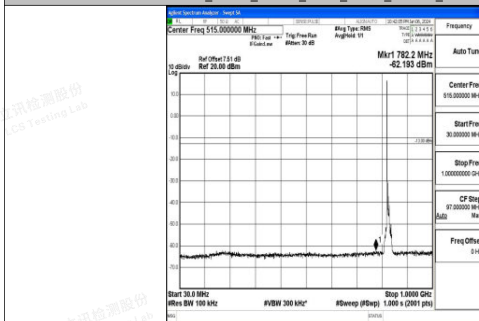
Band26_10MHz_16QAM_26840_1RB#0_30~1000_30~1000
