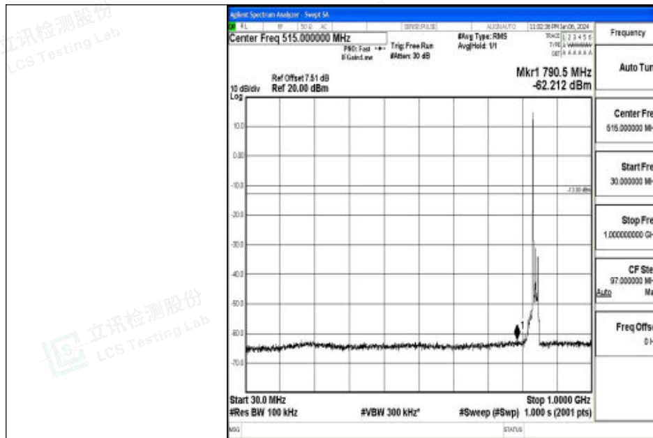
Band26_15MHz_QPSK_26965_1RB#0_30~1000_30~1000
