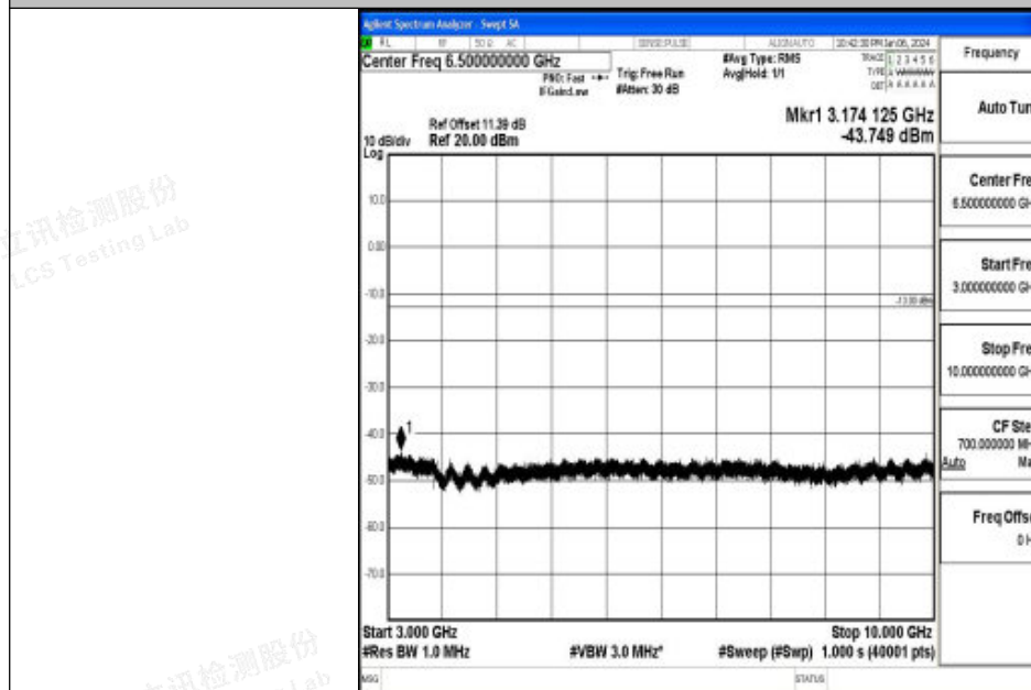
Band26_10MHz_16QAM_26840_1RB#0_3000~10000_3000~10000
