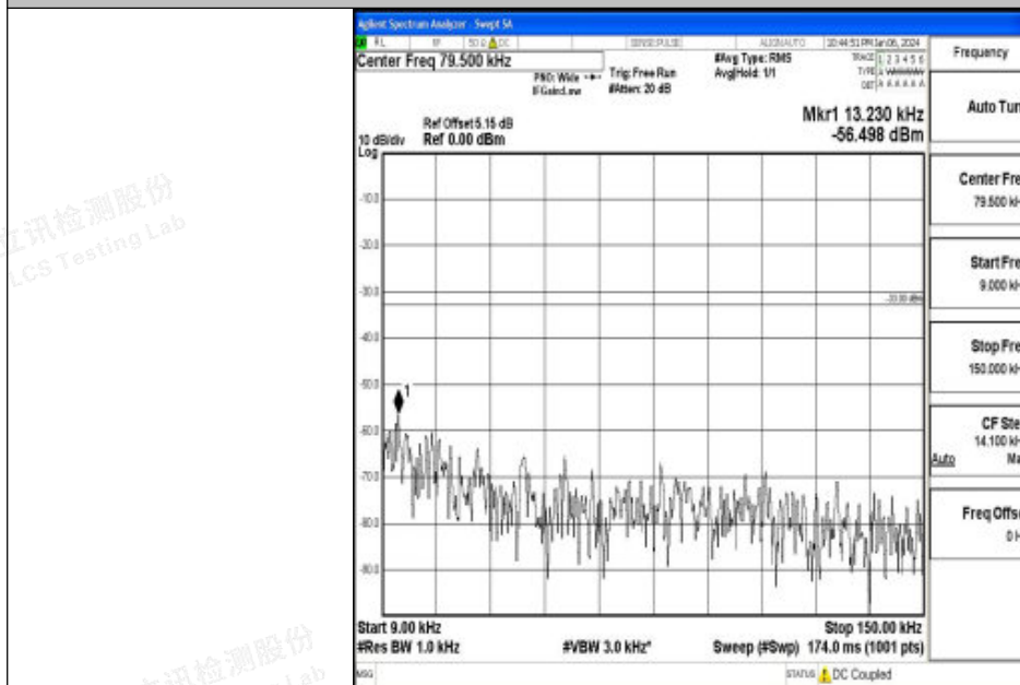
Band26_10MHz_16QAM_26990_1RB#0_0.009~0.15_0.009~0.15
