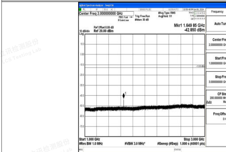
Band26_15MHz_QPSK_26865_1RB#0_1000~3000_1000~3000
