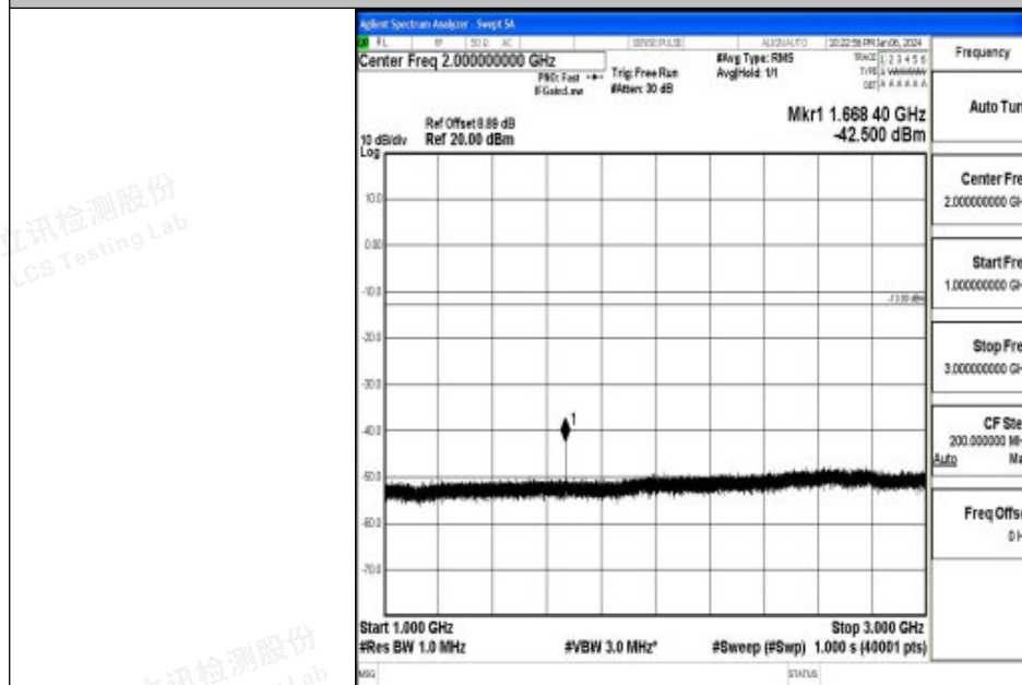
Band26_5MHz_QPSK_26915_1RB#0_1000~3000_1000~3000
