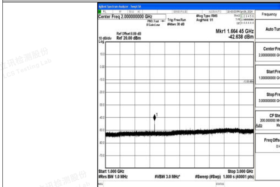
Band26_10MHz_QPSK_26915_1RB#0_1000~3000_1000~3000
