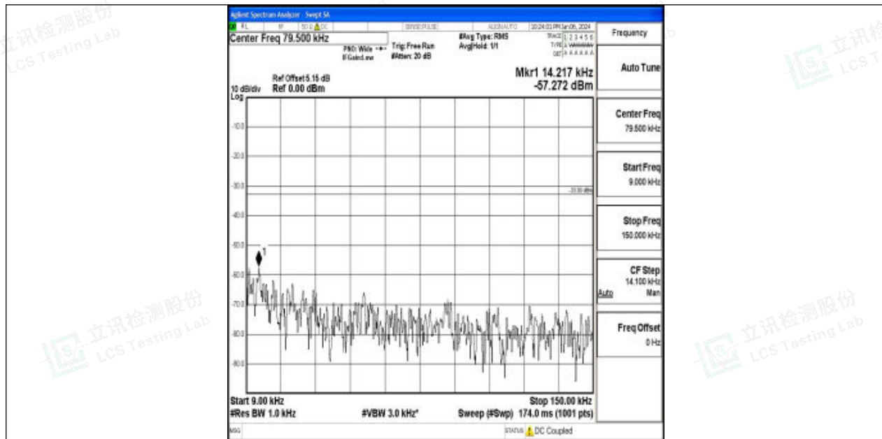
Band26_5MHz_QPSK_27015_1RB#0_0.009~0.15_0.009~0.15
