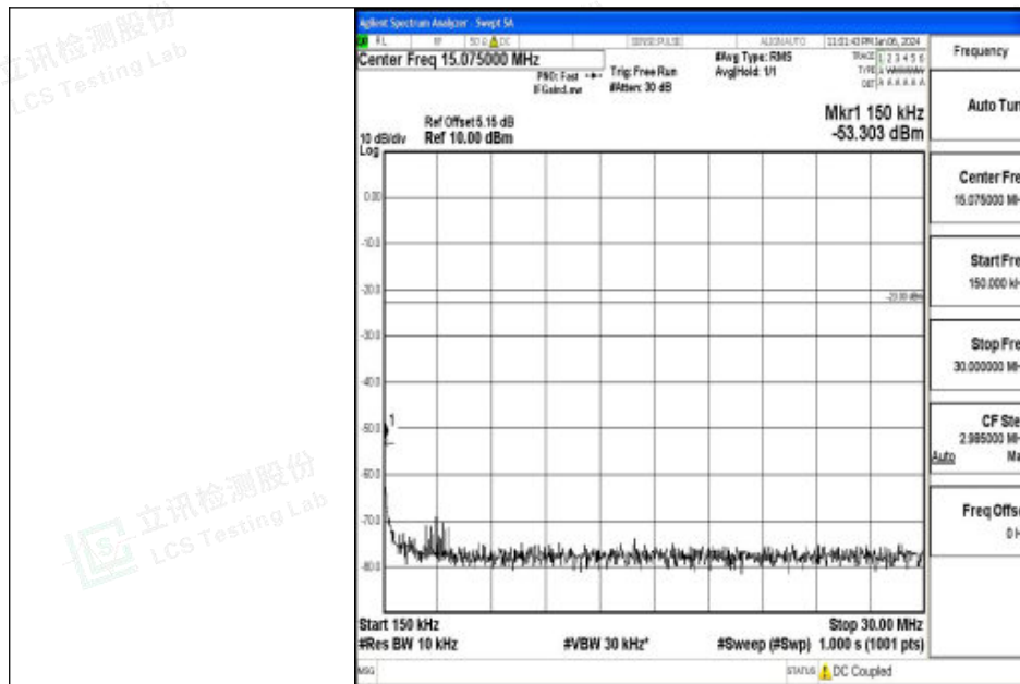
Band26_15MHz_16QAM_26915_1RB#0_0.15~30_0.15~30
