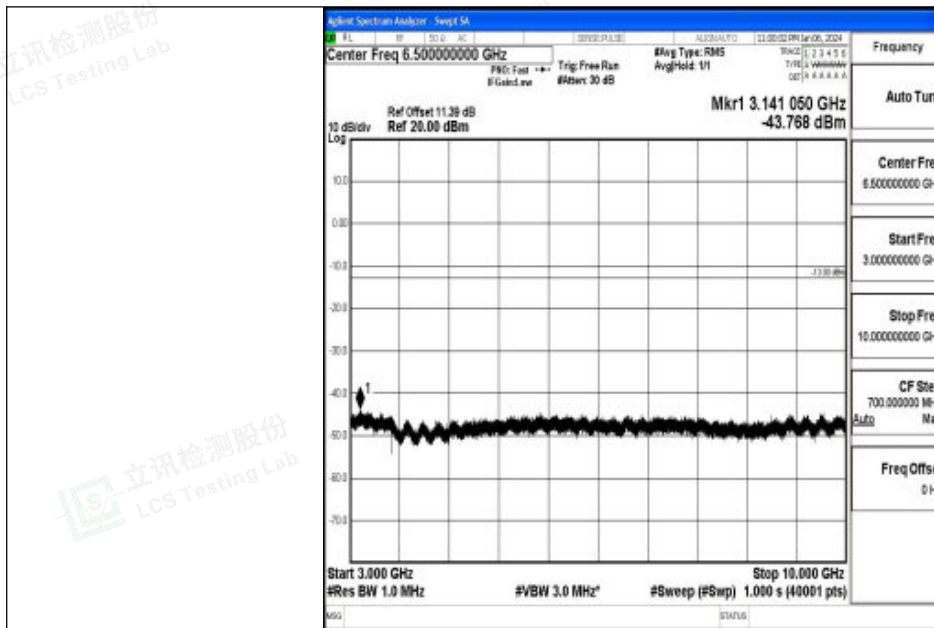
Band26_15MHz_QPSK_26865_1RB#0_3000~10000_3000~10000
