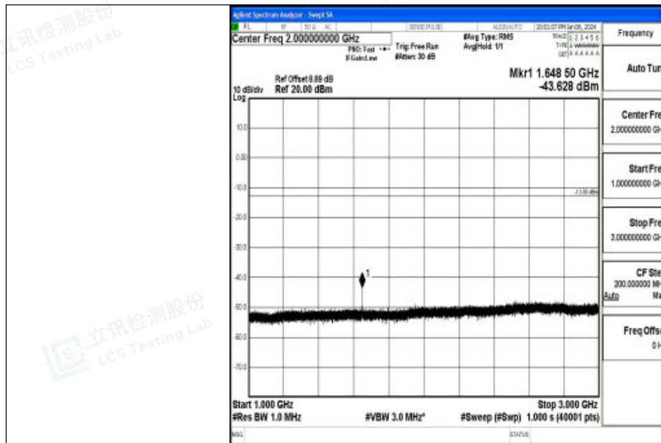
Band26_3MHz_16QAM_26805_1RB#0_1000~3000_1000~3000
