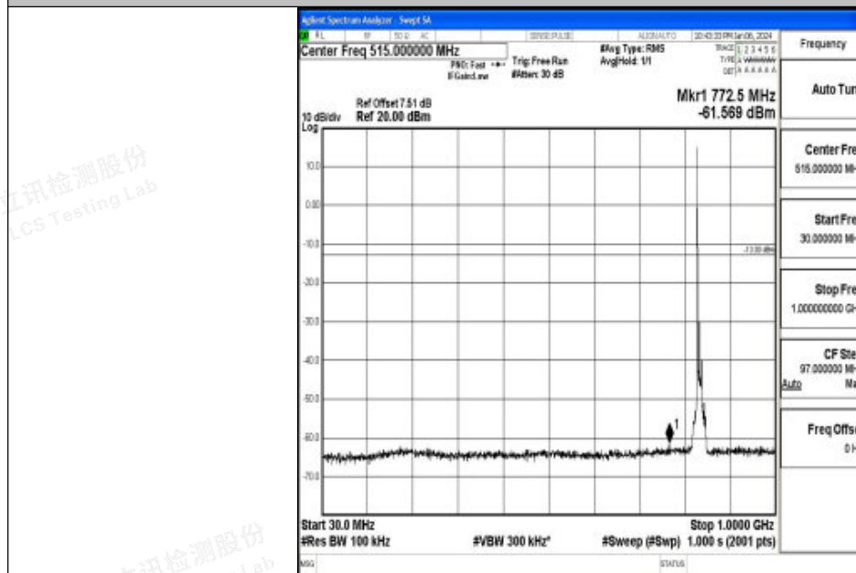
Band26_10MHz_16QAM_26915_1RB#0_30~1000_30~1000
