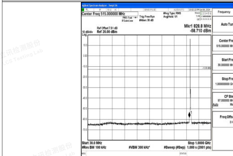
Band26_3MHz_16QAM_26915_1RB#0_30~1000_30~1000
