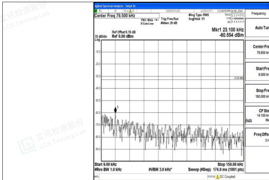
Band26_15MHz_QPSK_26915_1RB#0_0.009~0.15_0.009~0.15
