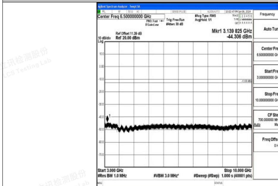
Band26_3MHz_16QAM_26915_1RB#0_3000~10000_3000~10000
