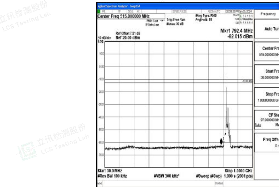
Band26_15MHz_QPSK_26865_1RB#0_30~1000_30~1000
