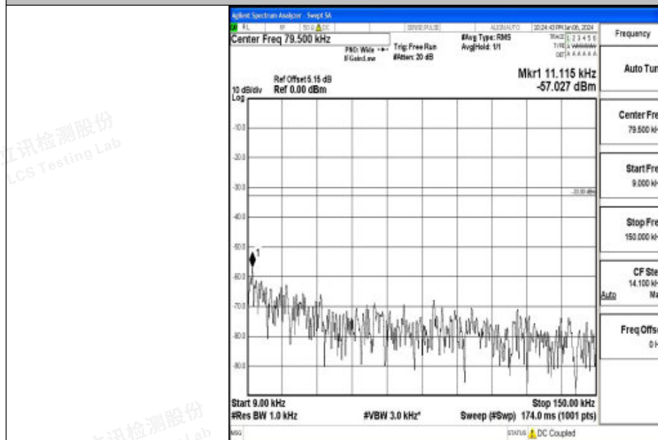
Band26_5MHz_16QAM_27015_1RB#0_0.009~0.15_0.009~0.15
