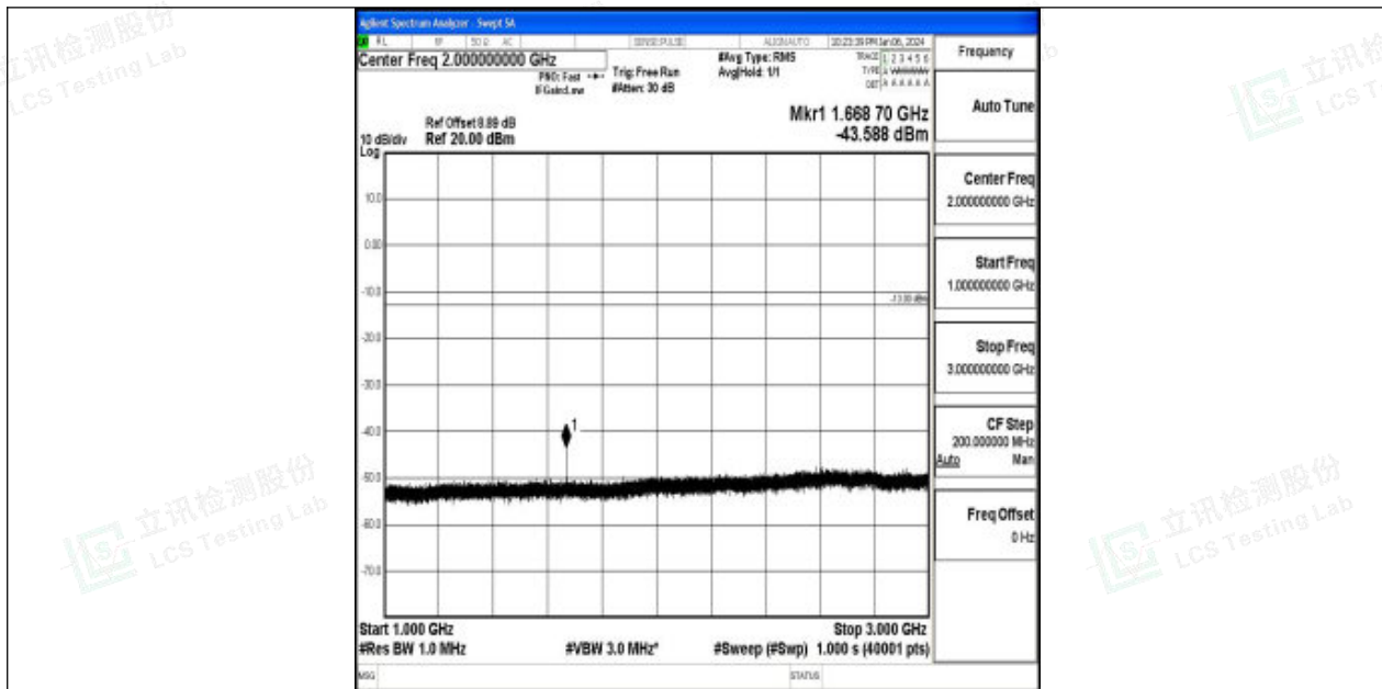
Band26_5MHz_16QAM_26915_1RB#0_1000~3000_1000~3000
