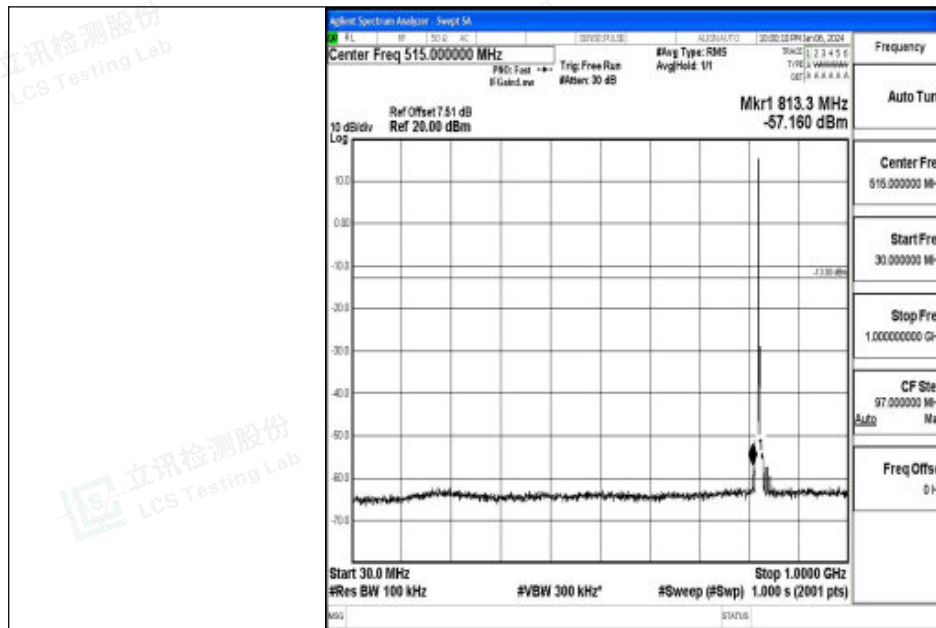
Band26_3MHz_QPSK_26805_1RB#0_30~1000_30~1000
