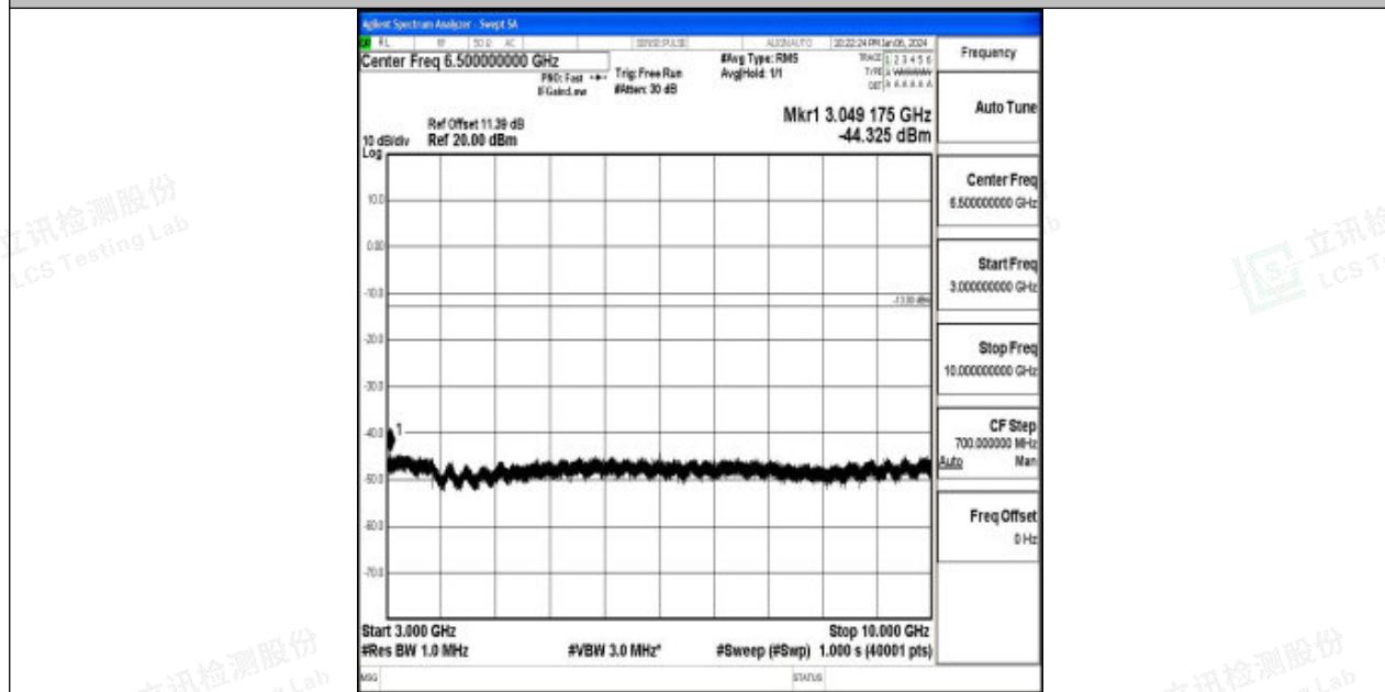
Band26_5MHz_16QAM_26815_1RB#0_3000~10000_3000~10000
