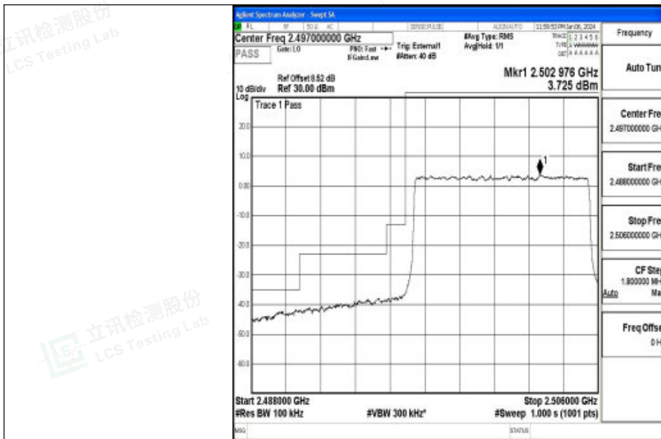
Band41_10MHz_16QAM_39700_50RB#0
