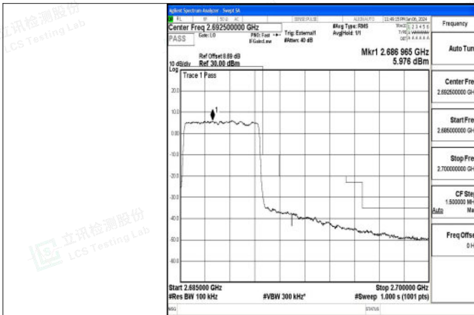
Band41_5MHz_16QAM_41565_25RB#0
