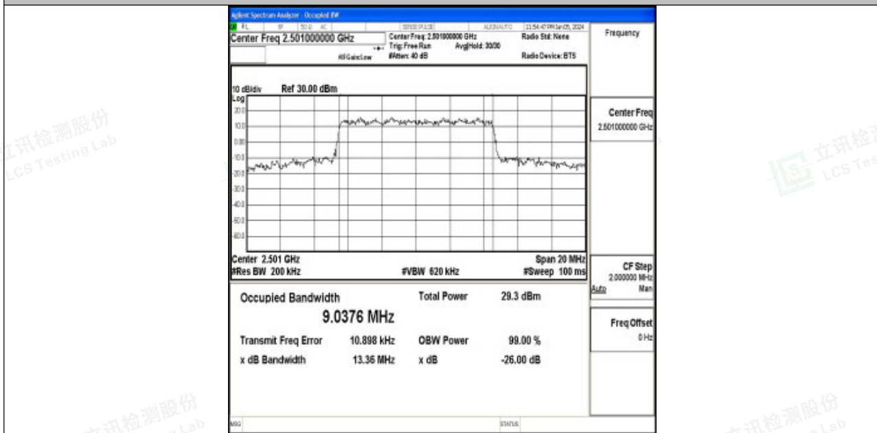
Band41-10MHz-QPSK-39700-50RB#0-PASS
