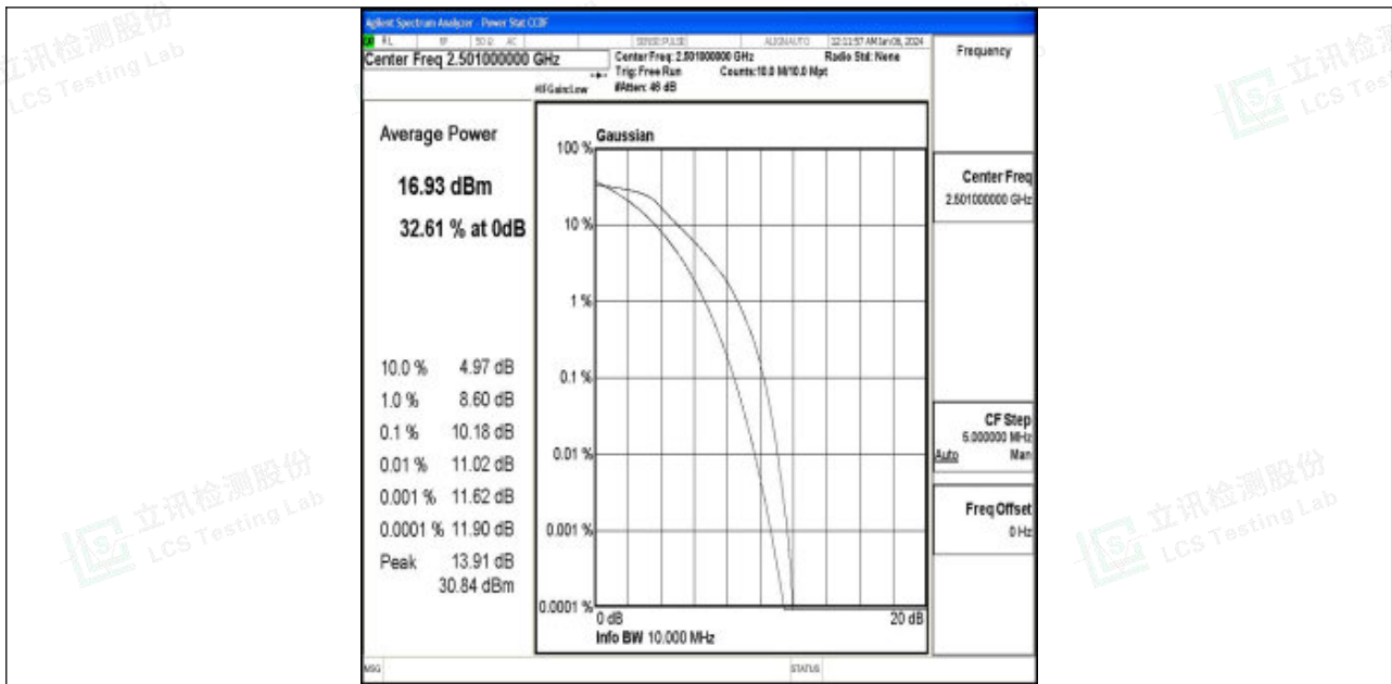
Band41-10MHz-QPSK-39700-50RB#0-PASS
