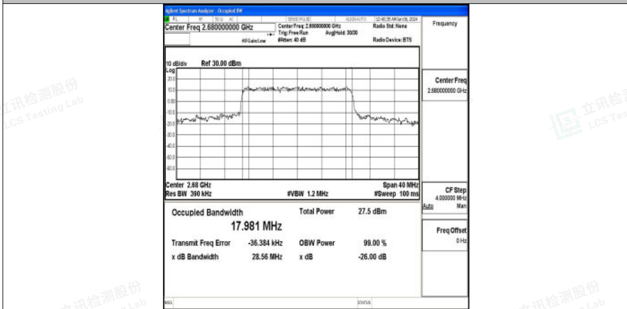
Band41-20MHz-16QAM-41490-100RB#0-PASS
