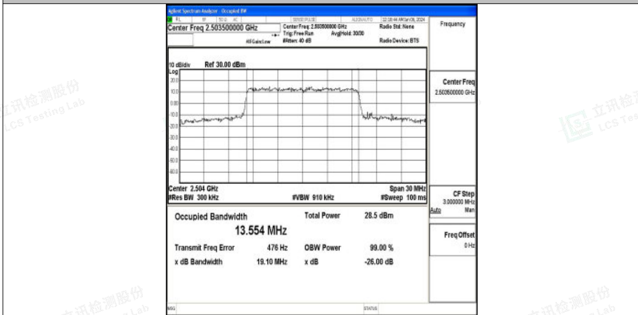
Band41-15MHz-16QAM-39725-75RB#0-PASS
