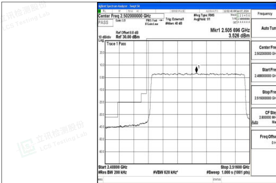
Band41_20MHz_16QAM_39750_100RB#0
