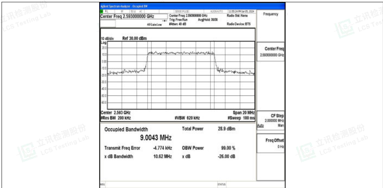
Band41-10MHz-16QAM-40620-50RB#0-PASS
