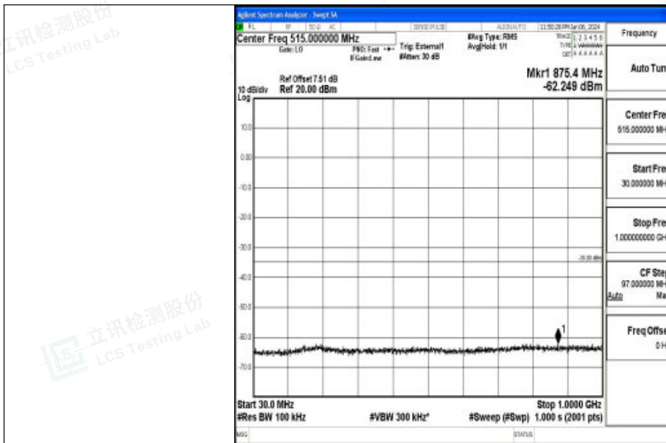
Band41_5MHz_QPSK_39675_1RB#0_30~1000_30~1000
