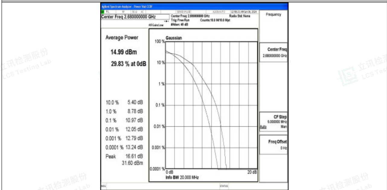
Band41-20MHz-16QAM-41490-100RB#0-PASS
