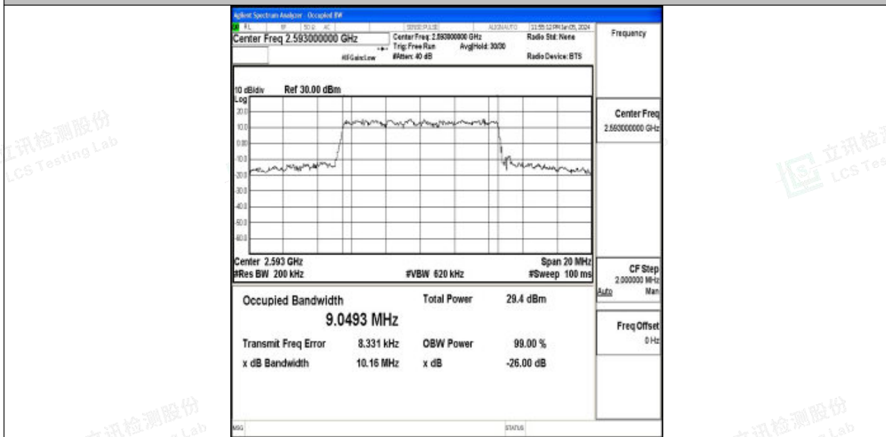
Band41-10MHz-QPSK-40620-50RB#0-PASS
