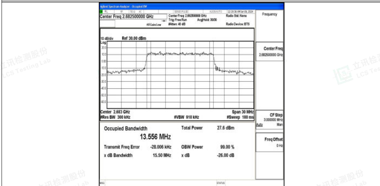
Band41-15MHz-16QAM-41515-75RB#0-PASS
