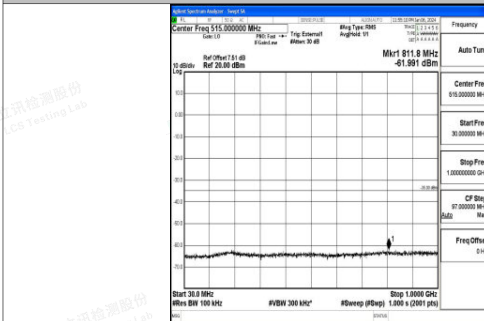
Band41_5MHz_16QAM_40620_1RB#0_30~1000_30~1000
