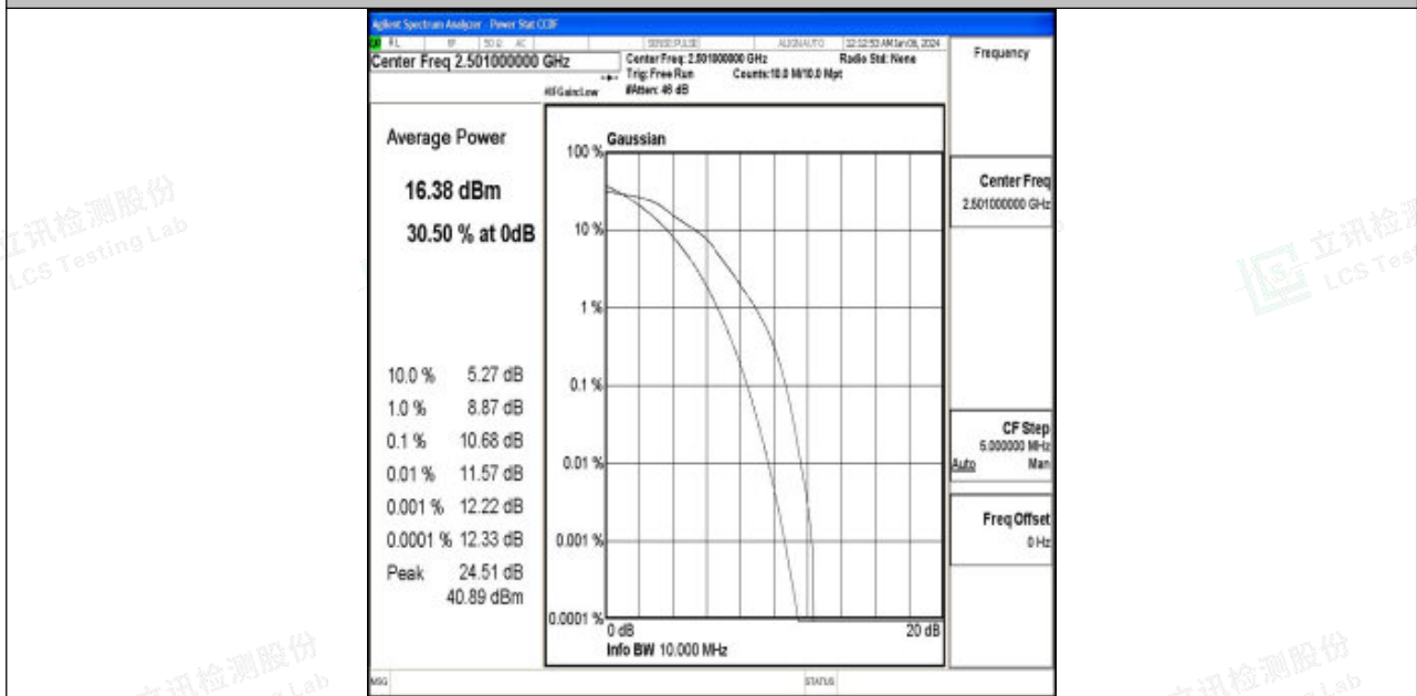
Band41-10MHz-16QAM-39700-50RB#0-PASS
