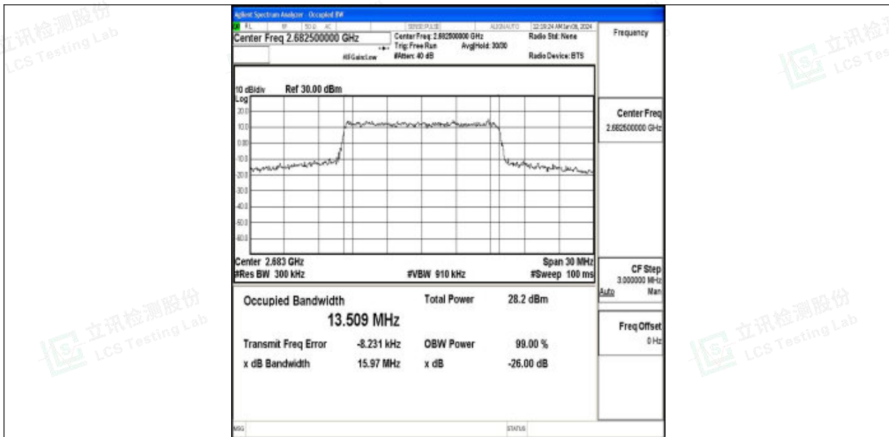
Band41-15MHz-QPSK-41515-75RB#0-PASS
