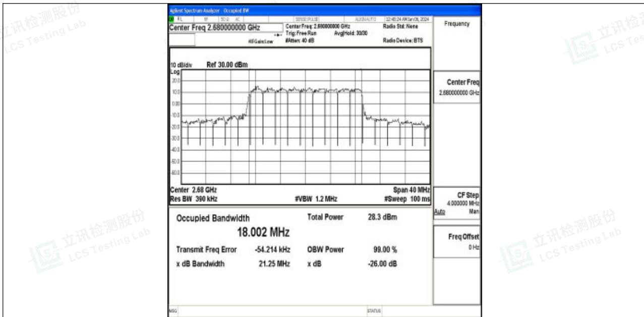
Band41-20MHz-QPSK-41490-100RB#0-PASS
