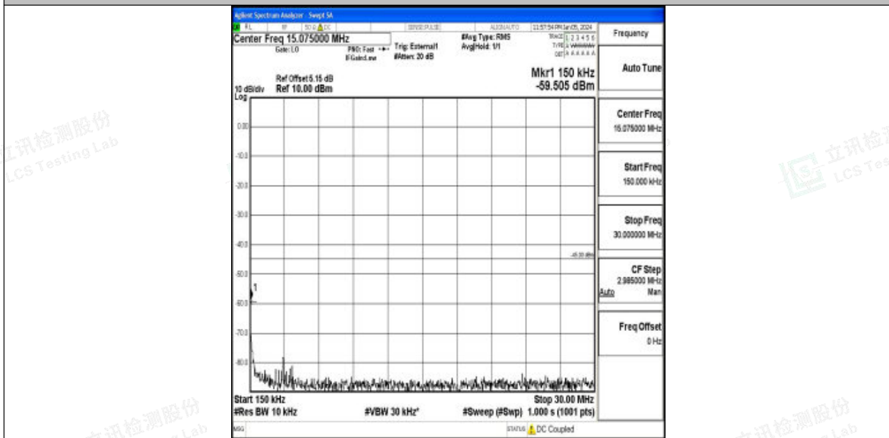
Band41_10MHz_QPSK_39700_1RB#0_0.15~30_0.15~30
