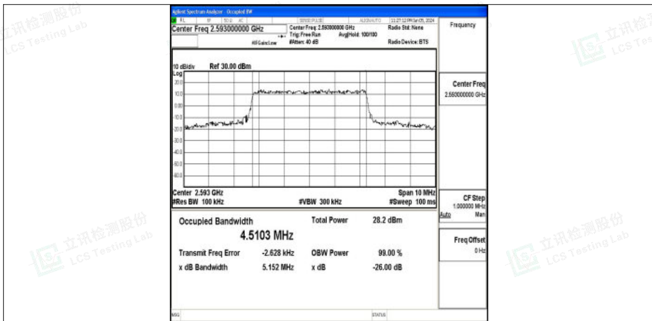
Band41-5MHz-16QAM-40620-25RB#0-PASS
