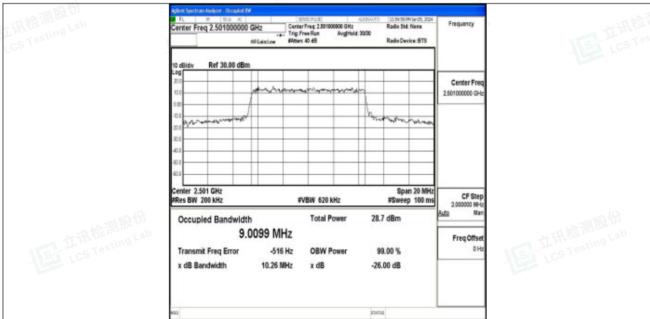
Band41-10MHz-16QAM-39700-50RB#0-PASS
