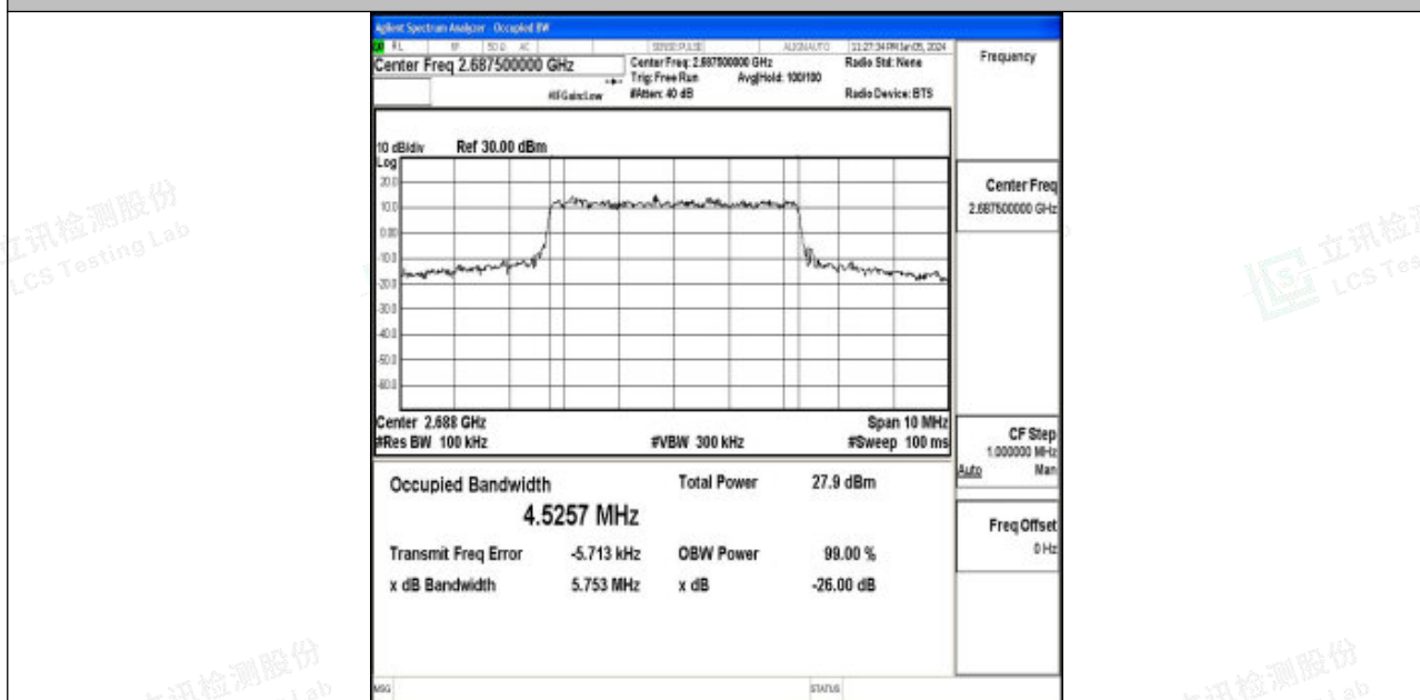
Band41-5MHz-QPSK-41565-25RB#0-PASS
