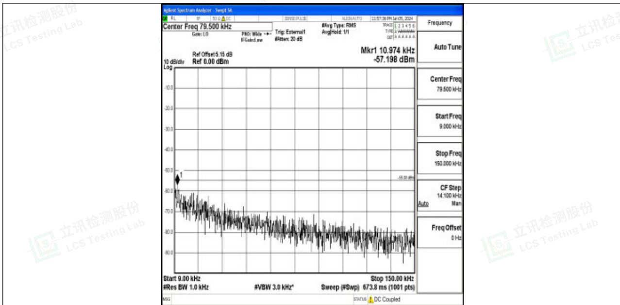
Band41_10MHz_QPSK_39700_1RB#0_0.009~0.15_0.009~0.15
