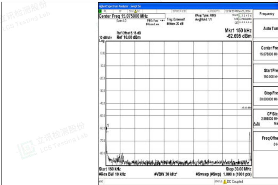
Band41_5MHz_16QAM_40620_1RB#0_0.15~30_0.15~30
