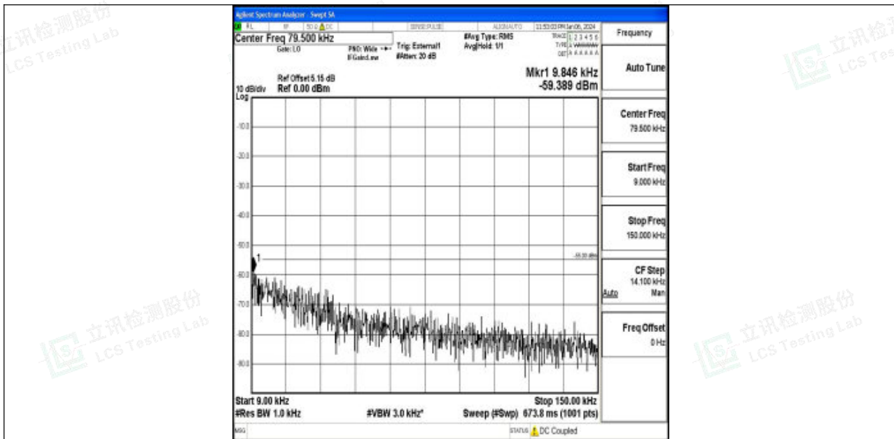
Band41_5MHz_QPSK_40620_1RB#0_0.009~0.15_0.009~0.15
