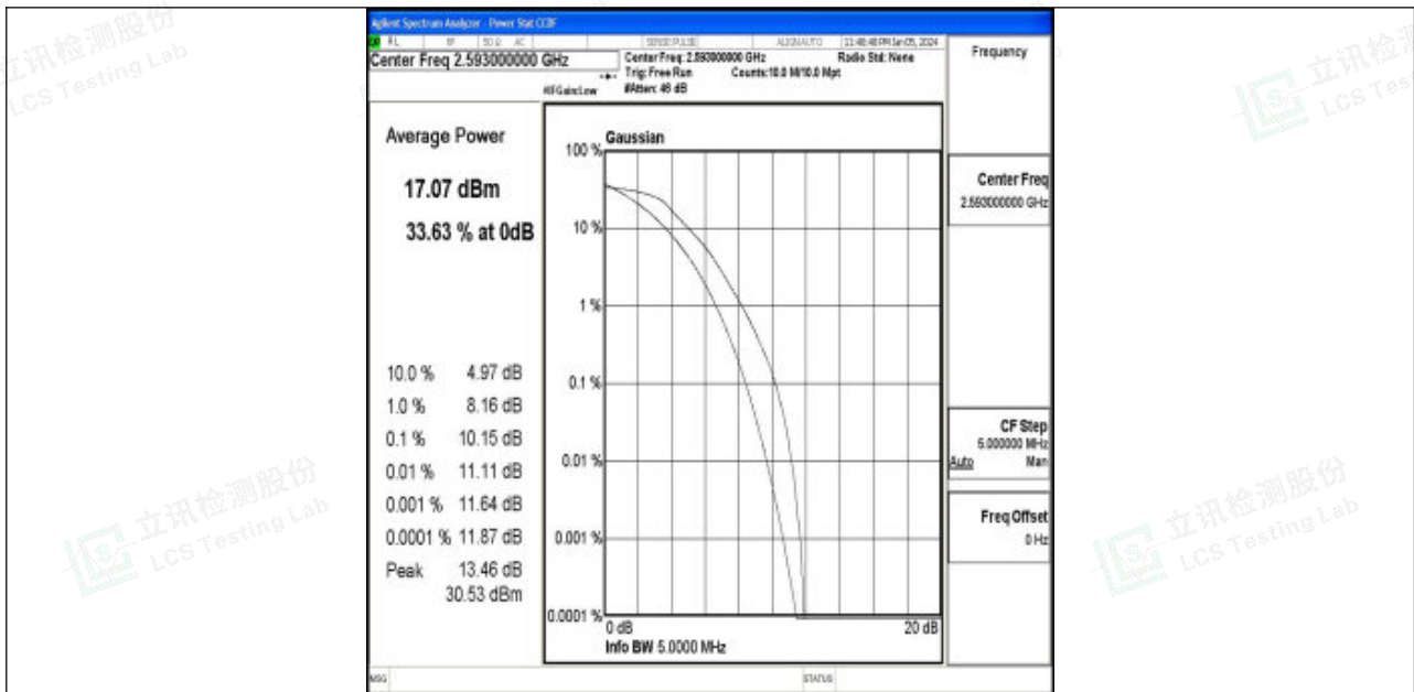
Band41-5MHz-QPSK-40620-25RB#0-PASS
