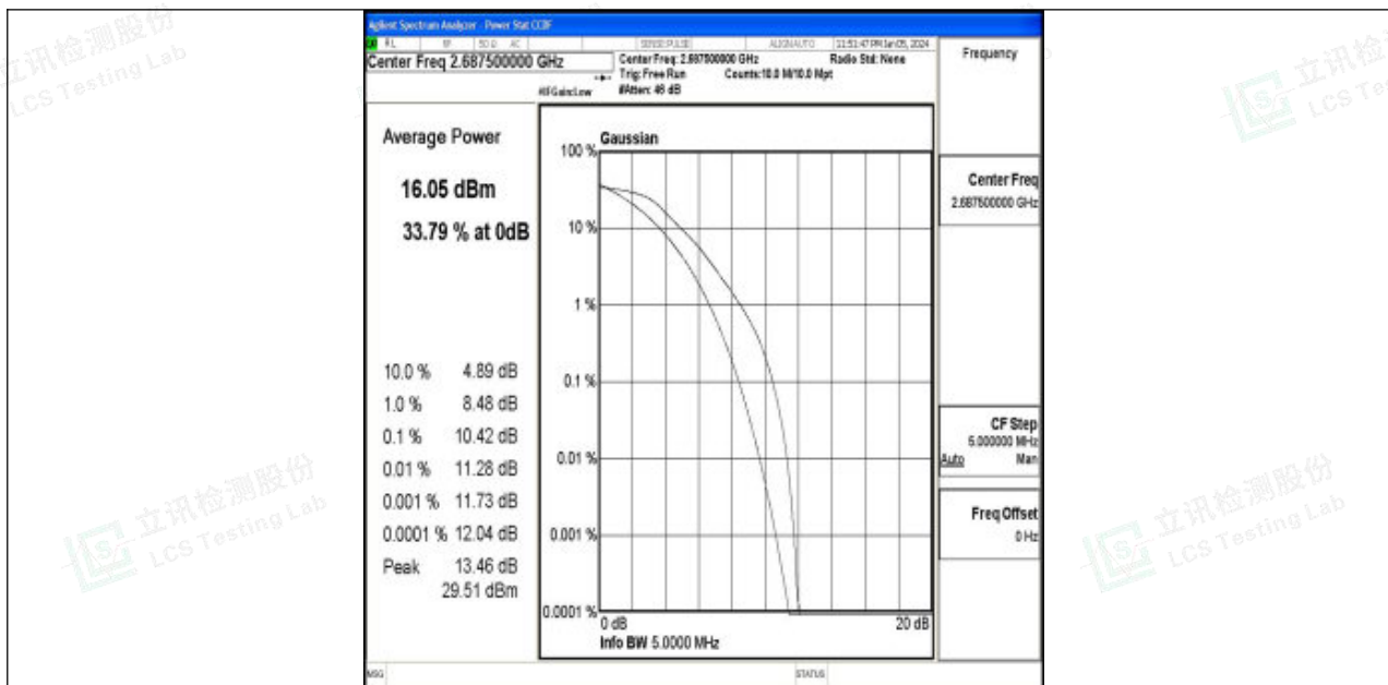
Band41-5MHz-QPSK-41565-25RB#0-PASS
