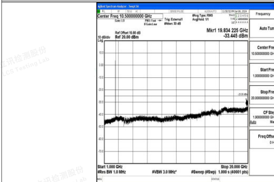
Band41_5MHz_QPSK_39675_1RB#0_1000~20000_1000~20000
