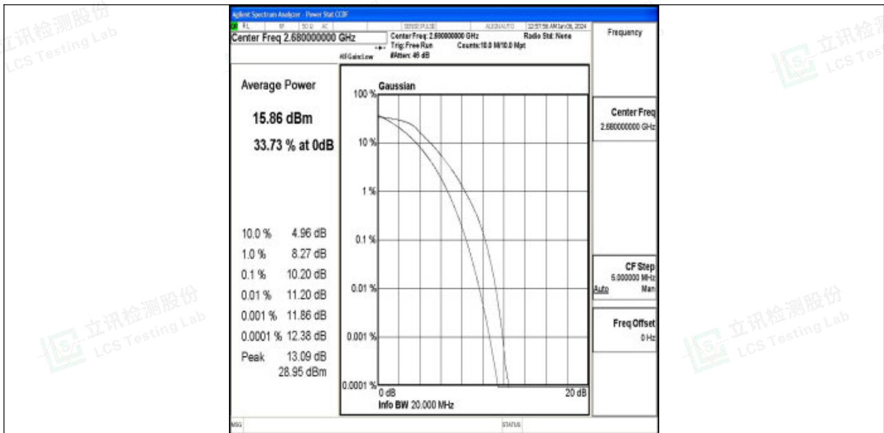
Band41-20MHz-QPSK-41490-100RB#0-PASS
