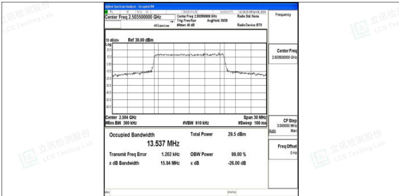
Band41-15MHz-QPSK-39725-75RB#0-PASS
