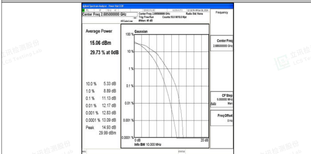
Band41-10MHz-16QAM-41540-50RB#0-PASS
