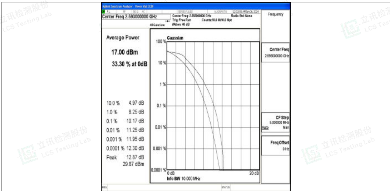
Band41-10MHz-QPSK-40620-50RB#0-PASS
