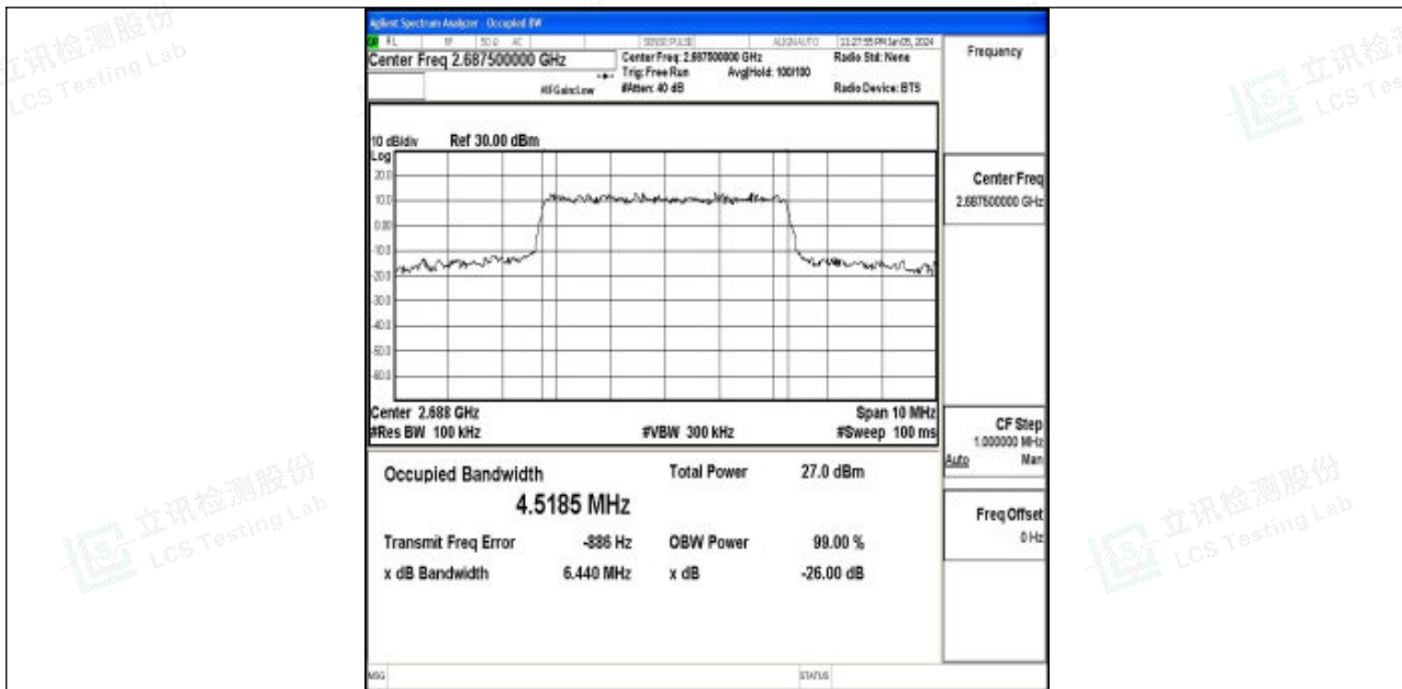
Band41-5MHz-16QAM-41565-25RB#0-PASS
