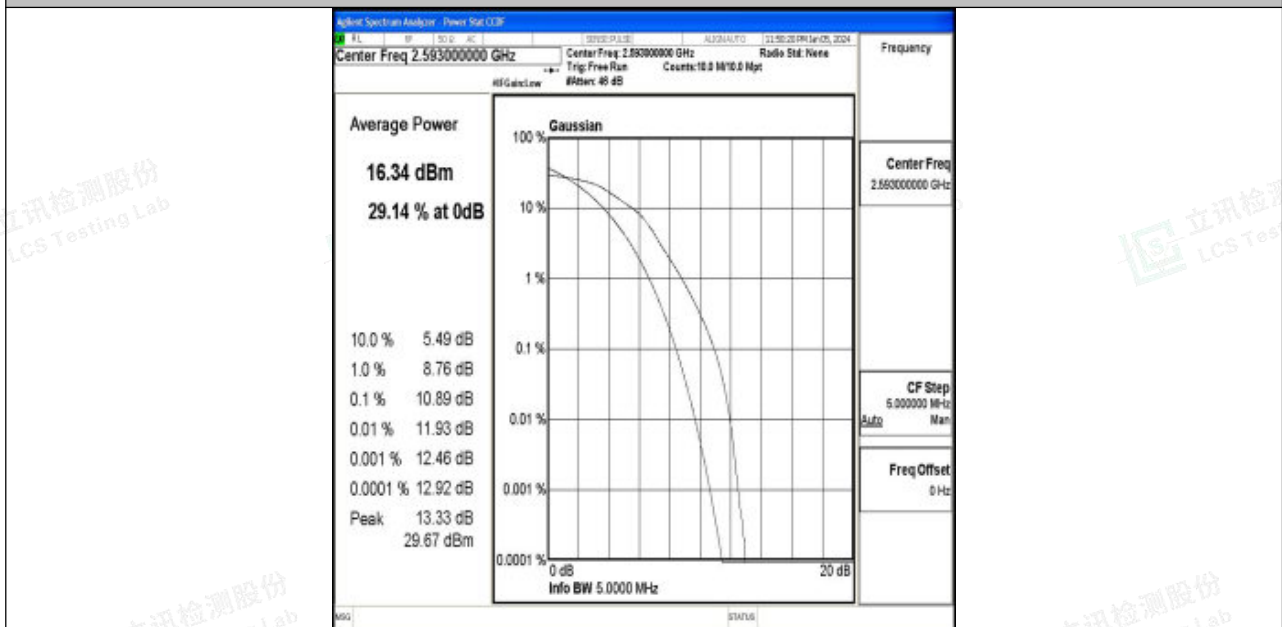
Band41-5MHz-16QAM-40620-25RB#0-PASS
