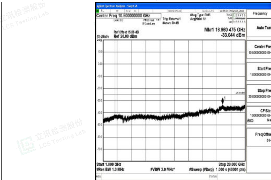
Band41_5MHz_16QAM_40620_1RB#0_1000~20000_1000~20000
