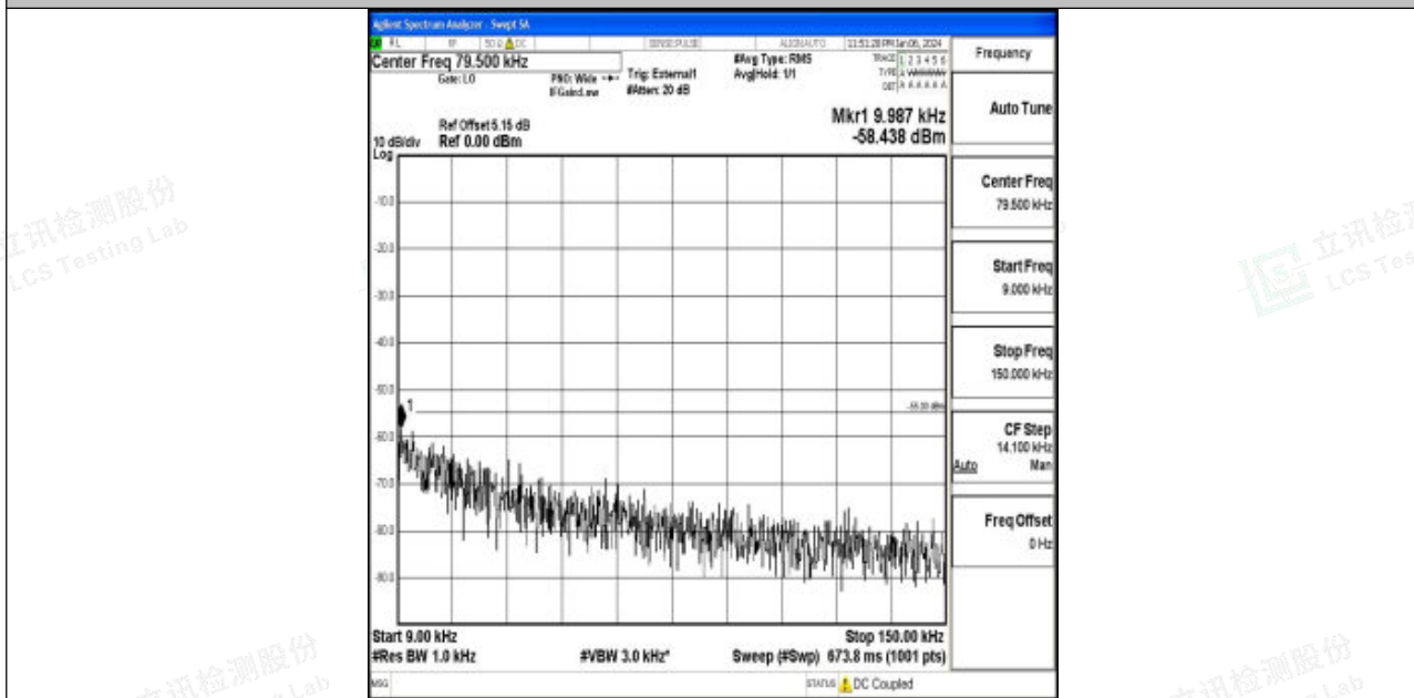
Band41_5MHz_16QAM_39675_1RB#0_0.009~0.15_0.009~0.15
