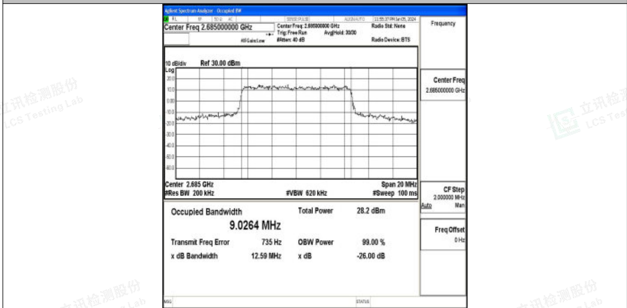
Band41-10MHz-QPSK-41540-50RB#0-PASS
