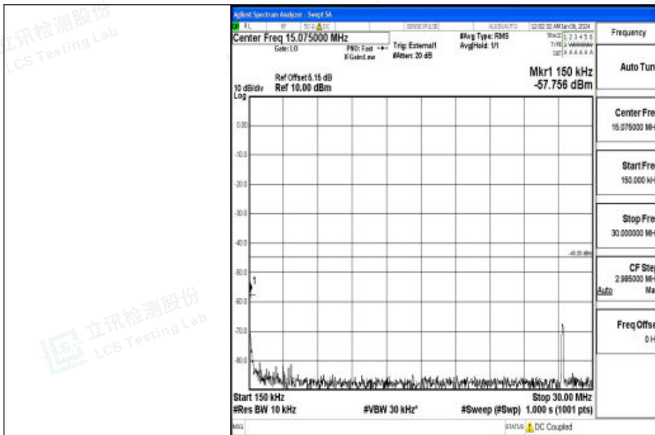
Band41_10MHz_16QAM_40620_1RB#0_0.15~30_0.15~30
