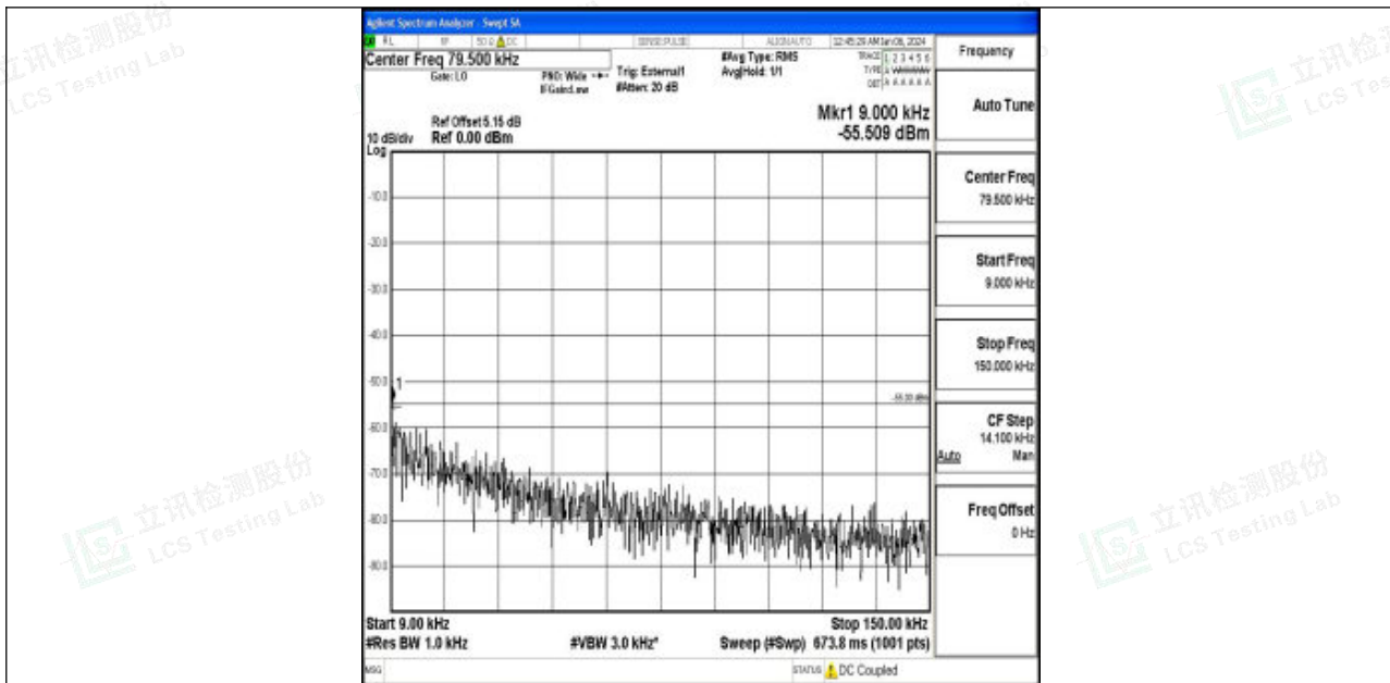
Band41_20MHz_QPSK_40620_1RB#0_0.009~0.15_0.009~0.15
