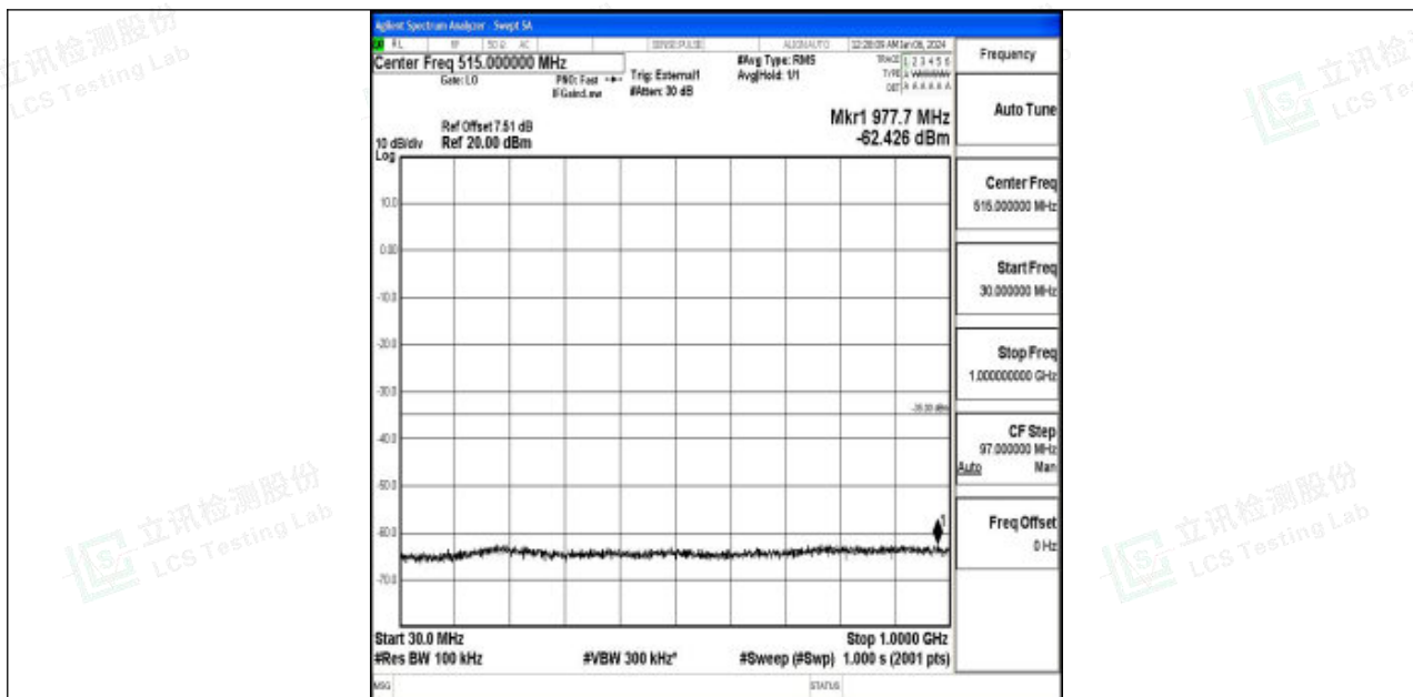
Band41_15MHz_QPSK_41515_1RB#0_30~1000_30~1000
