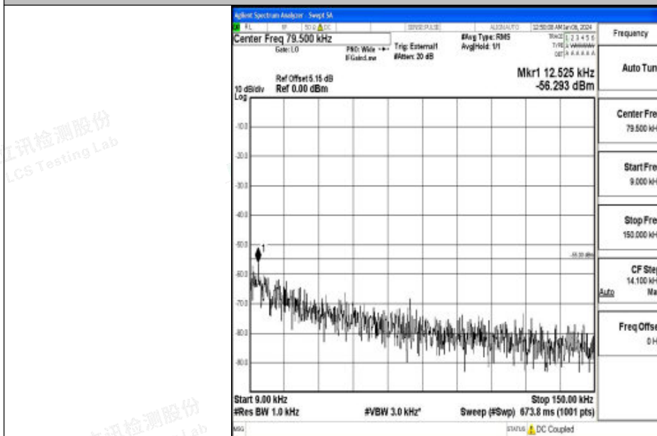
Band41_20MHz_16QAM_41490_1RB#0_0.009~0.15_0.009~0.15
