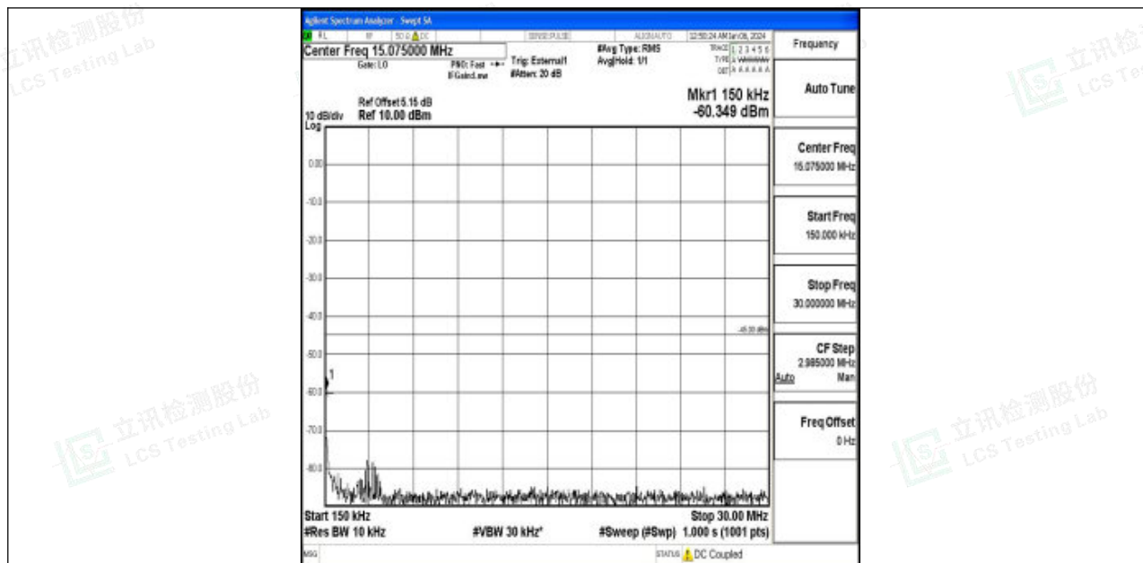
Band41_20MHz_16QAM_41490_1RB#0_0.15~30_0.15~30
