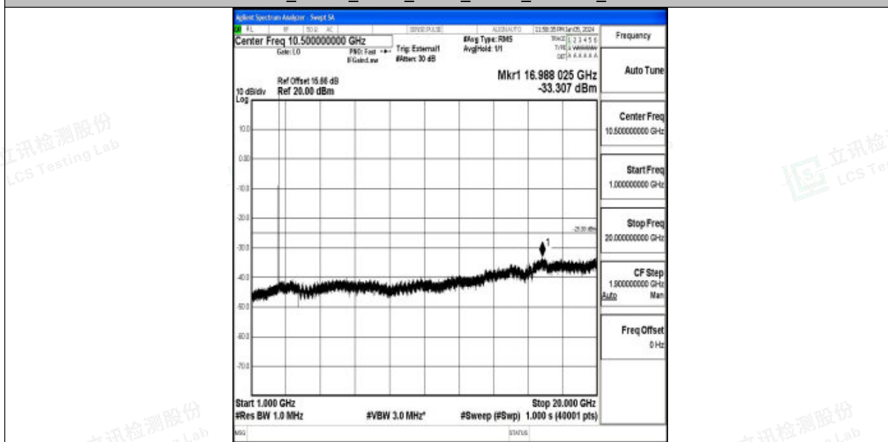
Band41_10MHz_QPSK_39700_1RB#0_1000~20000_1000~20000
