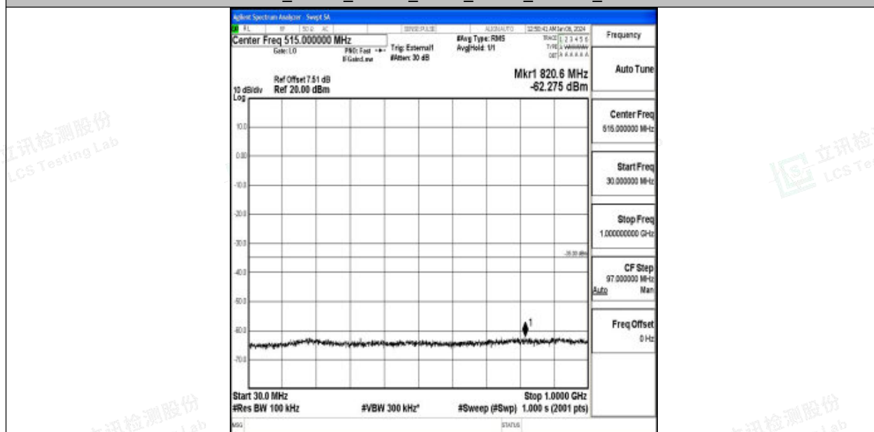
Band41_20MHz_16QAM_41490_1RB#0_30~1000_30~1000
