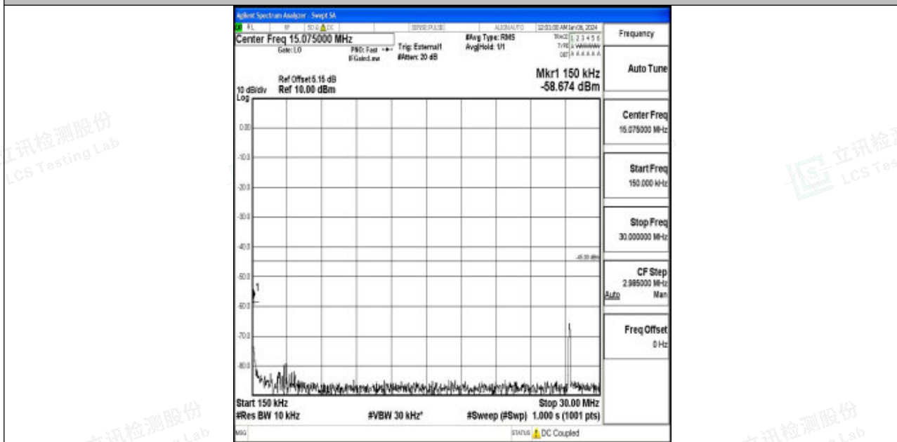
Band41_10MHz_QPSK_40620_1RB#0_0.15~30_0.15~30
