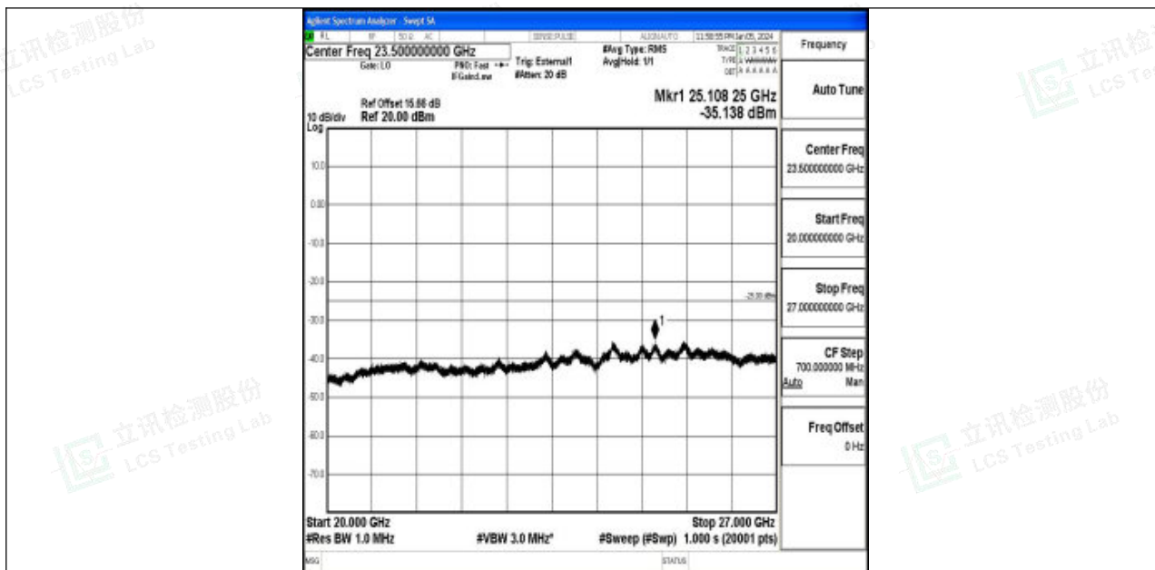
Band41_10MHz_QPSK_39700_1RB#0_20000~27000_20000~27000
