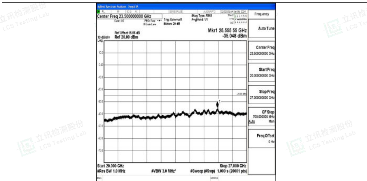
Band41_10MHz_QPSK_40620_1RB#0_20000~27000_20000~27000
