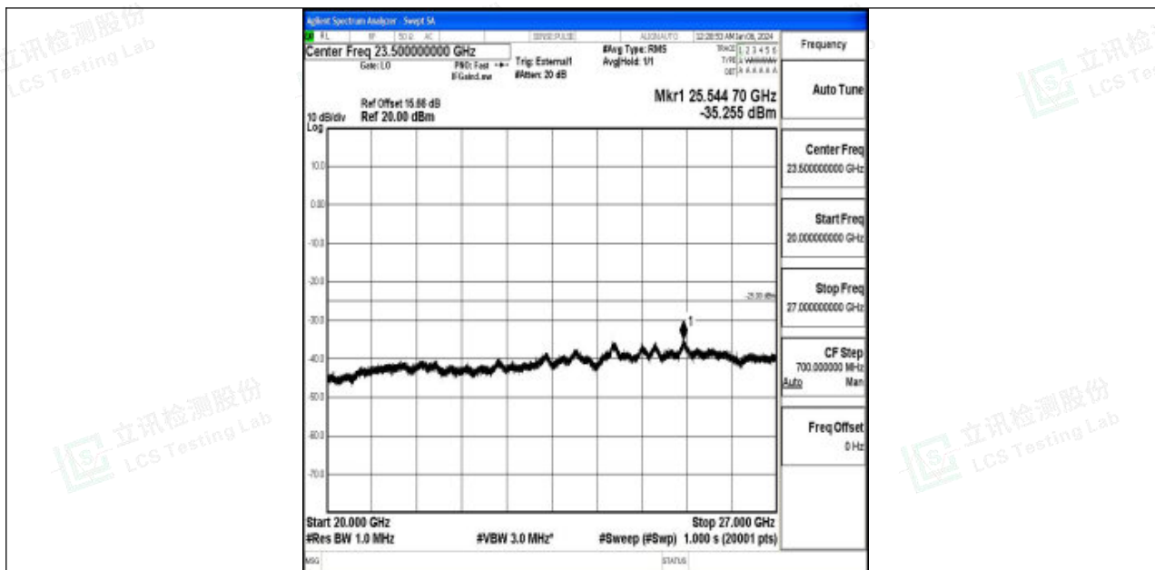
Band41_15MHz_QPSK_41515_1RB#0_20000~27000_20000~27000
