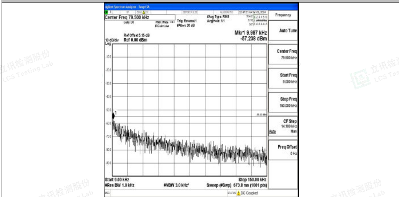
Band41_20MHz_16QAM_40620_1RB#0_0.009~0.15_0.009~0.15
