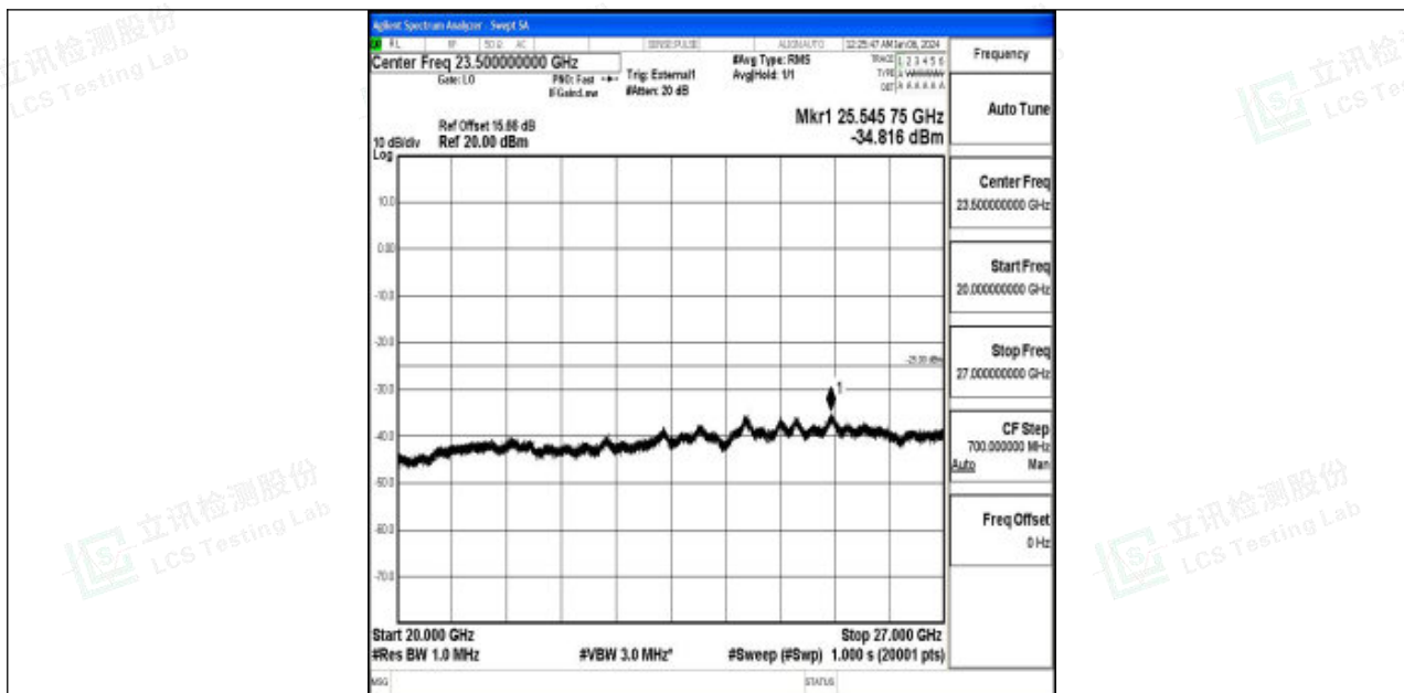
Band41_15MHz_QPSK_40620_1RB#0_20000~27000_20000~27000
