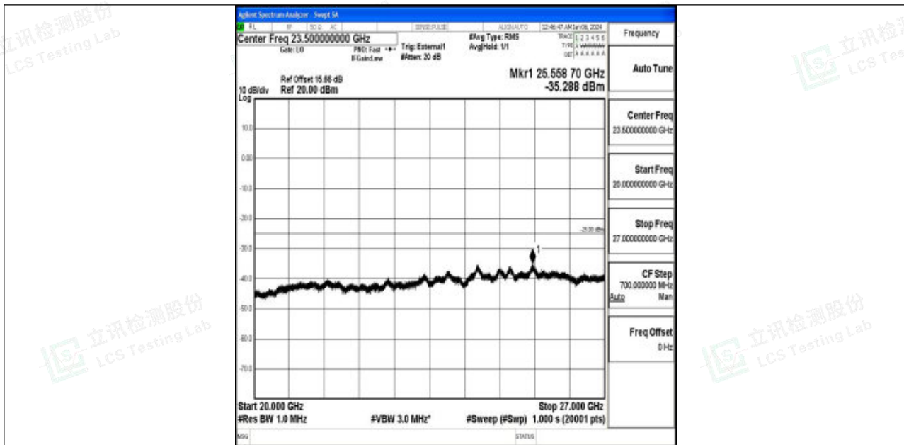
Band41_20MHz_QPSK_40620_1RB#0_20000~27000_20000~27000
