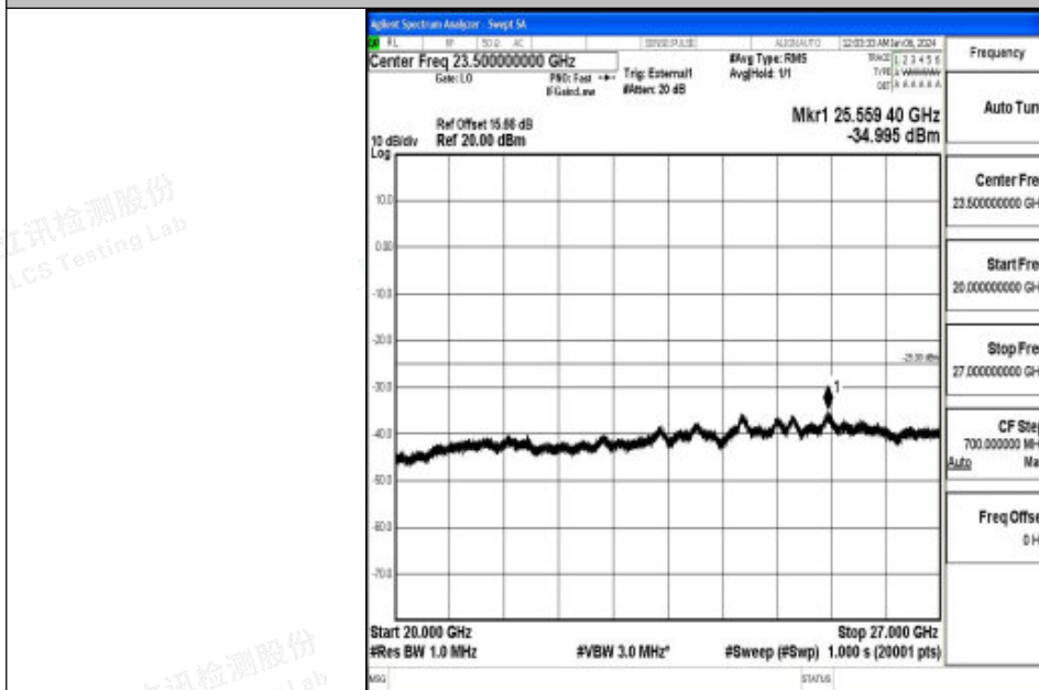
Band41_10MHz_16QAM_40620_1RB#0_20000~27000_20000~27000
