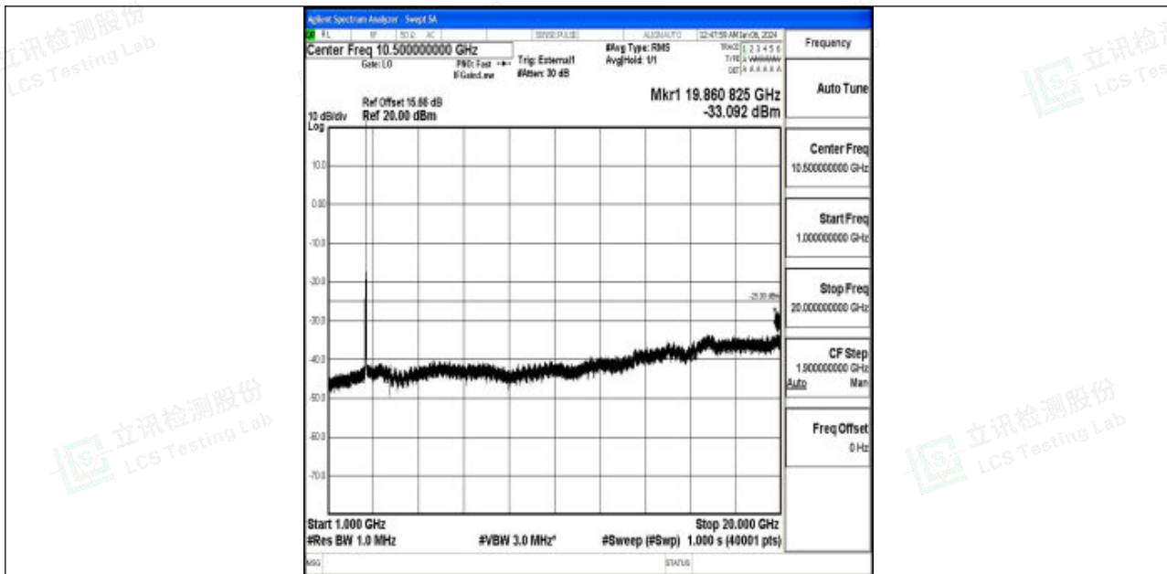
Band41_20MHz_16QAM_40620_1RB#0_1000~20000_1000~20000
