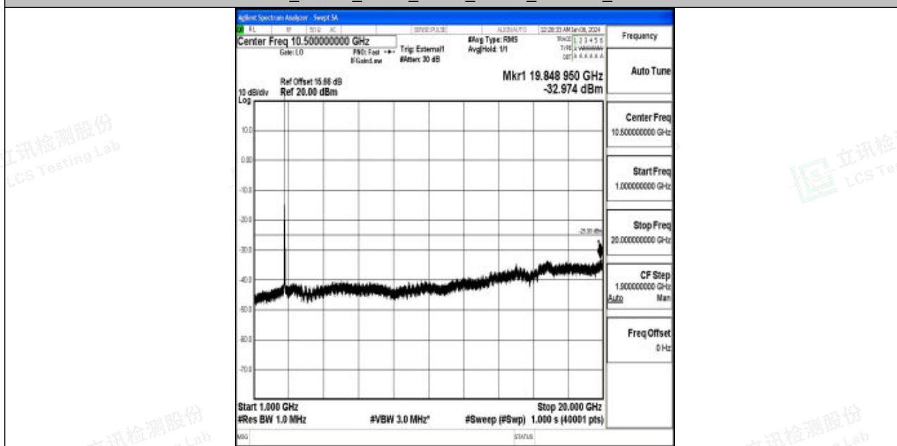
Band41_15MHz_QPSK_41515_1RB#0_1000~20000_1000~20000
