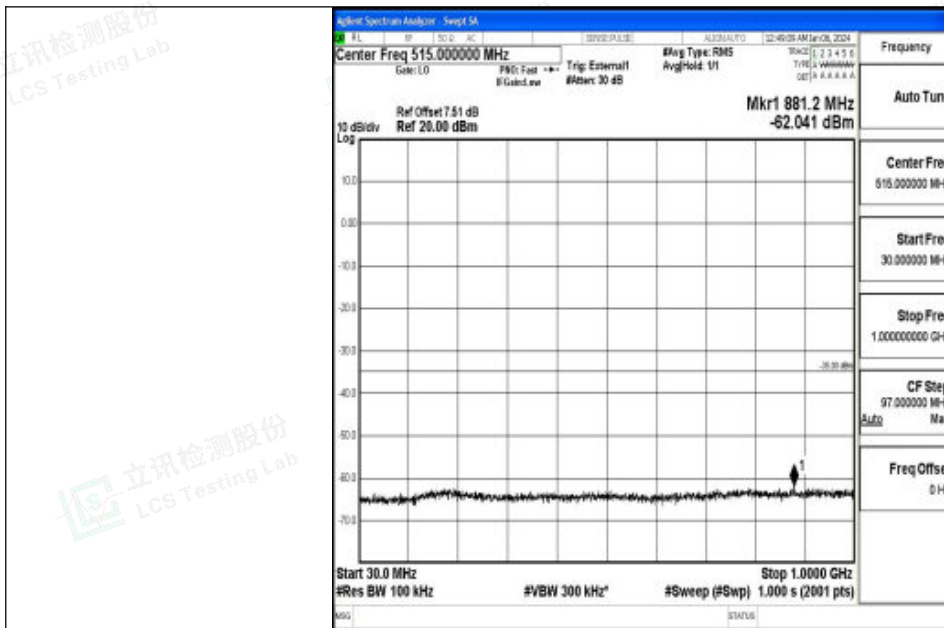
Band41_20MHz_QPSK_41490_1RB#0_30~1000_30~1000
