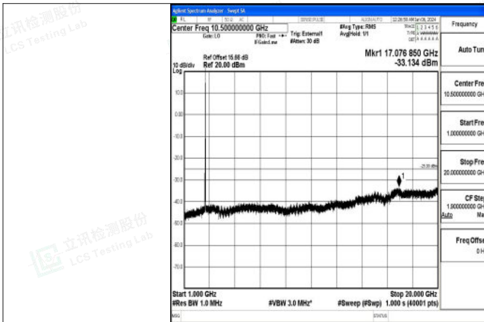
Band41_15MHz_16QAM_40620_1RB#0_1000~20000_1000~20000
