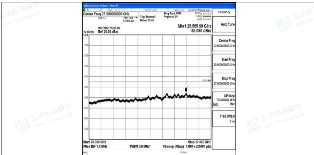
Band41_20MHz_QPSK_39750_1RB#0_20000~27000_20000~27000
