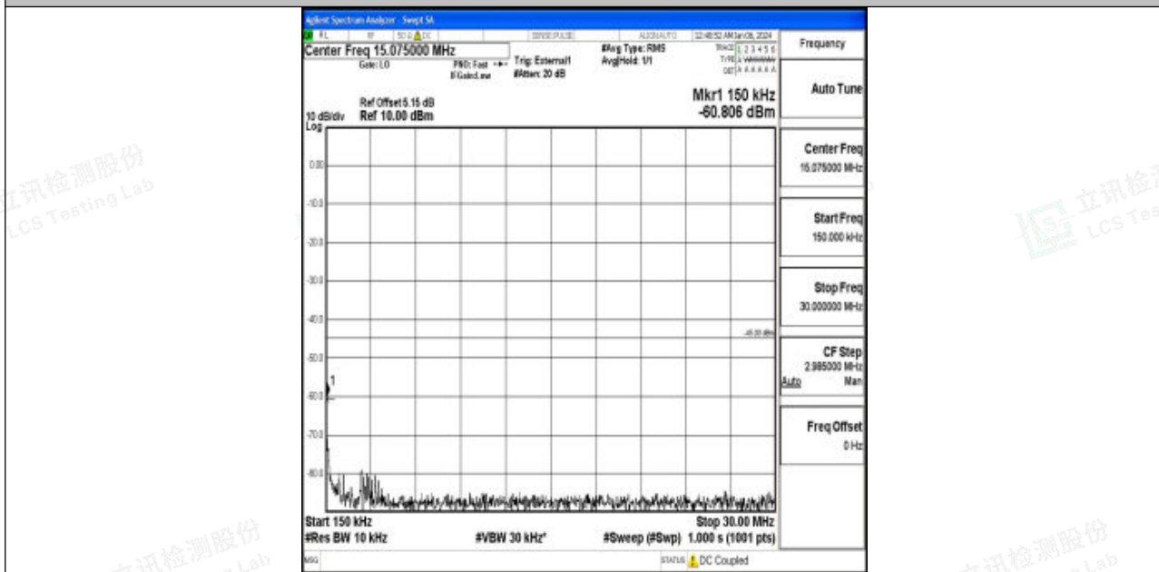
Band41_20MHz_QPSK_41490_1RB#0_0.15~30_0.15~30
