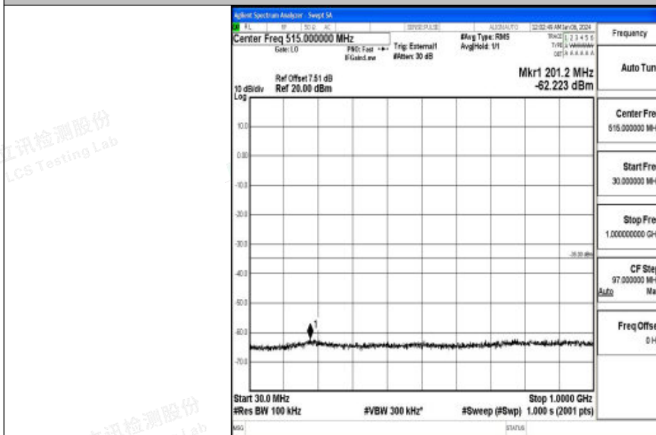
Band41_10MHz_16QAM_40620_1RB#0_30~1000_30~1000
