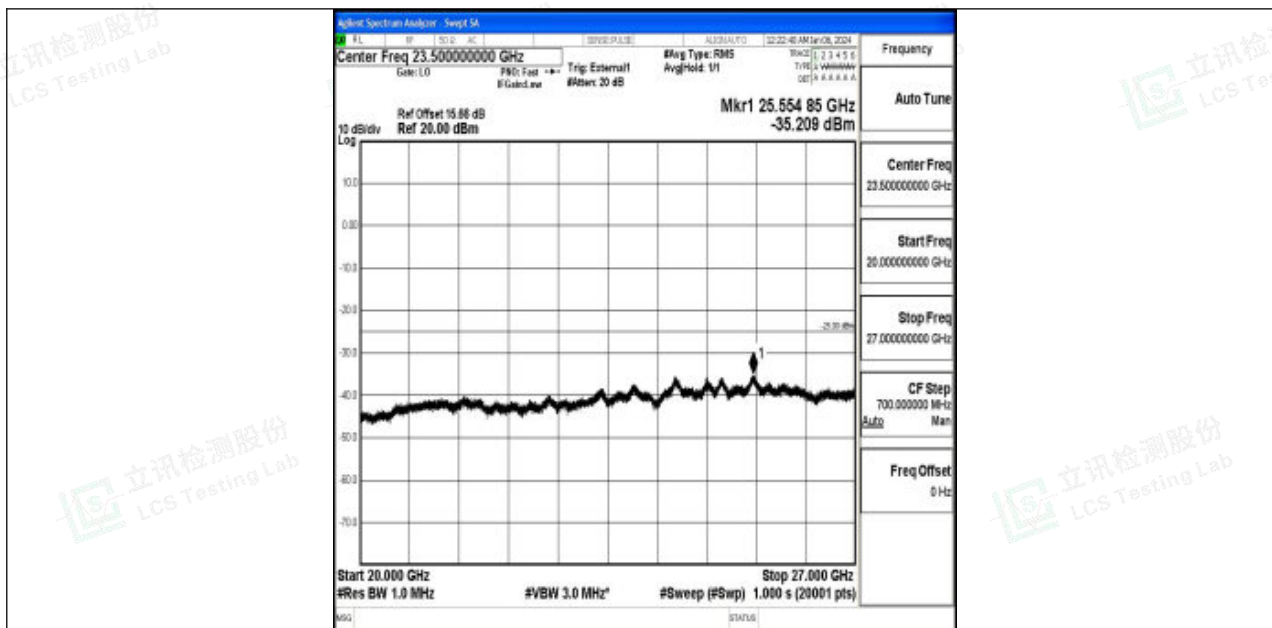
Band41_15MHz_QPSK_39725_1RB#0_20000~27000_20000~27000
