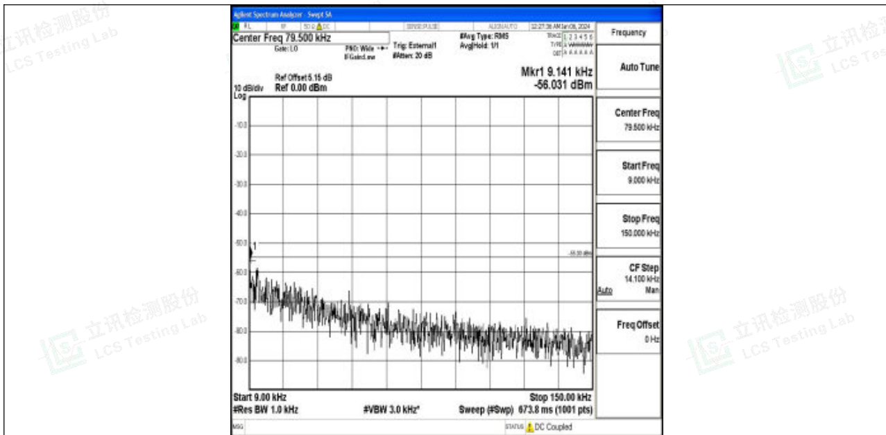
Band41_15MHz_QPSK_41515_1RB#0_0.009~0.15_0.009~0.15
