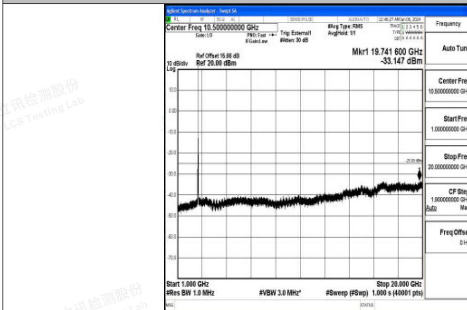
Band41_20MHz_QPSK_40620_1RB#0_1000~20000_1000~20000
