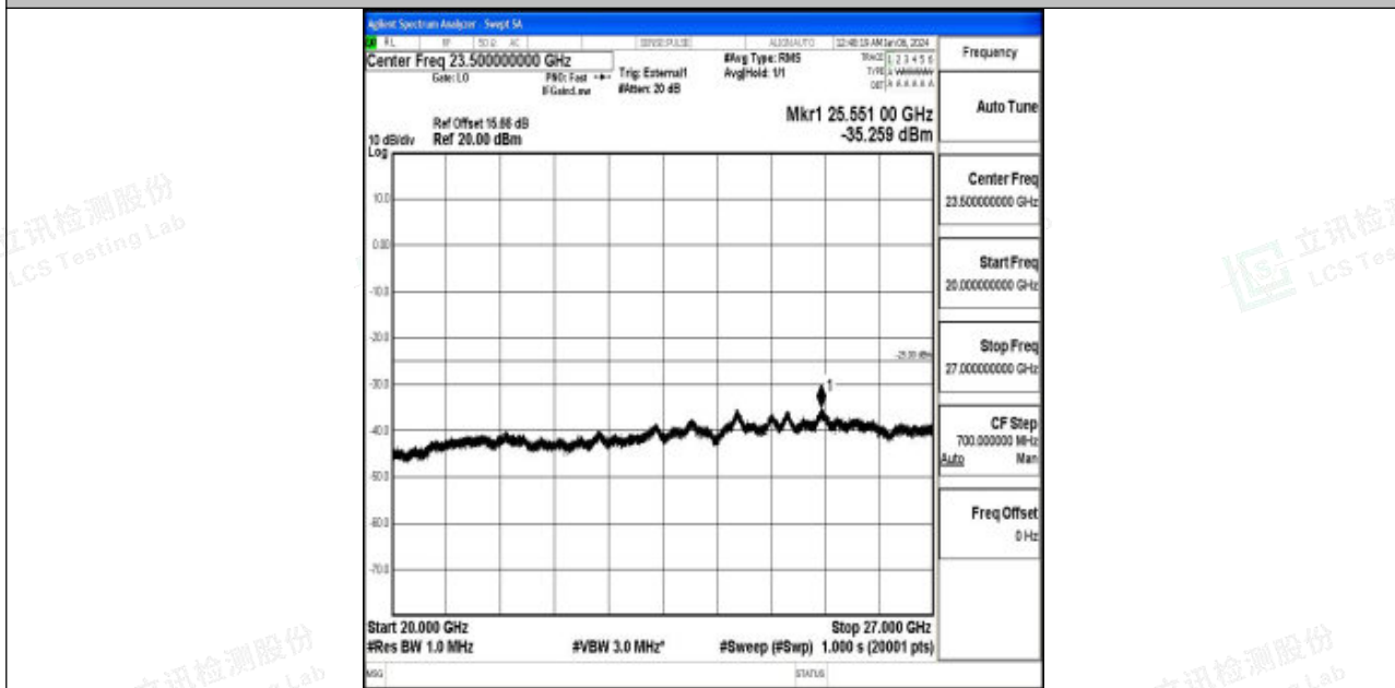
Band41_20MHz_16QAM_40620_1RB#0_20000~27000_20000~27000
