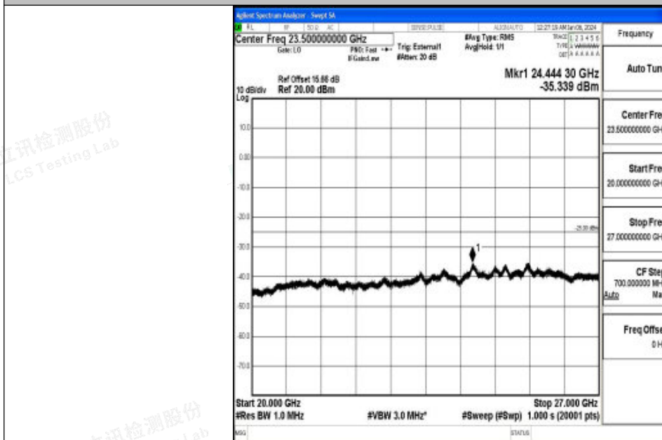
Band41_15MHz_16QAM_40620_1RB#0_20000~27000_20000~27000
