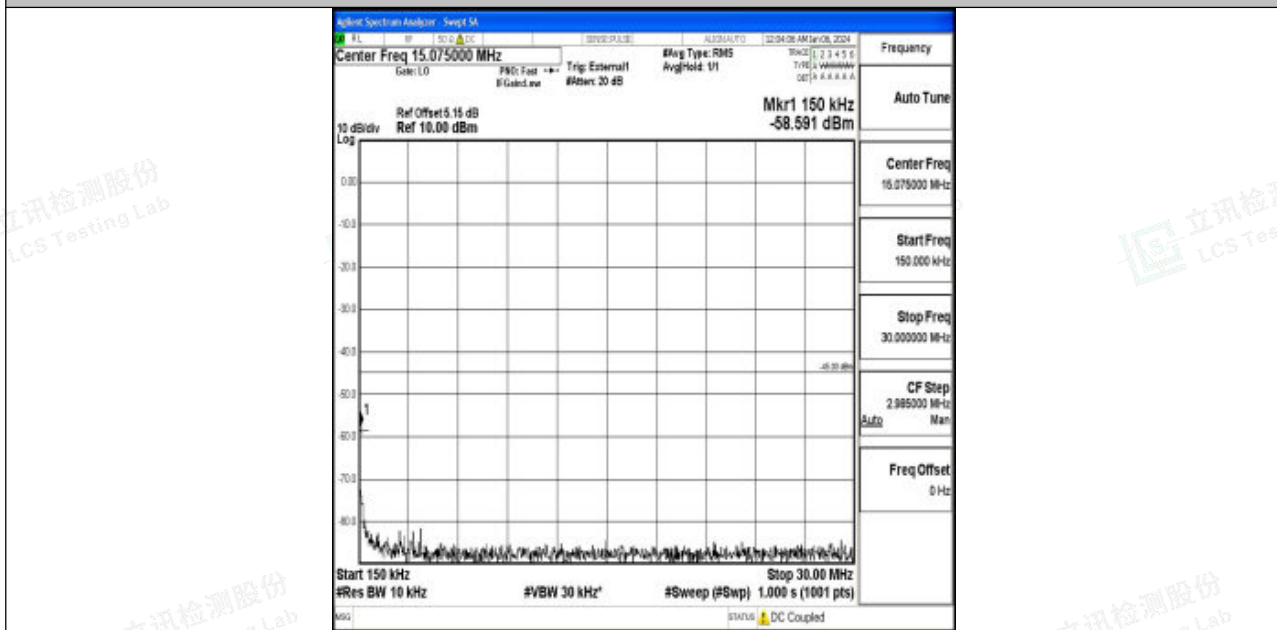
Band41_10MHz_QPSK_41540_1RB#0_0.15~30_0.15~30
