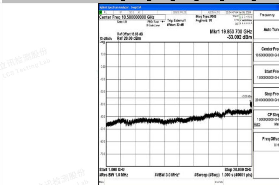
Band41_10MHz_QPSK_41540_1RB#0_1000~20000_1000~20000
