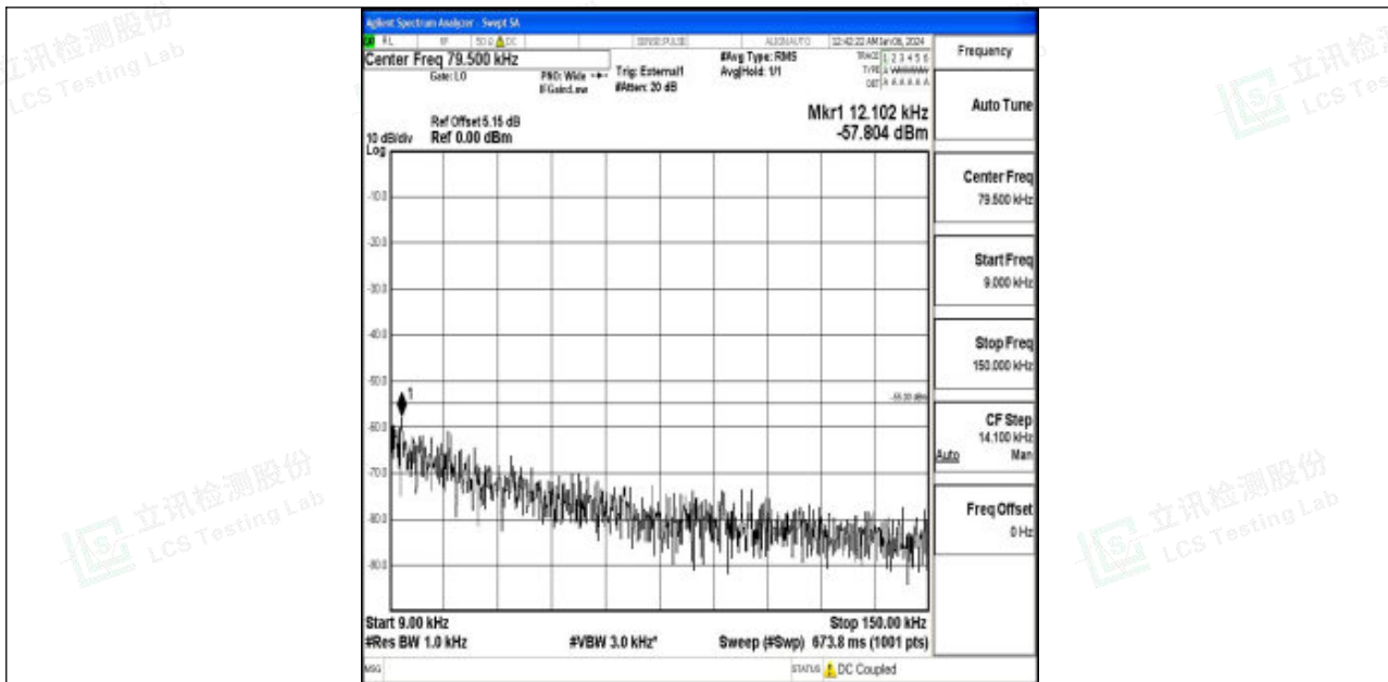
Band41_20MHz_QPSK_39750_1RB#0_0.009~0.15_0.009~0.15
