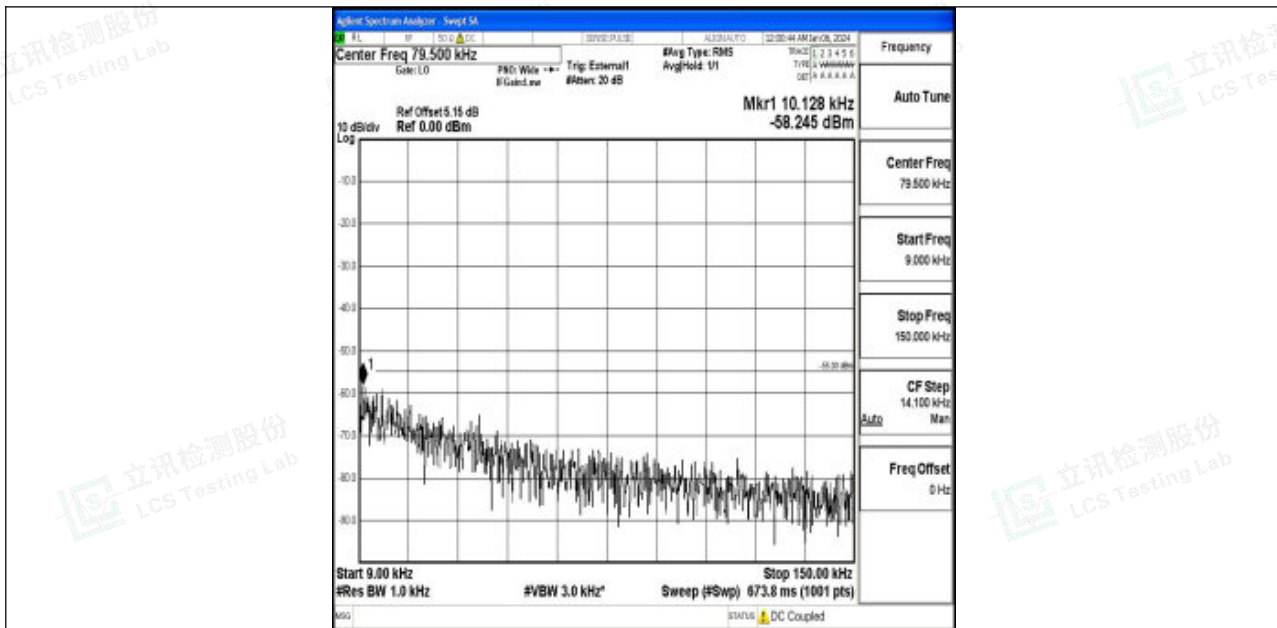
Band41_10MHz_QPSK_40620_1RB#0_0.009~0.15_0.009~0.15
