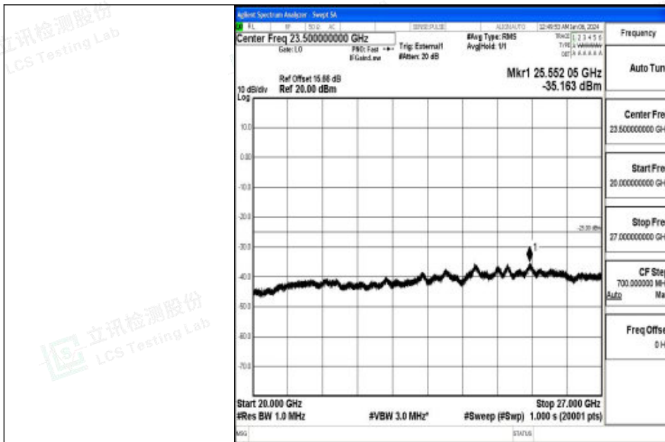
Band41_20MHz_QPSK_41490_1RB#0_20000~27000_20000~27000
