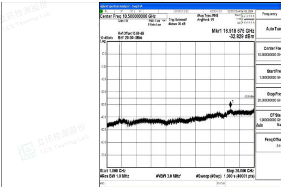
Band41_10MHz_16QAM_40620_1RB#0_1000~20000_1000~20000
