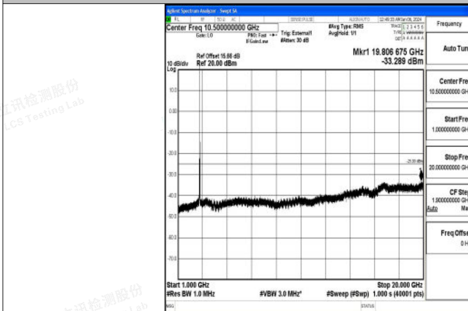
Band41_20MHz_QPSK_41490_1RB#0_1000~20000_1000~20000
