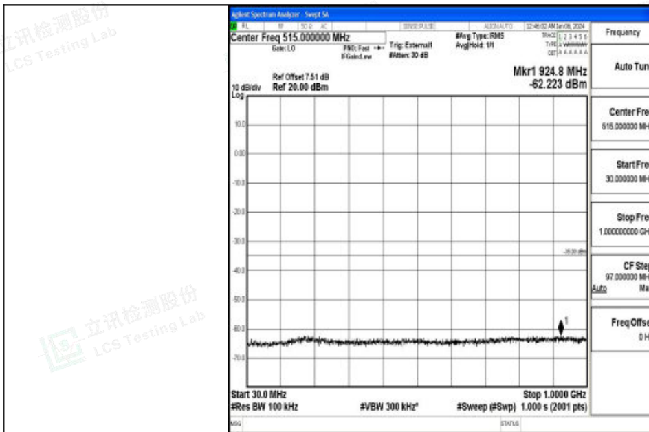
Band41_20MHz_QPSK_40620_1RB#0_30~1000_30~1000
